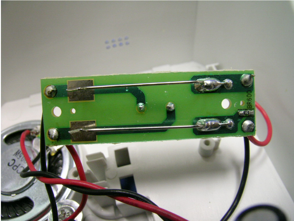
Base Unit Charging Board "2" PCB front side
