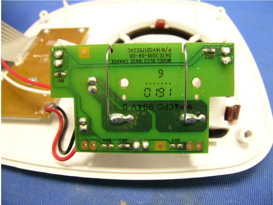
Base Unit Charging Board "1" PCB front side
