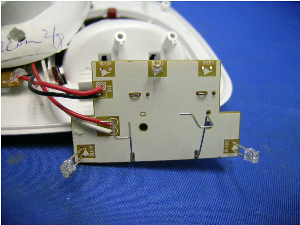
Base Unit Charging Board "1" PCB rear side
