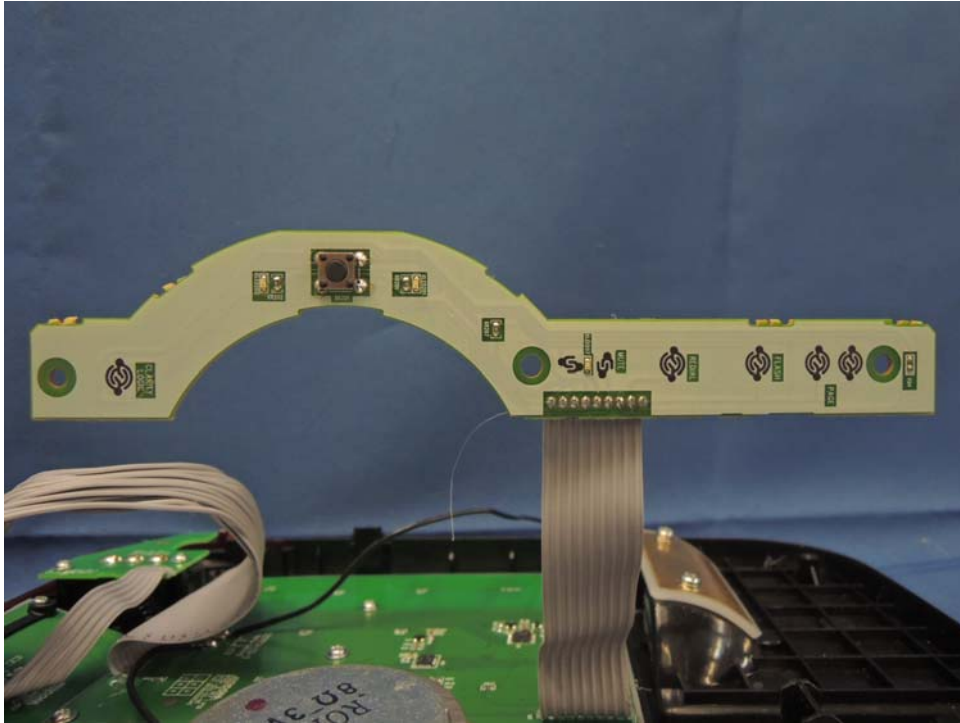
Base Unit another Keypad front side
