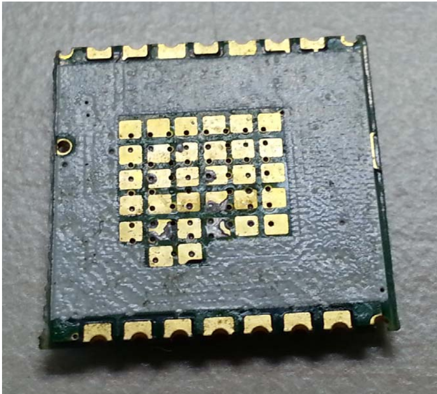
Base Unit WiFi Module solder side
