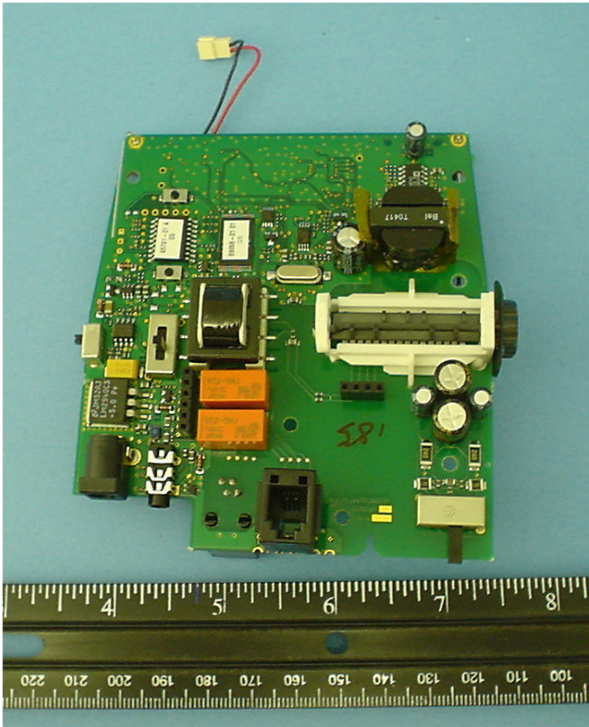
AL8CS55XXXX internal view, backside.
