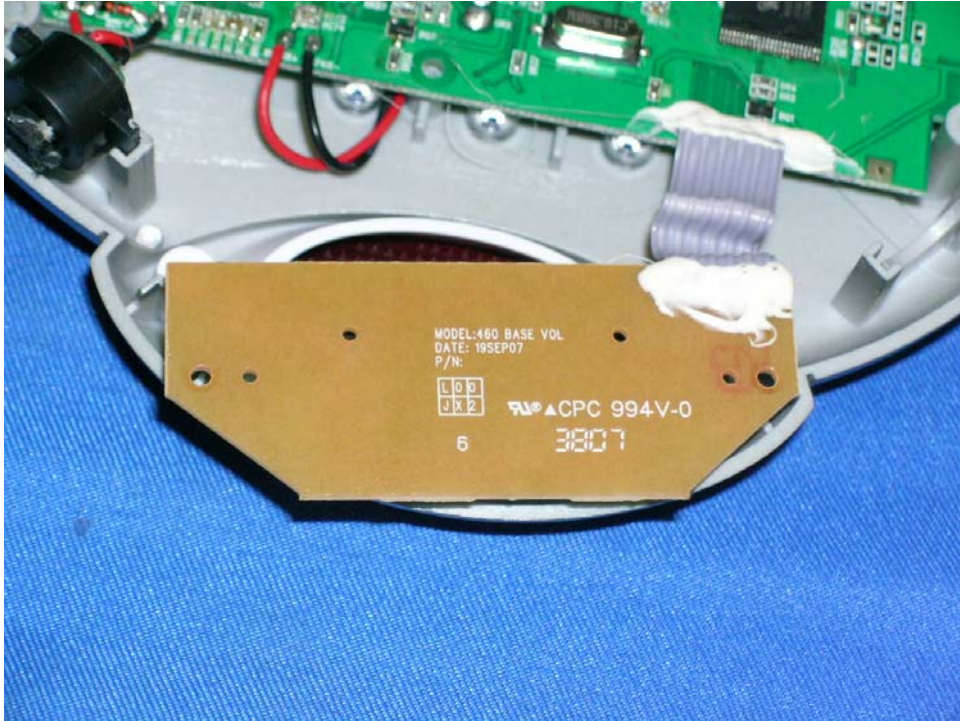
Base Unit Boost Key rear side
