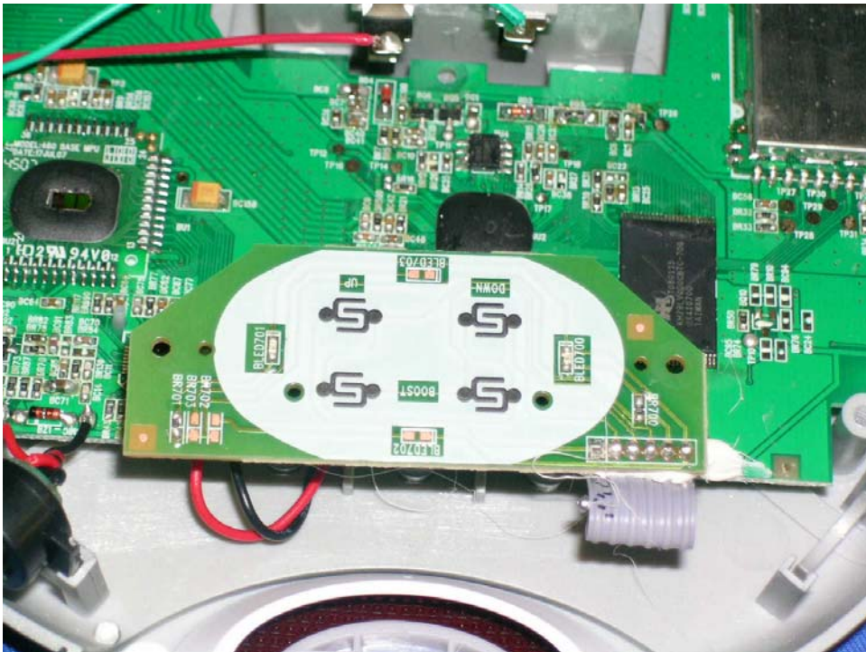
Base Unit Boost Key front side
