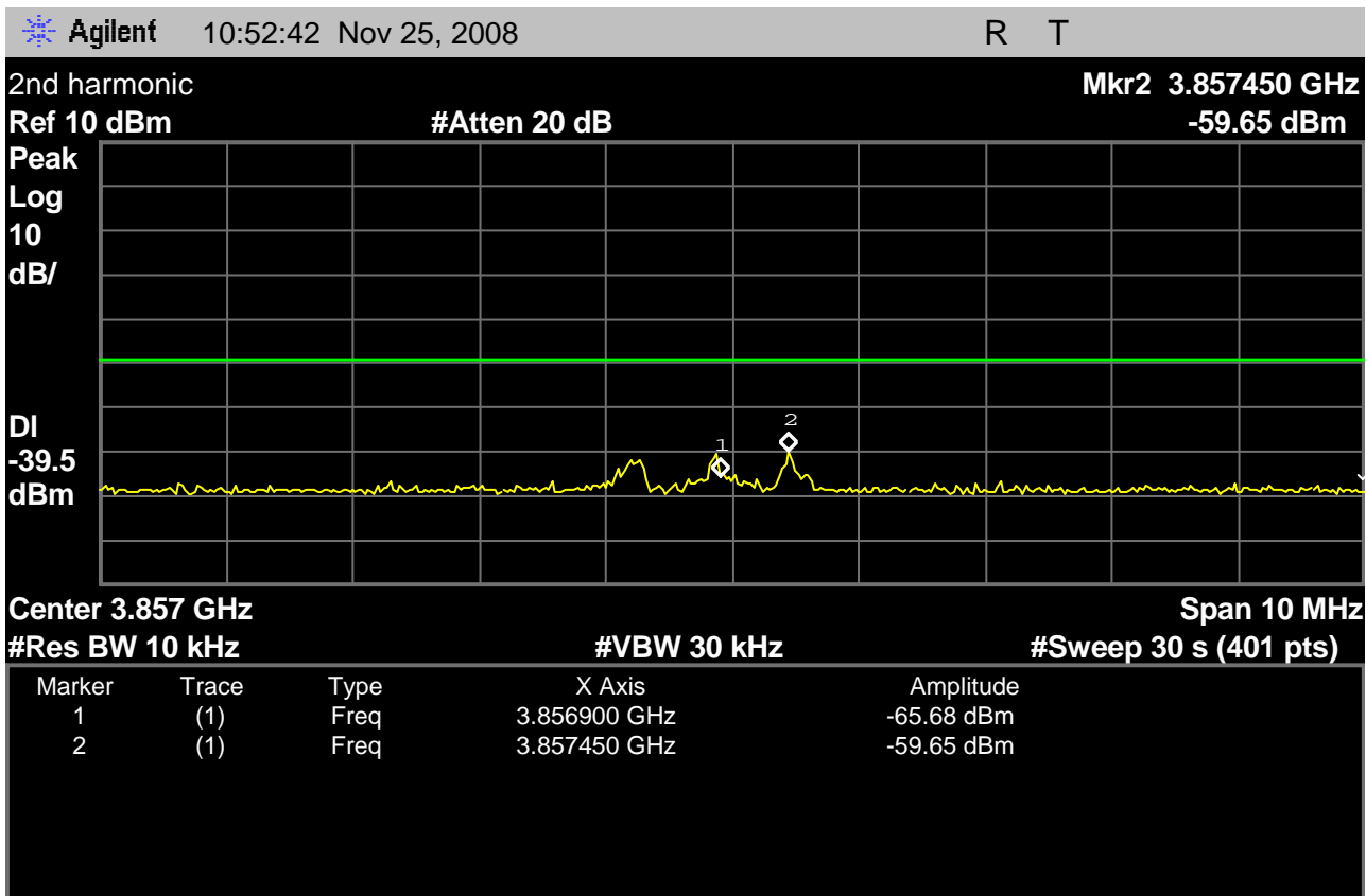
Fig. 36 – Base emissions measured in 10kHz resolution bandwidth in the region where the 1935MHz to 19.3GHz sweep at 300kHz observed a 2 nd harmonic response, for the Base transmitting on the high carrier, 1928.448MHz. A peak of -59.65dBm is measured in the specified resolution bandwidth, a margin of 20.15dB from the -39.5dBm spec limit.
