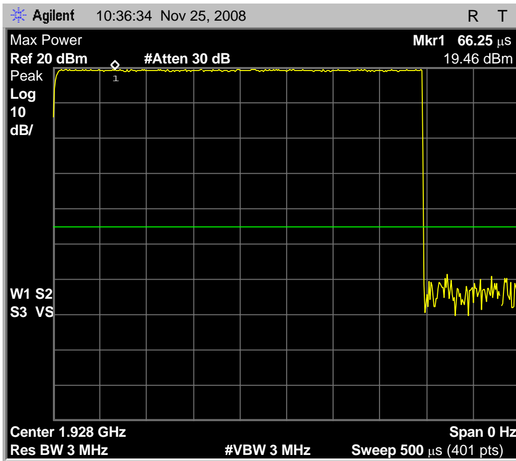
Fig. 10 - Base EUT transmit power received by spectrum analyzer configured according to the requirements of clause 6.1.2 of C63.17-2006, high carrier. Maximum observed transmit power is 19.46 dBm.
