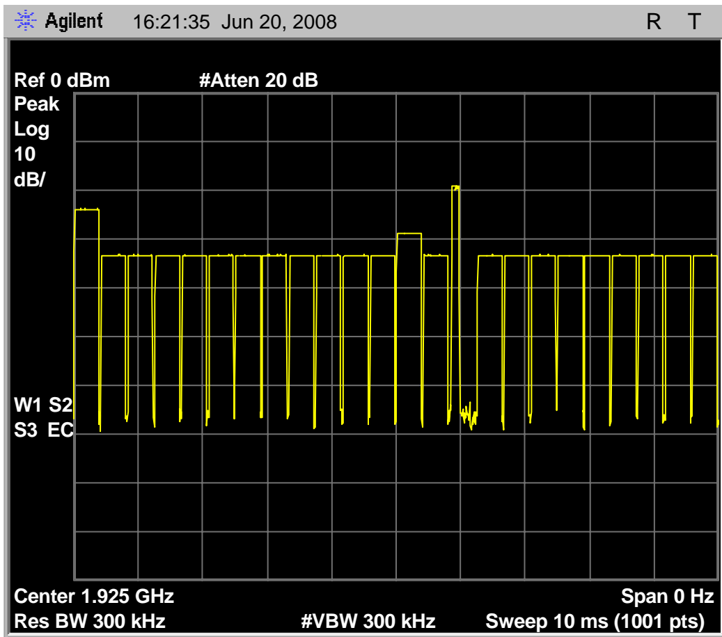
Fig. 61 – Zero-span (single frequency receiver mode) sweep of TDMA interference on carrier at 1924.993MHz, f_1 , with Base EUT beacon transmissions in the single unblocked timeslot.
