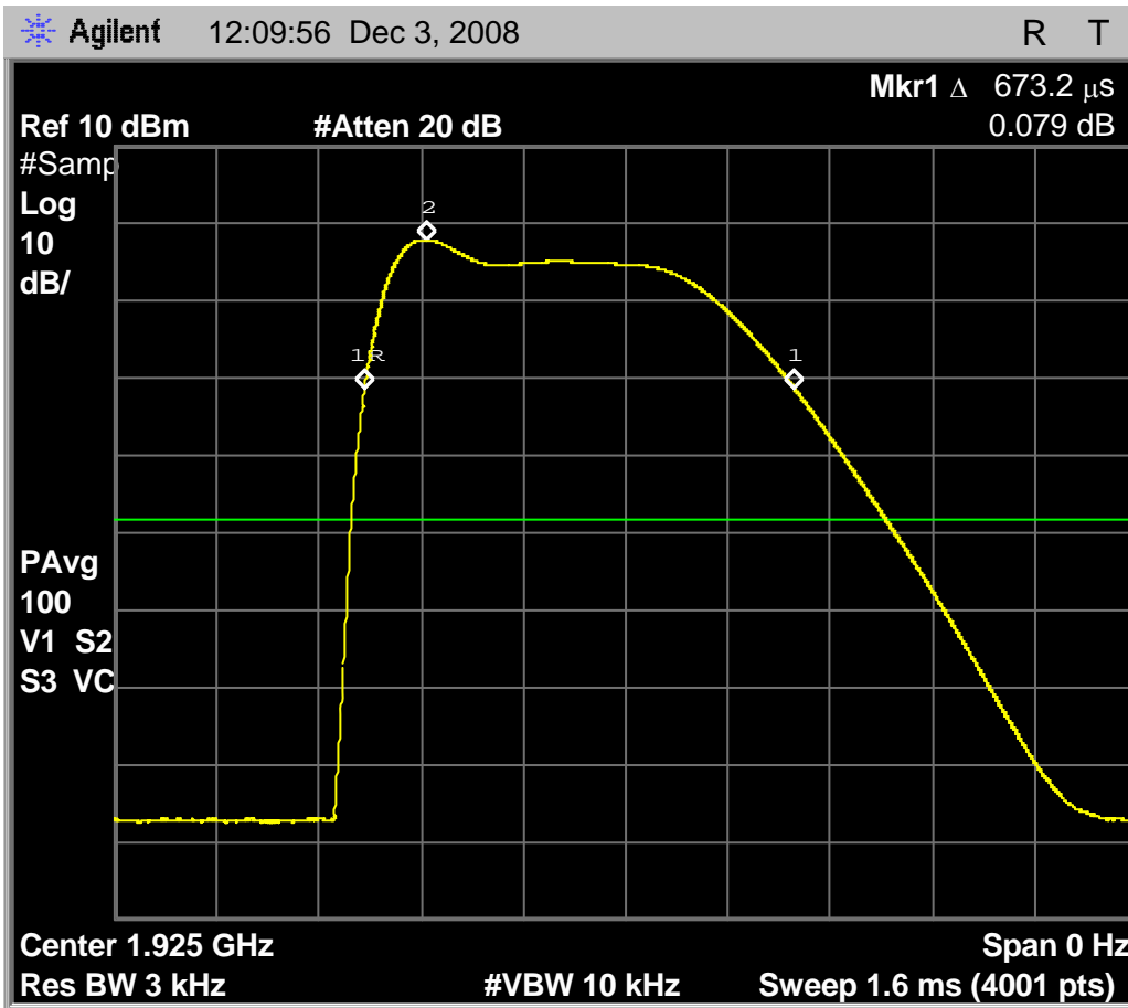
Fig. 16 – Zero-span sweep for Base EUT, middle carrier, for 3kHz maximum power spectral density. The peak level is at -0.99dBm, and the interval between samples at the -20dB points spans is 673.2us.
