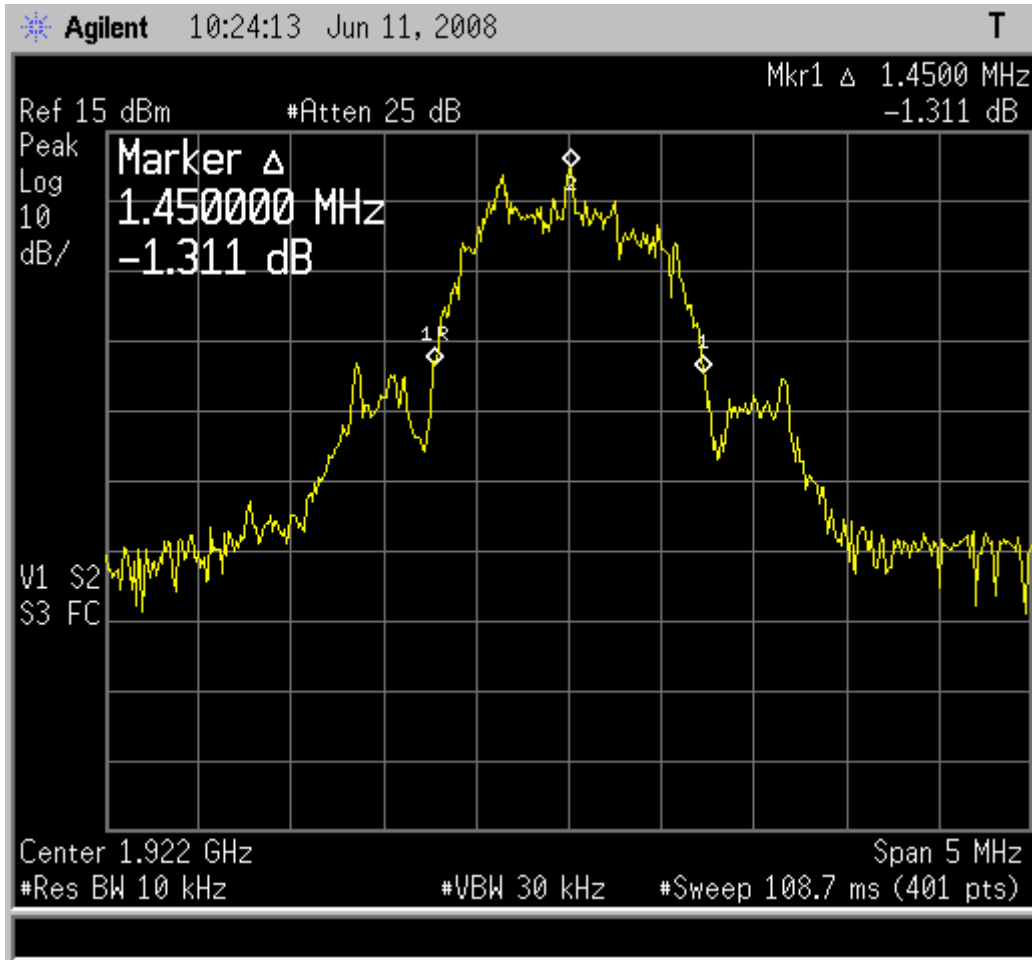
Fig. 11 - Base EUT, 1.45MHz emissions bandwidth on low carrier.
