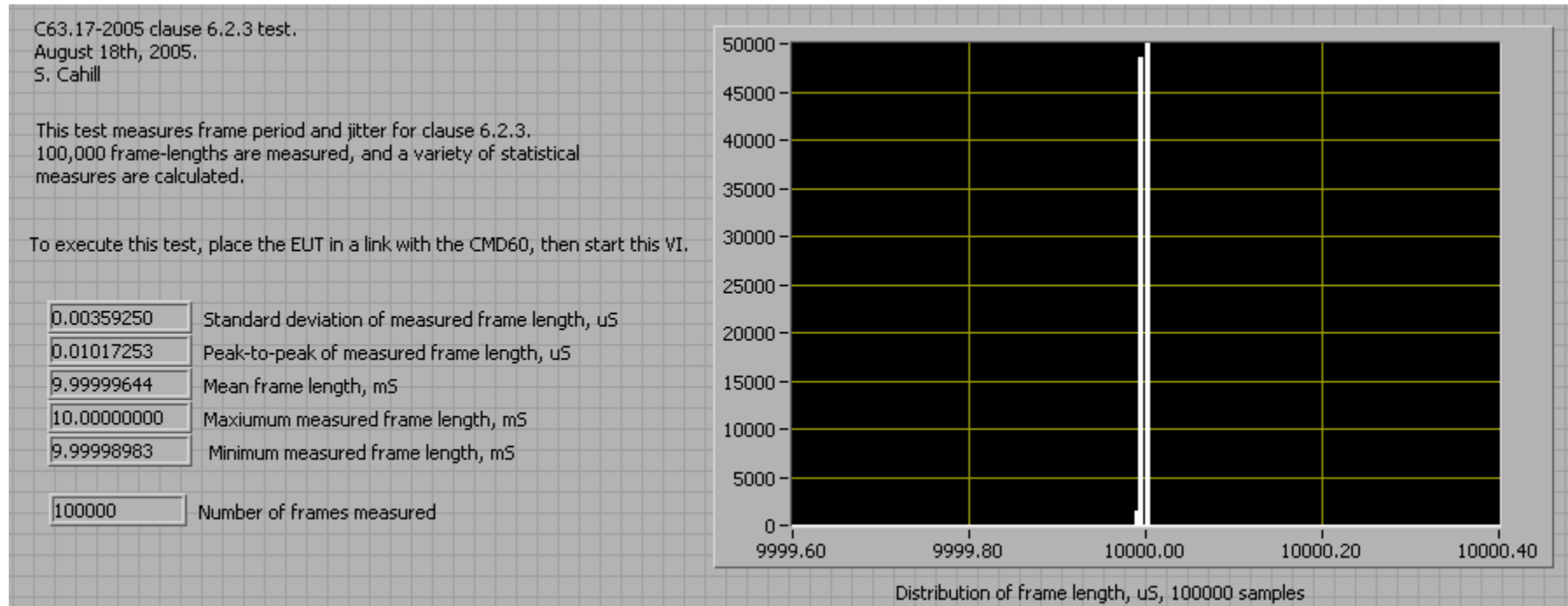
Fig. 45 - Test of Base EUT for frame period and jitter, according to the requirements of clause 6.2.3.
