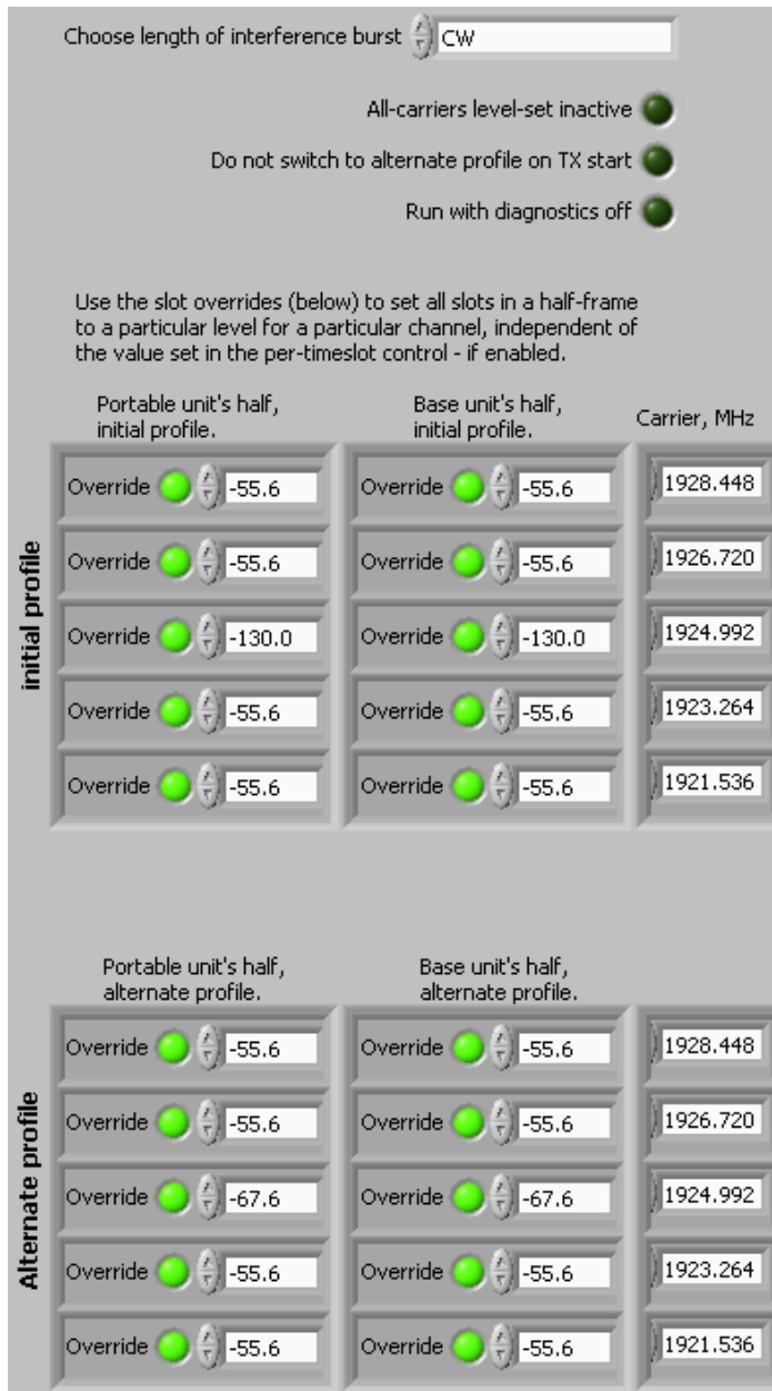
Fig. 66 - PXI-5670 multi-carrier interference generator control panel for the test of 8.2.1(c), for the Base EUT.
