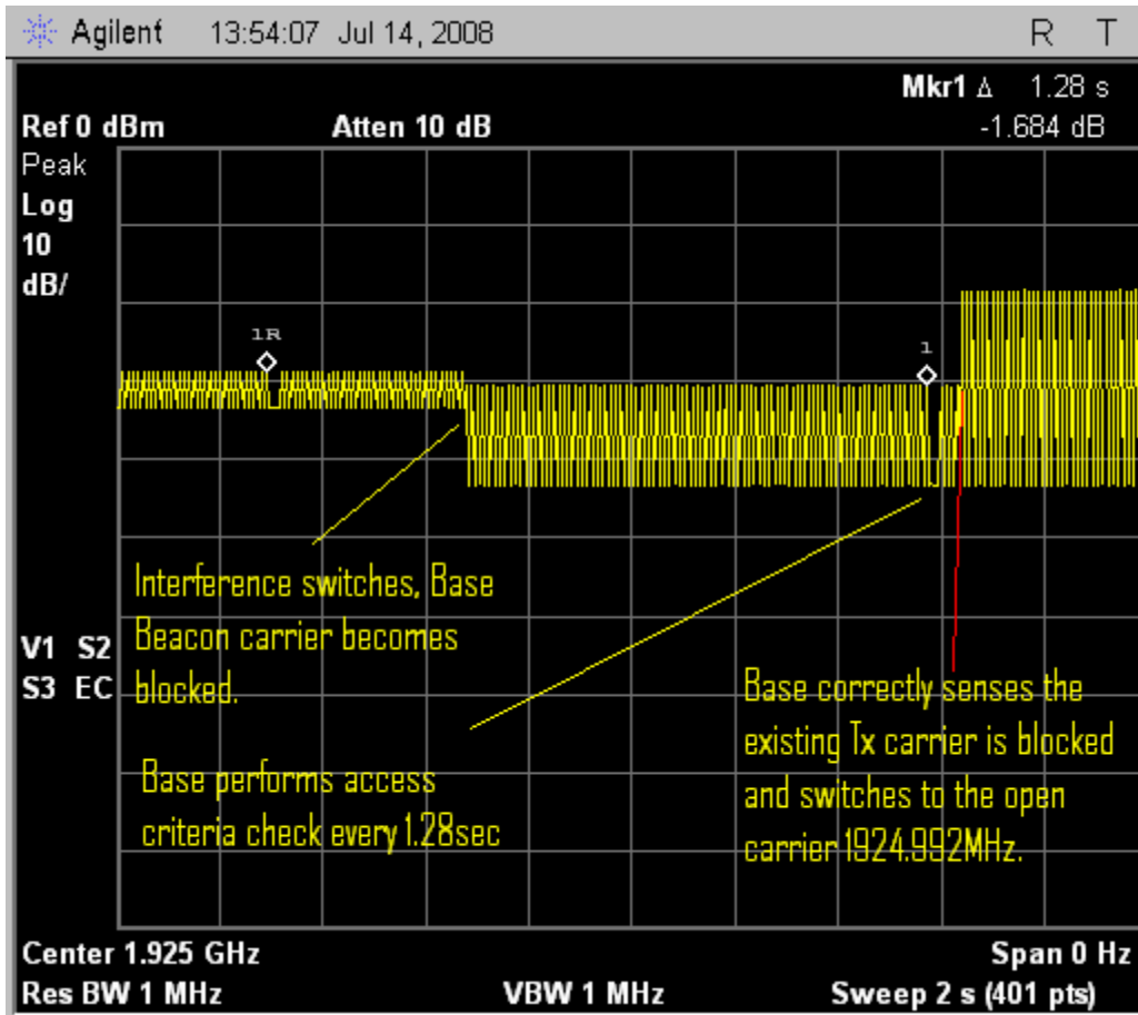
Fig. 65 – Zero span spectrum analyzer display of Base EUT pausing the transmission of signaling to check access criteria, finding the channel no longer meets the access criteria, and resuming transmissions on an alternate carrier.
