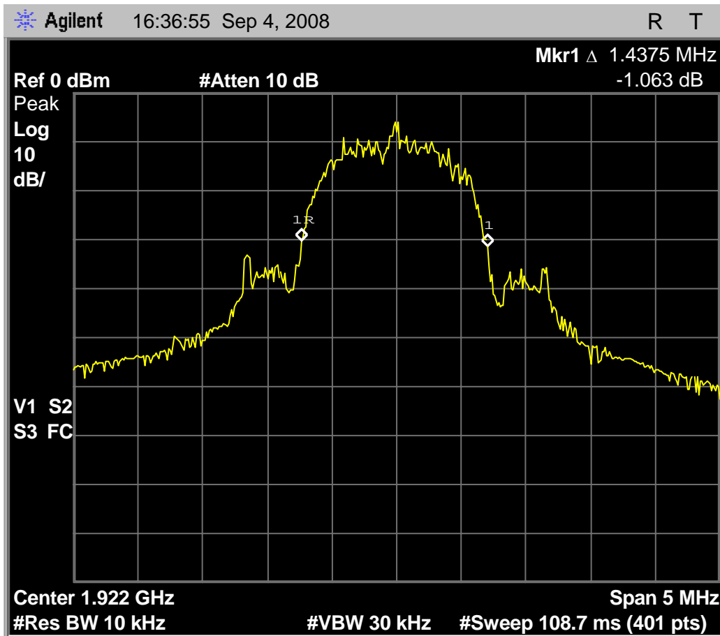
Fig. 71 - Base EUT in low power WBM, 1.45MHz emissions bandwidth on low carrier; vs. 1.45MHz in max power normal mode.
