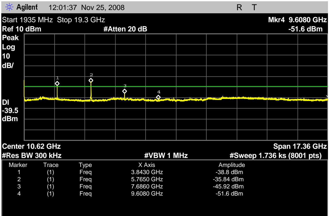
Fig. 27 – Base EUT out-of-band emissions including the regions from 1935MHz to 19.3GHz with the Base EUT transmitting on the lowest carrier, 1921.536MHz.
