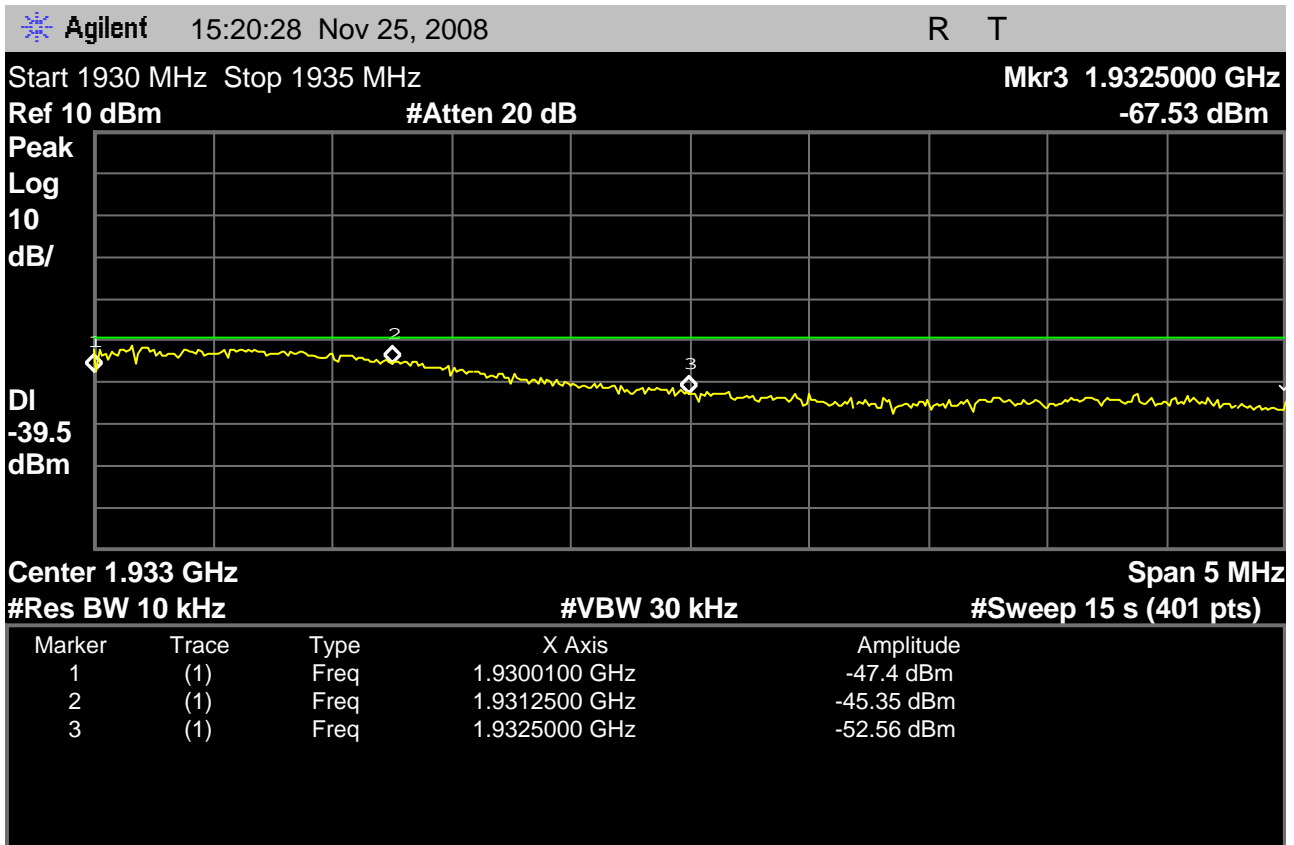
Fig. 34 – Base EUT out-of-band emissions showing the regions from band edge to +1.25MHz, and from +1.25MHz to +2.5MHz, with the Base EUT transmitting on the highest carrier, 1928.448MHz. Note the green display line is the spec limit marker only for the region outside +2.5MHz.
