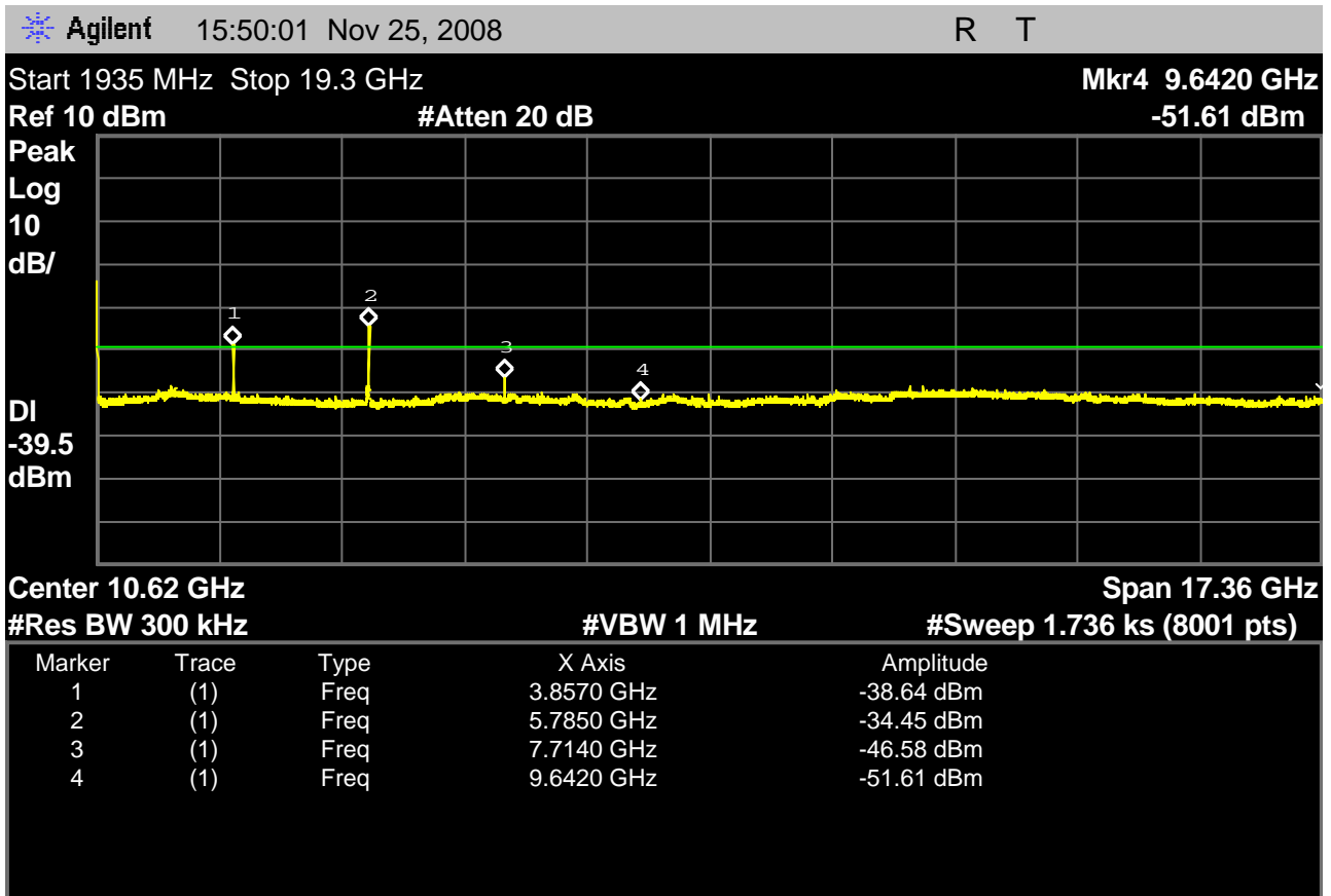
Fig. 35 – Base EUT out-of-band emissions including the regions from 1935MHz to 19.3GHz with the Base EUT transmitting on the highest carrier, 1928.448MHz.
