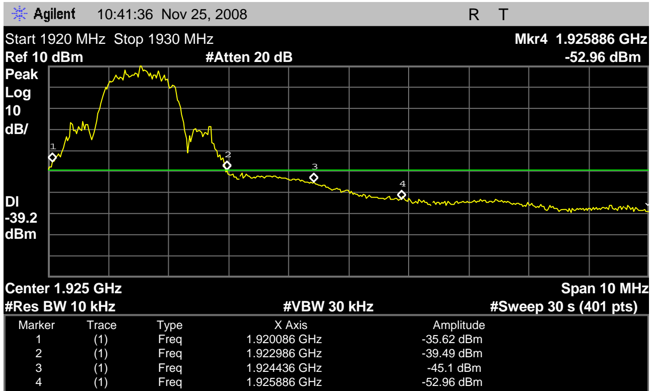
Fig. 20 - Spectrum analyzer screenshot for transmit emissions showing in-band unwanted emissions with the Base EUT transmitter at the lowest carrier, 1921.536MHz, according to the requirements of 6.1.6.1.
