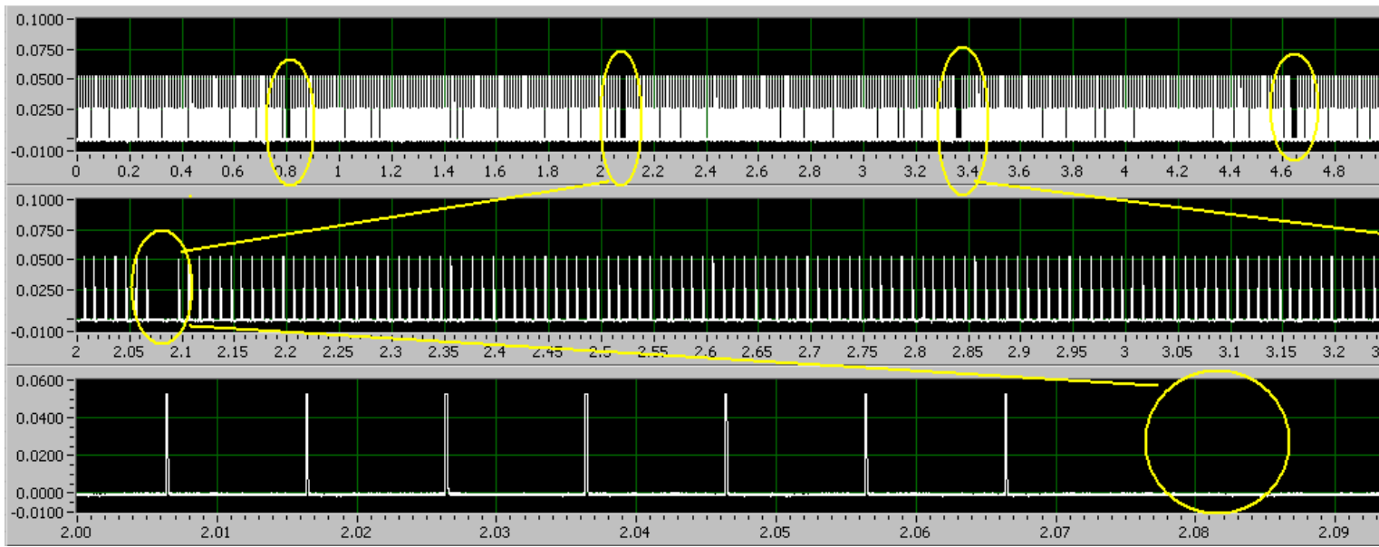
Fig. 63 – Capture of demodulated transmissions of Base EUT signaling transmissions; the signal present at the RF detector output. The resolution of detail may require viewing this document in electronic format at 150% resolution. Irreducible image artifacts occur in the top trace due to pixilation in the original screen capture.
