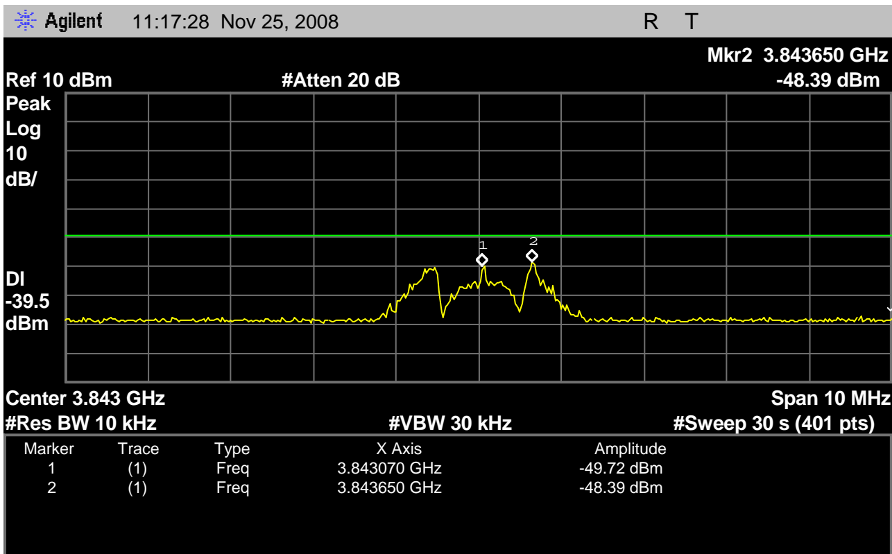
Fig. 28 – Base EUT out-of-band emissions in the region around the 2 nd harmonic, with the Base EUT transmitting on the lowest carrier, 1921.536MHz.
