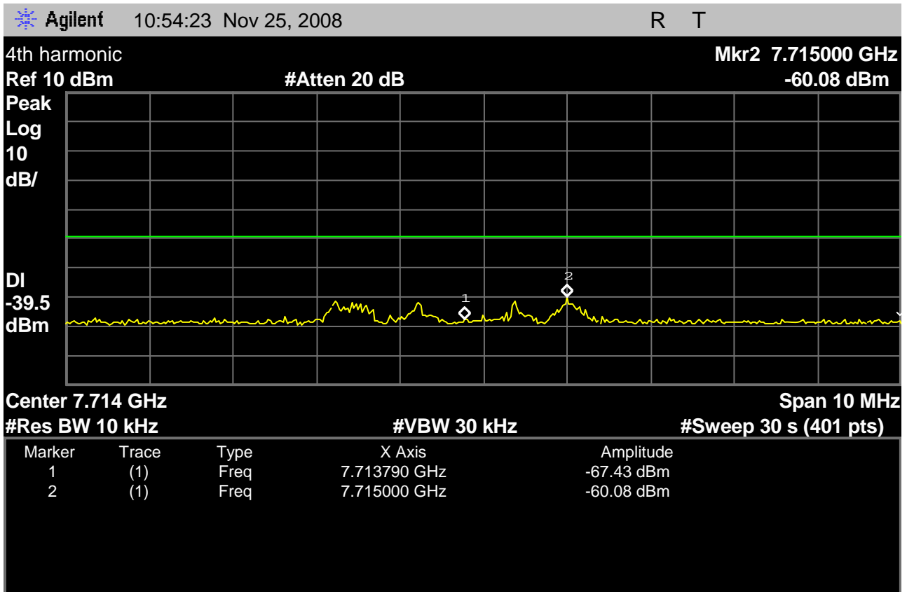
Fig. 38 – Base EUT out-of-band emissions in the region around the 4 th harmonic, with the Base EUT transmitting on the highest carrier, 1928.448MHz.
