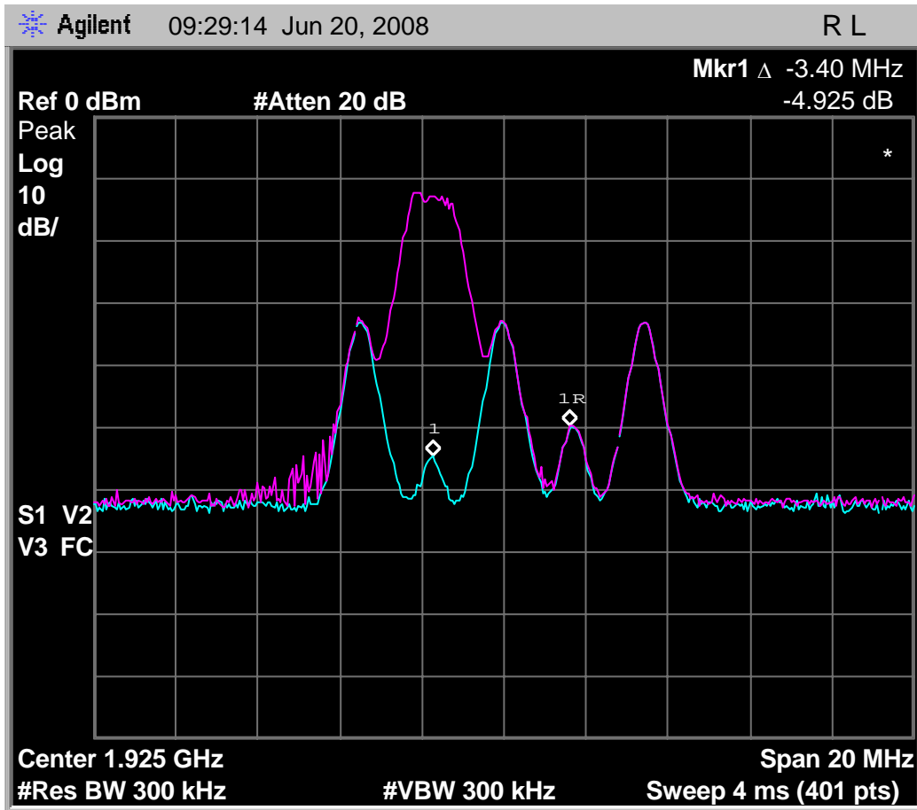
Fig. 49 - Emissions and interference profile spectrum, Base EUT, test 7.3.3(d).
