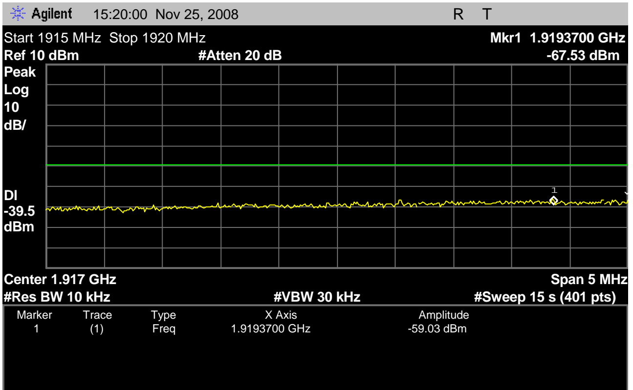
Fig. 33 – Base EUT out-of-band emissions showing the regions from band edge to -1.25MHz, and from -1.25MHz to -2.5MHz, with the Base EUT transmitting on the highest carrier, 1928.448MHz.
