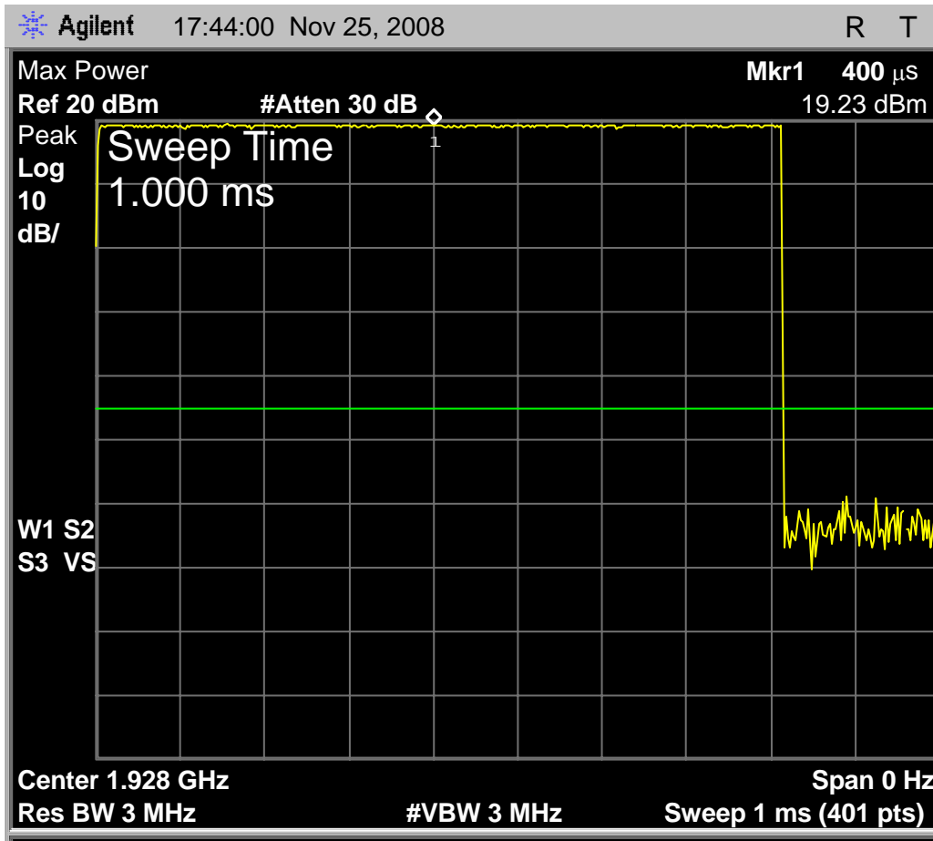
Fig. 69 - Base EUT transmit power received by spectrum analyzer configured according to the requirements of clause 6.1.2 of C63.17-2006, high carrier. Maximum observed transmit power is 19.23 dBm in WBM; output power for normal mode on mid channel was 19.46dBm ( P_{max} = 20.8 dBm).
