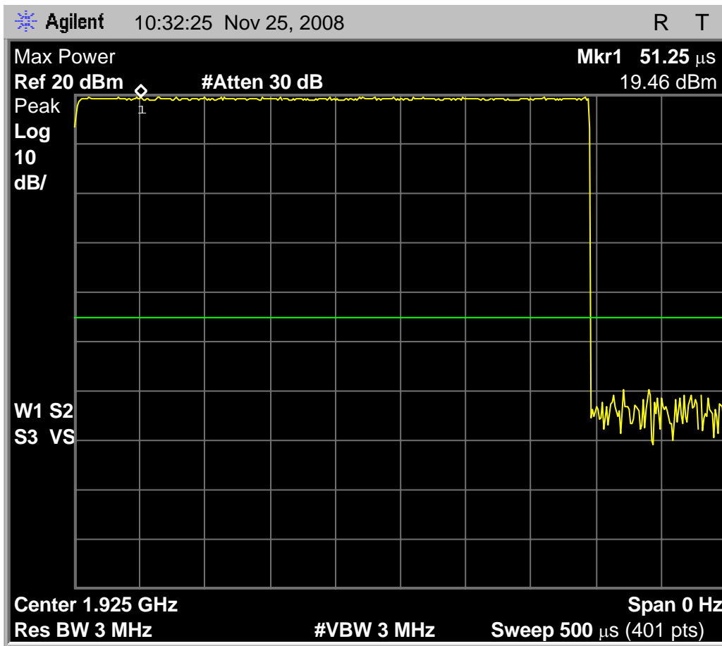
Fig. 9 - Base EUT transmit power received by spectrum analyzer configured according to the requirements of clause 6.1.2 of C63.17-2006, mid carrier. Maximum observed transmit power is 19.46 dBm
