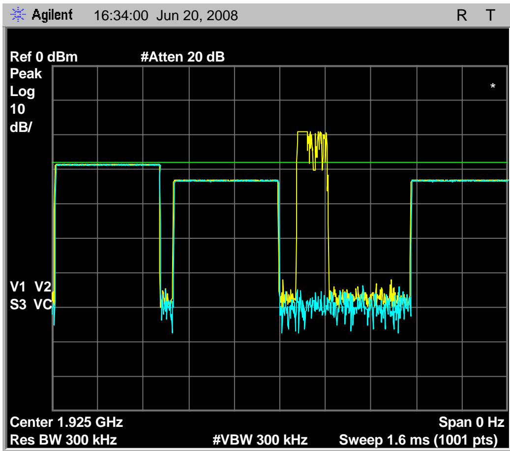
Fig. 62 – Zero-span (single frequency receiver mode) sweep of TDMA interference on carrier at 1924.993MHz, f_1 , with Base EUT beacon transmissions in single open timeslot.
