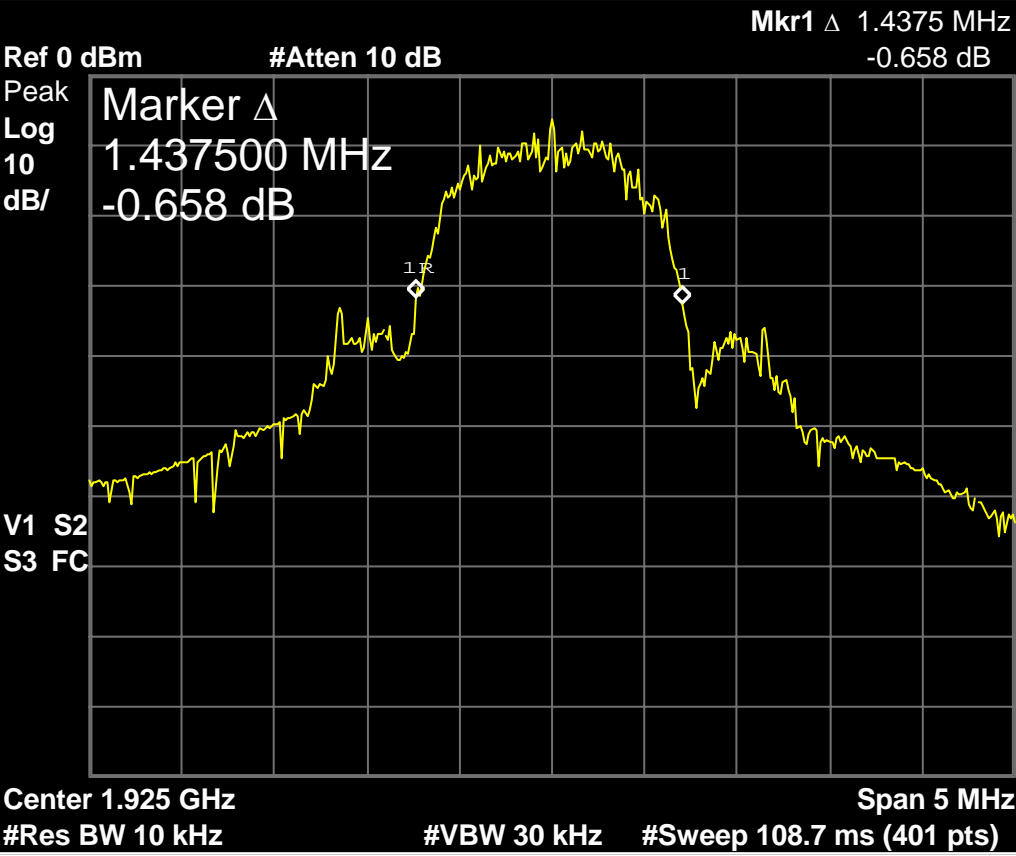
Fig. 72 - Base EUT in low power WBM, 1.44MHz emissions bandwidth on mid carrier vs. 1.45MHz in max power normal mode.
