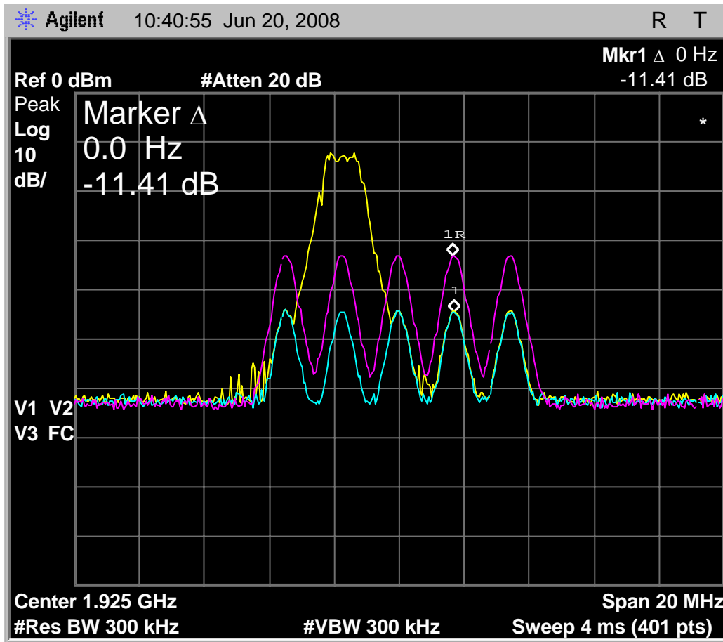
Fig. 56 - Transmit spectrum of 50uS interference pulses, with Base EUT no longer deferring with interference pulses of level T_U - U_M .
