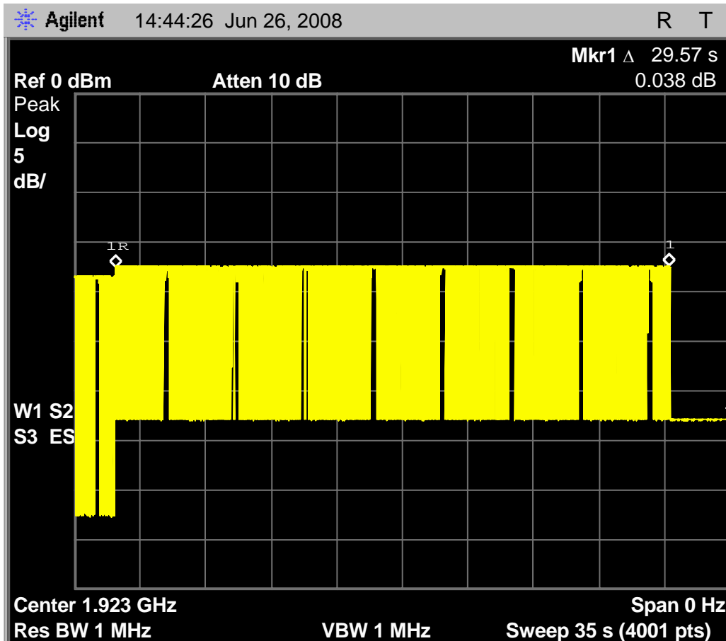
Fig. 68 – The spectrum analyzer zero span screen capture shows upon interference switch (at marker 1R), which now interference blocks the previously unblocked channel of 1923.264MHz, the beacon remains up, but prior to 30 seconds from the blocked interference the Base EUT beacon is brought down, since there are no open channels to move the beacon.
