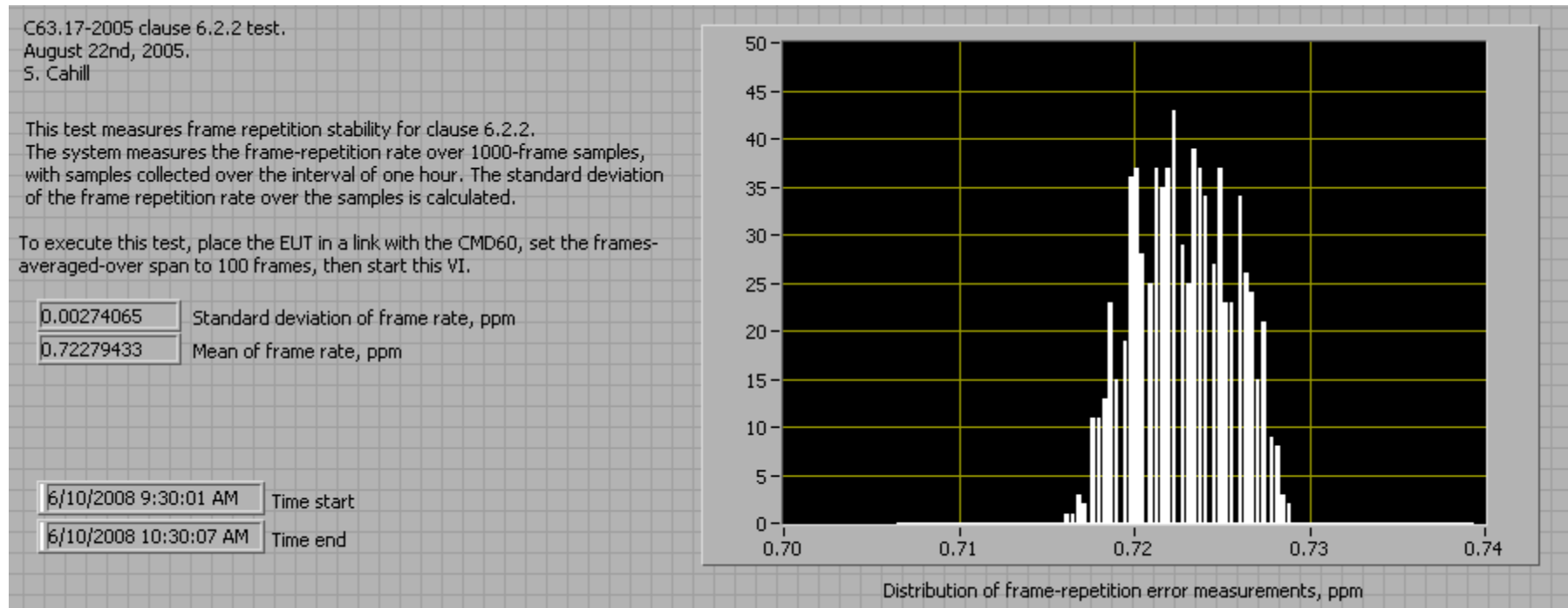
Fig. 44 - Test of Base EUT according to the conditions of clause 6.2.2 for frame repetition rate stability
