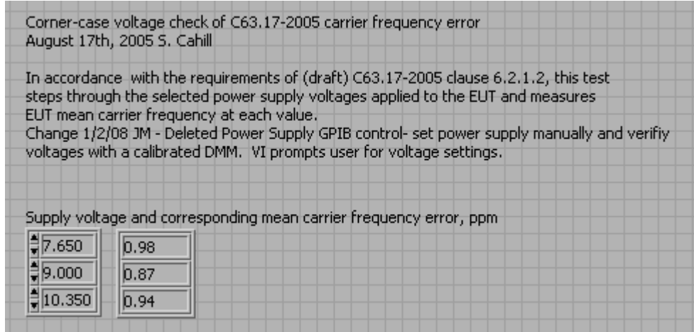
Fig. 42 - Measured mean carrier frequency, Base EUT , at 7.650V, 9.000V, and 10.350V.
