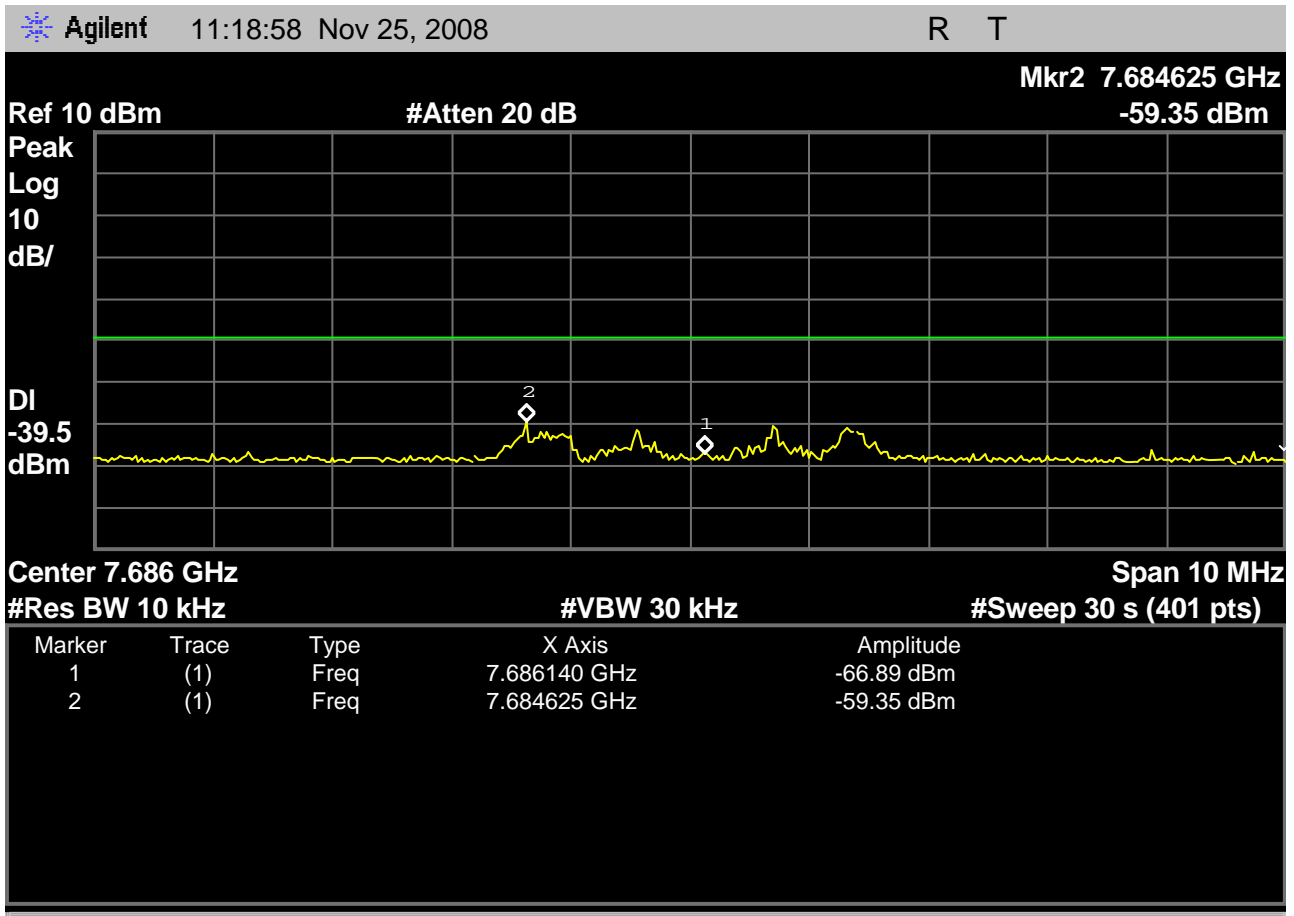
Fig. 30 – Base EUT out-of-band emissions in the region around the 4th harmonic, with the Base EUT transmitting on the lowest carrier, 1921.536MHz.
