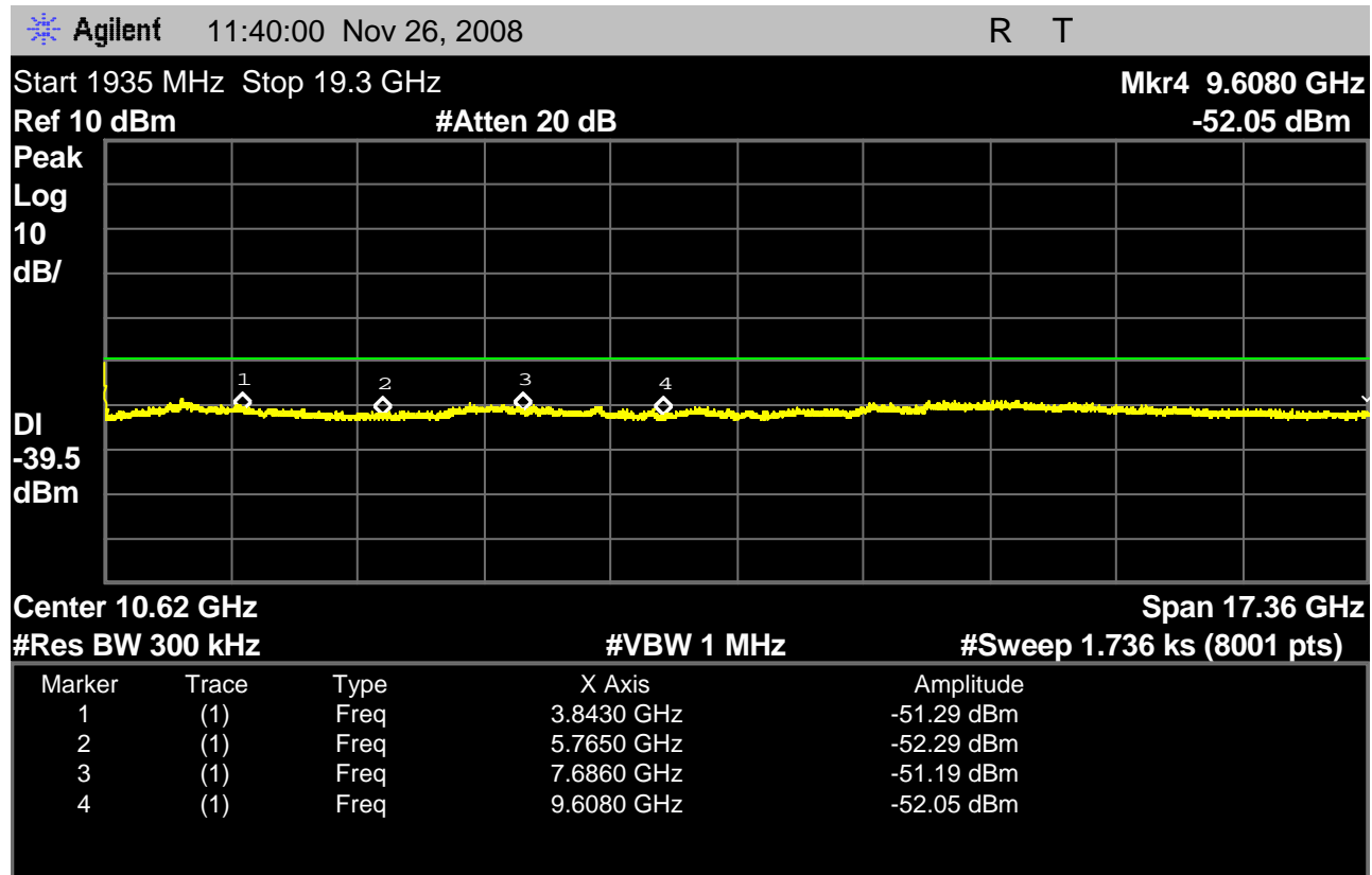
Fig. 74 - - Base EUT in minimum power WBM on high carrier. All harmonics are below specification in minimum power, even when measured in the 300kHz (greater) resolution bandwidth.
