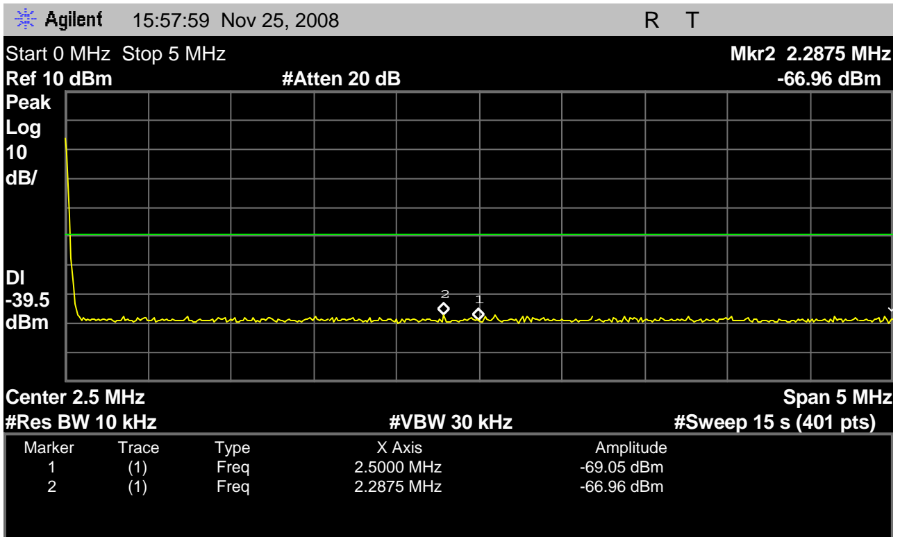
Fig. 31 – Base EUT out-of-band emissions showing the regions from DC to 5MHz, with the transmitter using the highest carrier, 1928.448MHz.
