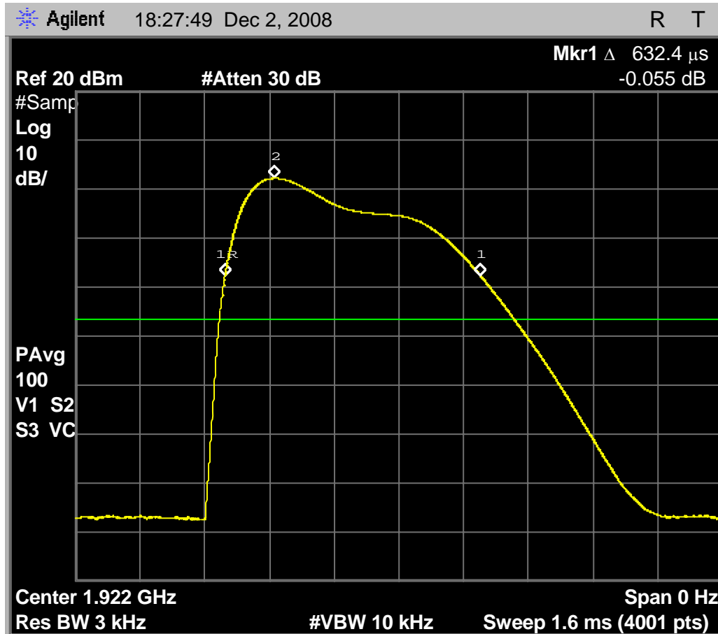
Fig. 14 – Zero-span sweep for Base EUT, low carrier, for 3kHz maximum power spectral density. The peak level is at 2.19dBm, and the interval between samples at the -20dB points is from 632.4us.
