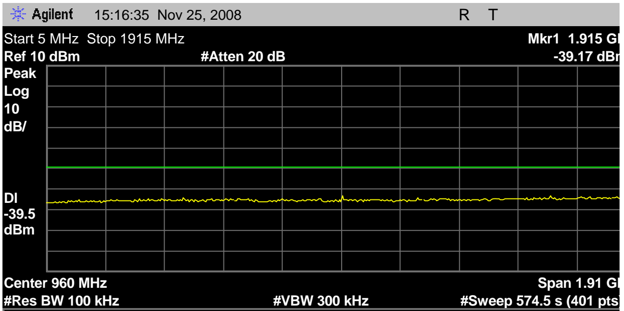
Fig. 32 – Base EUT out-of-band emissions showing the region from 5MHz to 1915MHz, with the transmitter using the highest carrier, 1928.448MHz.
