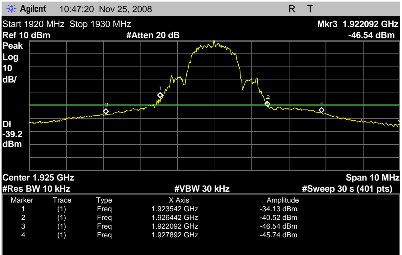
Fig. 21 - Spectrum analyzer screenshot for transmit emissions showing in-band unwanted emissions with the Base EUT transmitter at the middle carrier, 1924.992MHz, according to the requirements of 6.1.6.1.
