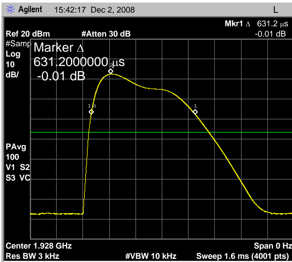
Fig. 18 – Zero-span sweep for Base EUT, high carrier, for 3kHz maximum power spectral density. The peak level is at 2.44dBm, and the interval between samples at the -20dB points is 631.2us.
