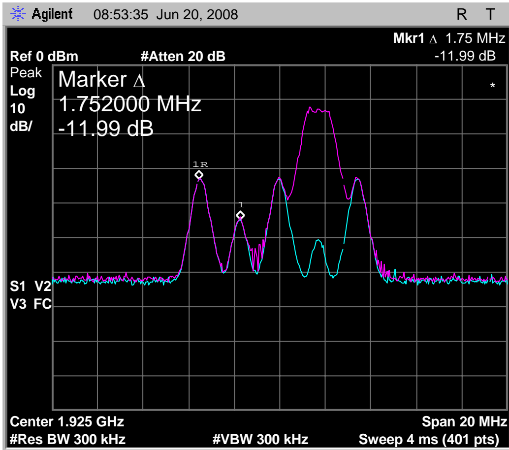
Fig. 48 - Emissions and interference profile spectrum, Base EUT, test 7.3.3(c).
