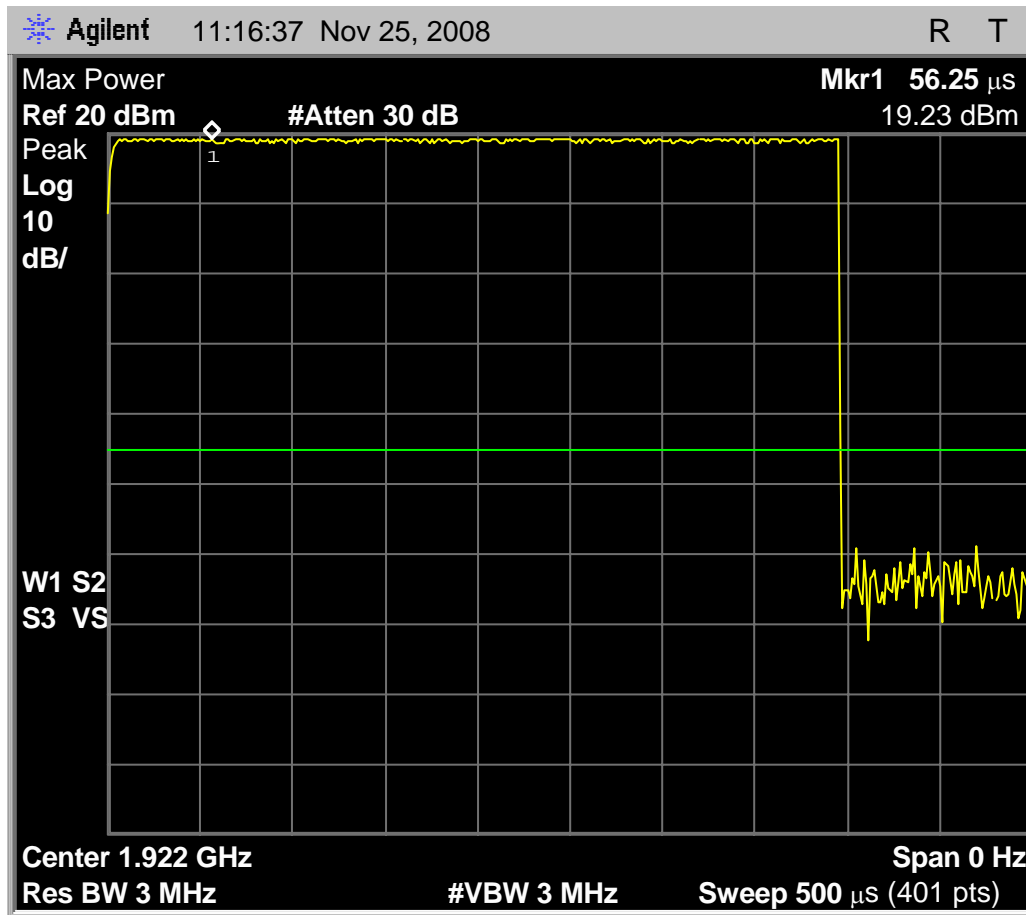
Fig. 8 - Base EUT transmit power received by spectrum analyzer configured according to the requirements of clause 6.1.2 of C63.17-2006, low carrier. Maximum observed transmit power is 19.23 dBm.
