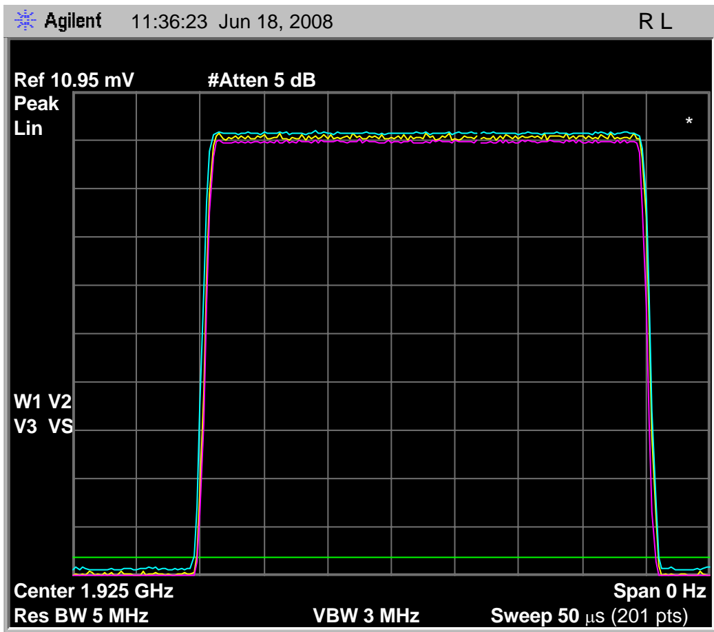
Fig. 58 - 35uS interference pulse for 7.5(d), duration and amplitude variation over the duration of the pulse and over multiple pulses. Spectrum analyzer is set to linear response.
