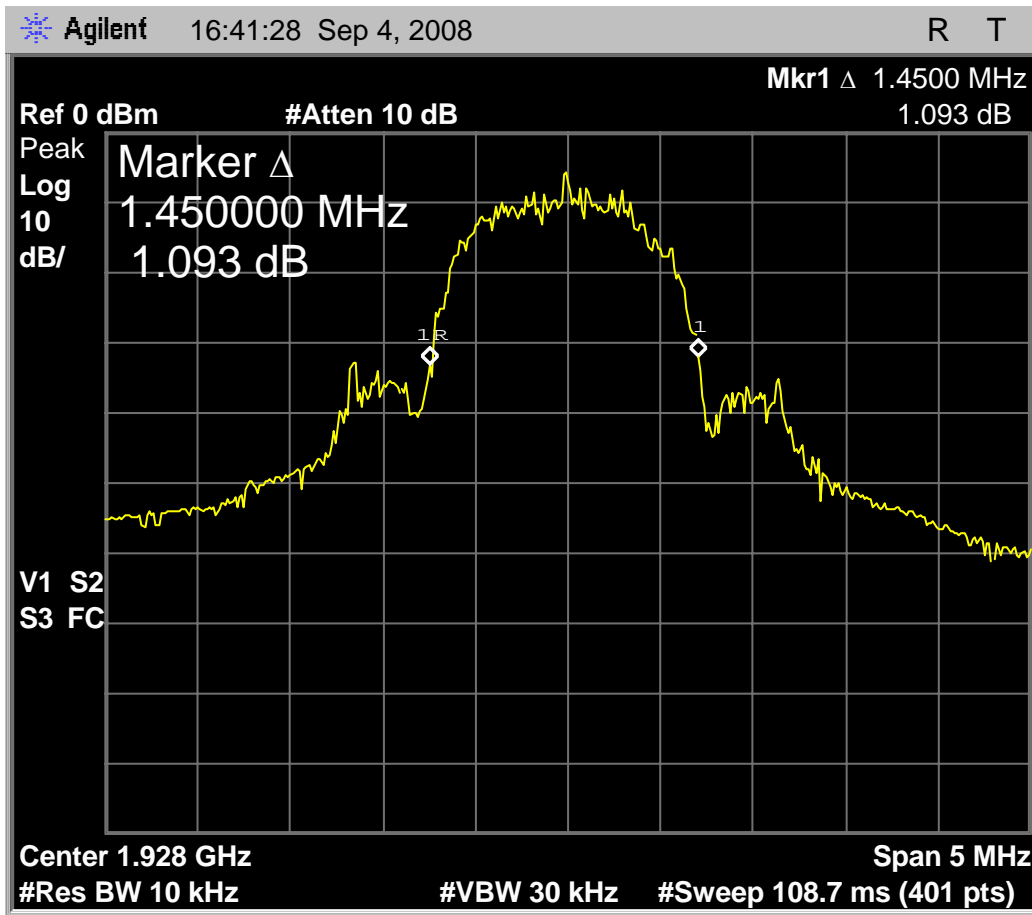
Fig. 73 - Base EUT in low power WBM, 1.45MHz emissions bandwidth on mid carrier vs. 1.45MHz in max power normal mode.
