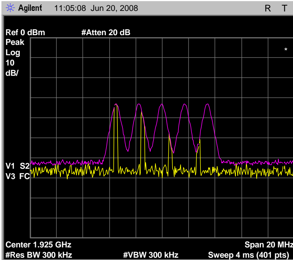
Fig. 55 - Base EUT shown deferring when all channels are blocked with 50uS pulses at TU + UM . Top trace is detected RF transmissions (no transmissions are detected), bottom trace is headset EUT transmission setup attempt series (as indicated by the software flag for getting-ready-to-transmit attempts) in response to the press of the TALK button, with each pulse of the software transmission-attempt flag then not being followed by the transmissions, due to the access criteria check failure.
