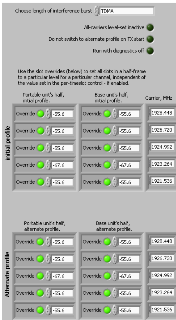
Fig. 64 – Control panel for the multi-carrier interference generator for the test of 8.1.2.
