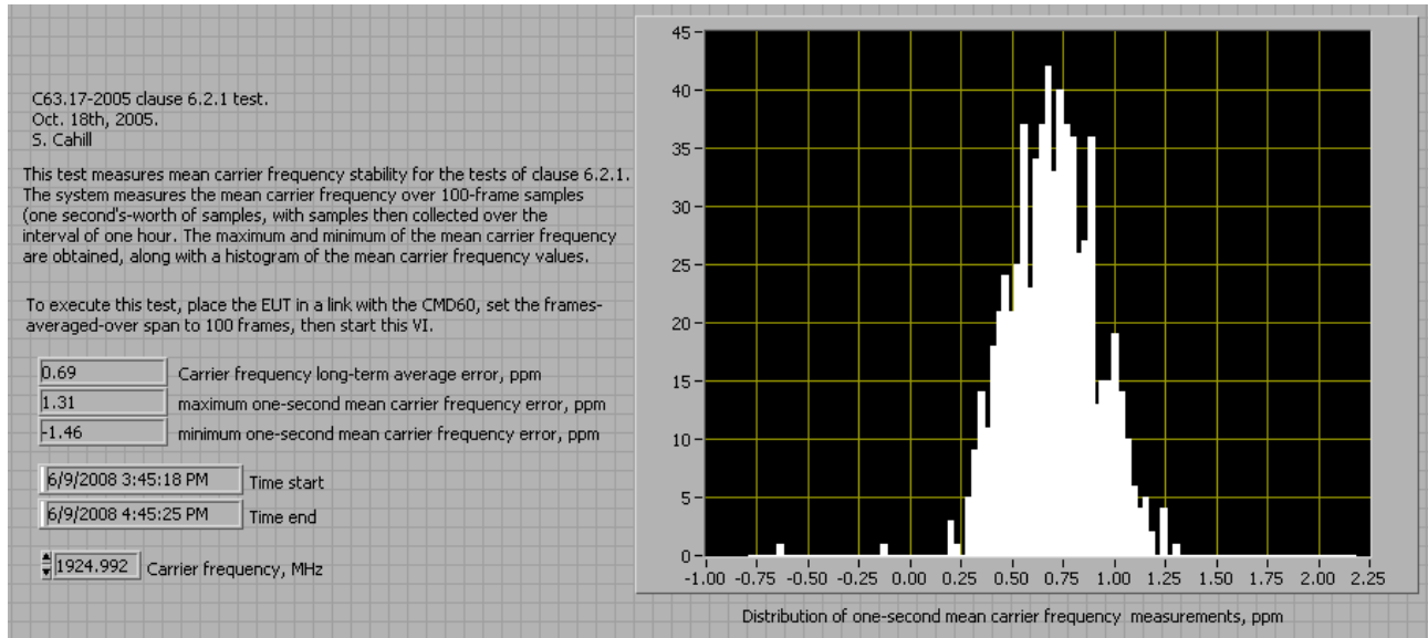
Fig. 41 - Measured one-second mean carrier frequency, Base EUT, and observed maximum, average value and observed minimum of the mean carrier frequency.
