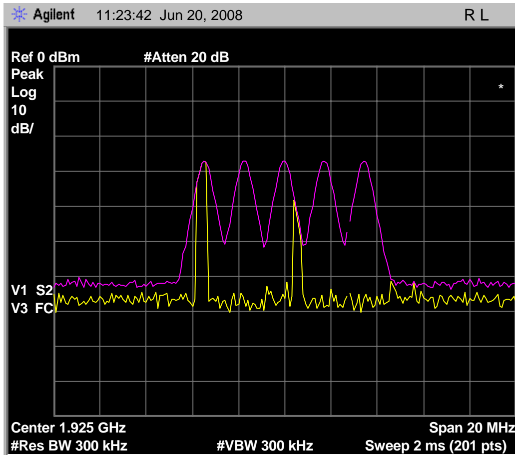
Fig. 59 - Transmit spectrum of 35uS interference pulses in each timeslot for each carrier, with Base EUT deferring due to interference pulses of T_U + U_M + 6\text{dB} .
