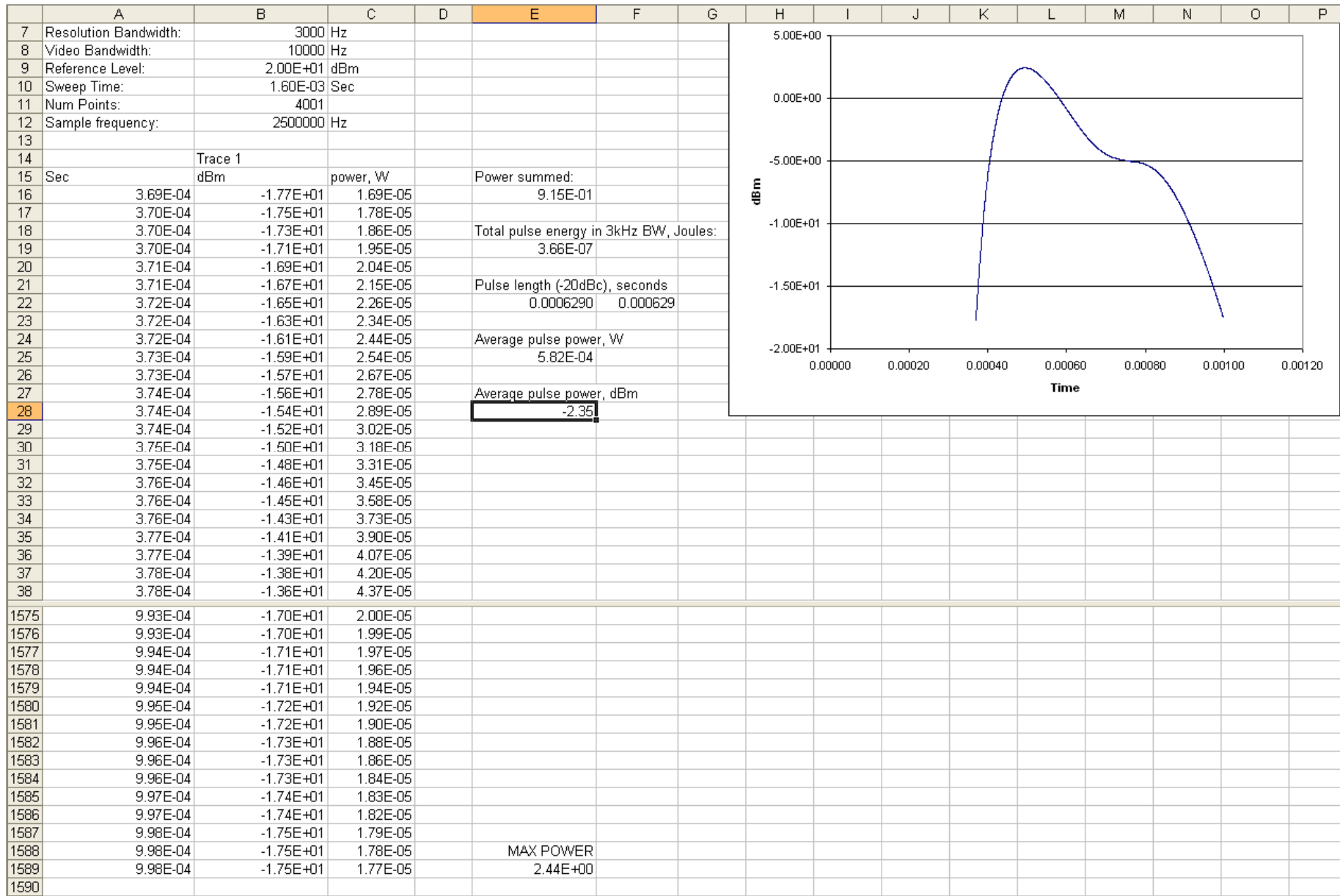
Fig. 19 – Screenshot of Excel file showing PSDlimit calculations for Base EUT, high carrier; -2.35dBm.
