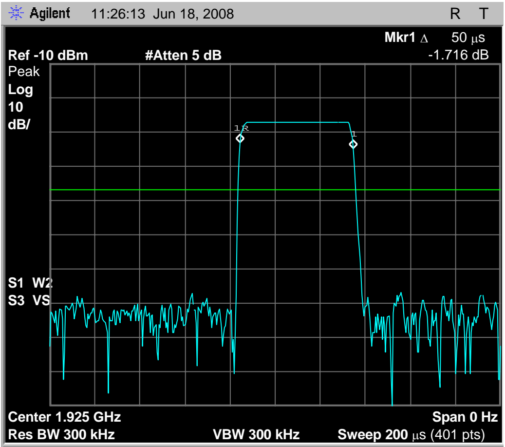
Fig. 52 - Interference pulse, one frame shown, for the test of 7.5(c).
