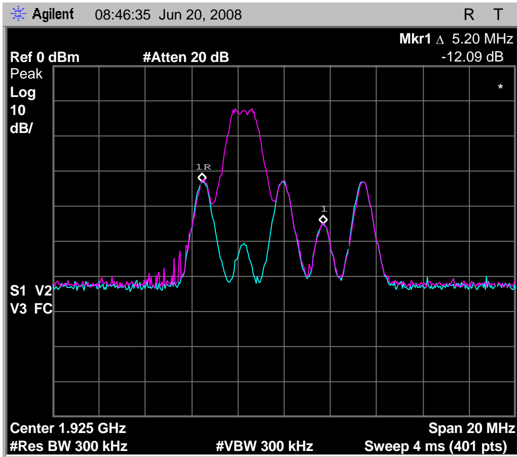
Fig. 47 - Emissions and interference profile spectrum, Base EUT, test 7.3.3(b).
