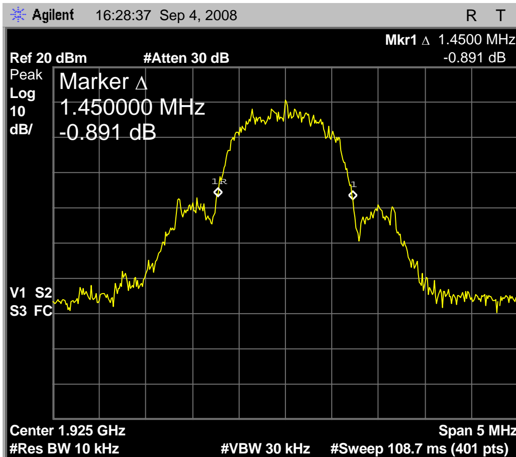
Fig. 70 - Base EUT in WBM, 1.45MHz (maximum of 2.5MHz, minimum of 50kHz) emissions bandwidth vs. 1.45MHz in normal mode.
