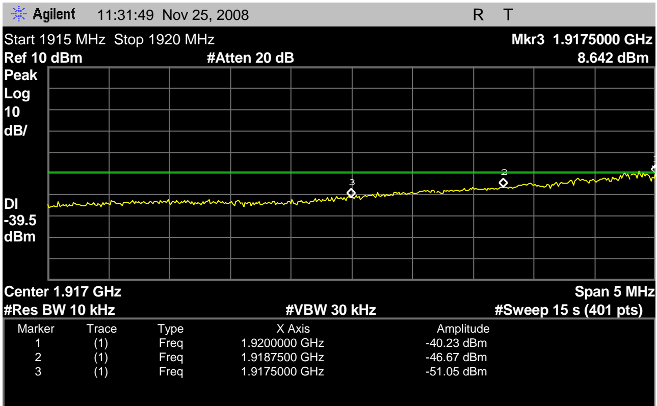
Fig. 25 – Base EUT out-of-band emissions showing the regions from band edge to -1.25MHz, and from -1.25MHz to -2.5MHz, with the Base EUT transmitting on the lowest carrier, 1921.536MHz. . Note the green display line is the spec limit marker only for the region outside +2.5MHz.
