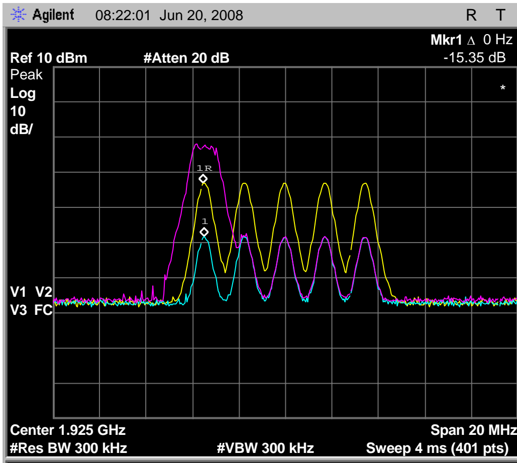
Fig. 46 - Emissions and interference profile spectrum, Base EUT, test 7.3.2.
