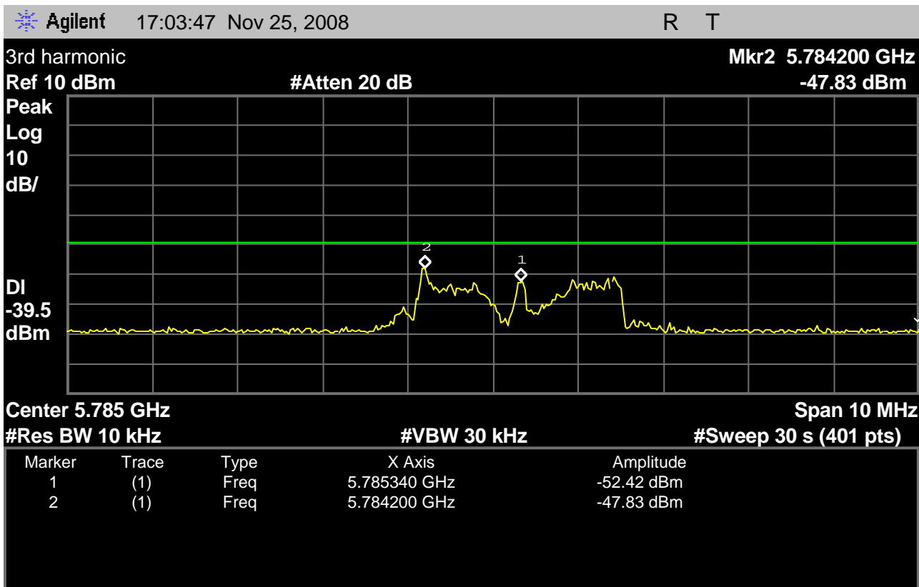
Fig. 37 – Base emissions measured in 10kHz resolution bandwidth in the region where the 1935MHz to 19.3GHz sweep at 300kHz observed a 3 rd harmonic response, for the Base transmitting on the high carrier, 1928.448MHz. A peak of -47.83dBm is measured in the specified resolution bandwidth, a margin of 8.33dB from the -39.5dBm spec limit.
