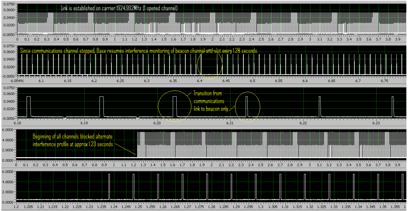
Fig. 67 – Capture of Base EUT transmission changing from communications link to beacon only.
