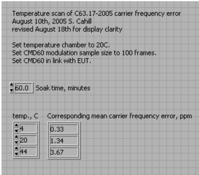
Fig. 43 - Measured mean carrier frequency, Base EUT , at +4C, +20C, +44C.
