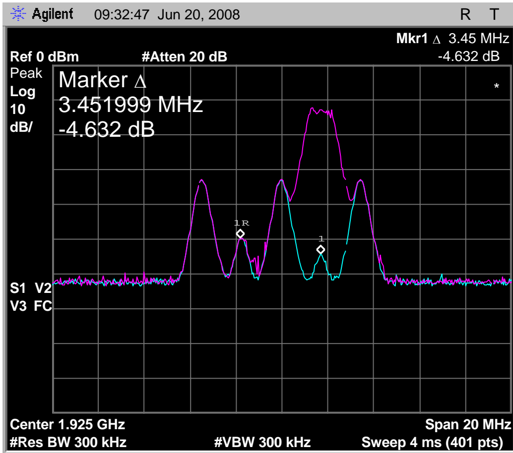
Fig. 50 - Emissions and interference profile spectrum, Base EUT, test 7.3.3(e).
