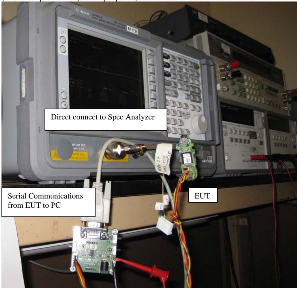
Fig. 5 - Headset EUT in direct connection with spectrum analyzer and radiated connection with base companion device, for the tests of clause 6.1.
