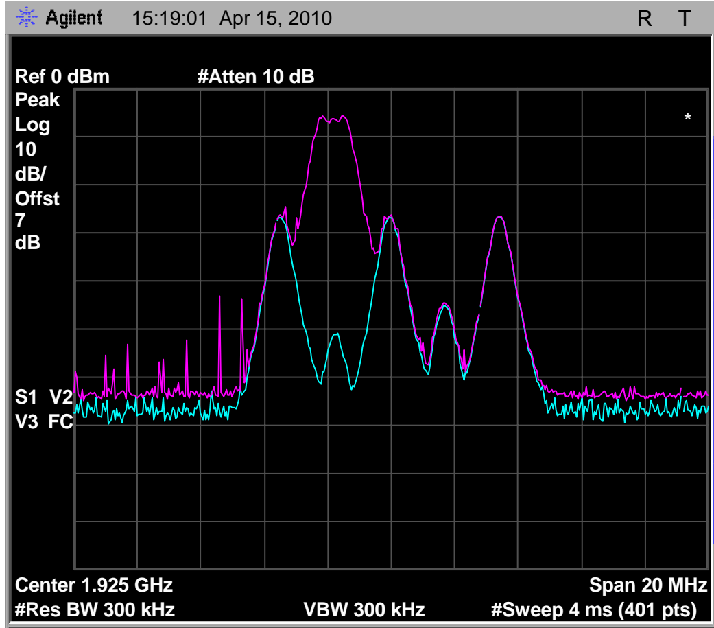
Fig. 45 - Emissions and interference profile spectrum, headset EUT, test 7.3.3(d).
