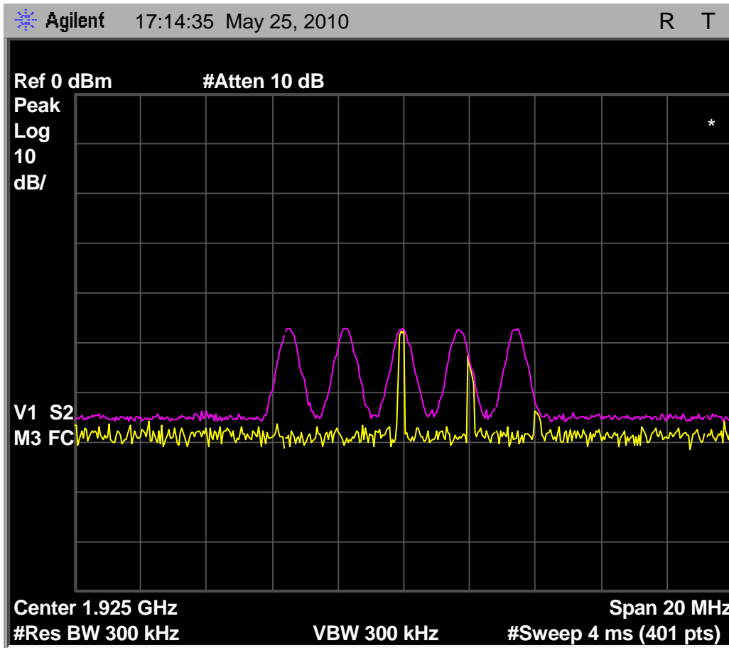
Fig. 79 - Transmit spectrum of 35uS interference pulses in each timeslot for each carrier, with headset EUT deferring due to interference pulses of T_L + U_M + 6\text{dB} .
