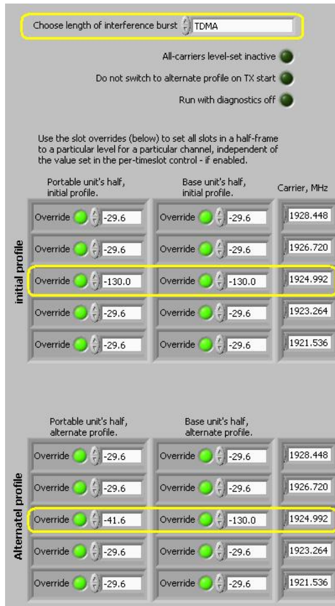
Fig. 63 - PXI-5670 multi-carrier interference generator control panel for the test of 8.2.1(c), for the headset EUT.
