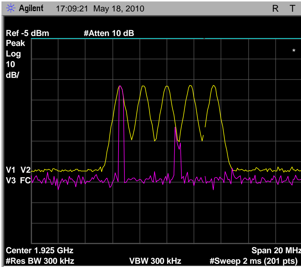
Fig. 57 - Transmit spectrum of 35uS interference pulses in each timeslot for each carrier, with headset EUT deferring due to interference pulses of T_U + U_M + 6\text{dB} .
