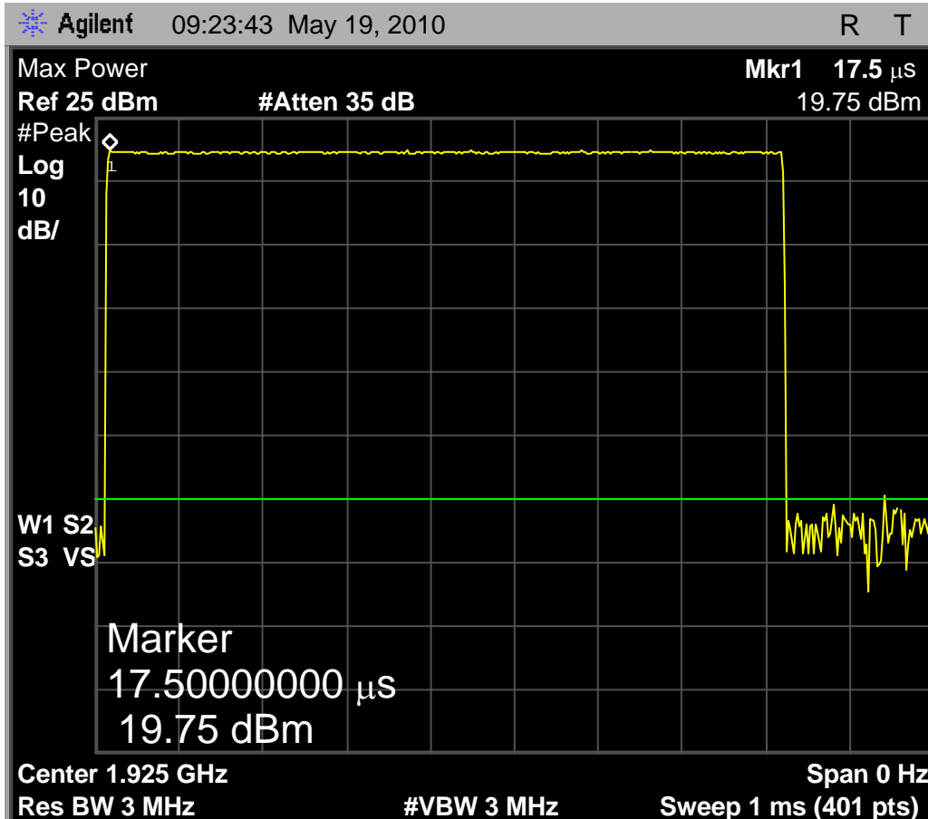
Fig. 73 - Headset EUT transmit power received by spectrum analyzer configured according to the requirements of clause 6.1.2 of C63.17-2006, mid carrier. Maximum observed transmit power is 19.75 dBm in WBM; output power for normal mode on mid channel was 19.75dBm.
