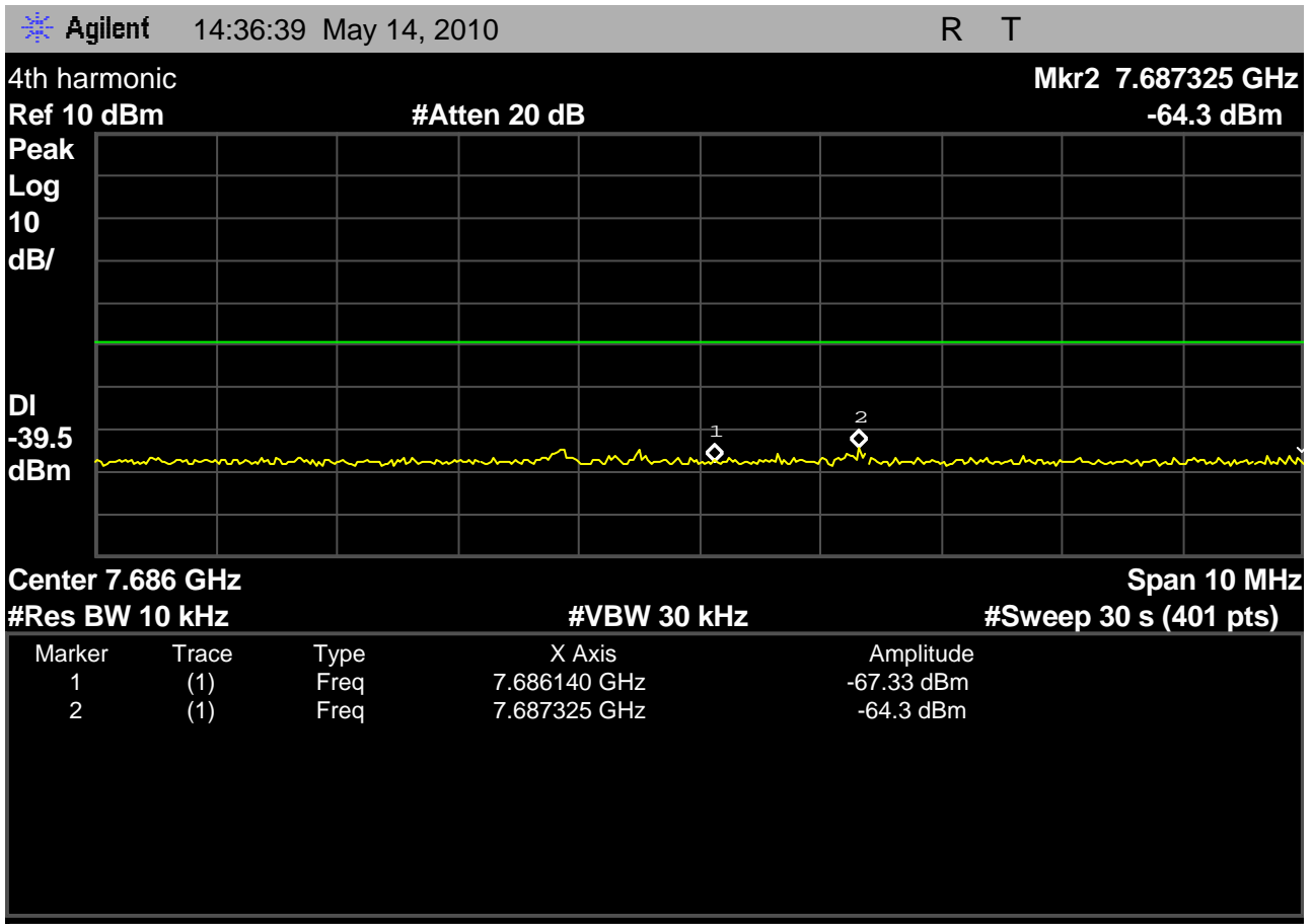
Fig. 29 – headset EUT out-of-band emissions in the region around the 4th harmonic, with the headset EUT transmitting on the lowest carrier, 1921.536MHz.
