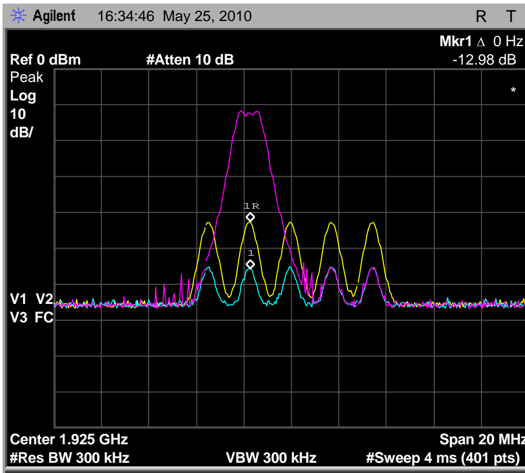
Fig. 75 - Emissions and interference profile spectrum, headset EUT, test 7.3.1 in WBM.
