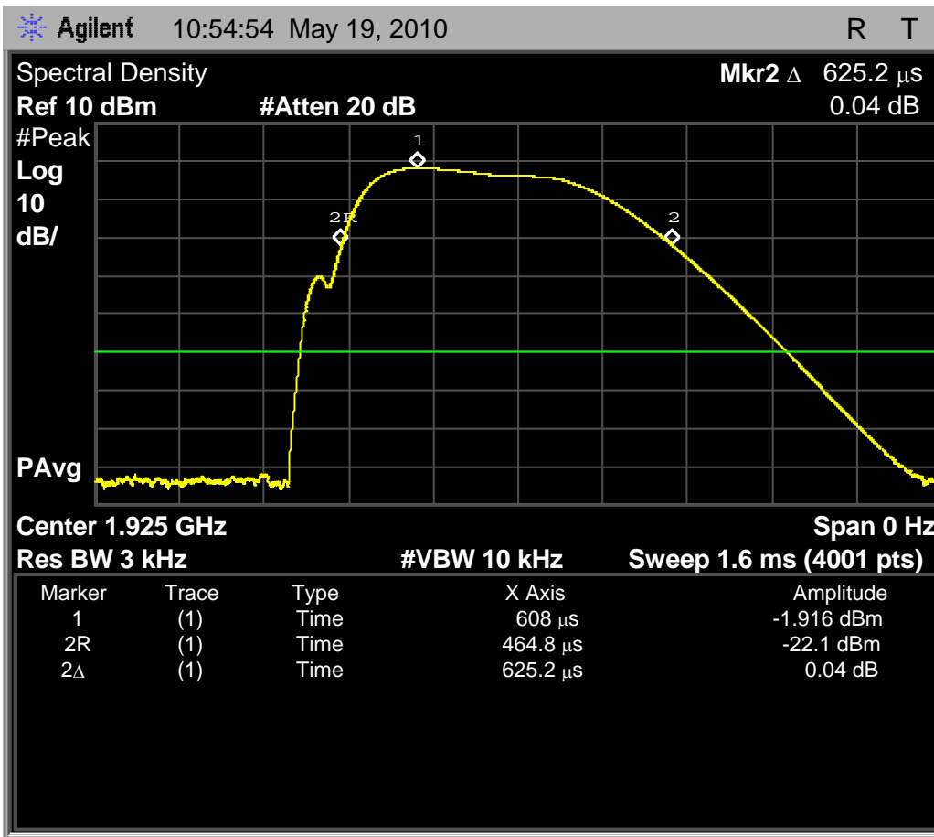
Fig. 15 – Zero-span sweep for headset EUT, middle carrier, for 3kHz maximum power spectral density. The peak level is at -1.916Bm, and the interval between samples at the -20dB points is 625.2us.
