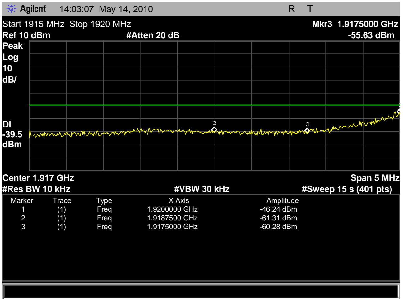
Fig. 24 – Headset EUT out-of-band emissions showing the regions from bandedge to -1.25MHz, and from -1.25MHz to -2.5MHz, with the headset EUT transmitting on the lowest carrier, 1921.536MHz.
