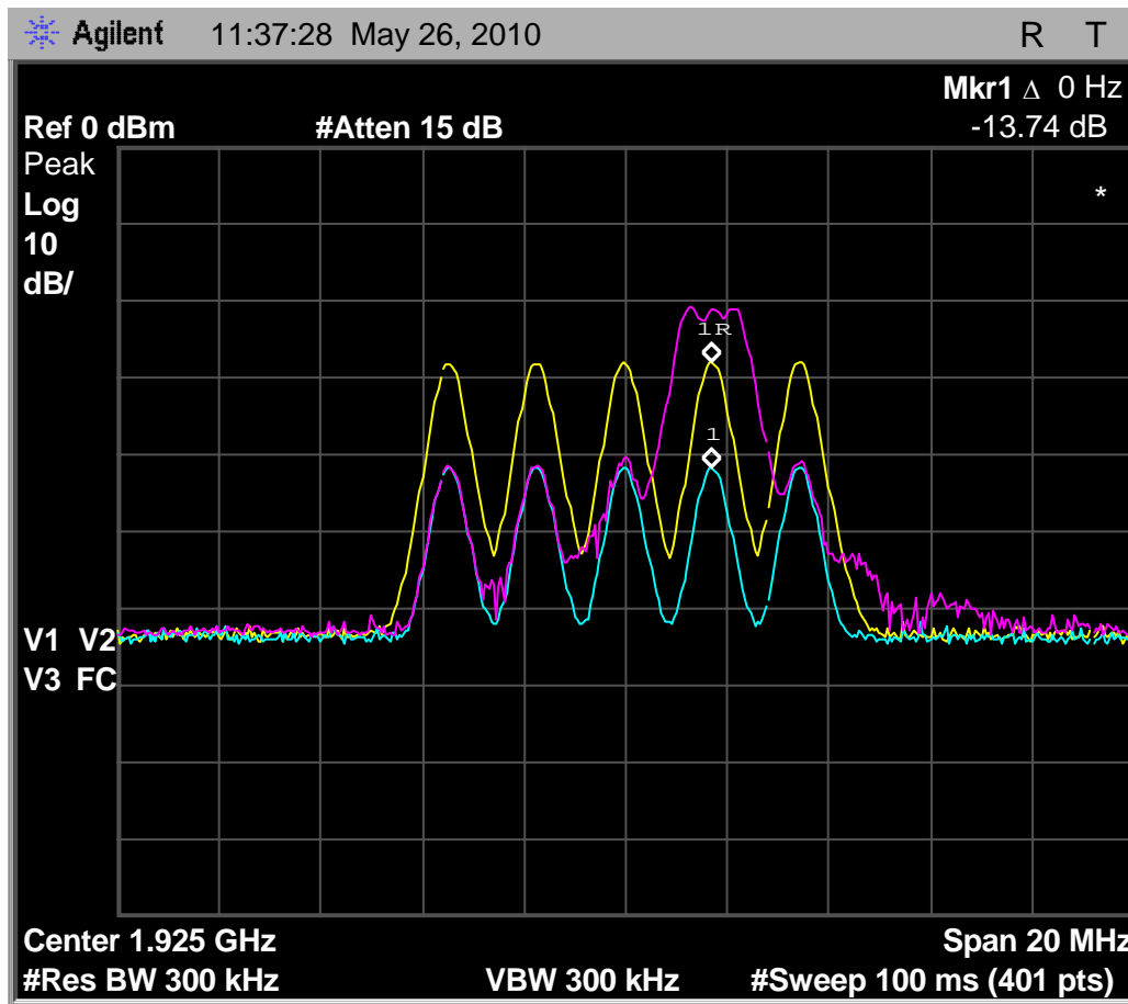
Fig. 91 - Emissions and interference profile spectrum, headset EUT, test 7.3.1 in low power WBM.
