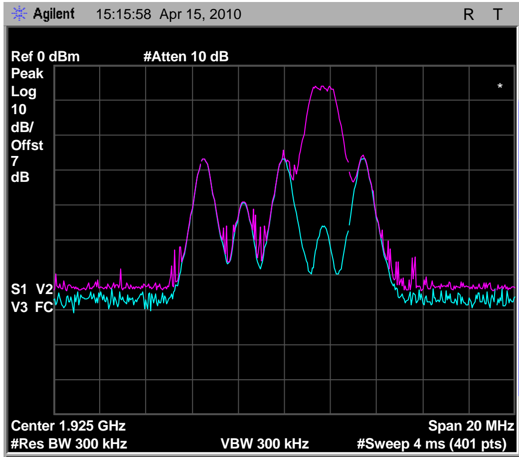
Fig. 44 - Emissions and interference profile spectrum, headset EUT, test 7.3.3(c).
