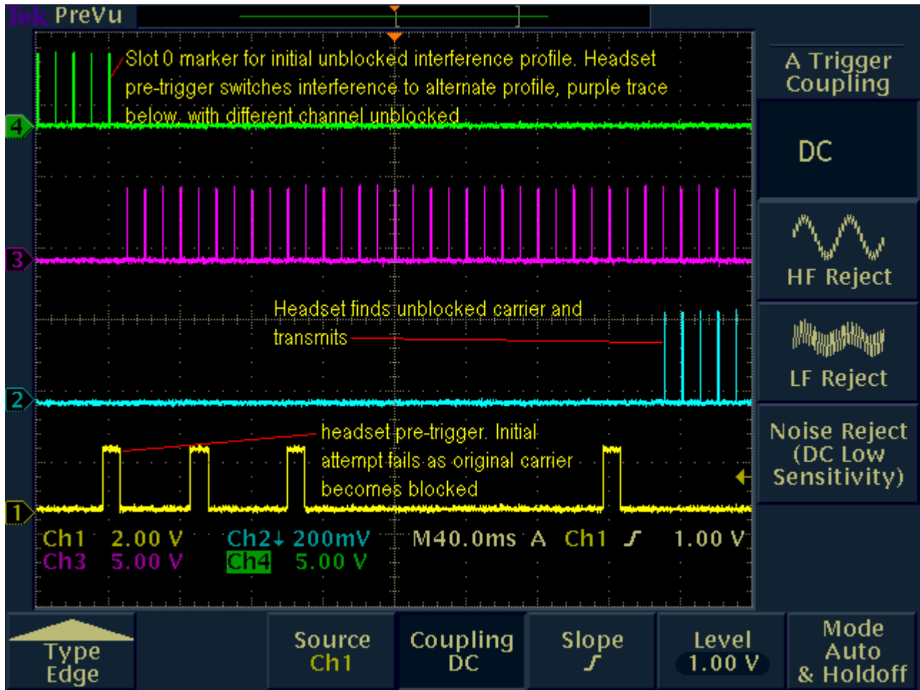
Fig. 48 - Screen shot of oscilloscope showing deferral by the headset EUT in the case where the interference profile changes in the frame previous to intended transmission and the selected time and frequency communications channel becomes blocked; and then later, transmission on unblocked channel.
