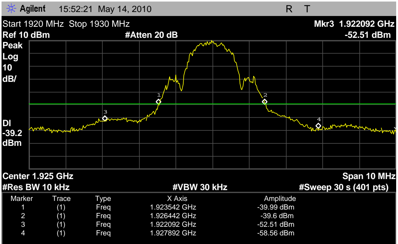
Fig. 20 - Spectrum analyzer screenshot for transmit emissions showing inband unwanted emissions with the headset EUT transmitter at the middle carrier, 1924.992MHz, according to the requirements of 6.1.6.1.
