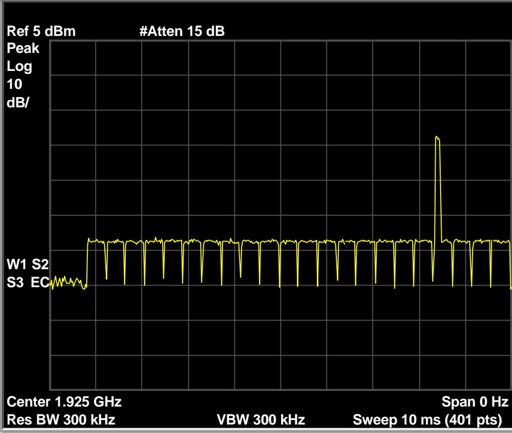
Fig. 83 – Interference profile for the Headset EUT that is above the threshold of -75.6\text{dBm} ( T_L + U_M ) without an open time slot pair. Headset EUT transmit slots that are interference free are 0 and 1 (one WBM slot).
