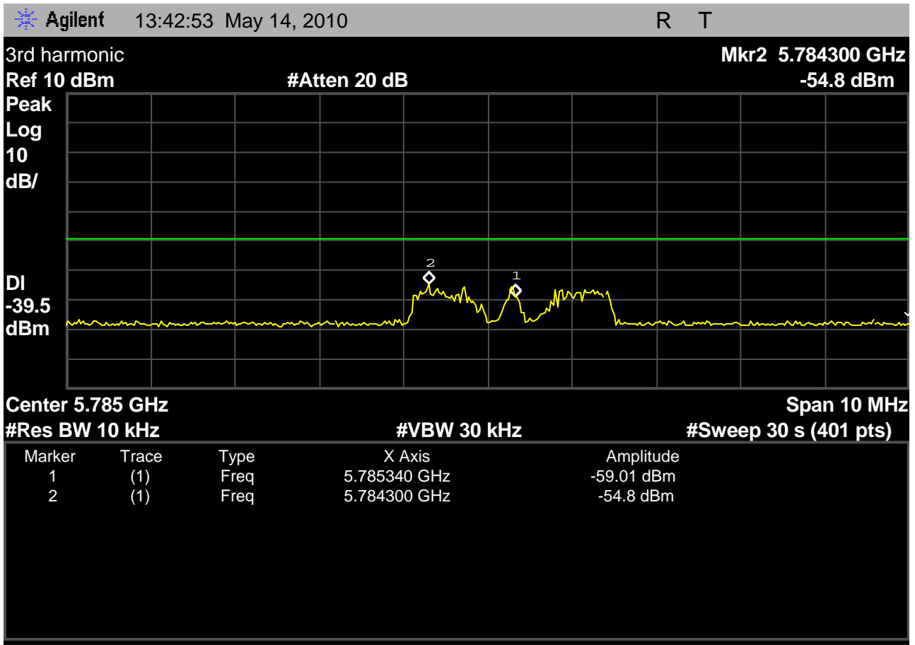
Fig. 36 – headset emissions measured in 10kHz resolution bandwidth in the region where the 1935MHz to 19.3GHz sweep at 300kHz observed a 3 rd harmonic response, for the headset transmitting on the high carrier, 1928.448MHz. A peak of -54.8dBm is measured in the specified bandwidth with a margin of 15.3dB from the -39.5dBm spec limit was observed when measured in the specified resolution bandwidth.
