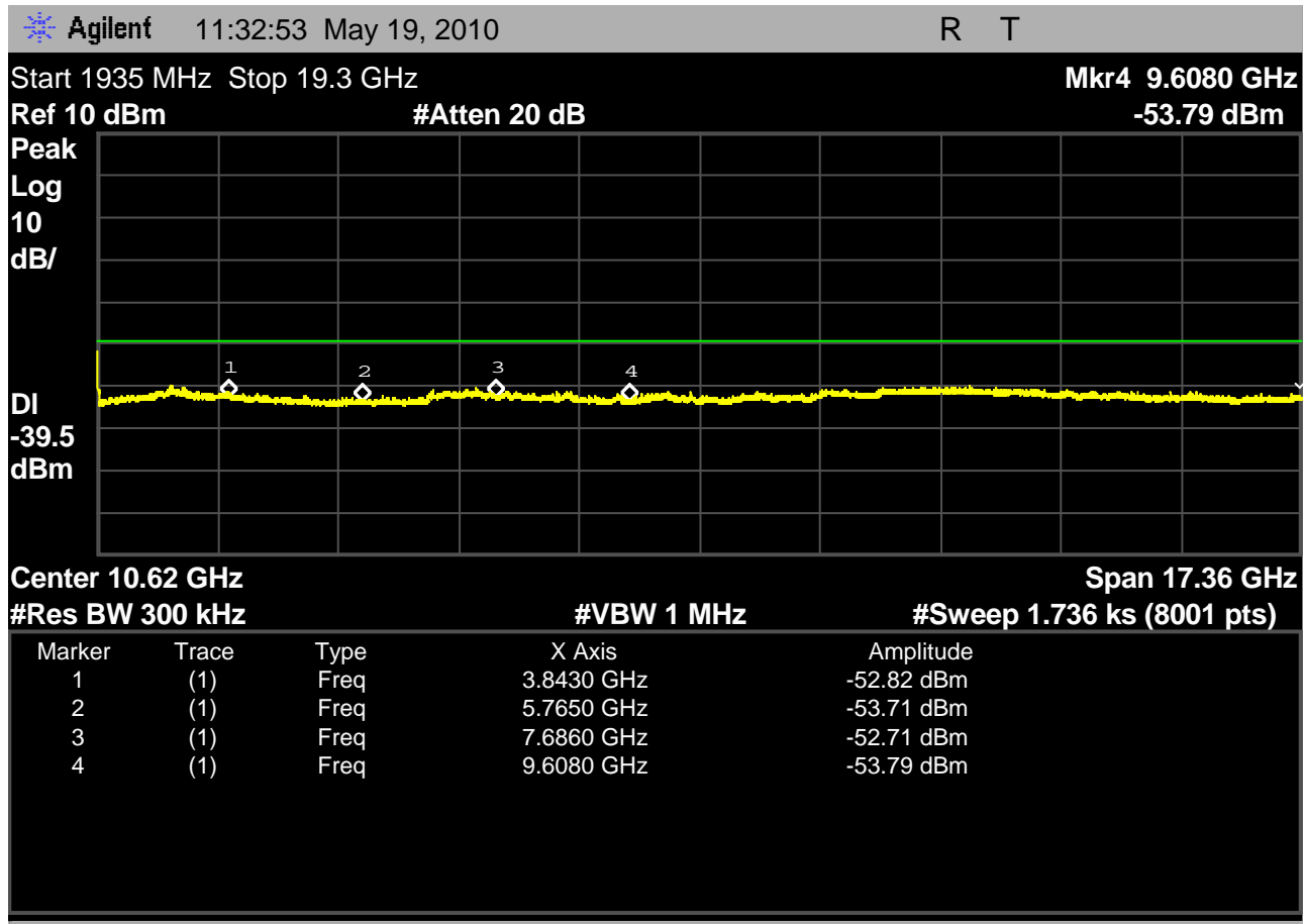
Fig. 89 - Headset EUT in minimum power WBM on low carrier, passes even with 10x the resolution bandwidth setting, all harmonics below maximum power mode, see section 6.1 of main report.
