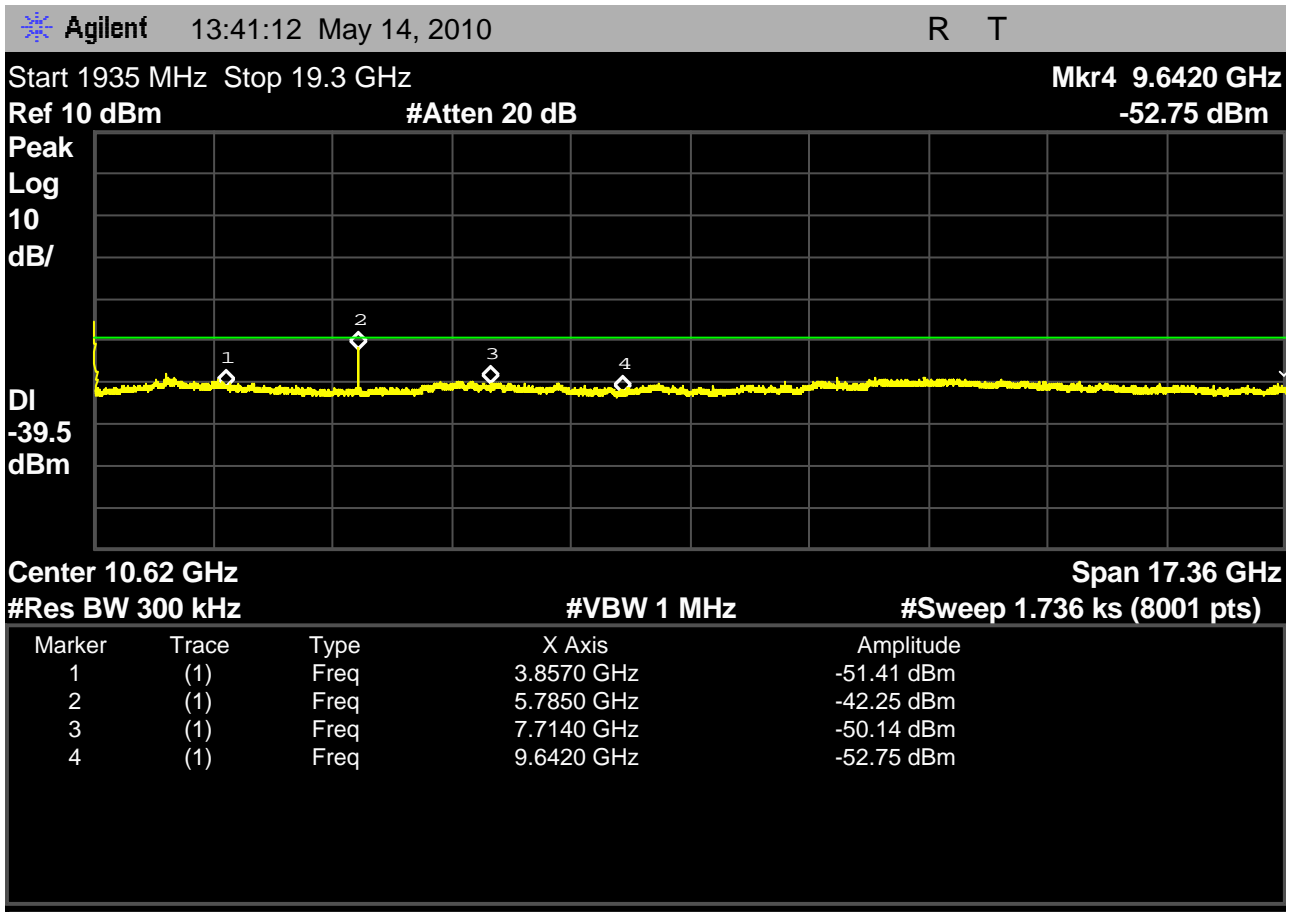
Fig. 34 – headset EUT out-of-band emissions including the regions from 1935MHz to 19.3GHz with the headset EUT transmitting on the highest carrier, 1928.448MHz.
