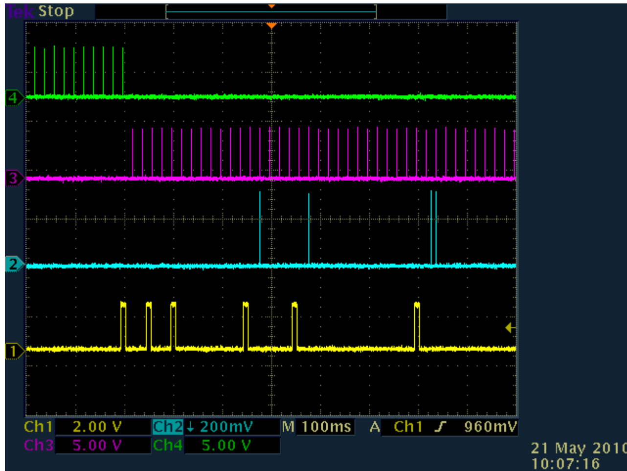
Fig. 60 - Screenshot of headset transmit-attempt flag activity (yellow Ch1 bottom trace) and RF detector output (cyan Ch2 2 nd from bottom) vs. time with the interference profiles (Ch4 is the primary interference which has an opened carrier (-130dBm interference level) and allows the headset and companion Base to idle lock to each other. The magenta trace is the Ch3 alternate interference profile which is automatically switched to when the headset TALK button is pressed. The headset tries to bring up a link without success as shown by (Ch2) RF detector having no signal after the initial attempts. The test was repeated and the RF detector trace monitored for 20 minutes without any further activity. In order to perform this test the headset heartbeat transmissions was disabled (heartbeat is every 30 seconds) and the heartbeat would continuously trigger the interference generator as well as have the headset transmit every 30 seconds since the interference is not above the threshold level.
