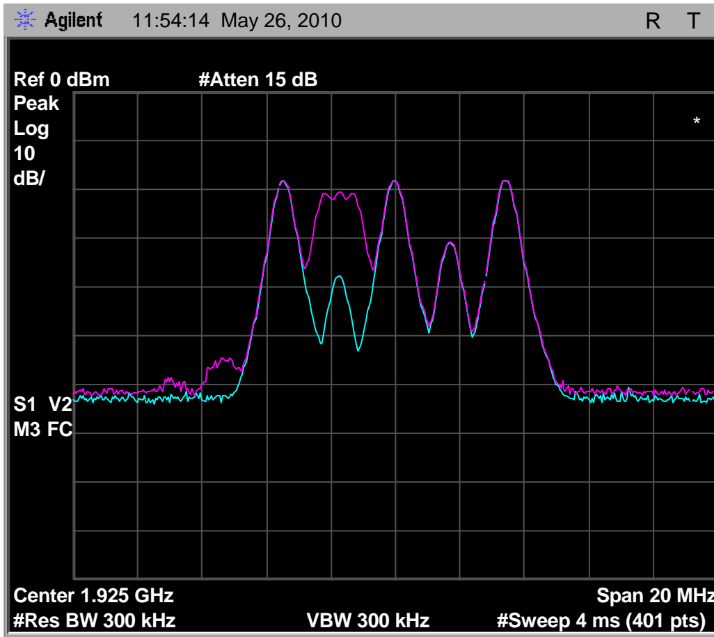
Fig. 93 - Emissions and interference profile spectrum, headset EUT, test 7.3.3(b).
