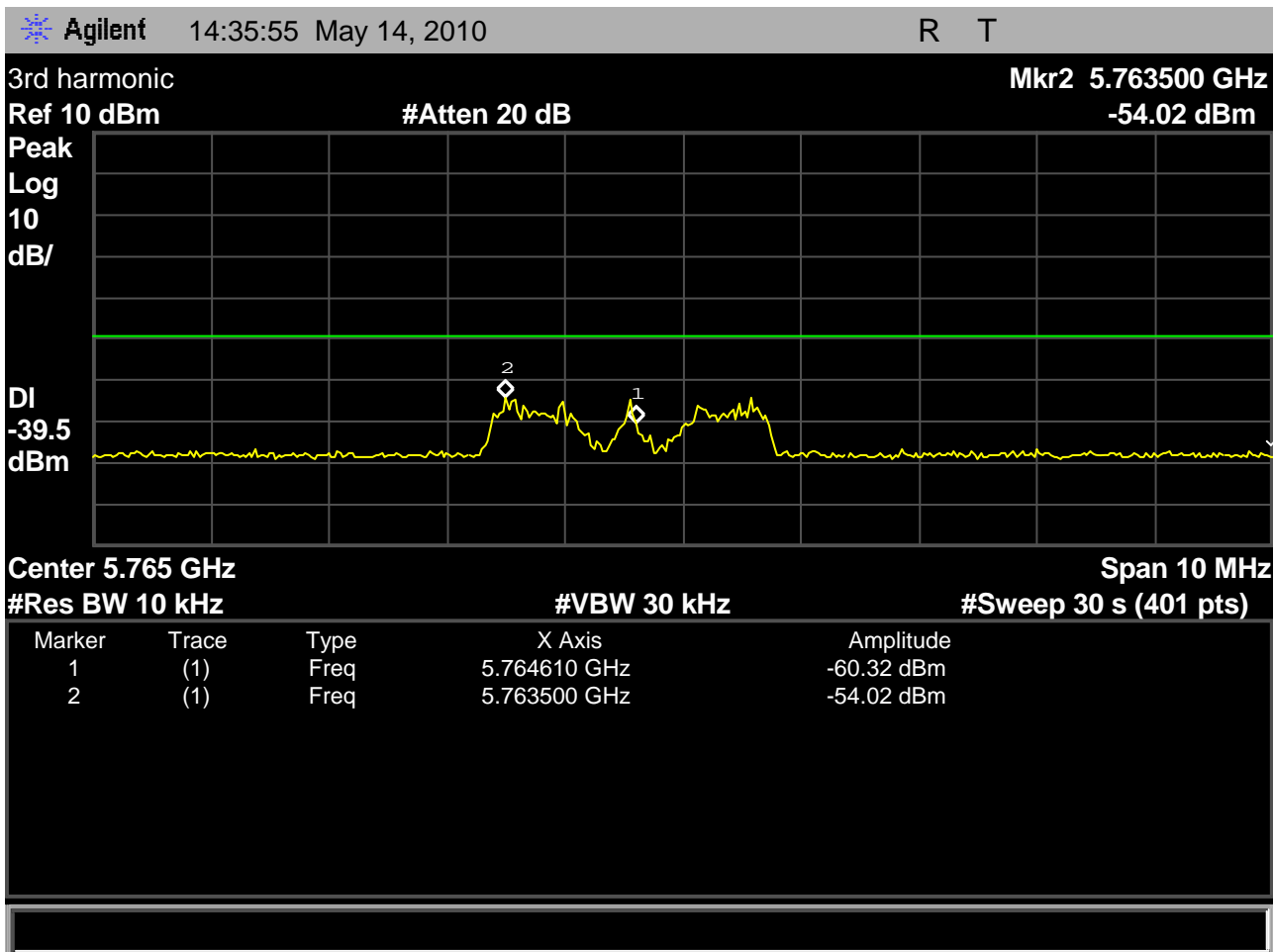
Fig. 28 – headset EUT out-of-band emissions in the region around the 3rd harmonic, with the headset EUT transmitting on the lowest carrier, 1921.536MHz.
