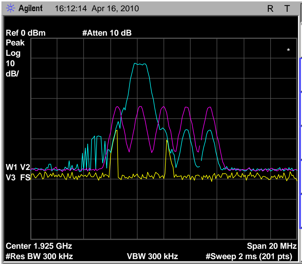
Fig. 53 - Transmit spectrum of 50uS interference pulses, with headset EUT no longer deferring with interference pulses of level T_U - U_M .
