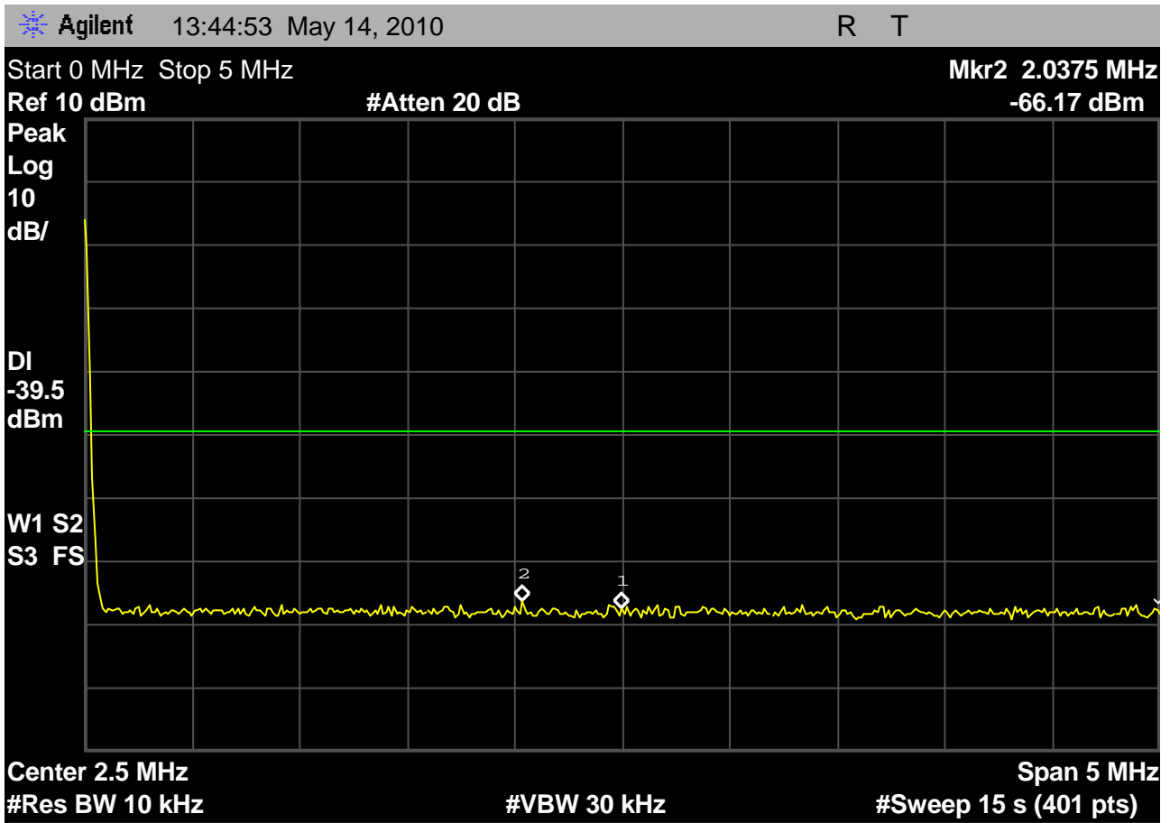
Fig. 30 – headset EUT out-of-band emissions showing the regions from DC to 5MHz, with the transmitter using the highest carrier, 1928.448MHz.
