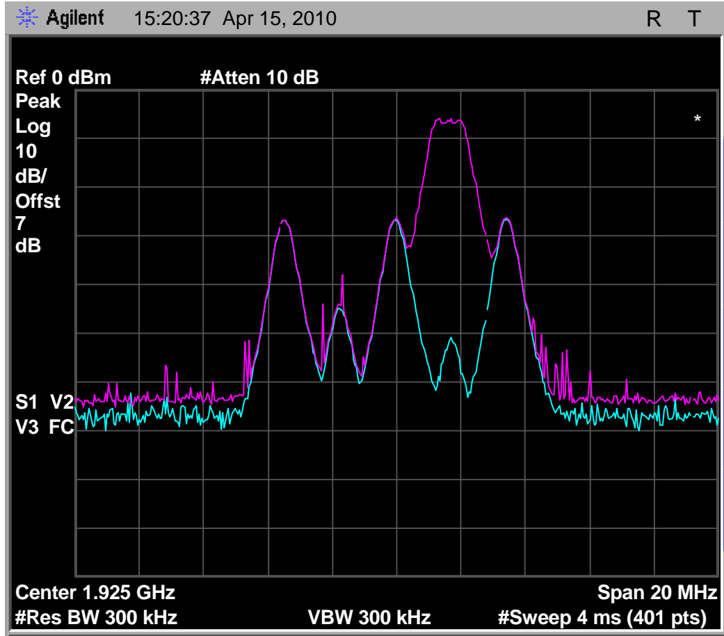
Fig. 46 - Emissions and interference profile spectrum, headset EUT, test 7.3.3(e).
