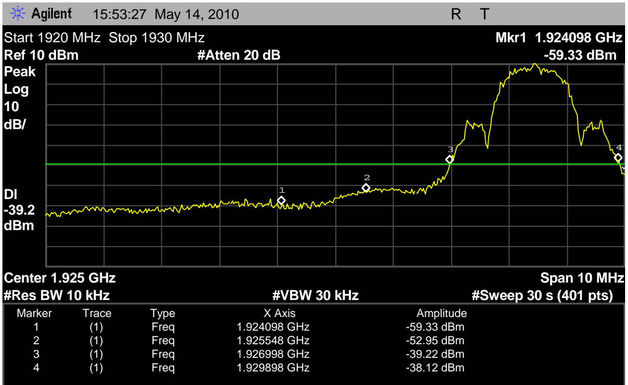
Fig. 21 - Spectrum analyzer screenshot for transmit emissions showing inband unwanted emissions with the headset EUT transmitter at the highest carrier, 1928.448MHz, according to the requirements of 6.1.6.1.
