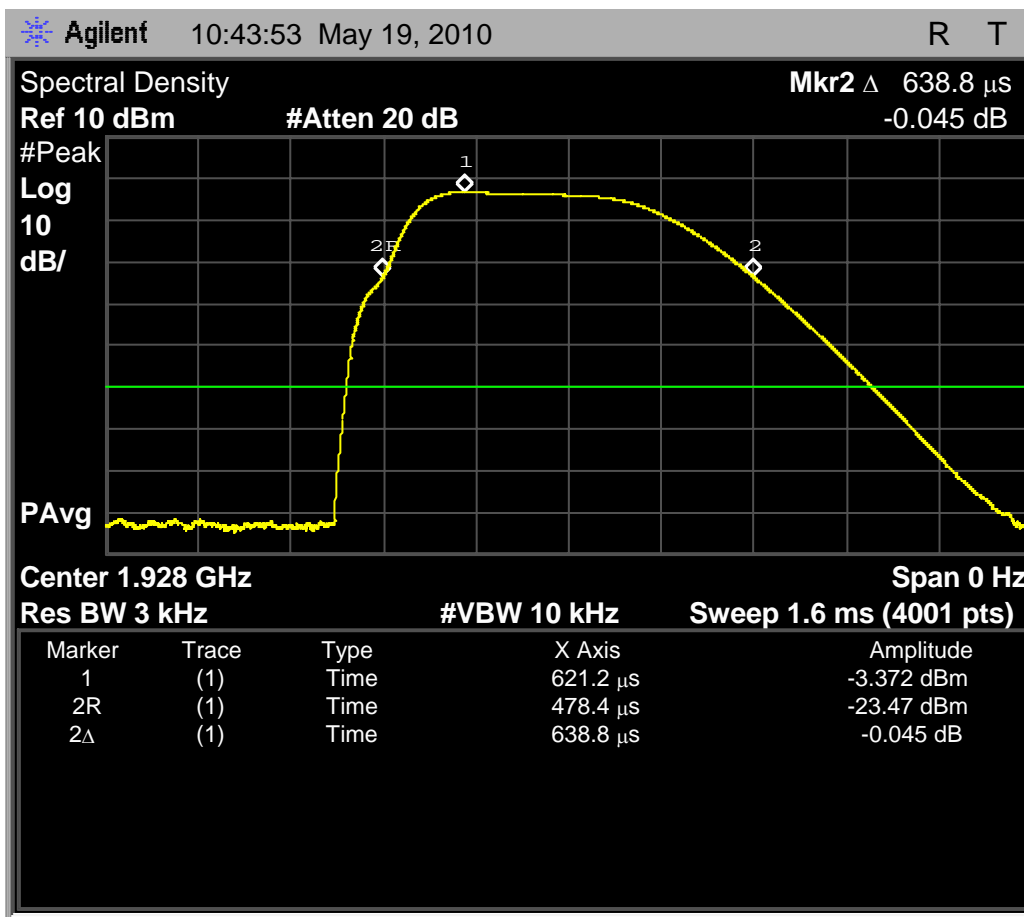
Fig. 17 – Zero-span sweep for headset EUT, high carrier, for 3kHz maximum power spectral density. The peak level is at -3.37dBm, and the interval between samples at the -20dB points is 638.8us.
