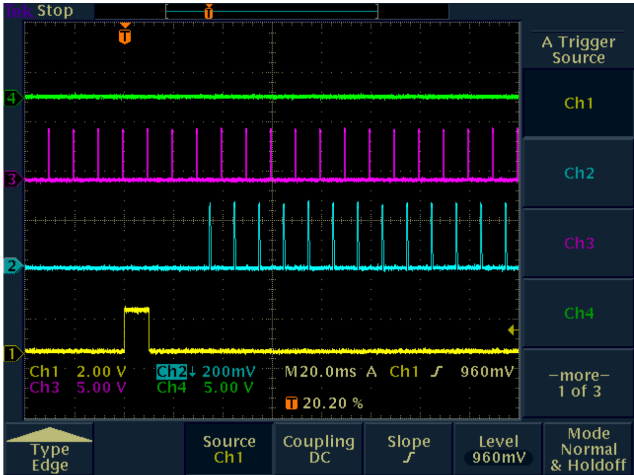
Fig. 54 - Normal initiation of transmissions by the headset EUT in the absence of over-threshold interference; the headset EUT software flags the start of the transmission setup (bottom yellow trace), and transmit emissions are recovered by the RF detector (third trace down-cyan) in the splitter/combiner network. The second trace from the top (magenta) indicates the interference profile was switched to T_U - U_M for which transmission is allowed. The top trace (green) was the T_U + U_M interference level, which prevented headset transmissions.
