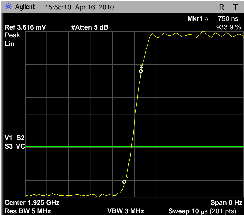
Fig. 51 - Rise time of interference pulse, per the requirements of 7.5 for less than 1uS for 10% to 90% transition.
