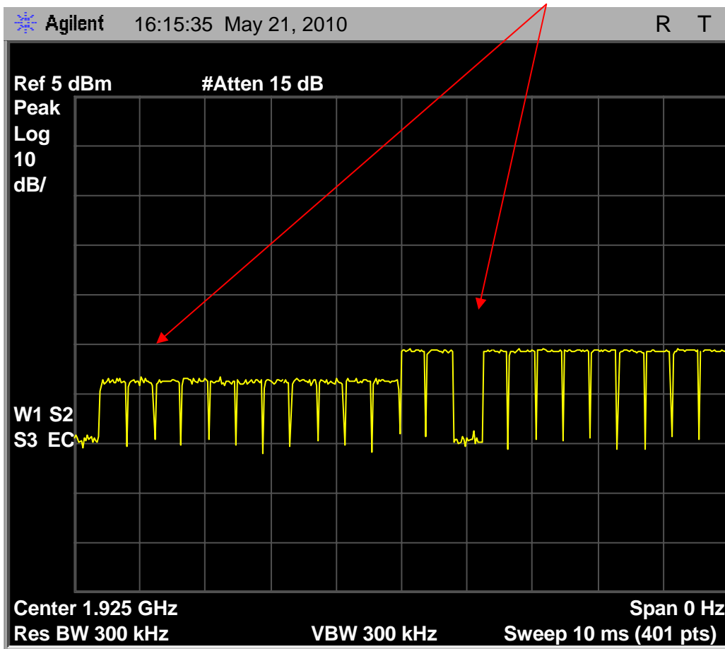
Fig. 67 – Spectrum analyzer screen capture of the interference pattern prior to headset link with companions Base (initial interference profile)
