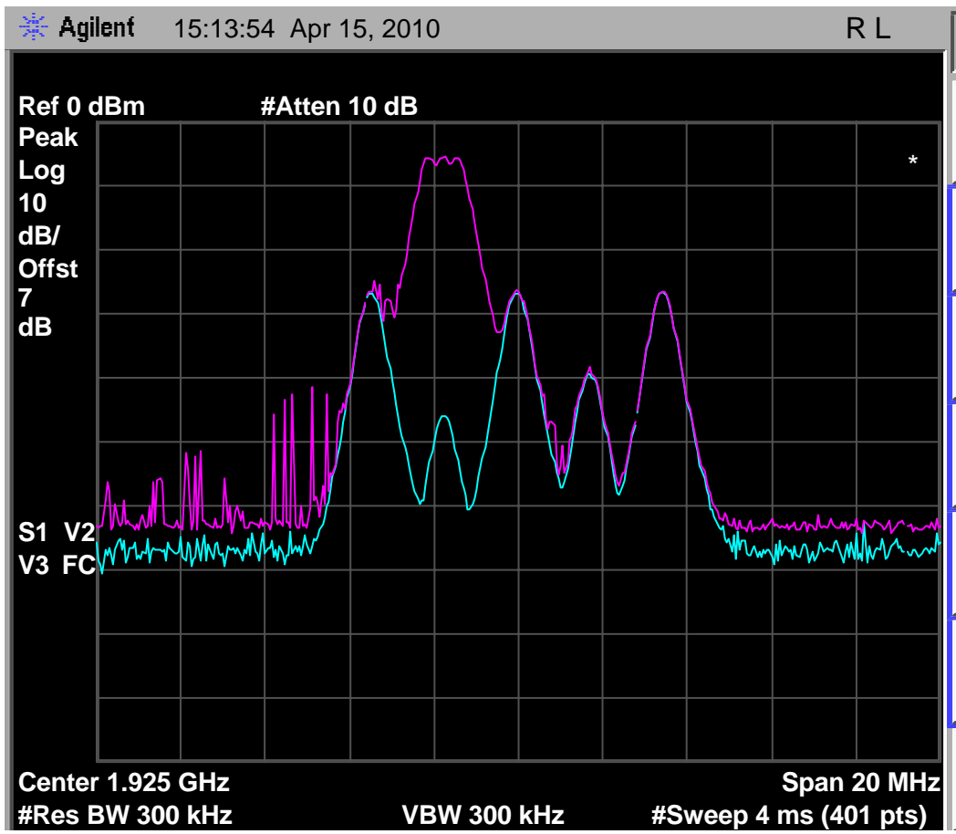
Fig. 43 - Emissions and interference profile spectrum, headset EUT, test 7.3.3(b).
