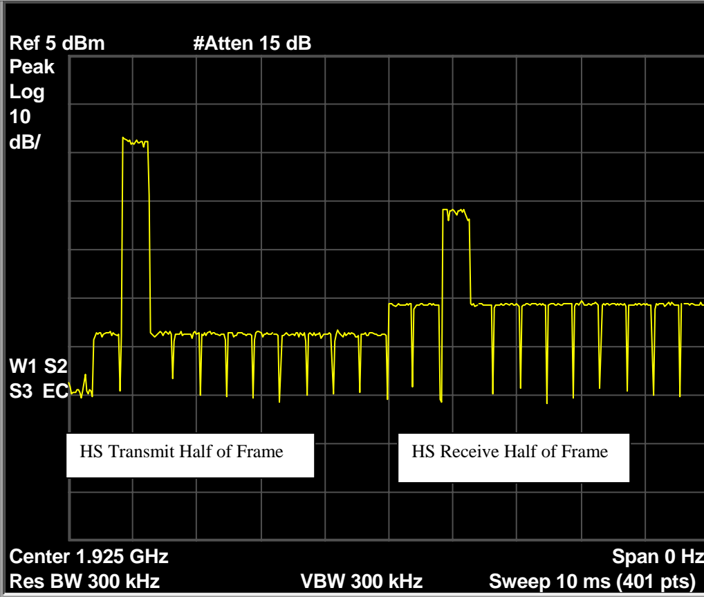
Fig. 68 – Headset EUT selects slot 2 pair which has the lowest maximum level of interference
