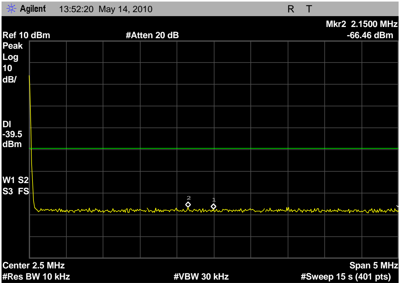
Fig. 22 – headset EUT out-of-band emissions showing the regions from DC to 5MHz, with the transmitter using the lowest carrier, 1921.536MHz.
