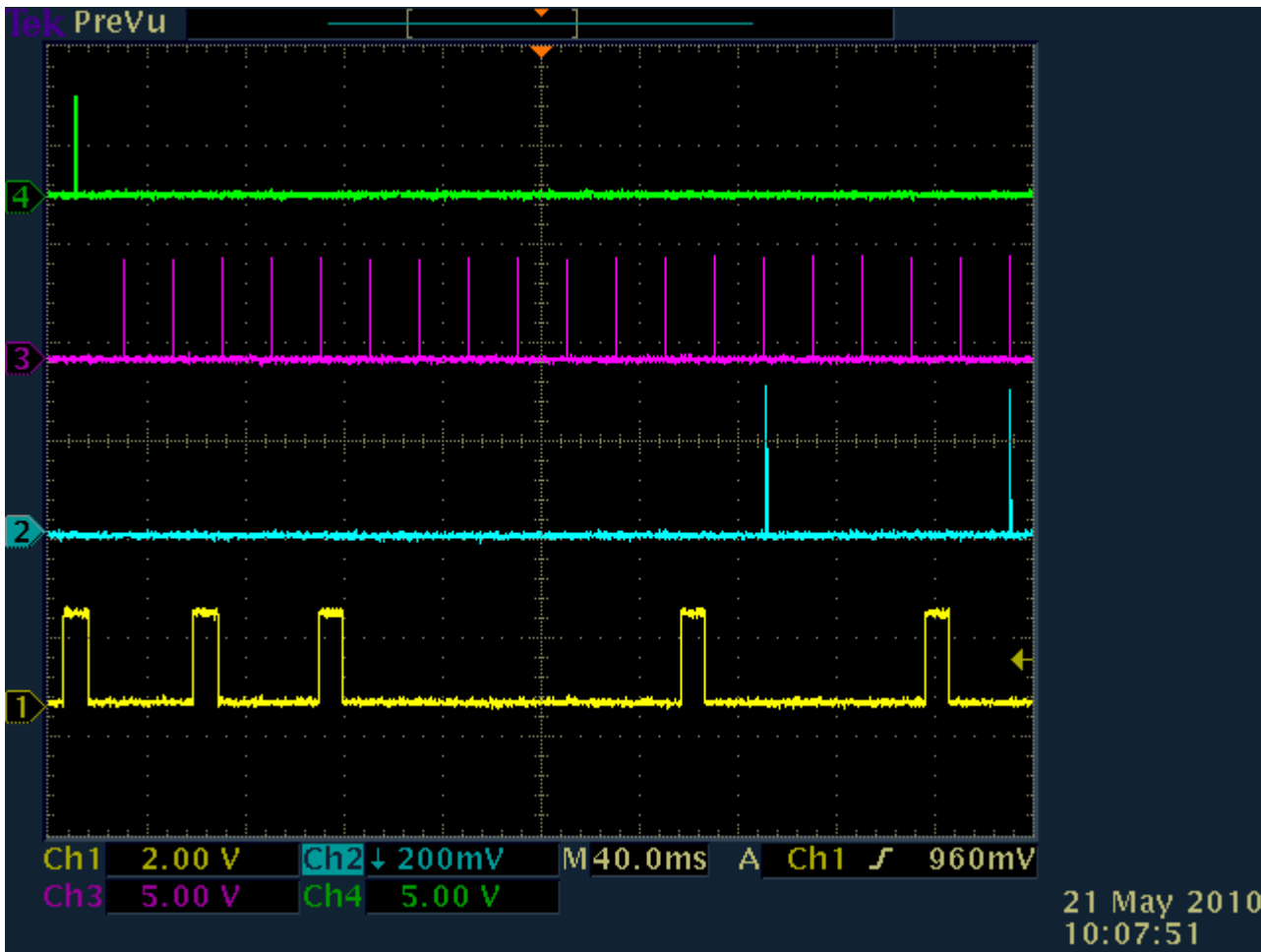
Fig. 61 – Screenshot zoom of the above figure. This screen capture shows that the first actual attempt to transmit a signal from the headset to the Base wasn't until the fourth attempt. The first 3 attempts Ch1 (yellow) trace have no corresponding RF output Ch2 (cyan) trace. The first attempt correctly recognizes that the interference level had changed and thus no RF transmission from Base to headset takes place, and the following two pulses on Ch1 also do not transmit as the RSSI (receive strength indicator) value is too large of a change, by the fourth Ch1 pulse the receiver has re-scanned the frequency time slots and found an acceptable (unblocked, and no large RSSI change) place to transmit.
