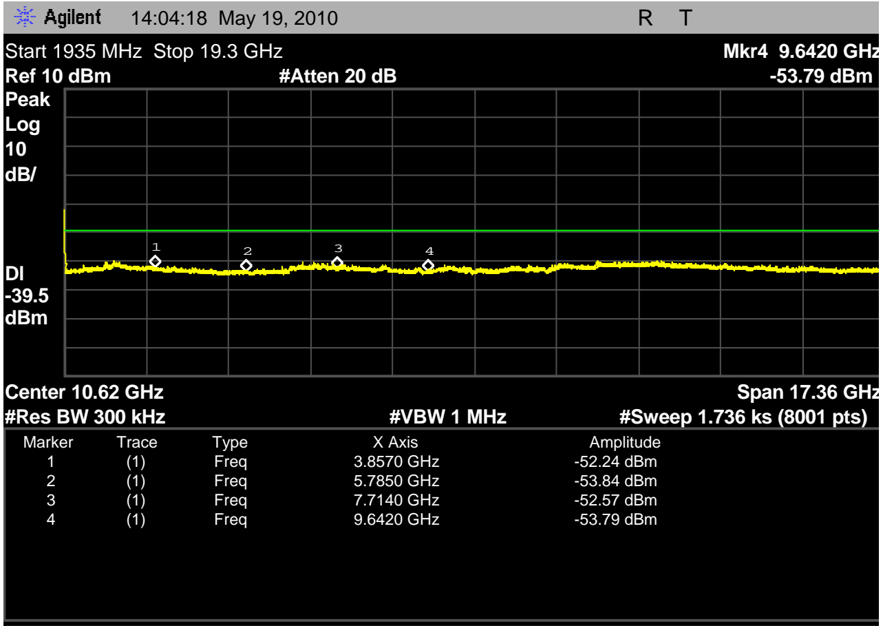
Fig. 90 - Headset EUT in minimum power WBM on high carrier, even with 10x the resolution bandwidth setting, all harmonics below maximum power mode, see section 6.1 of main report.
