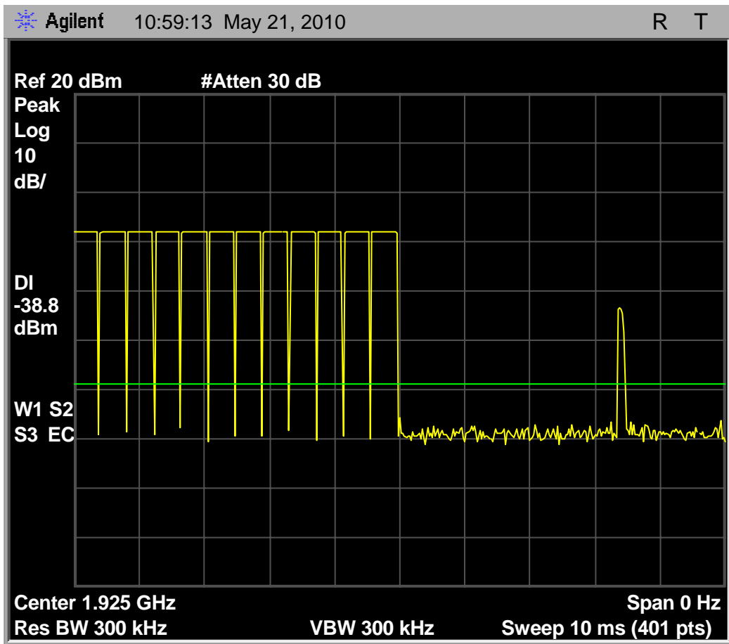
Fig. 59 - One frame of transmissions for a headset EUT and base companion device with a beacon present, interference present and high enough to block headset-to-base communications. Slots 0 – 11 have the interference present and the Base companion device transmit beacon signal is shown in slot 10.
