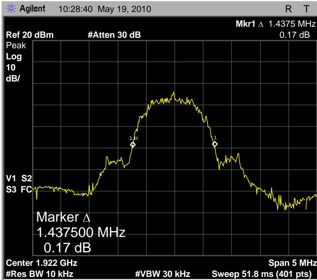
Fig. 86 - Headset EUT in WBM, 1.44MHz emissions bandwidth on low carrier vs. 1.43MHz in normal mode high power operation.
