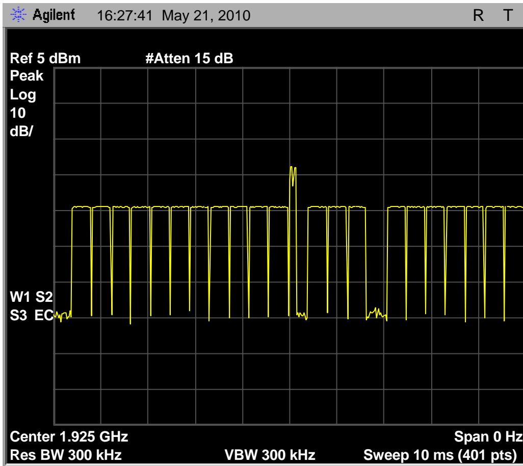
Fig. 72 – Interference profile for the Headset EUT that is above the threshold of -55.6\text{dBm} ( TU + UM ) without an open time slot pair. Slots that are opened are headset transmit slot 0 and headset receive slot 4 (slot 16). Note an additional time slot was opened to provide a place for the Base beacon of the companion device. If the base beacon was to occupy slot 0 or slot 16 a link could not be established and the test would pass but not be valid. Another option would be to force the Base to another carrier, but could not be monitored at the same time as the interference profile of interest.
