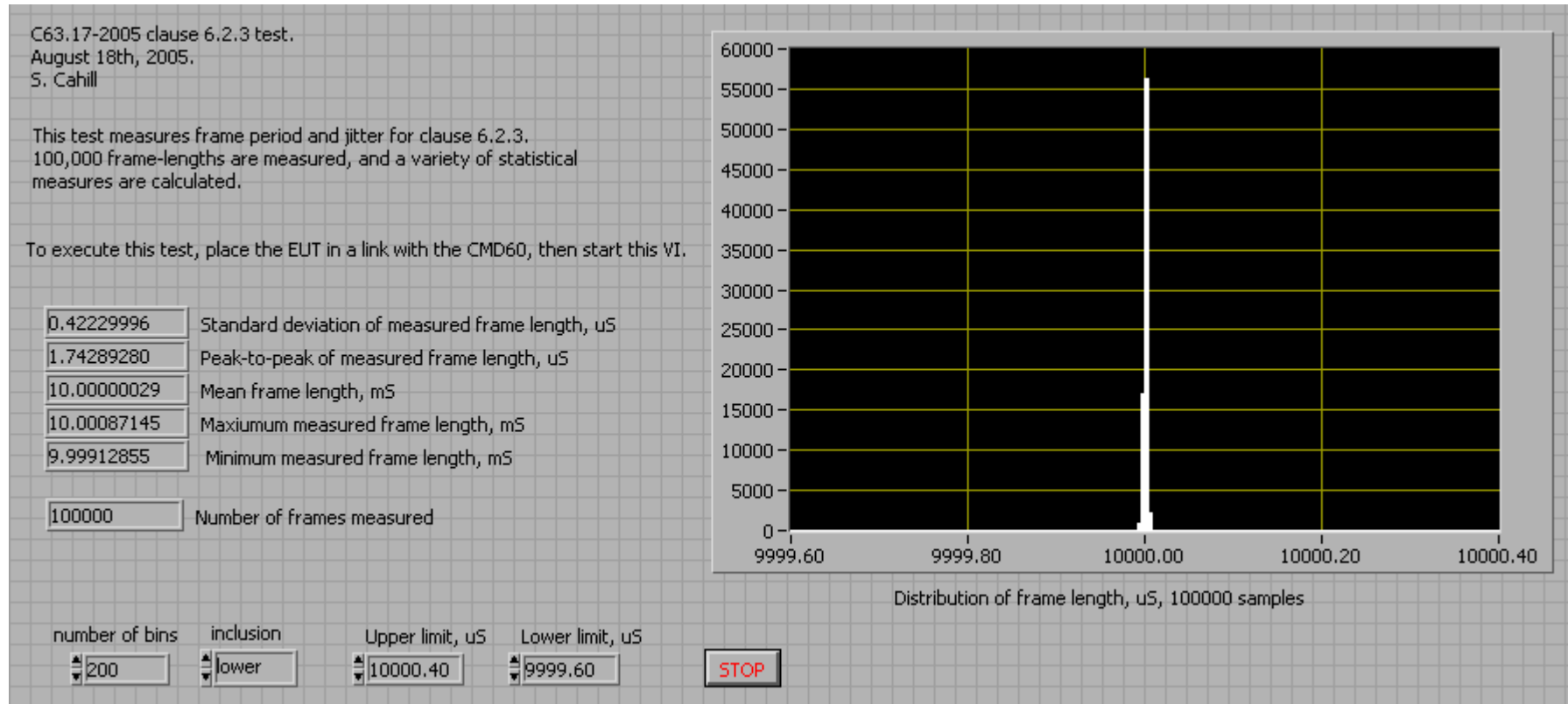
Fig. 41 - Test of headset EUT for frame period and jitter, according to the requirements of clause 6.2.3.
