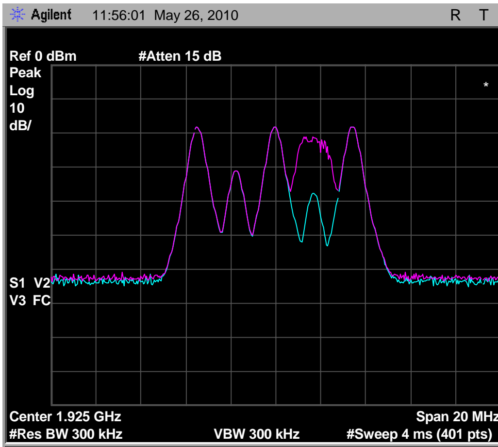
Fig. 94 - Emissions and interference profile spectrum, headset EUT, test 7.3.3(c).
