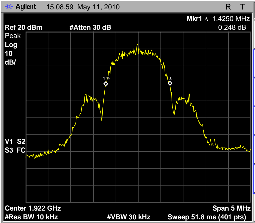
Fig. 10 - headset EUT, 1.43MHz emissions bandwidth on low carrier.
