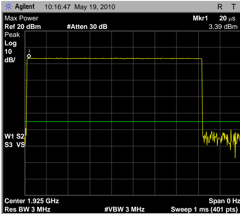
Fig. 85 - Headset EUT in WBM minimum power, max min power. The maximum minimum power measured was 3.39dBm.
