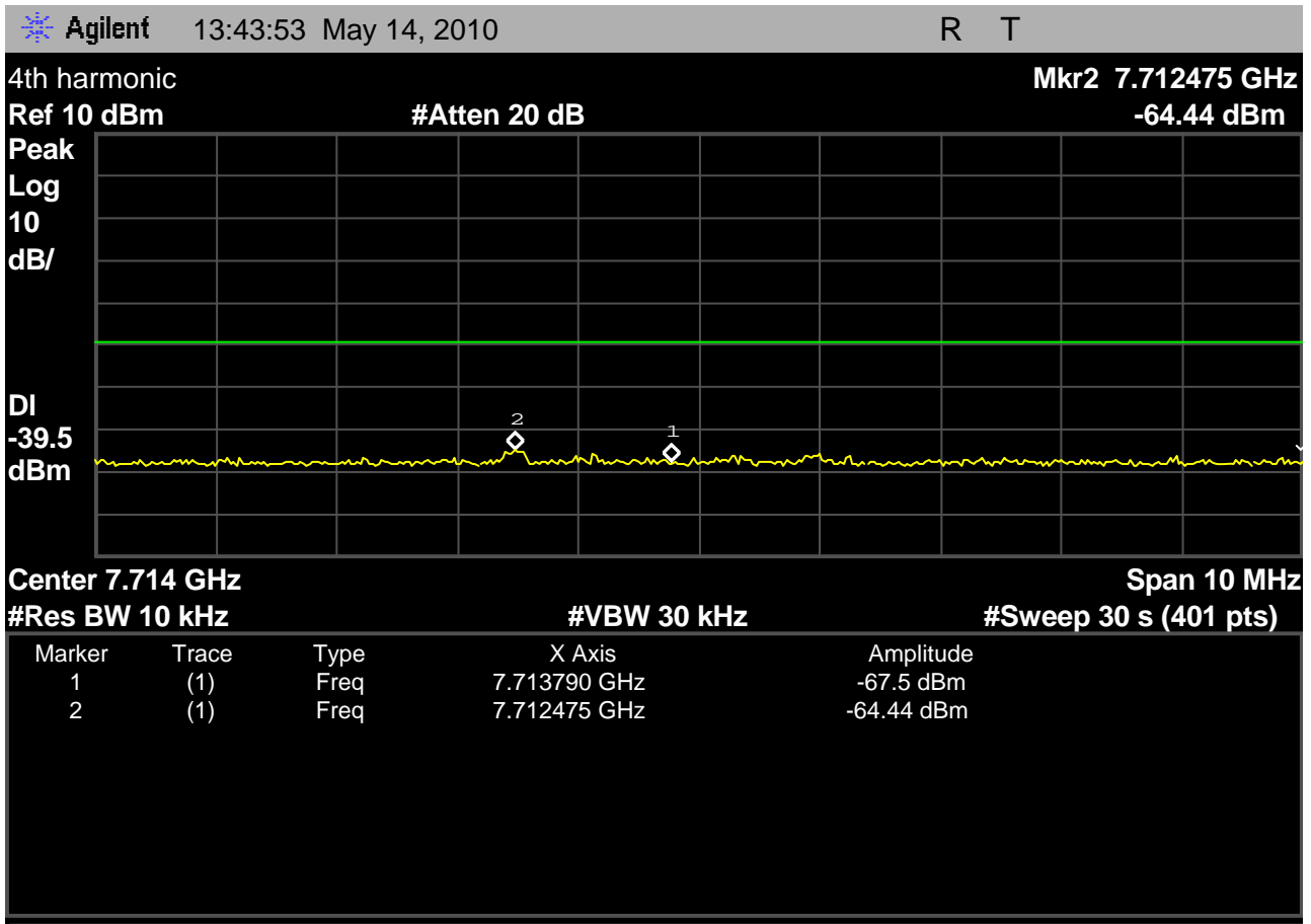
Fig. 37 – headset EUT out-of-band emissions in the region around the 4 th harmonic, with the headset EUT transmitting on the highest carrier, 1928.448MHz.
