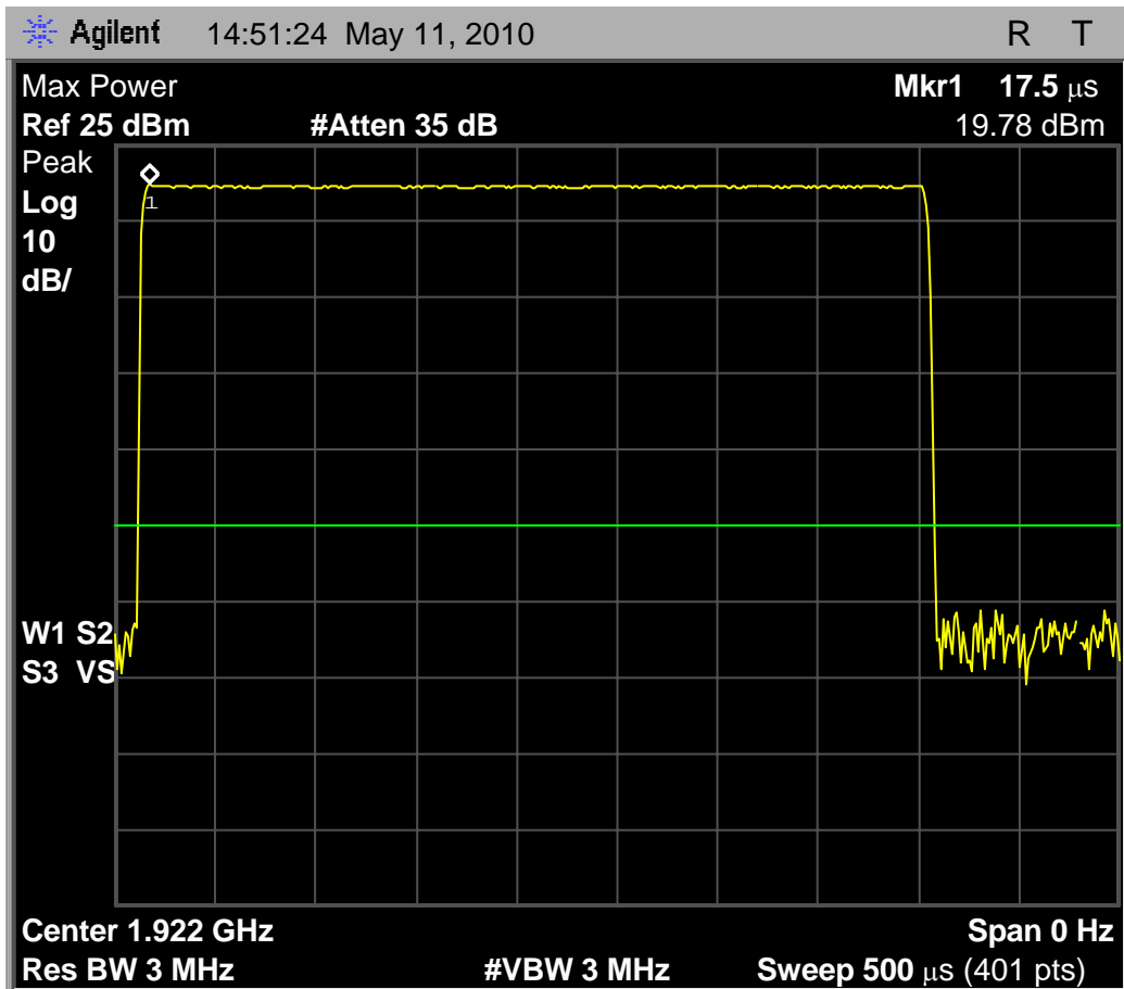
Fig. 7 - Headset EUT transmit power received by spectrum analyzer configured according to the requirements of clause 6.1.2 of C63.17-2006, low carrier. Maximum observed transmit power is 19.78 dBm.
