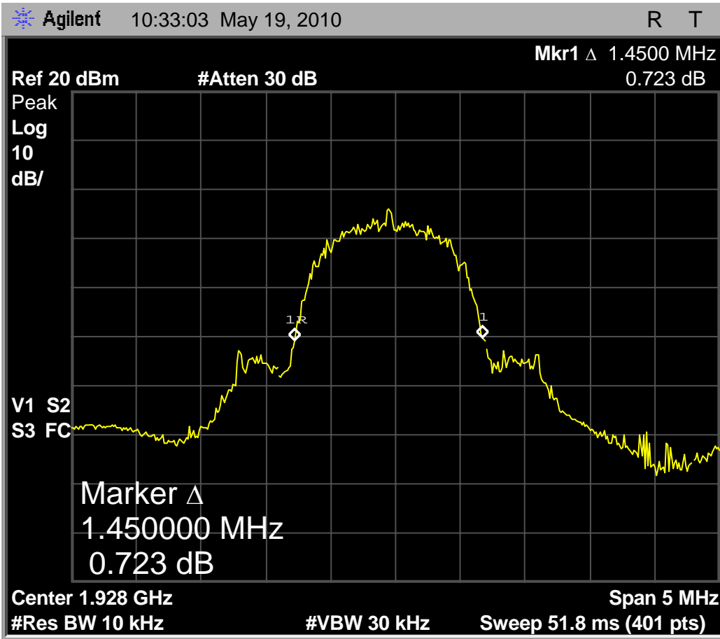
Fig. 88 - Headset EUT in WBM, 1.45MHz emissions bandwidth on high carrier vs. 1.45MHz in normal mode high power.
