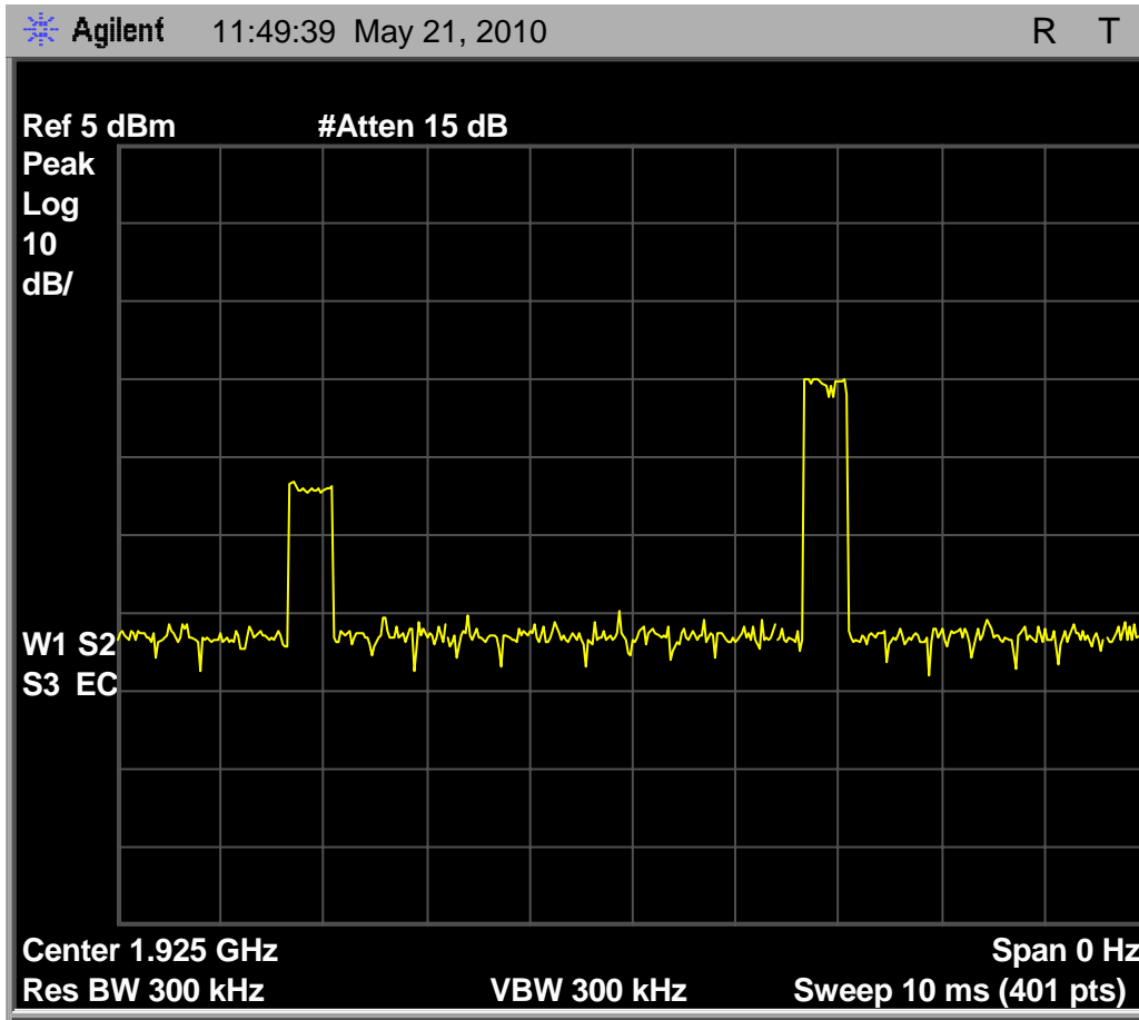
Fig. 62 - Screenshot of spectrum analyzer showing one frame of the channel with the initial interference profile present, which does not block the reception by the base EUT of the headset EUT's transmissions; an acknowledgement is generated when the headset EUT attempts to initiate the communications channel when the TALK button is pressed, and the communications channel is established, so the headset EUT meets the requirements of 8.2.1(b) for proper operation of the test setup when the acknowledgements are unblocked.
