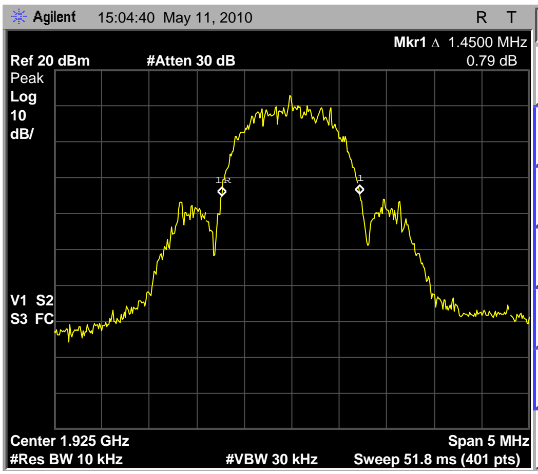
Fig. 11 - Headset EUT, 1.45MHz emissions bandwidth on middle carrier.
