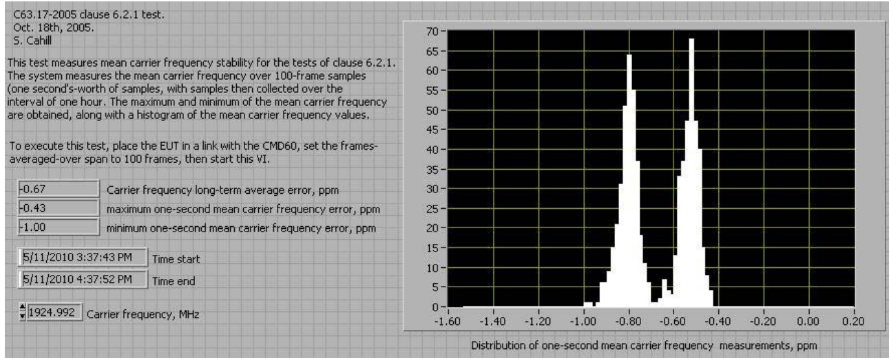
Fig. 38 - Measured one-second mean carrier frequency, headset EUT, and observed maximum, average value and observed minimum of the mean carrier frequency.
