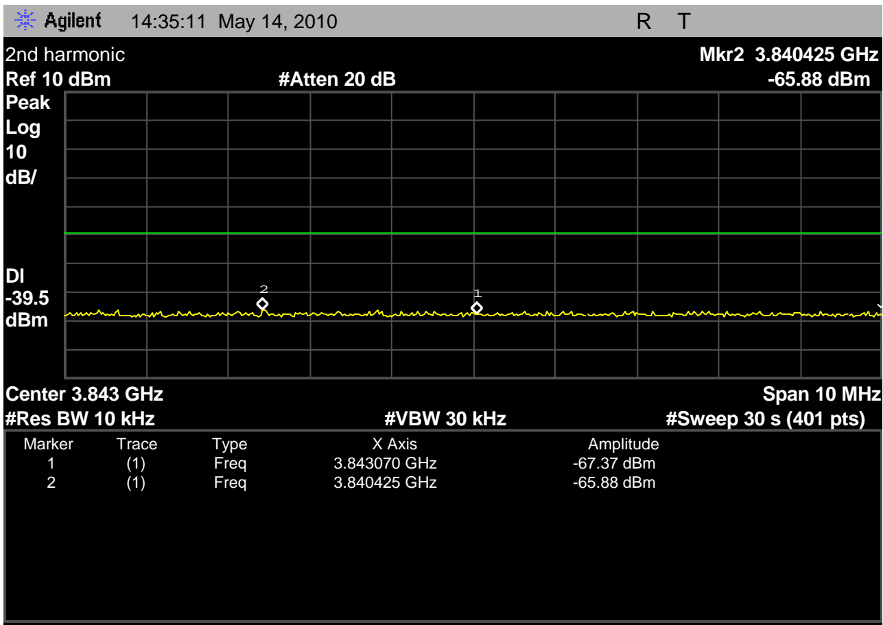
Fig. 27 – headset EUT out-of-band emissions in the region around the 2 nd harmonic, with the headset EUT transmitting on the lowest carrier, 1921.536MHz.
