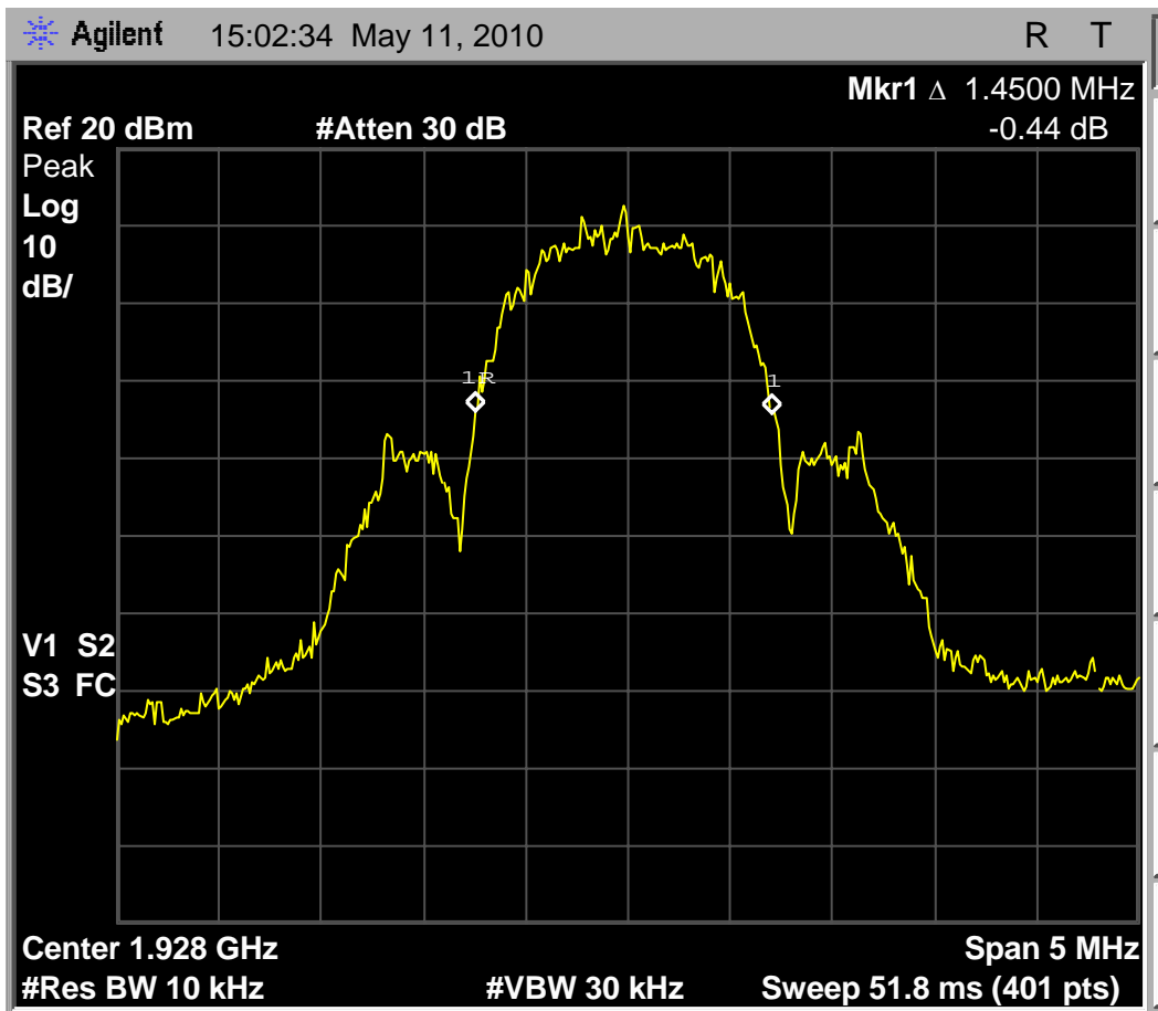
Fig. 12 - Headset EUT, 1.45MHz emissions bandwidth on high carrier.
