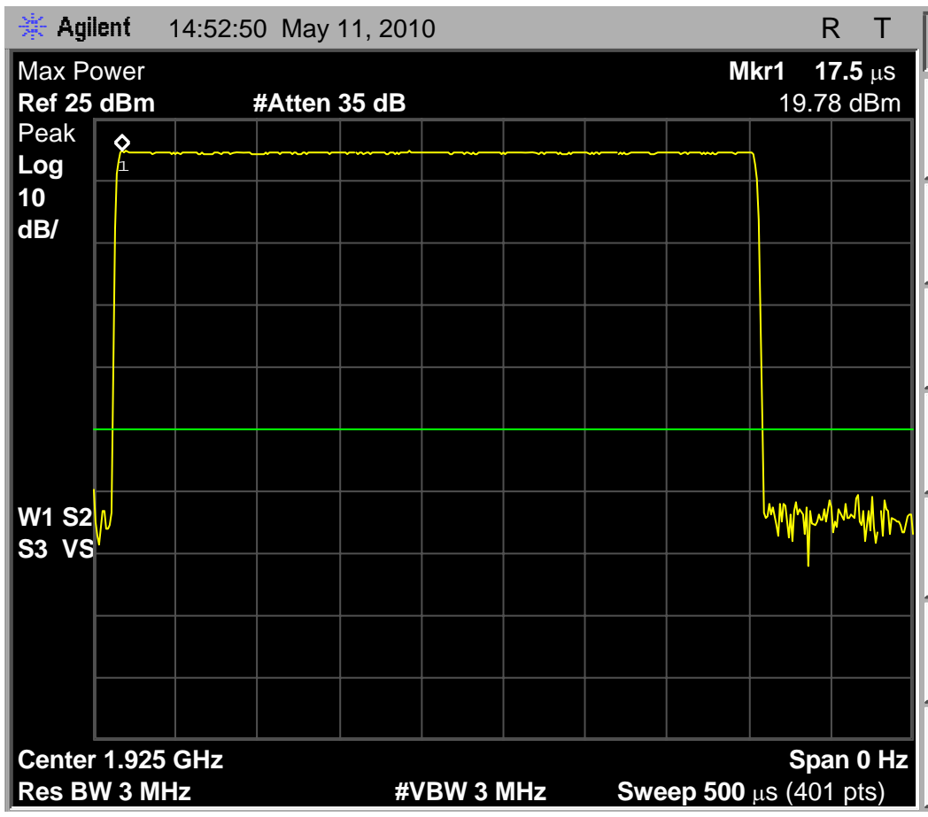
Fig. 8 - Headset EUT transmit power received by spectrum analyzer configured according to the requirements of clause 6.1.2 of C63.17-2006, mid carrier. Maximum observed transmit power is 19.78dBm
