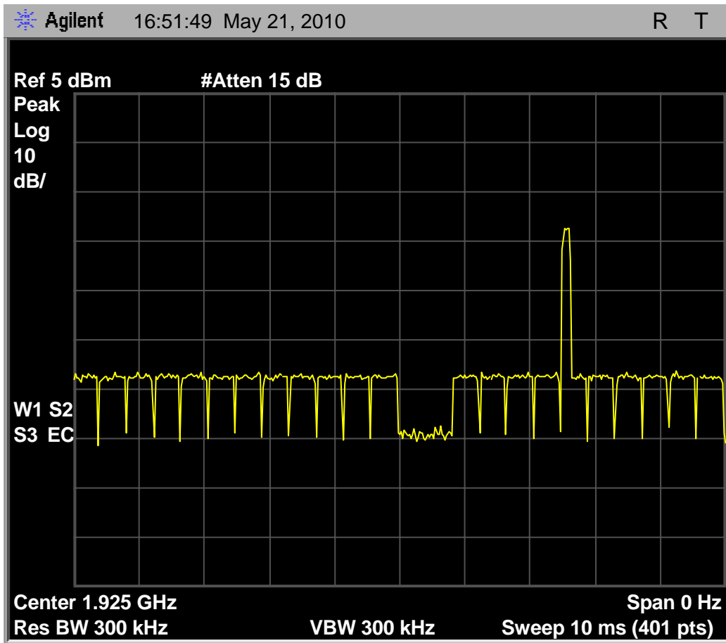
Fig. 81 – Interference profile for the Headset EUT that is above the threshold of -75.6\text{dBm} ( T_L + U_M ) without an open time slot pair. Slots that are interference free are headset receive slots 0 and 1 (slot 12 and 13).
