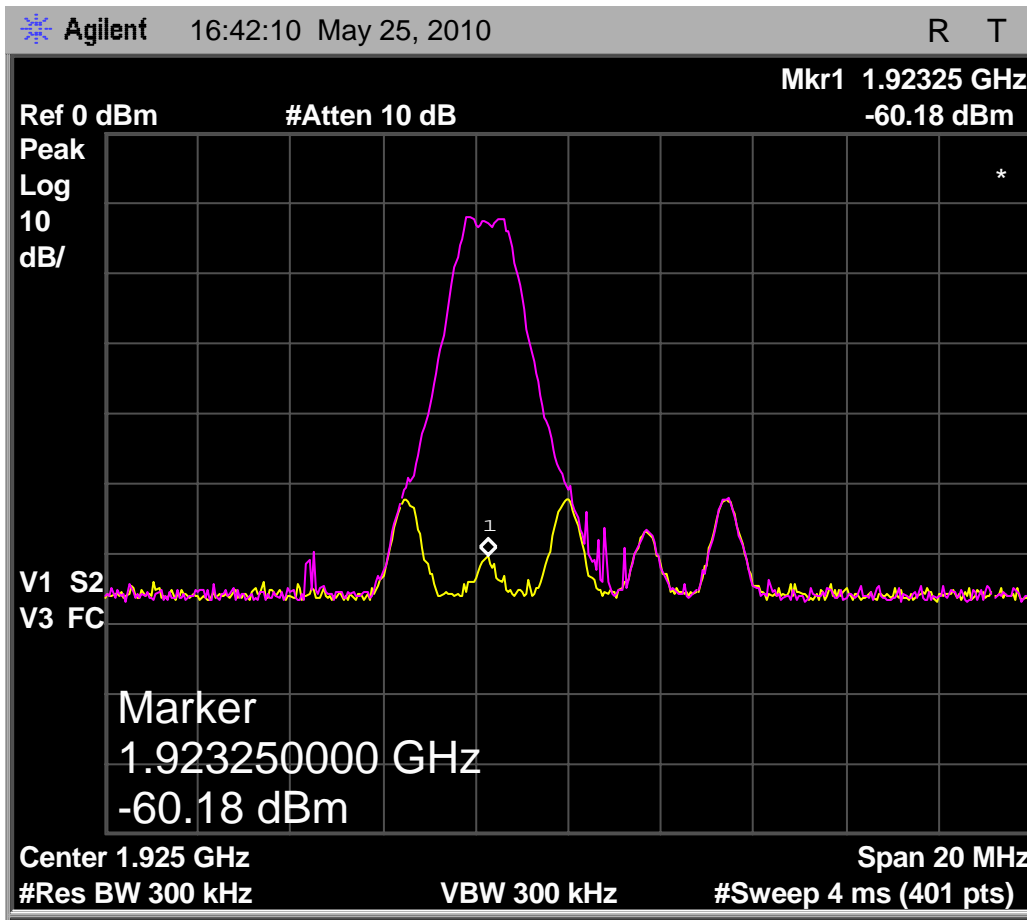
Fig. 76 - Emissions and interference profile spectrum, headset EUT, test 7.3.3(b).
