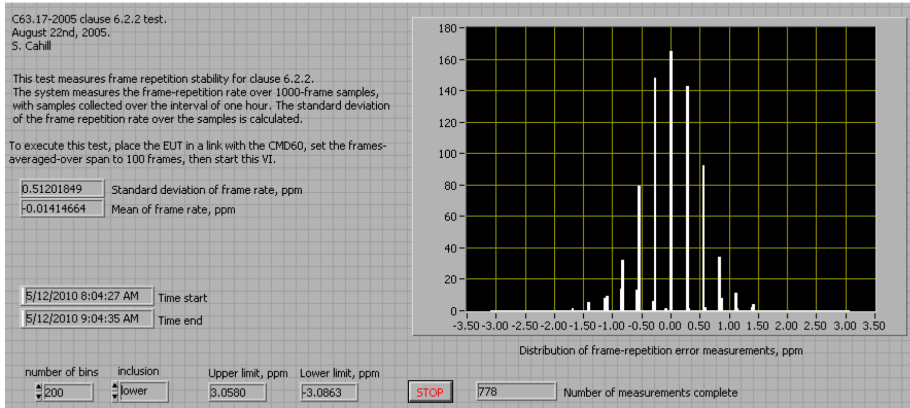
Fig. 40 - Test of headset EUT according to the conditions of clause 6.2.2 for frame repetition rate stability
