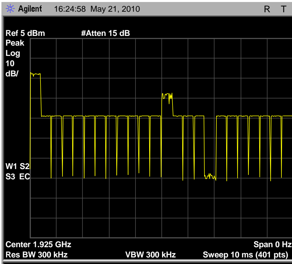
Fig. 71 – Interference profile for the Headset EUT that is above the threshold of -55.6\text{dBm} ( T_U + U_M ) WITH an open slot pair to demonstrate a link was possible for the test set up when 8.3.2 g) was performed.
