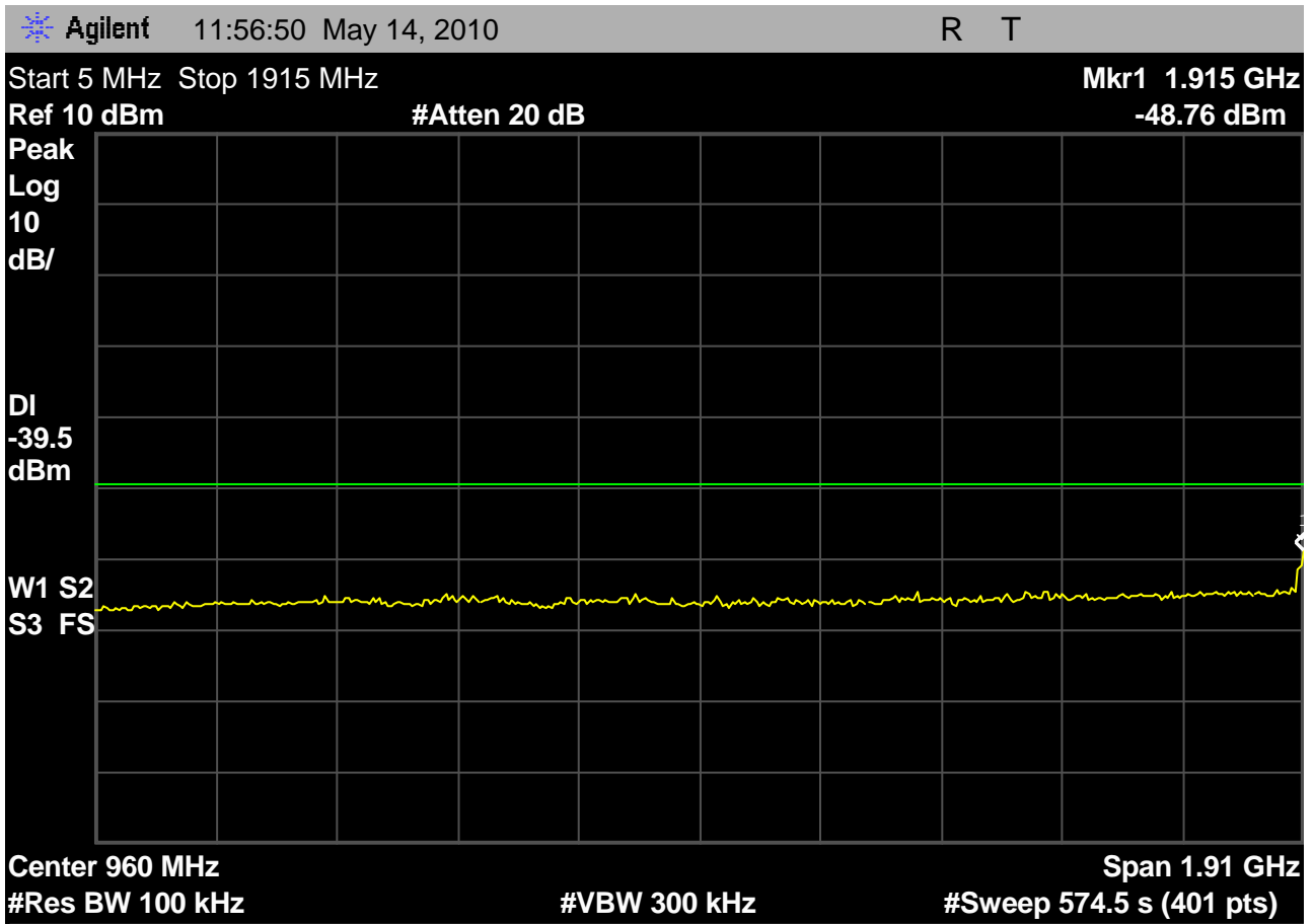
Fig. 23 – headset EUT out-of-band emissions showing the region from 5MHz to 1915MHz, with the transmitter using the lowest carrier, 1921.536MHz.
