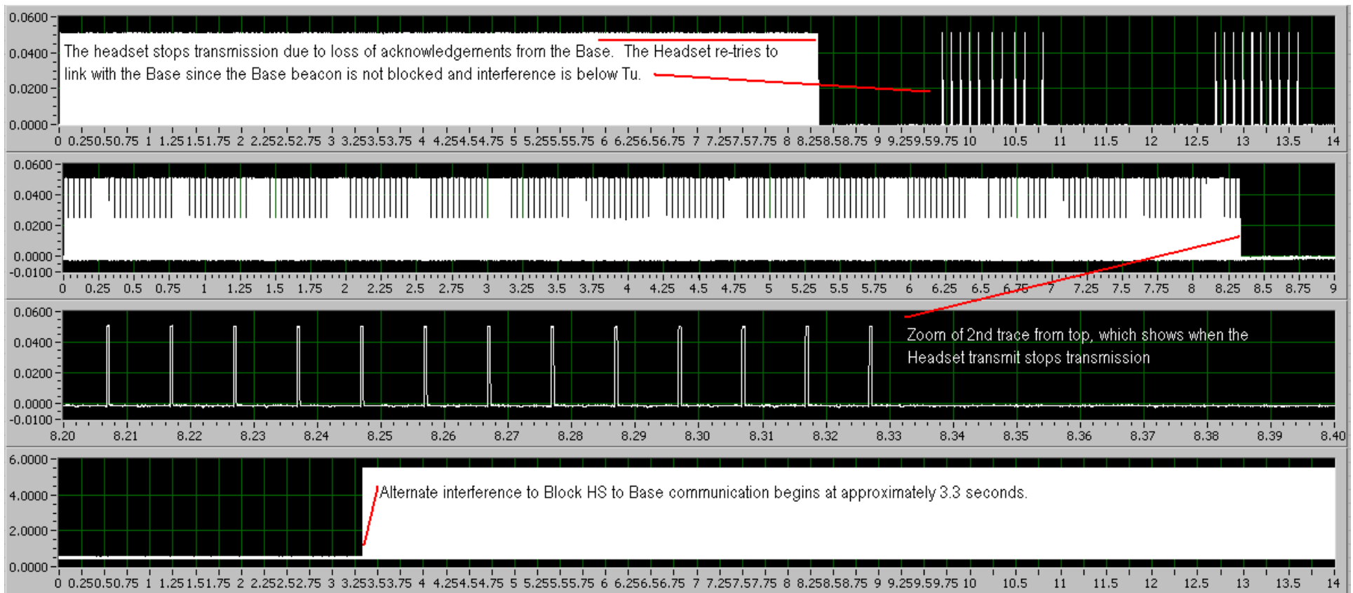
Fig. 64 - RF detector (top three traces) and alternate interference output (bottom trace) as headset EUT transmission goes blocked and transmissions stop.
