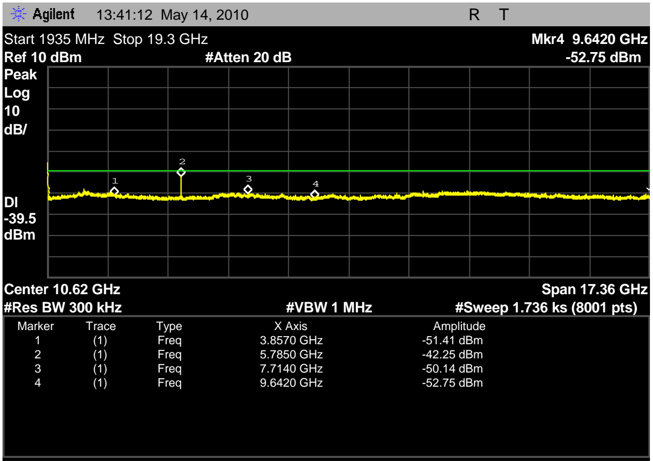
Fig. 26 – headset EUT out-of-band emissions including the regions from 1935MHz to 19.3GHz with the headset EUT transmitting on the lowest carrier, 1921.536MHz.
