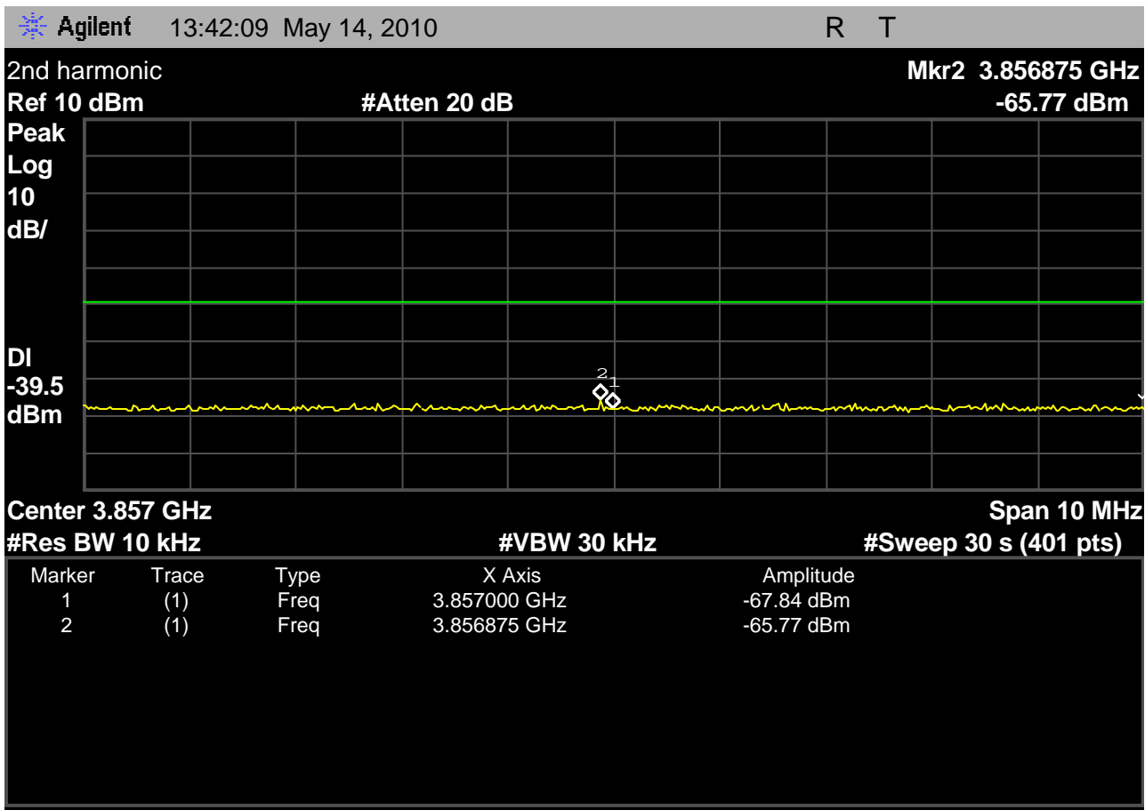
Fig. 35 – headset emissions measured in 10kHz resolution bandwidth in the region where the 1935MHz to 19.3GHz sweep at 300kHz observed a 2 nd harmonic response, for the headset transmitting on the high carrier, 1928.448MHz. A peak of -65.77dBm is measured in the specified resolution bandwidth, a margin of 26.27dB from the -39.5dBm spec limit.
