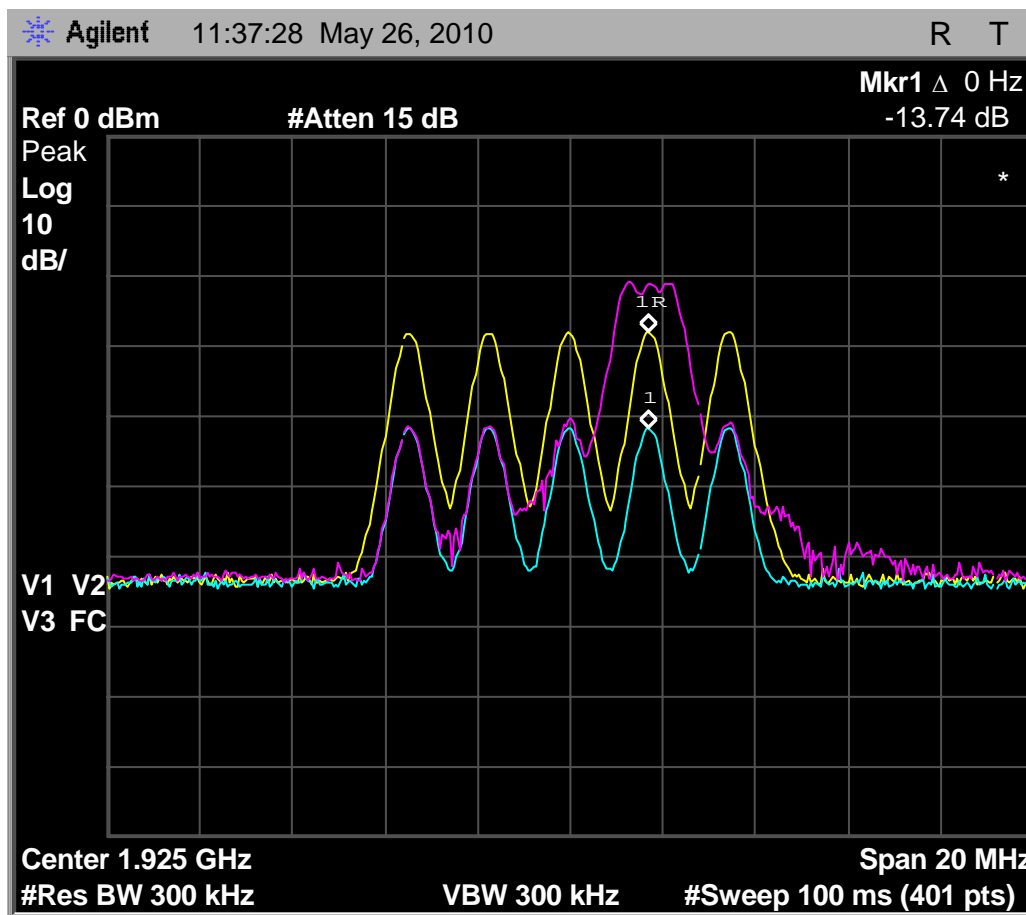
Fig. 92 - Emissions and interference profile spectrum, headset EUT, test 7.3.2.
