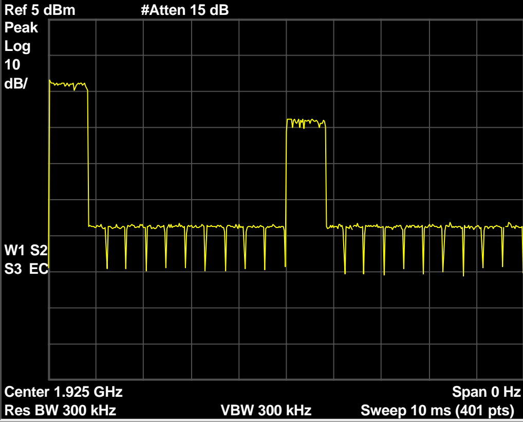
Fig. 84 – Interference profile for the headset EUT is above the threshold of -75.6\text{dBm} ( T_L + U_M ) WITH an open time slot pair, to ensure the test set up interference synchronization are working correctly, and that the link deferral tests above are valid. Slot 0 and slot 1 are interference free. A traffic link was established validating the test set up.
