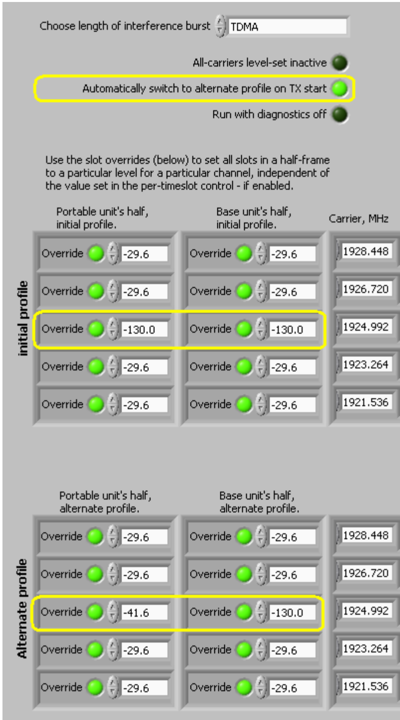
Fig. 58 - Multi-carrier interference generator configured according to the requirements for testing the headset EUT per 8.2.1(a), with automatic switching to the alternate interference profile enabled.
