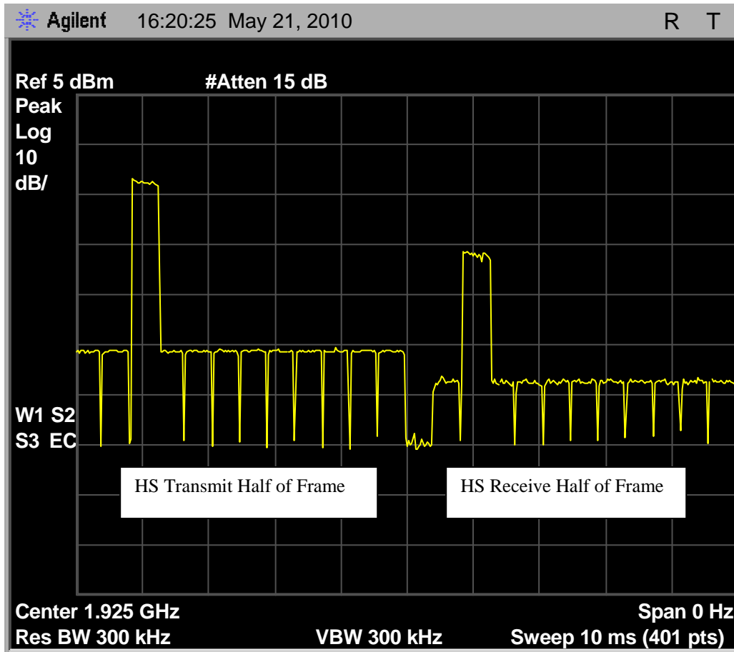
Fig. 70 – Headset EUT selects slot 2 pair which has the lowest maximum level of interference
