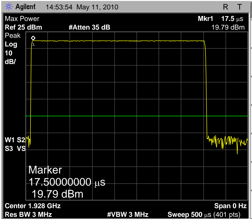
Fig. 9 - Headset EUT transmit power received by spectrum analyzer configured according to the requirements of clause 6.1.2 of C63.17-2006, high carrier. Maximum observed transmit power is 19.79dBm.
