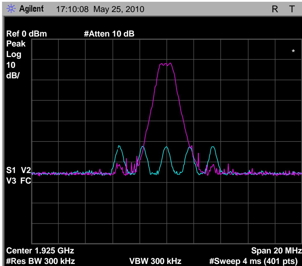
Fig. 78 - Transmit spectrum of 50uS interference pulses, with headset EUT no longer deferring with interference pulses of level T_L - U_M
