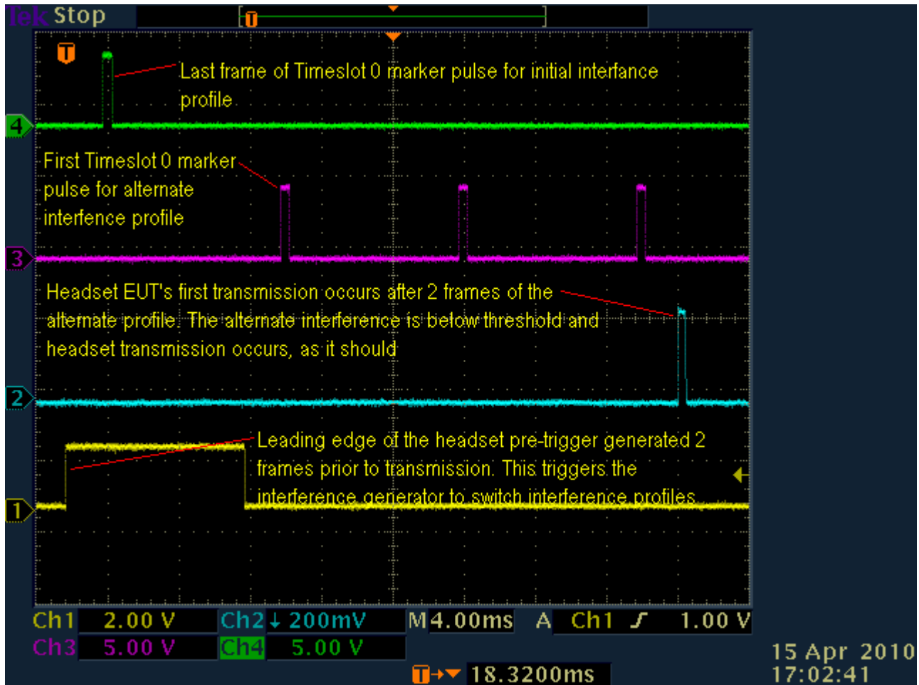
Fig. 47 - Example oscilloscope screenshot showing transition from initial to alternate interference profile in the frame before headset EUT initiation of transmission of the communications channel; for this example the alternate interference profile is configured to meet the access criteria.
