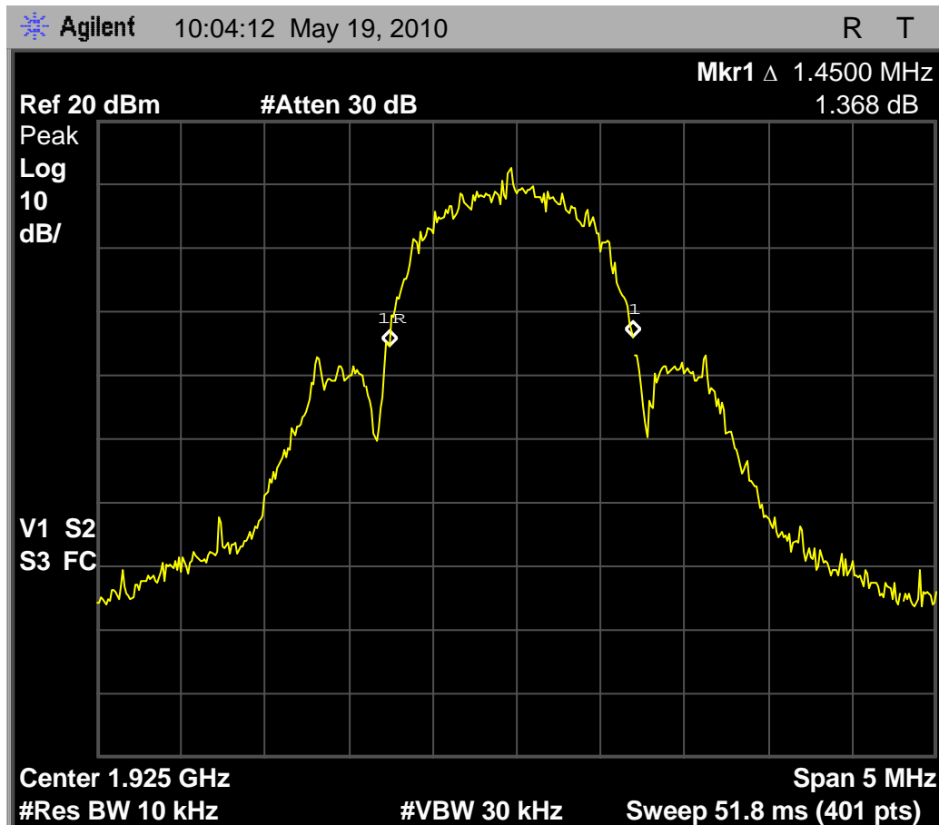
Fig. 74 - headset EUT in WBM, 1.45MHz emissions bandwidth on mid carrier; same results as in normal mode operation; no difference WBM vs. normal mode.
