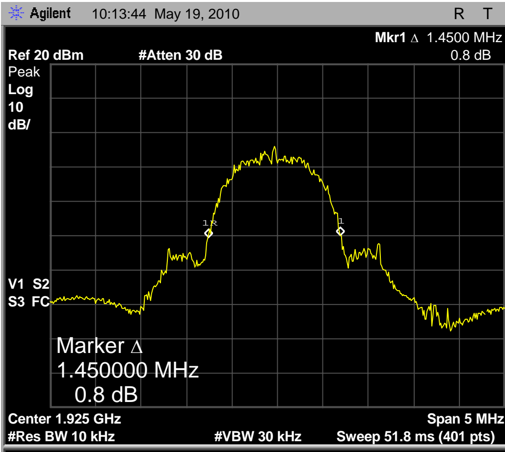
Fig. 87 - Headset EUT in WBM, 1.45MHz emissions bandwidth on mid carrier vs. 1.45MHz in normal mode high power.
