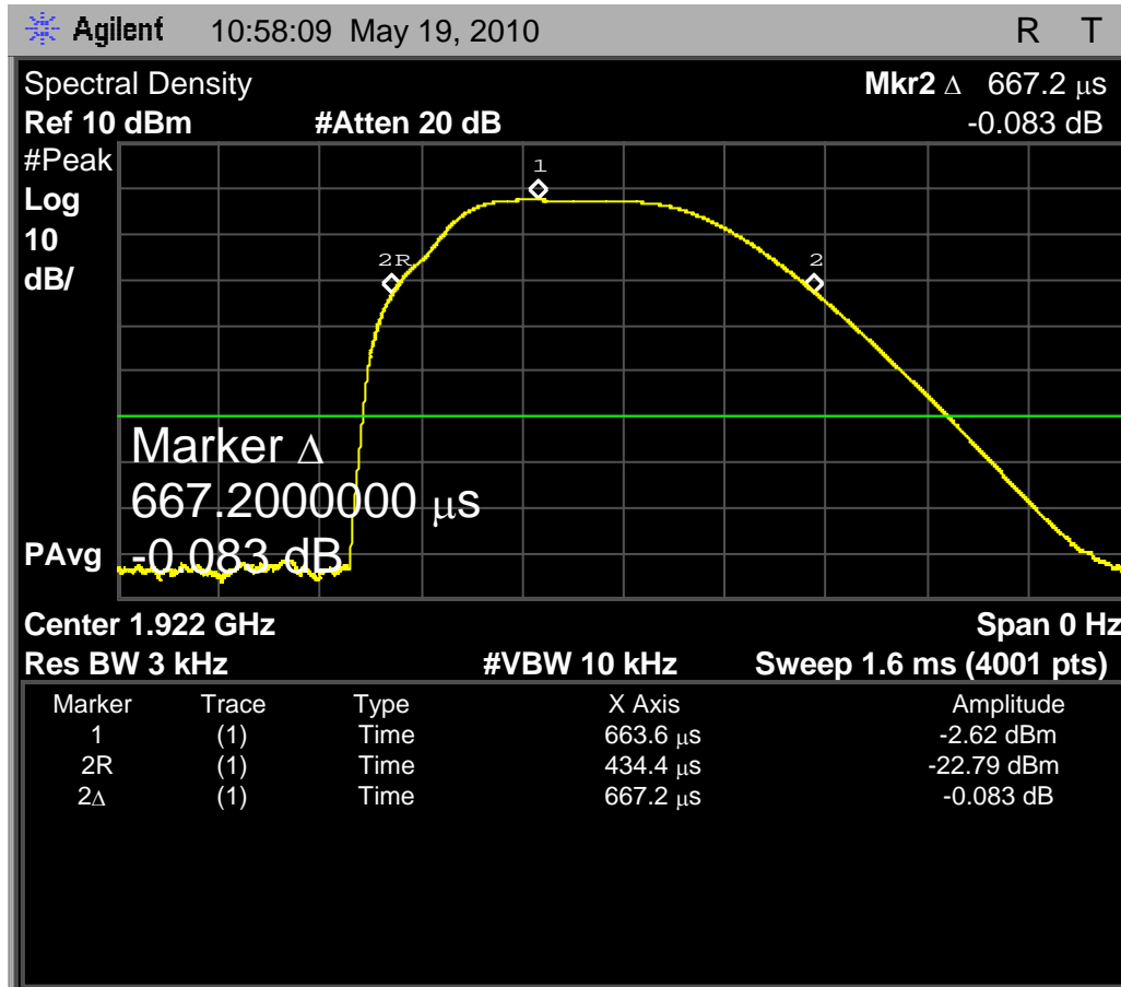
Fig. 13 – Zero-span sweep for headset EUT, low carrier, for 3kHz maximum power spectral density. The peak level is at -2.62dBm, and the interval between samples at the -20dB points is 667.2us.
