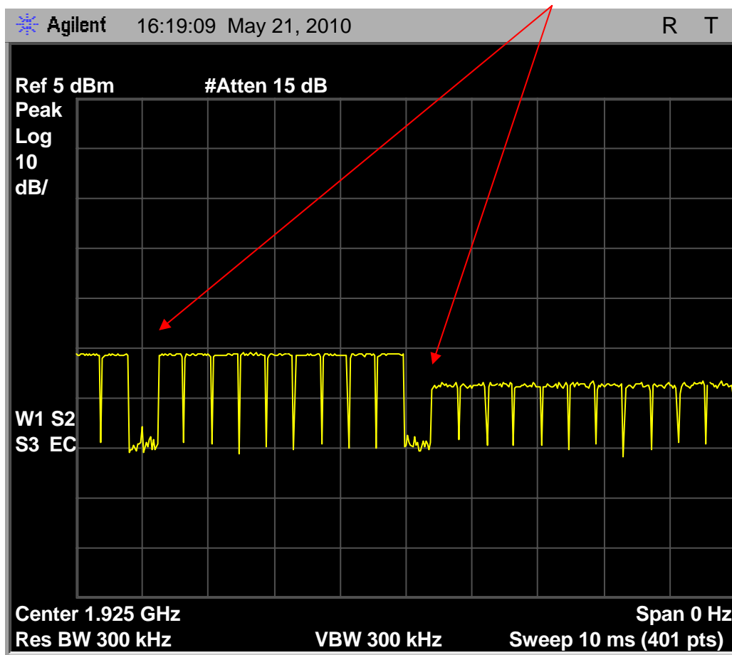
Fig. 69 – Spectrum analyzer screen capture of the interference pattern prior to headset link with companions Base (alternate interference profile from PXI screen capture of Fig 73)
