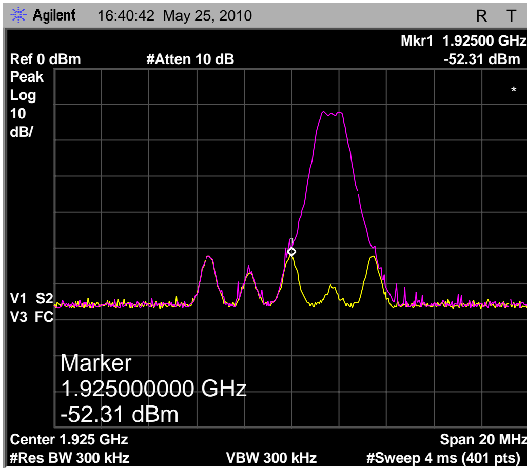
Fig. 77 - Emissions and interference profile spectrum, headset EUT, test 7.3.3(c).
