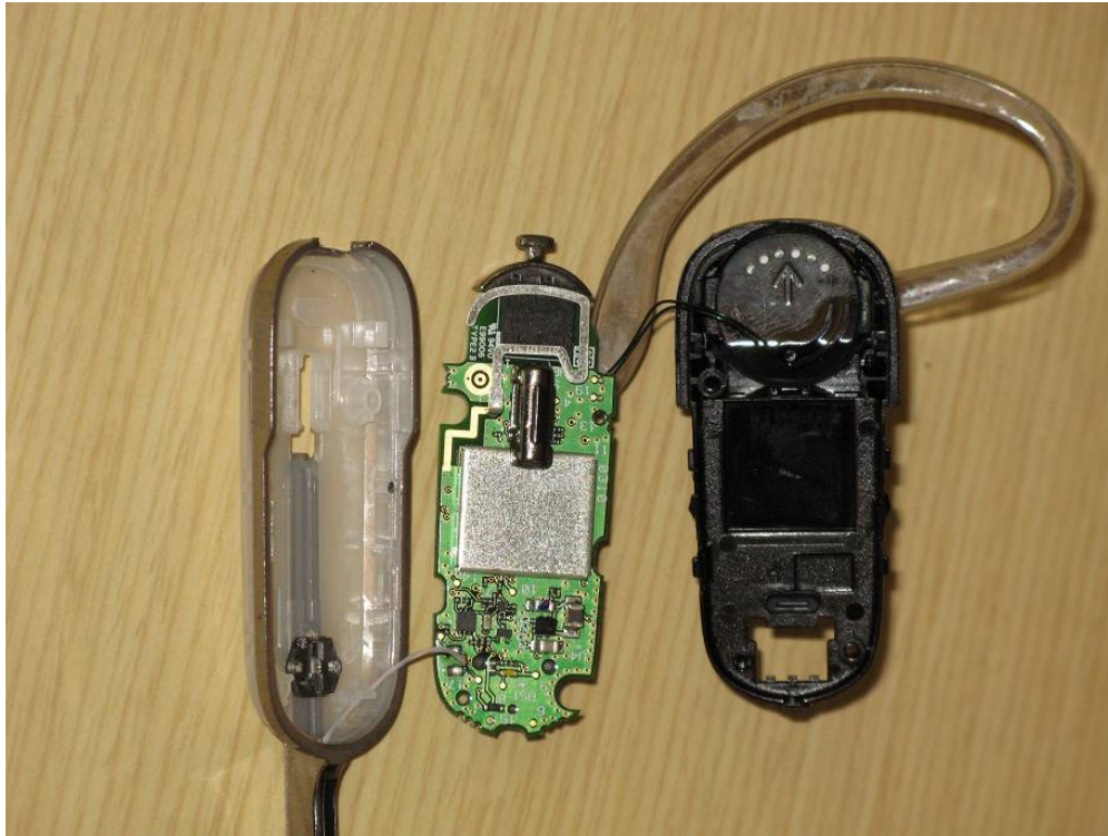
PCB Installed
