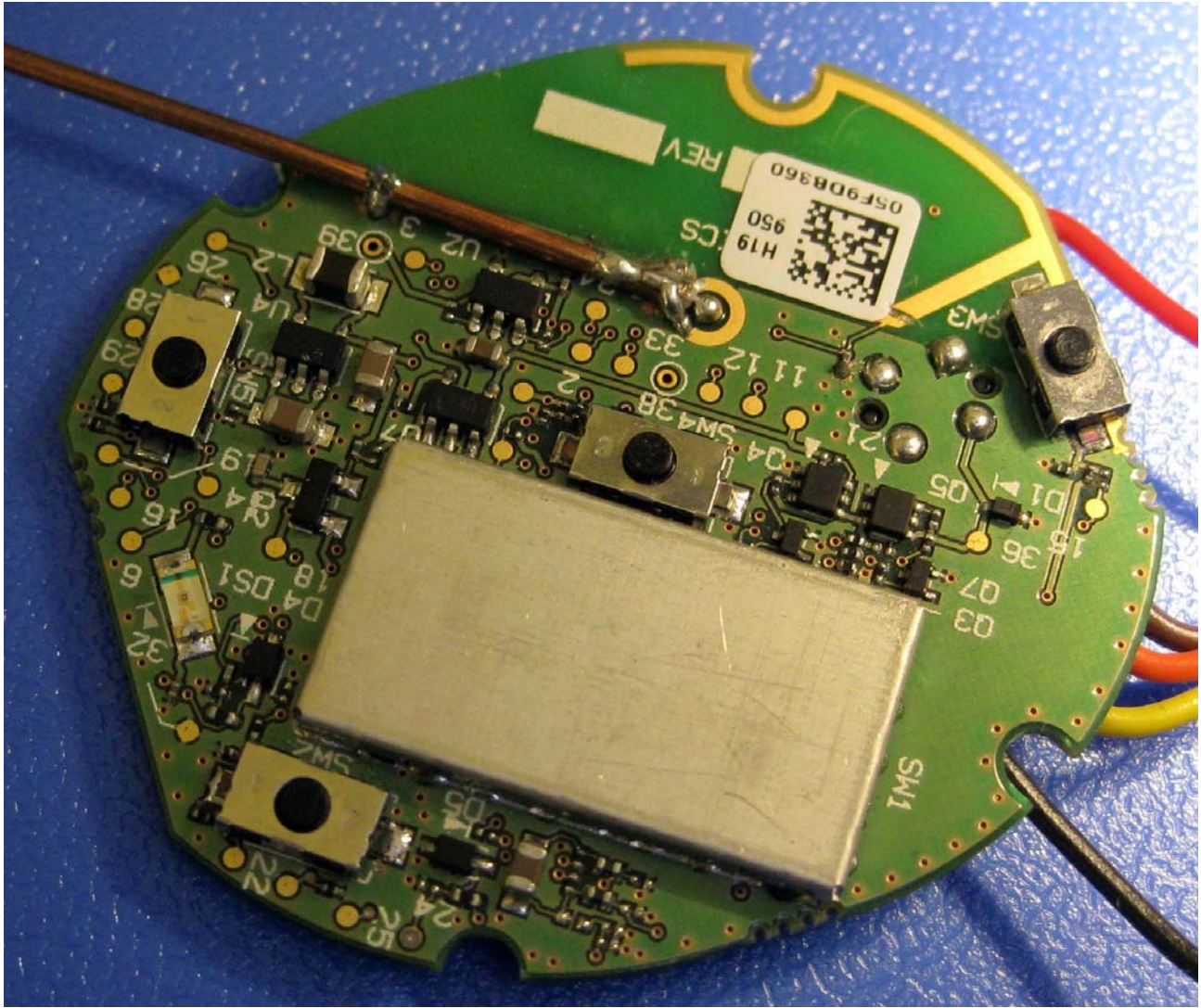
Fig. 7 – Detail of the attachment of the RF connection for conducted measurements.
