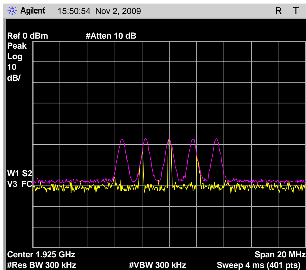
Fig. 82 - Transmit spectrum of 35uS interference pulses in each timeslot for each carrier, with headset EUT deferring due to interference pulses of T_L + U_M + 6\text{dB} .
