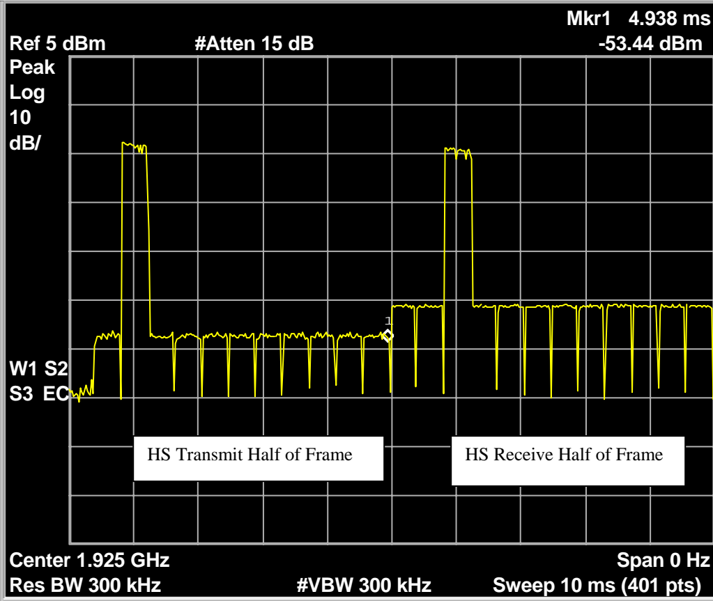
Fig. 70 – Headset EUT selects slot 2 pair which has the lowest maximum level of interference
