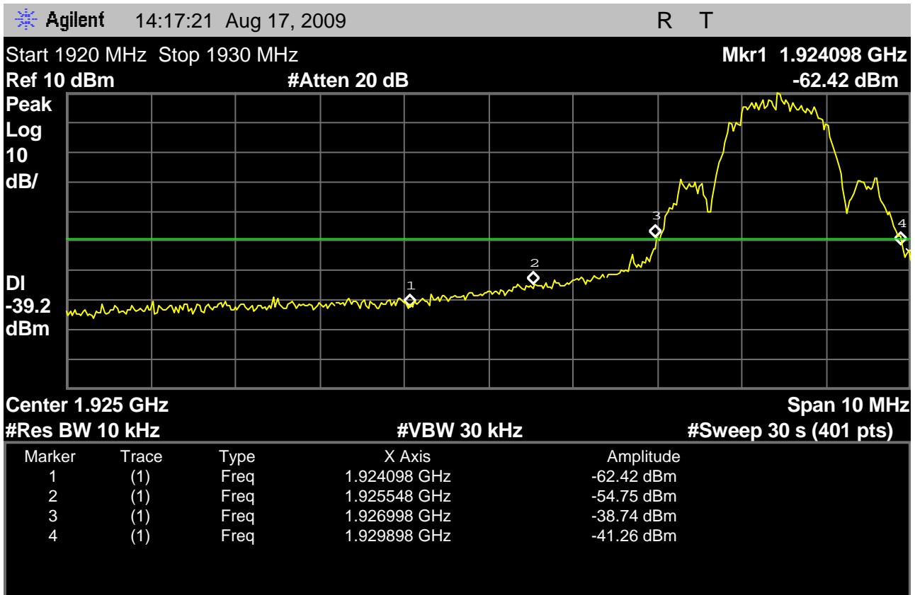
Fig. 22 - Spectrum analyzer screenshot for transmit emissions showing inband unwanted emissions with the headset EUT transmitter at the highest carrier, 1928.448MHz, according to the requirements of 6.1.6.1.
