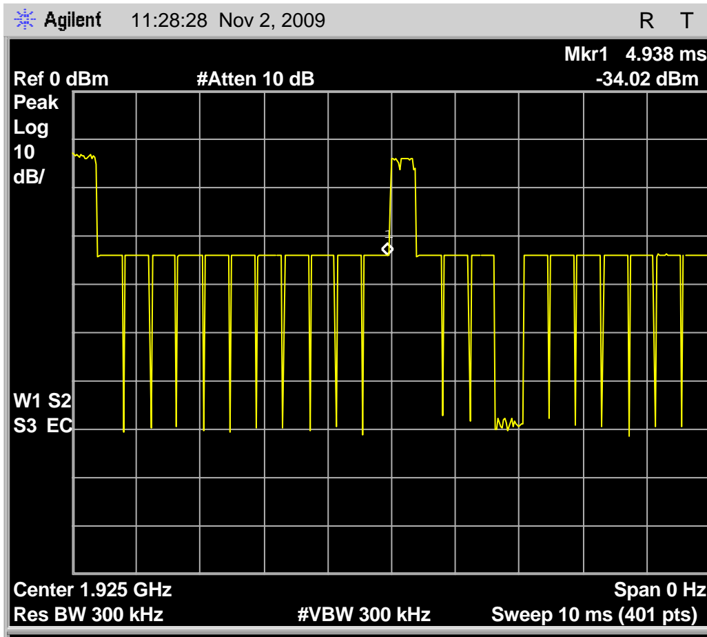
Fig. 73 – Interference profile for the Headset EUT that is above the threshold of -55.6\text{dBm} (T_U + U_M) WITH an open slot pair to demonstrate a link was possible for the test set up when 8.3.2 g) was performed.
