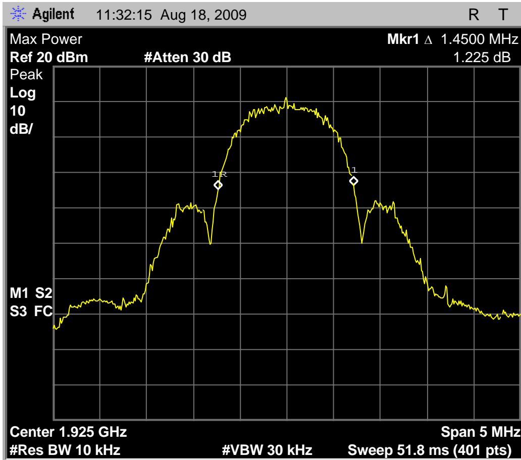
Fig. 76 - headset EUT in WBM, 1.45MHz emissions bandwidth on mid carrier; same results as in normal mode operation; no difference WBM vs normal mode.
