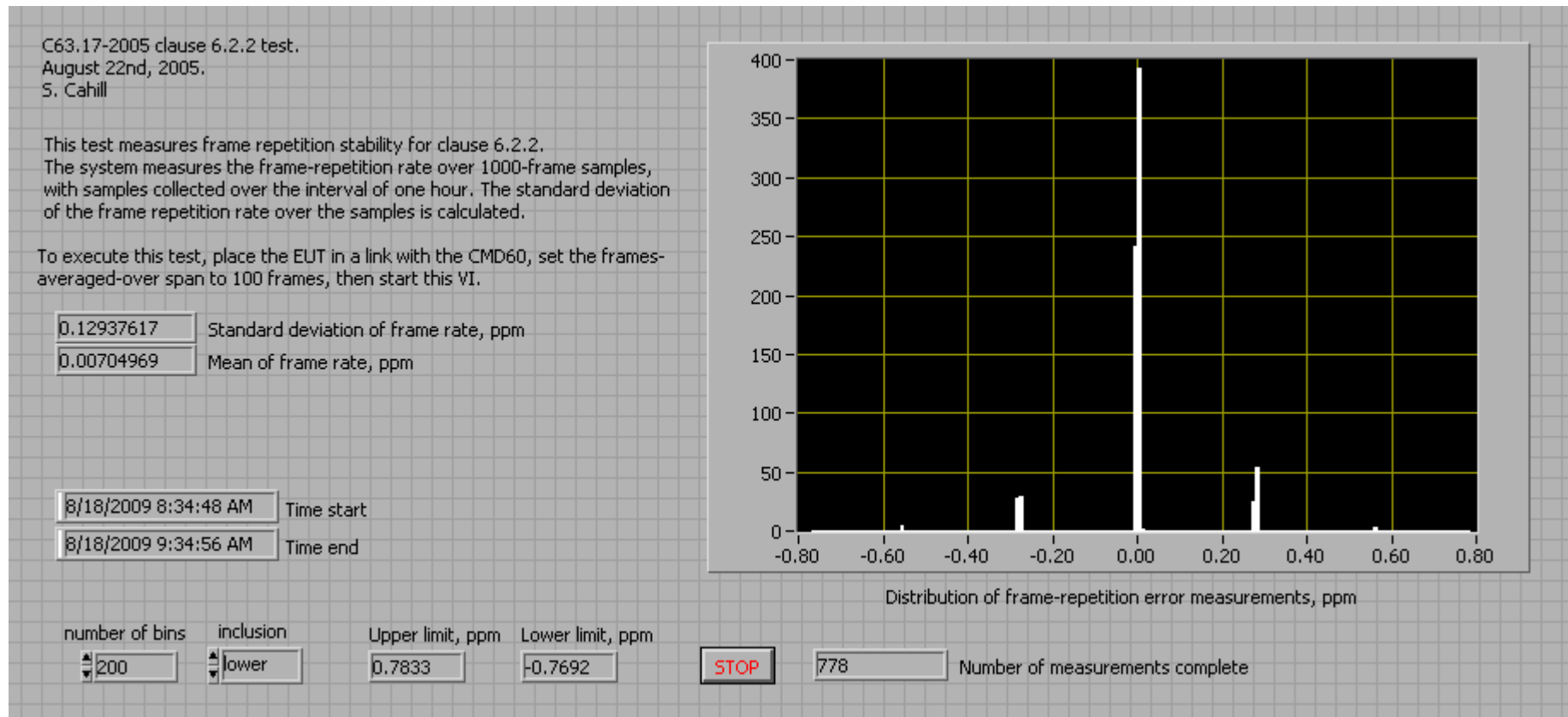
Fig. 42 - Test of headset EUT according to the conditions of clause 6.2.2 for frame repetition rate stability
