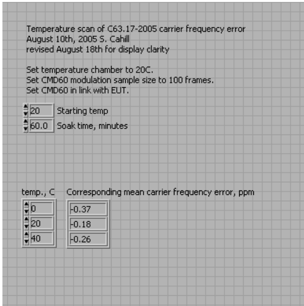
Fig. 41 - Measured mean carrier frequency, headset EUT , at 0C, +20C, +40C.
