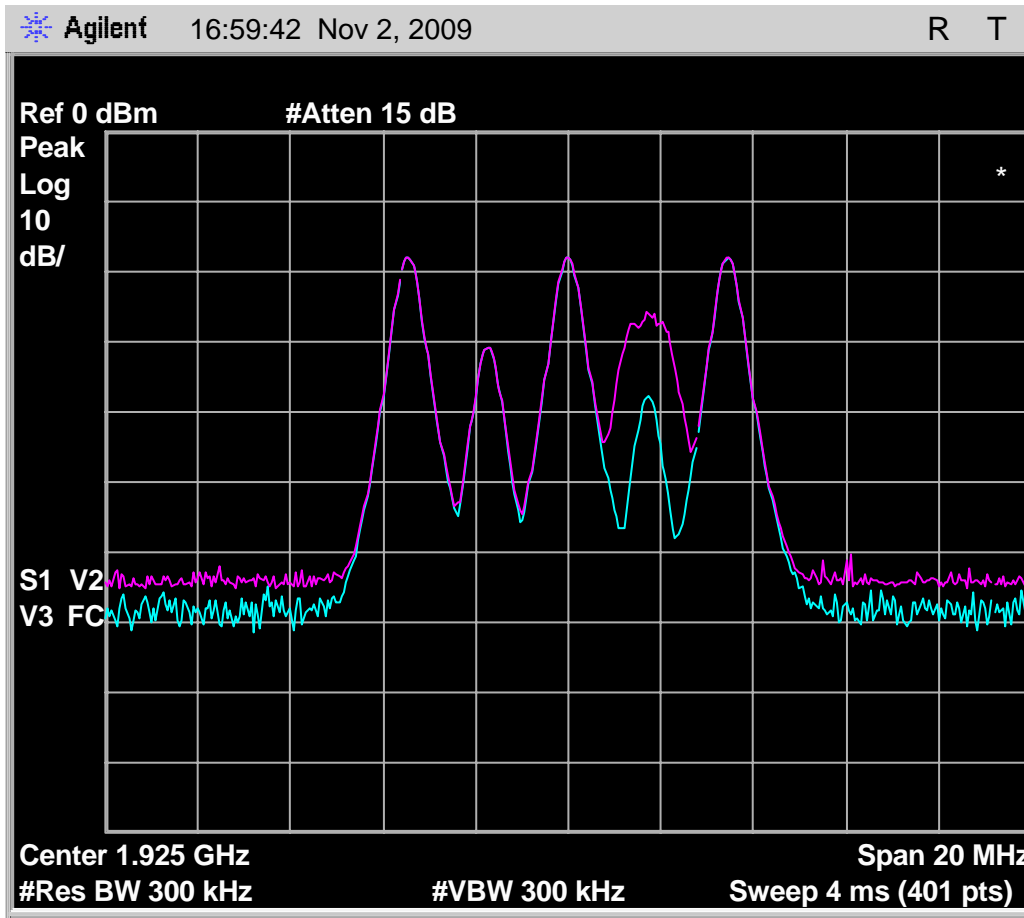
Fig. 96 - Emissions and interference profile spectrum, headset EUT, test 7.3.3(c).
