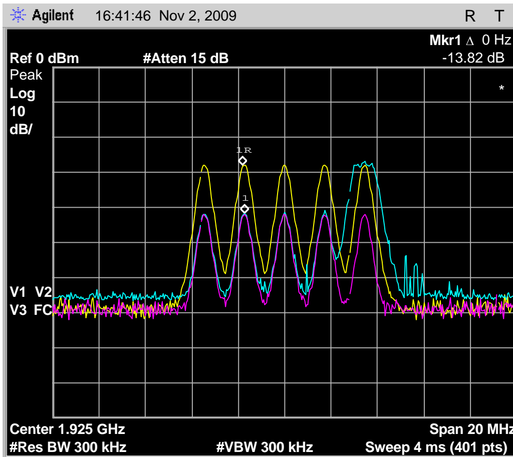
Fig. 93 - Emissions and interference profile spectrum, headset EUT, test 7.3.1 in low power WBM.
