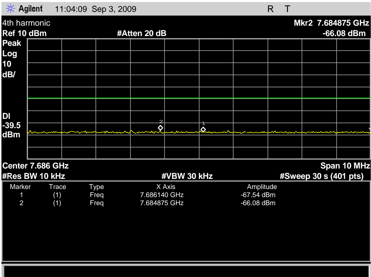
Fig. 30 – headset EUT out-of-band emissions in the region around the 4th harmonic, with the headset EUT transmitting on the lowest carrier, 1921.536MHz.
