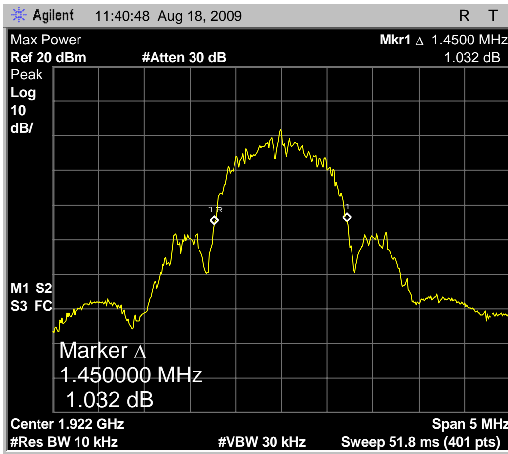
Fig. 88 - Headset EUT in WBM, 1.45MHz emissions bandwidth on low carrier vs. 1.45MHz in normal mode high power operation.
