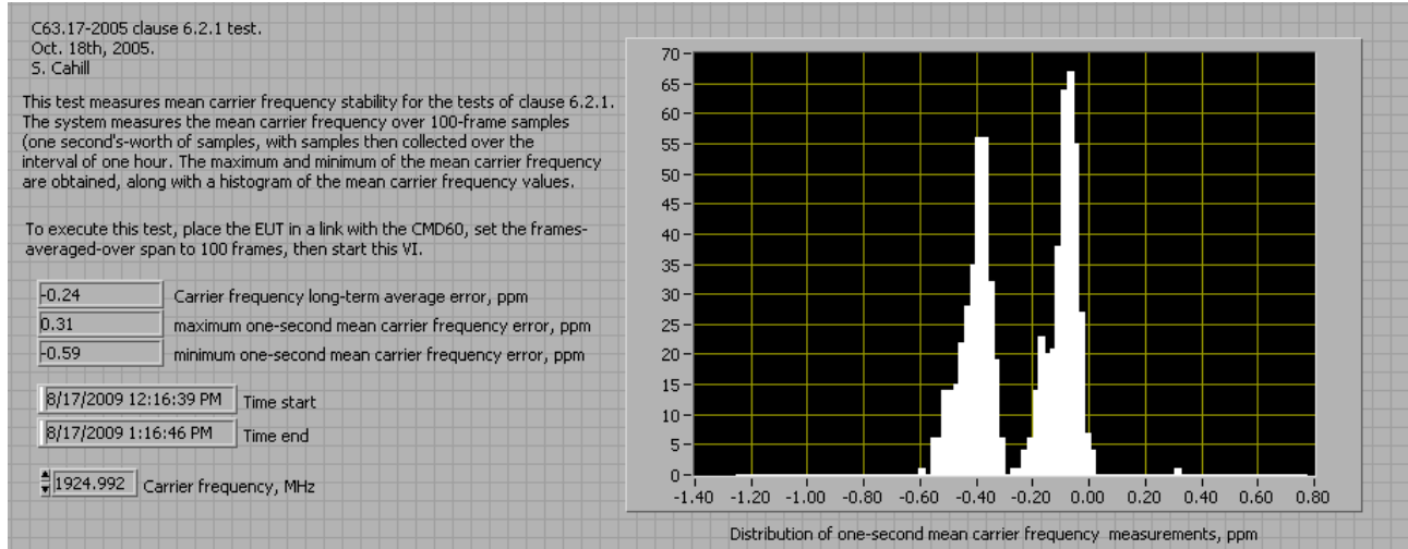
Fig. 40 - Measured one-second mean carrier frequency, headset EUT, and observed maximum, average value and observed minimum of the mean carrier frequency.
