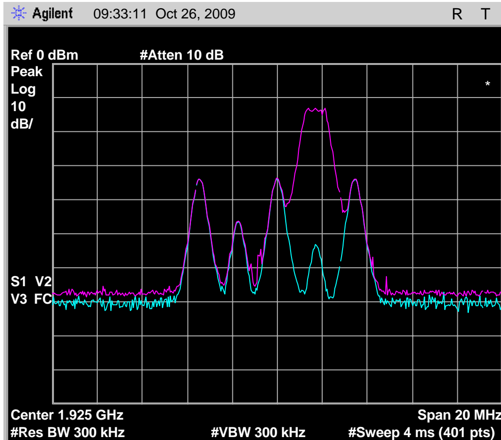
Fig. 46 - Emissions and interference profile spectrum, headset EUT, test 7.3.3(c).
