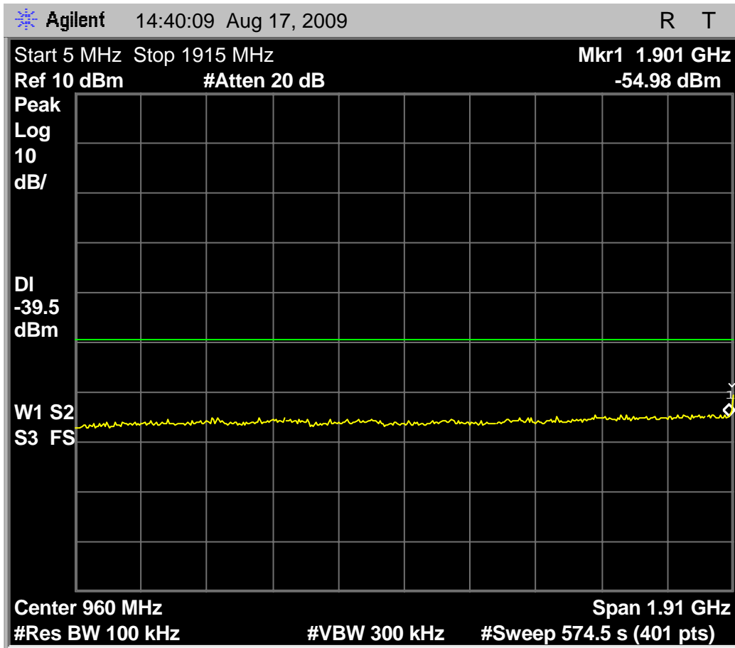
Fig. 32 – headset EUT out-of-band emissions showing the region from 5MHz to 1915MHz, with the transmitter using the highest carrier, 1928.448MHz.
