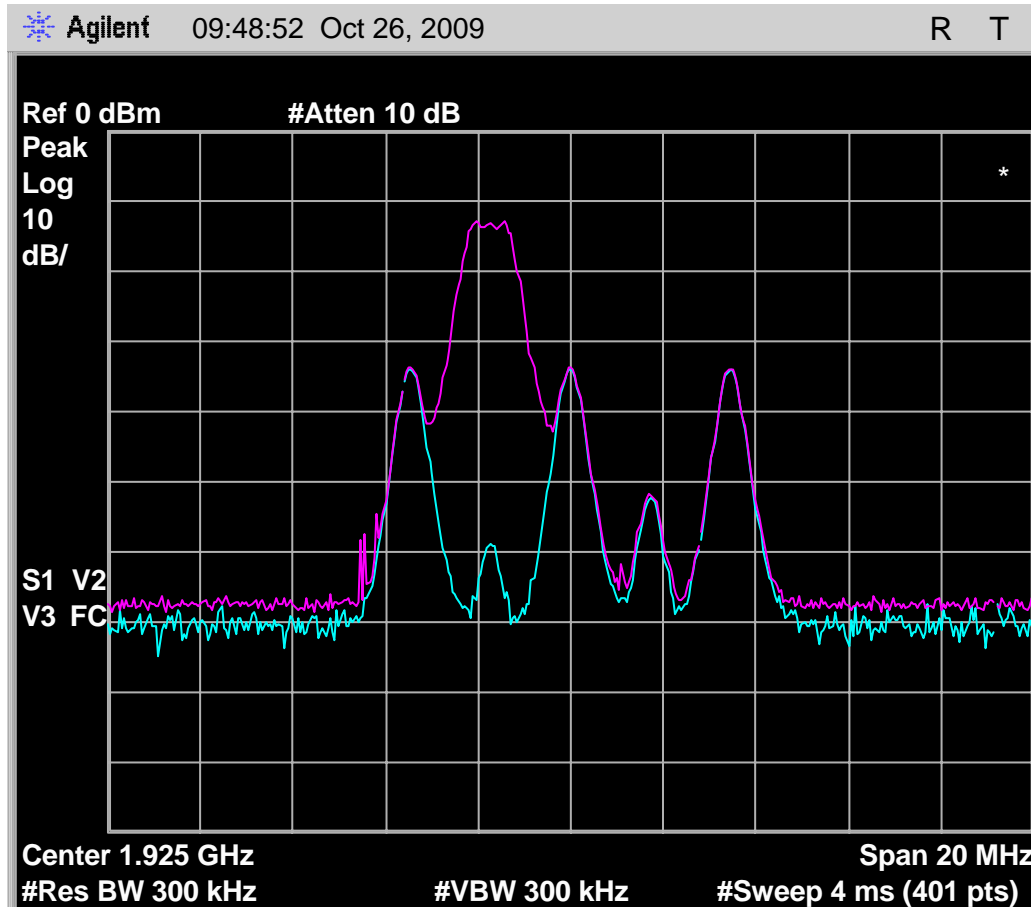
Fig. 47 - Emissions and interference profile spectrum, headset EUT, test 7.3.3(d).
