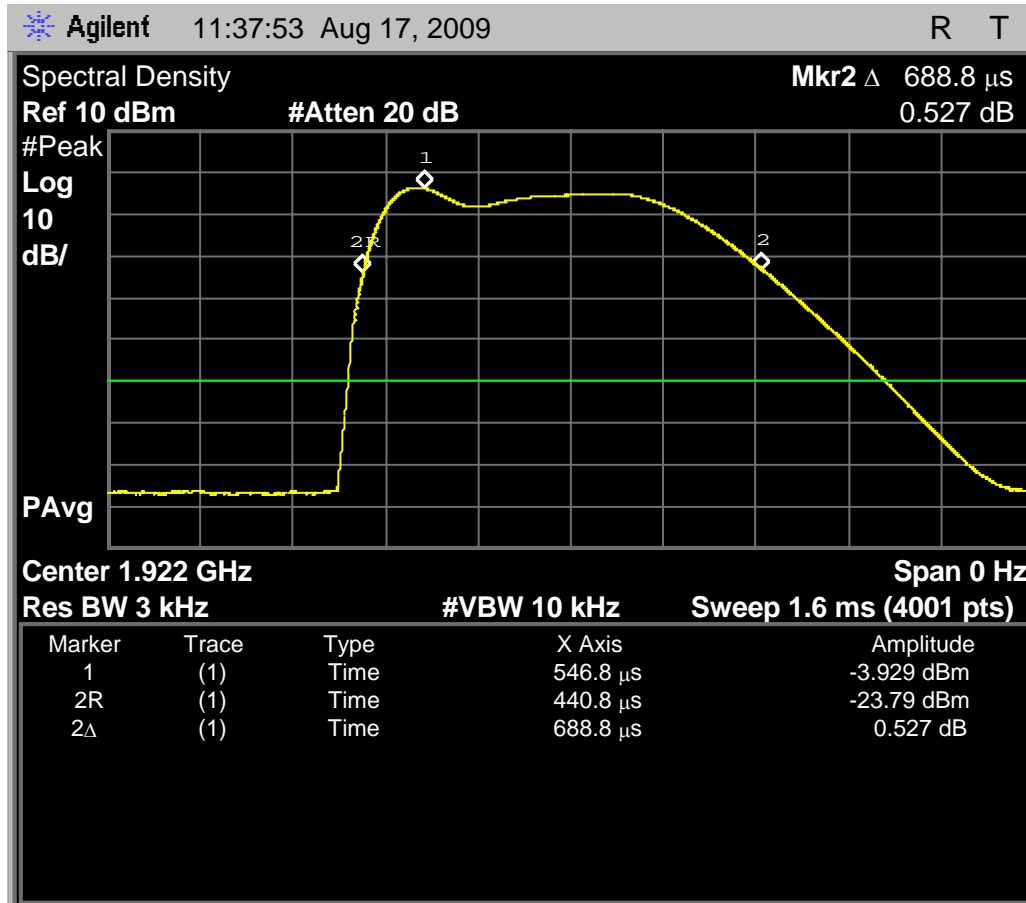
Fig. 14 – Zero-span sweep for headset EUT, low carrier, for 3kHz maximum power spectral density. The peak level is at -3.93dBm, and the interval between samples at the -20dB points is 688.8us.
