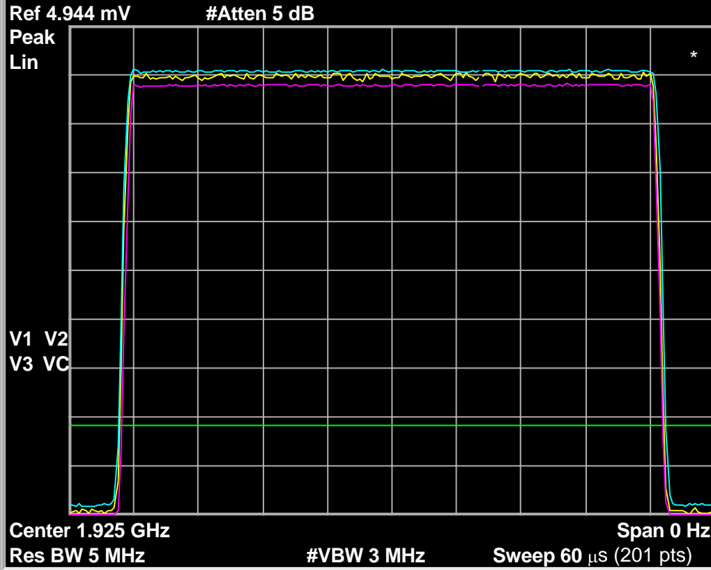
Fig. 54 – 50uS interference pulse for 7.5(c), duration and amplitude variation over the duration of the 50 uS pulse and over multiple pulses. Spectrum analyzer is set to linear response.
