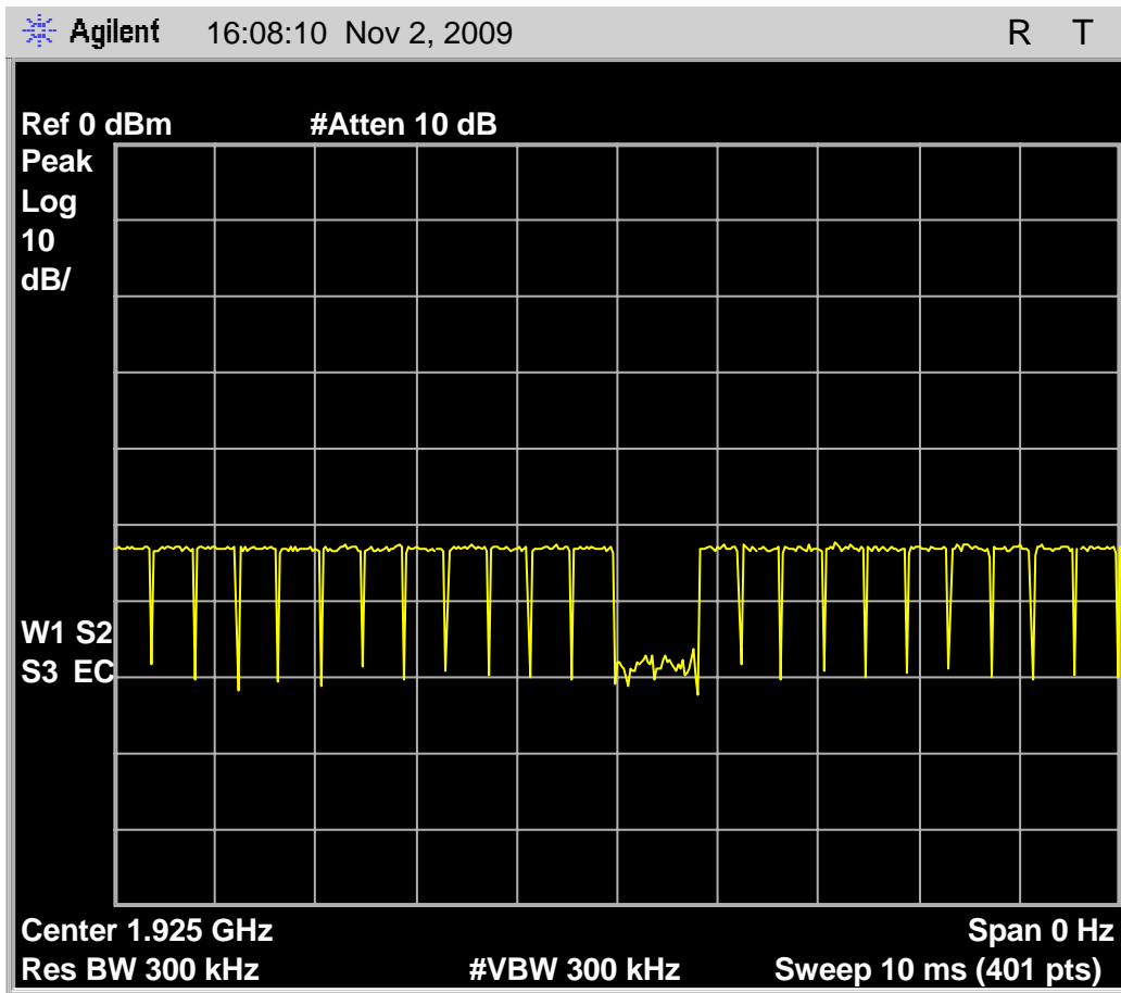
Fig. 84 – Interference profile for the Headset EUT that is above the threshold of -75.6\text{dBm} ( T_L + U_M ) without an open time slot pair. Slots that are interference free are headset receive slots 0 and 1 (slot 12 and 13).
