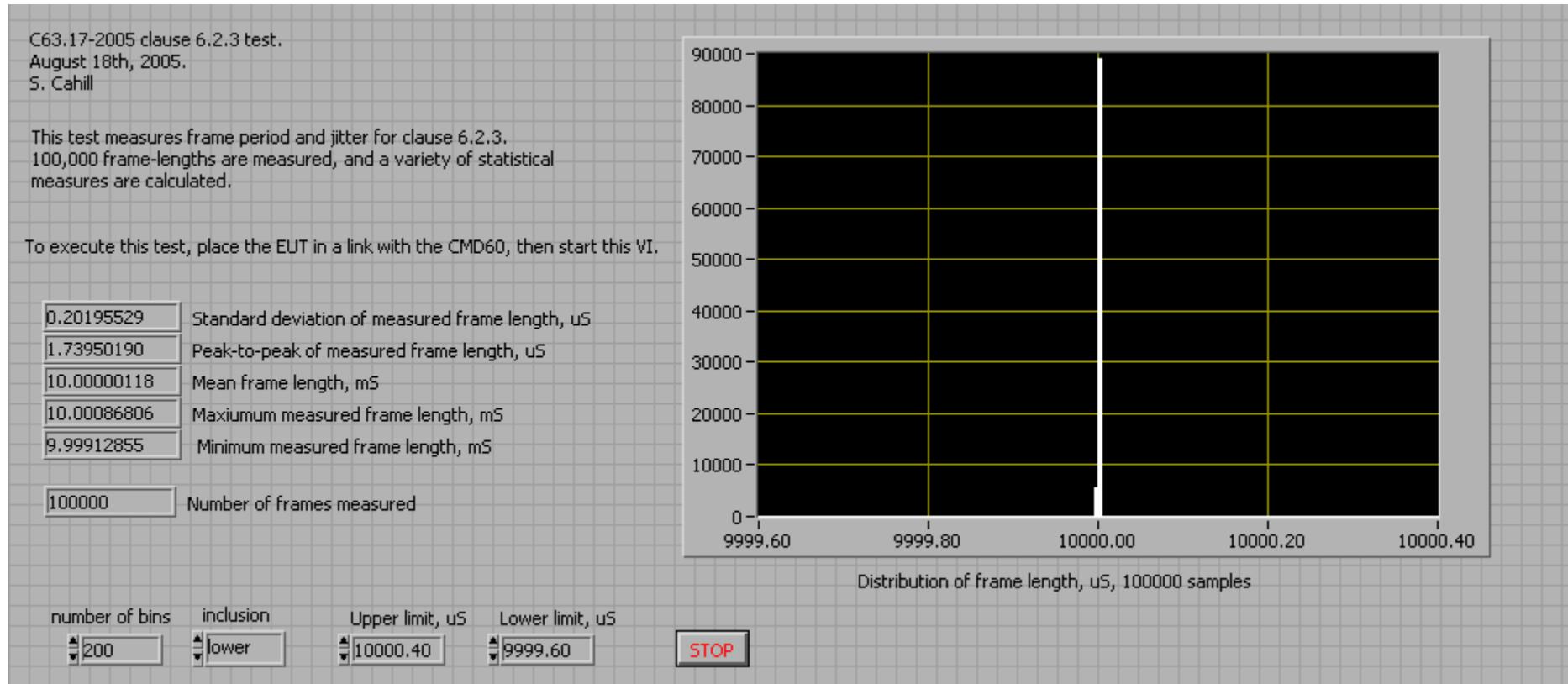
Fig. 43 - Test of headset EUT for frame period and jitter, according to the requirements of clause 6.2.3.
