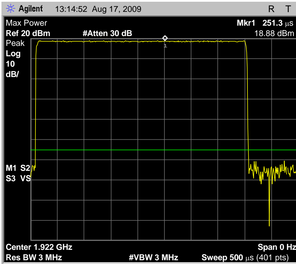
Fig. 8 - Headset EUT transmit power received by spectrum analyzer configured according to the requirements of clause 6.1.2 of C63.17-2006, low carrier. Maximum observed transmit power is 18.88 dBm.
