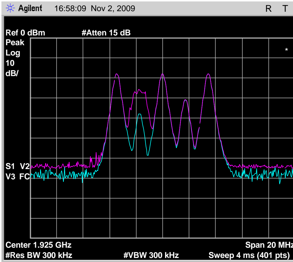
Fig. 95 - Emissions and interference profile spectrum, headset EUT, test 7.3.3(b).
