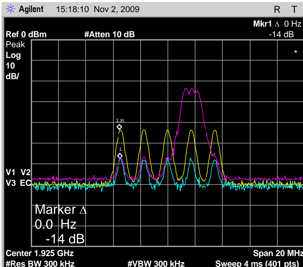
Fig. 77 - Emissions and interference profile spectrum, headset EUT, test 7.3.1 in WBM.
