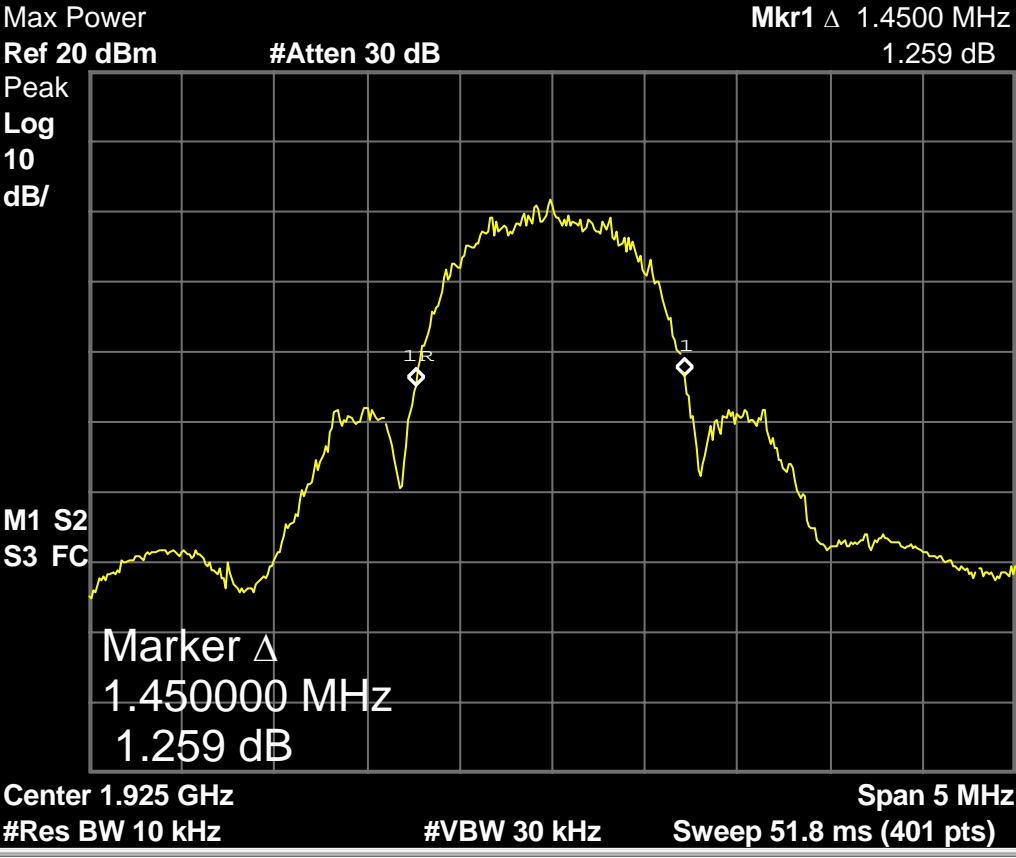
Fig. 89 - Headset EUT in WBM, 1.45MHz emissions bandwidth on mid carrier vs. 1.45MHz in normal mode high power.
