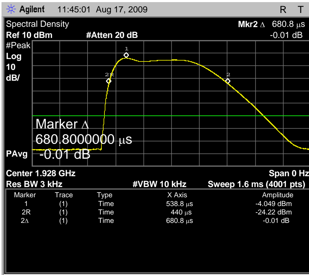
Fig. 18 – Zero-span sweep for headset EUT, high carrier, for 3kHz maximum power spectral density. The peak level is at -4.049dBm, and the interval between samples at the -20dB points is 680.8us.
