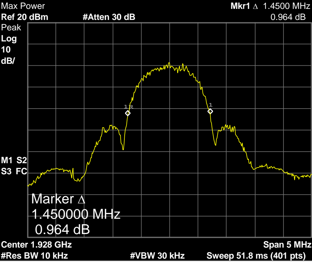
Fig. 90 - Headset EUT in WBM, 1.45MHz emissions bandwidth on high carrier vs. 1.44MHz in normal mode high power.
