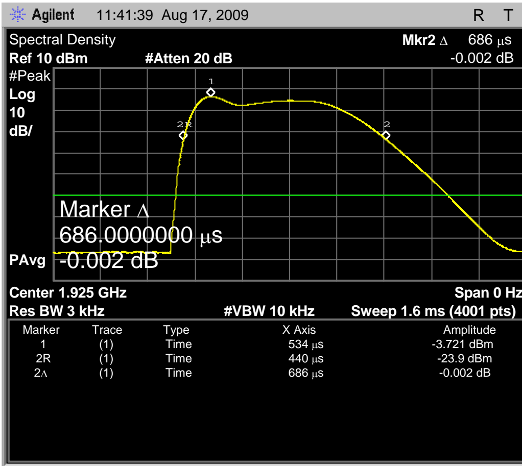
Fig. 16 – Zero-span sweep for headset EUT, middle carrier, for 3kHz maximum power spectral density. The peak level is at -3.721Bm, and the interval between samples at the -20dB points is 686.0us.
