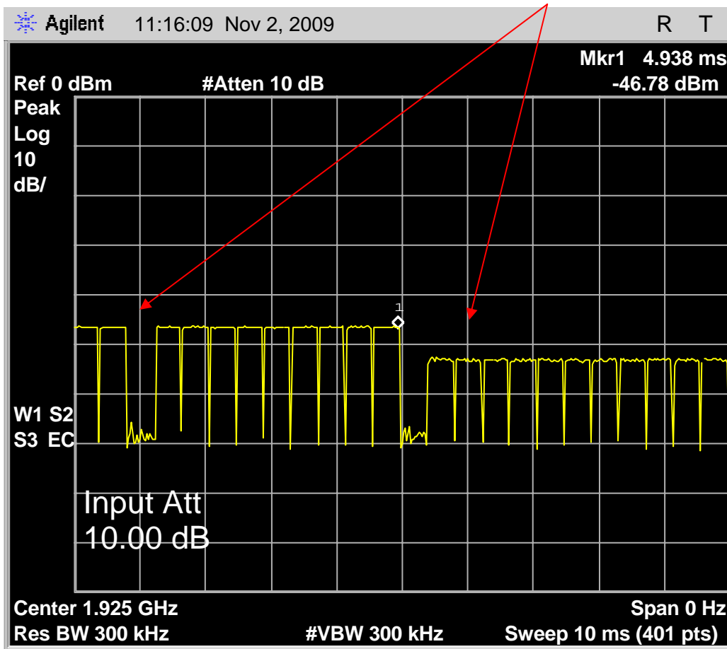
Fig. 71 – Spectrum analyzer screen capture of the interference pattern prior to headset link with companions Base (alternate interference profile from PXI screen capture of Fig 73)
