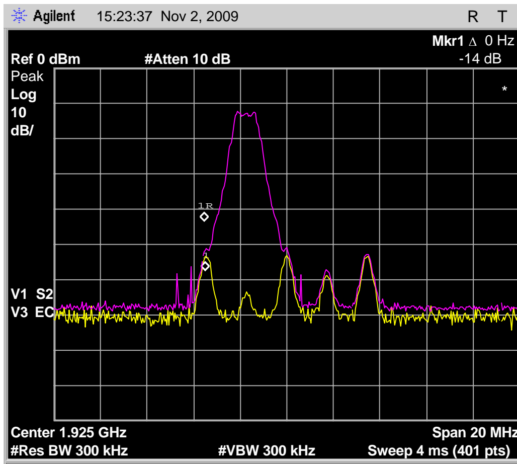
Fig. 78 - Emissions and interference profile spectrum, headset EUT, test 7.3.3(b).
