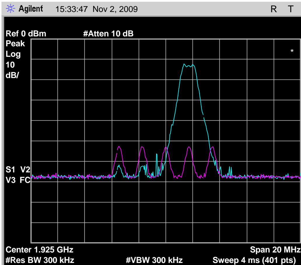
Fig. 80 - Transmit spectrum of 50uS interference pulses, with headset EUT no longer deferring with interference pulses of level T_L - U_M
