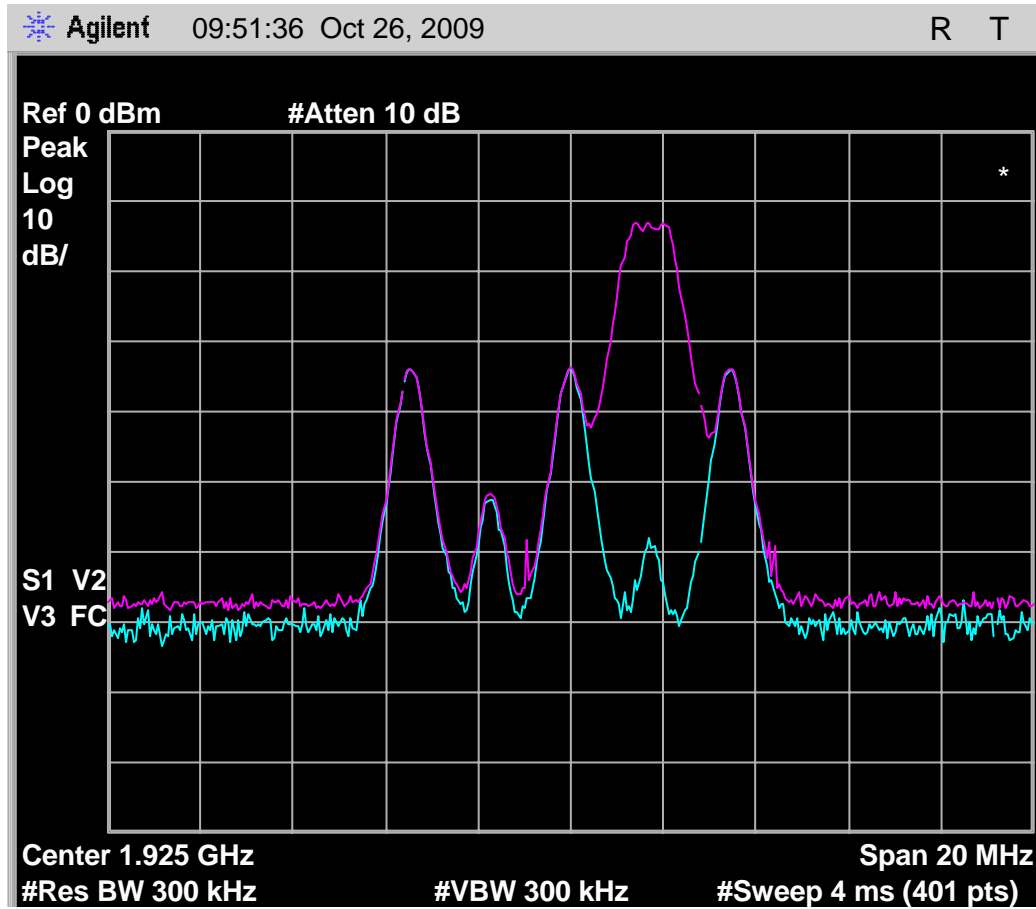
Fig. 48 - Emissions and interference profile spectrum, headset EUT, test 7.3.3(e).
