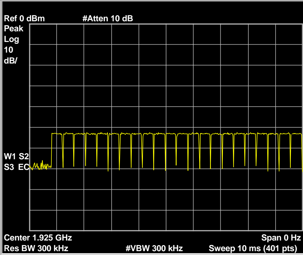
Fig. 86 – Interference profile for the Headset EUT that is above the threshold of -75.6\text{dBm} ( T_L + U_M ) without an open time slot pair. Headset EUT transmit slots that are interference free are 0 and 1 (one WBM slot).
