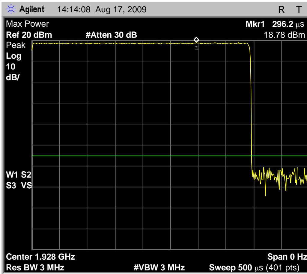
Fig. 10 - Headset EUT transmit power received by spectrum analyzer configured according to the requirements of clause 6.1.2 of C63.17-2006, high carrier. Maximum observed transmit power is 18.78dBm.
