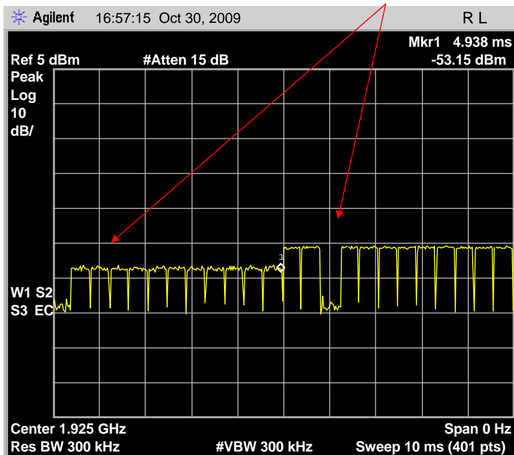
Fig. 69 – Spectrum analyzer screen capture of the interference pattern prior to headset link with companions Base (initial interference profile)
