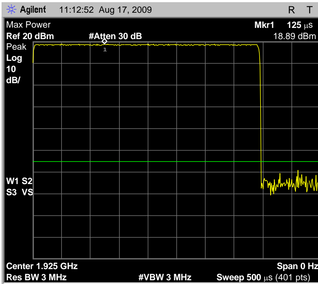
Fig. 9 - Headset EUT transmit power received by spectrum analyzer configured according to the requirements of clause 6.1.2 of C63.17-2006, mid carrier. Maximum observed transmit power is 18.89dBm
