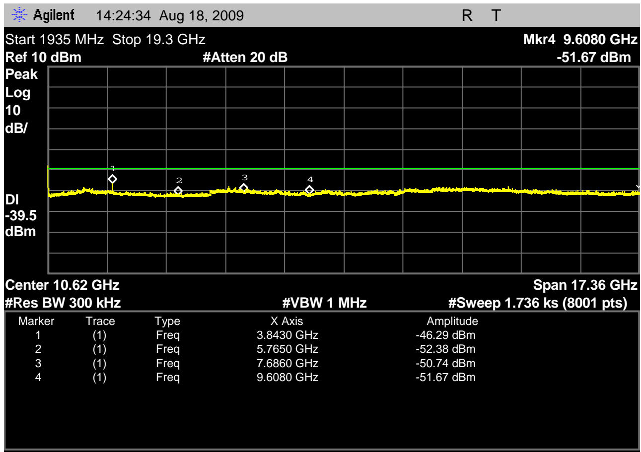
Fig. 91 - Headset EUT in minimum power WBM on low carrier, 2 nd harmonic passes even with 10x the resolution bandwidth setting, all harmonics below maximum power mode, see section 6.1 of main report.
