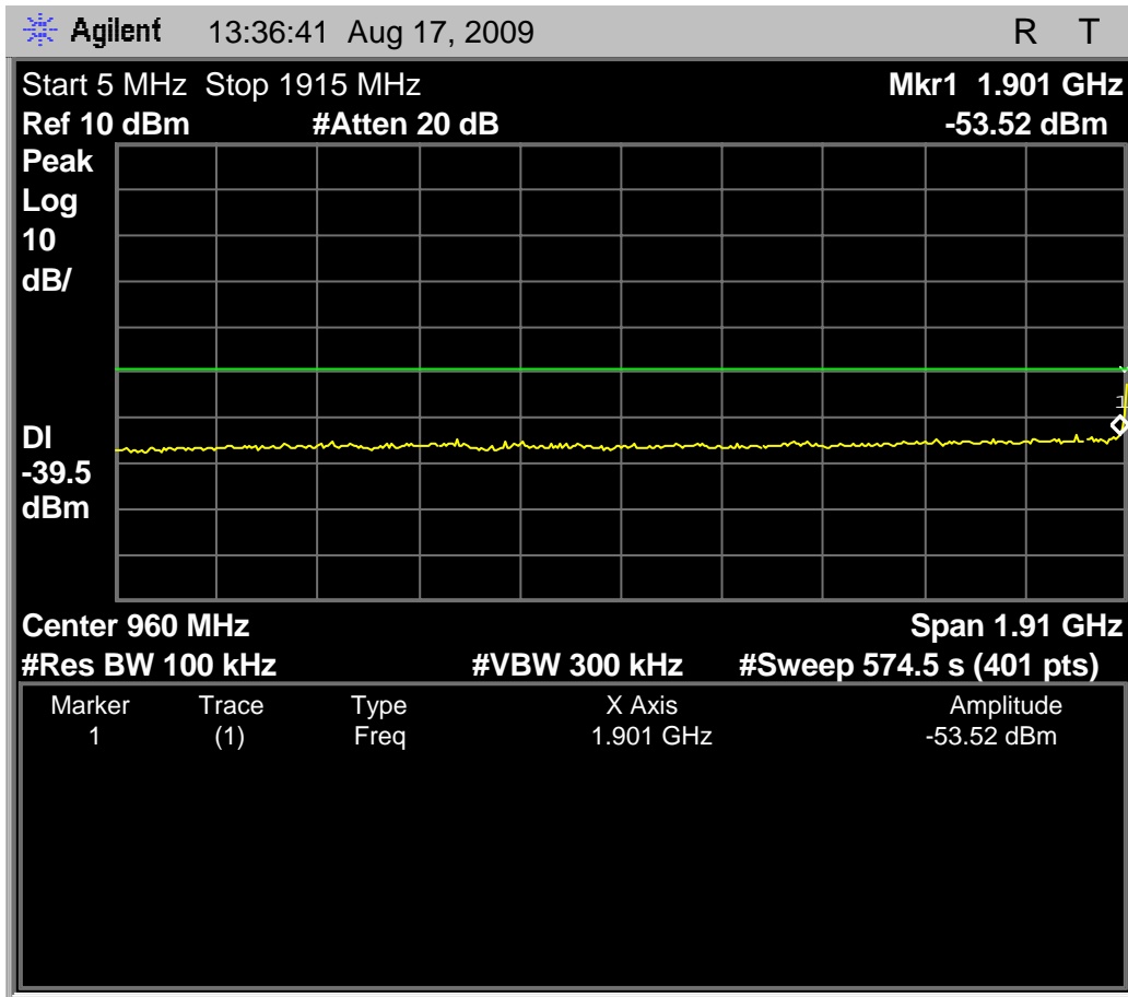
Fig. 24 – headset EUT out-of-band emissions showing the region from 5MHz to 1915MHz, with the transmitter using the lowest carrier, 1921.536MHz.
