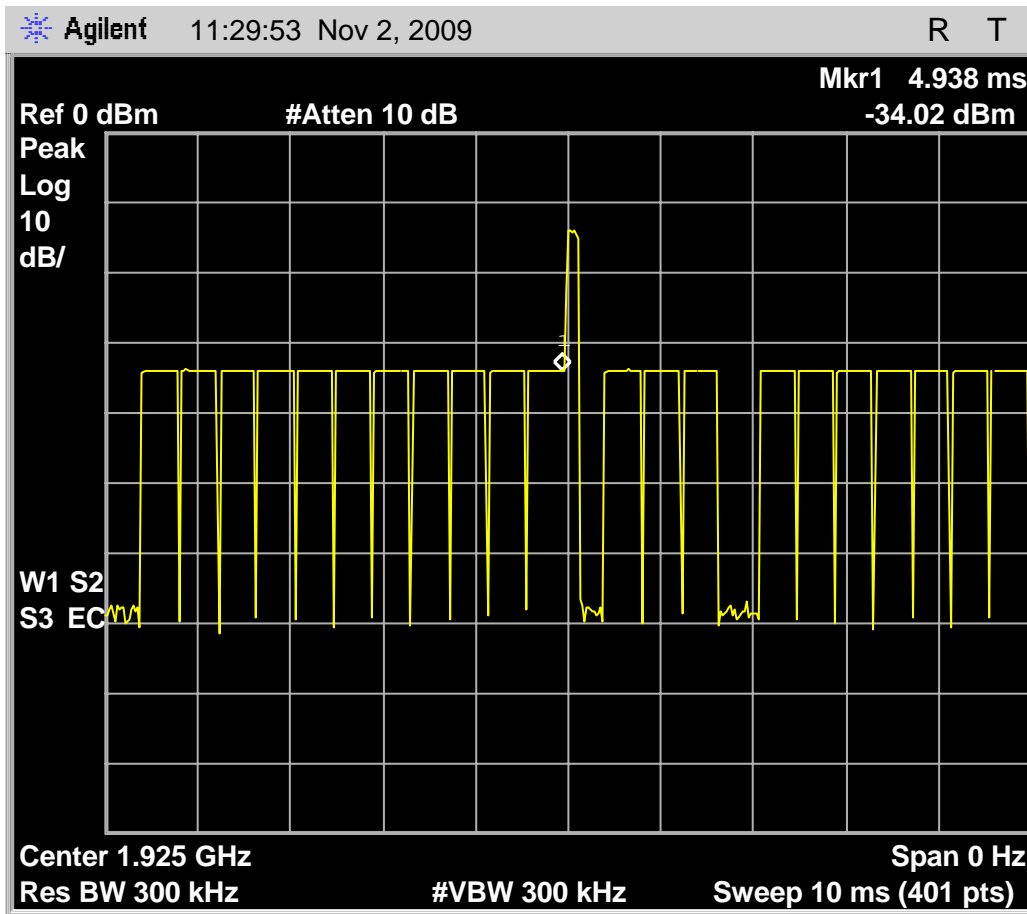
Fig. 74 – Interference profile for the Headset EUT that is above the threshold of -55.6\text{dBm} ( TU + UM ) without an open time slot pair. Slots that are opened are headset transmit slot 0 and headset receive slot 4 (slot 16). Note an additional time slot was opened to provide a place for the Base beacon of the companion device. If the base beacon was to occupy slot 0 or slot 16 a link could not be established and the test would pass but not be valid. Another option would be to force the Base to another carrier, but could not be monitored at the same time as the interference profile of interest.
