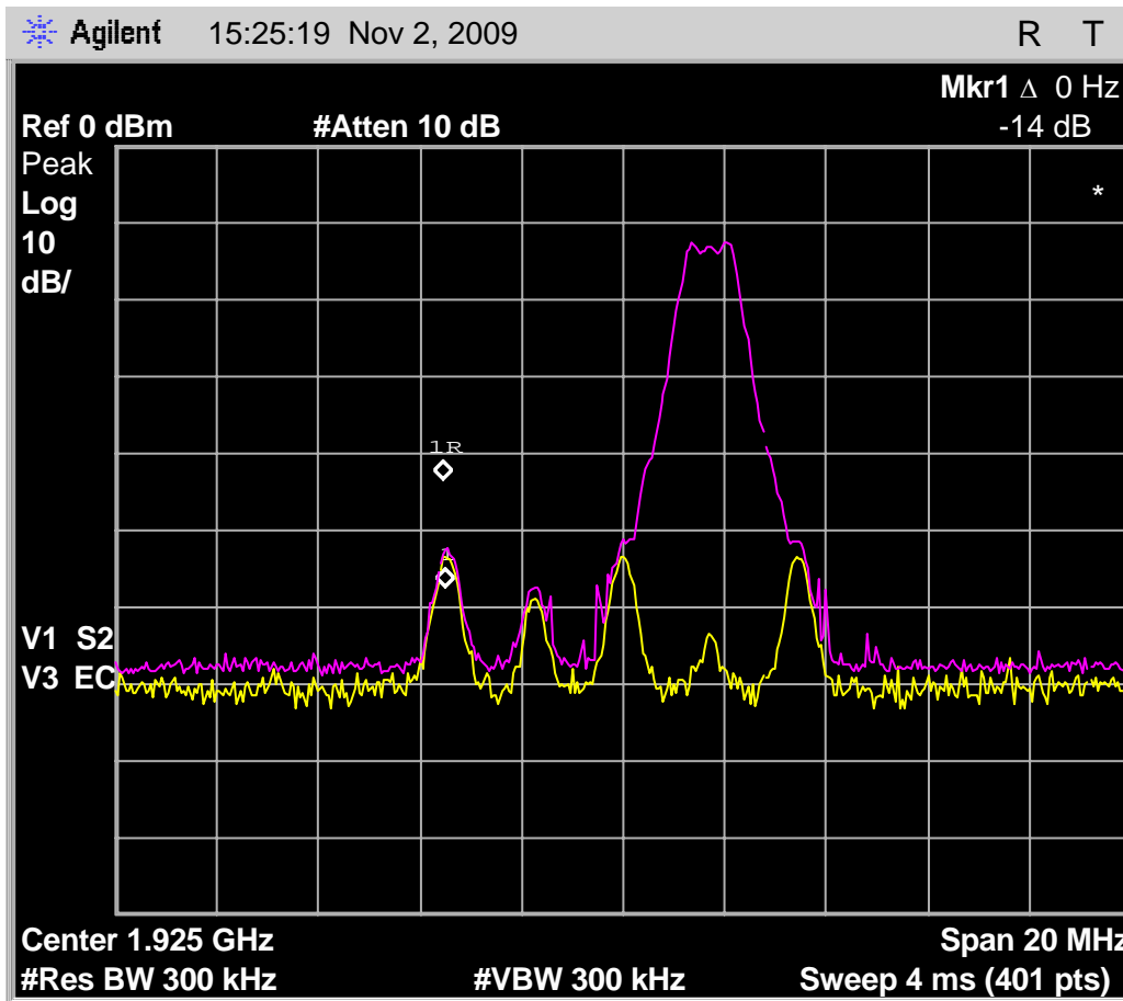
Fig. 79 - Emissions and interference profile spectrum, headset EUT, test 7.3.3(c).
