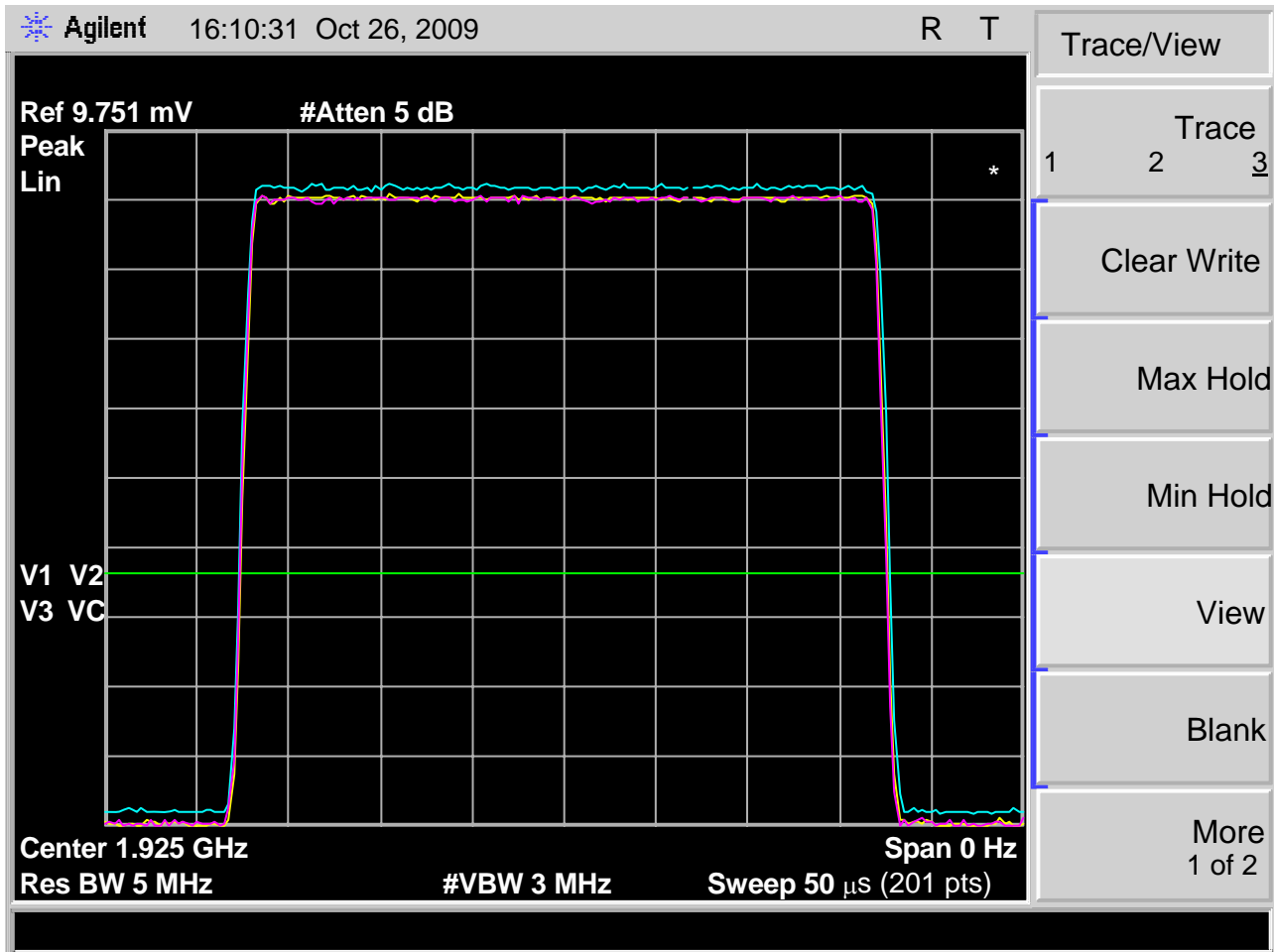
Fig. 58 - 35µs interference pulse for 7.5(d), duration and amplitude variation over the duration of the pulse and over multiple pulses. Spectrum analyzer is set to linear response.
