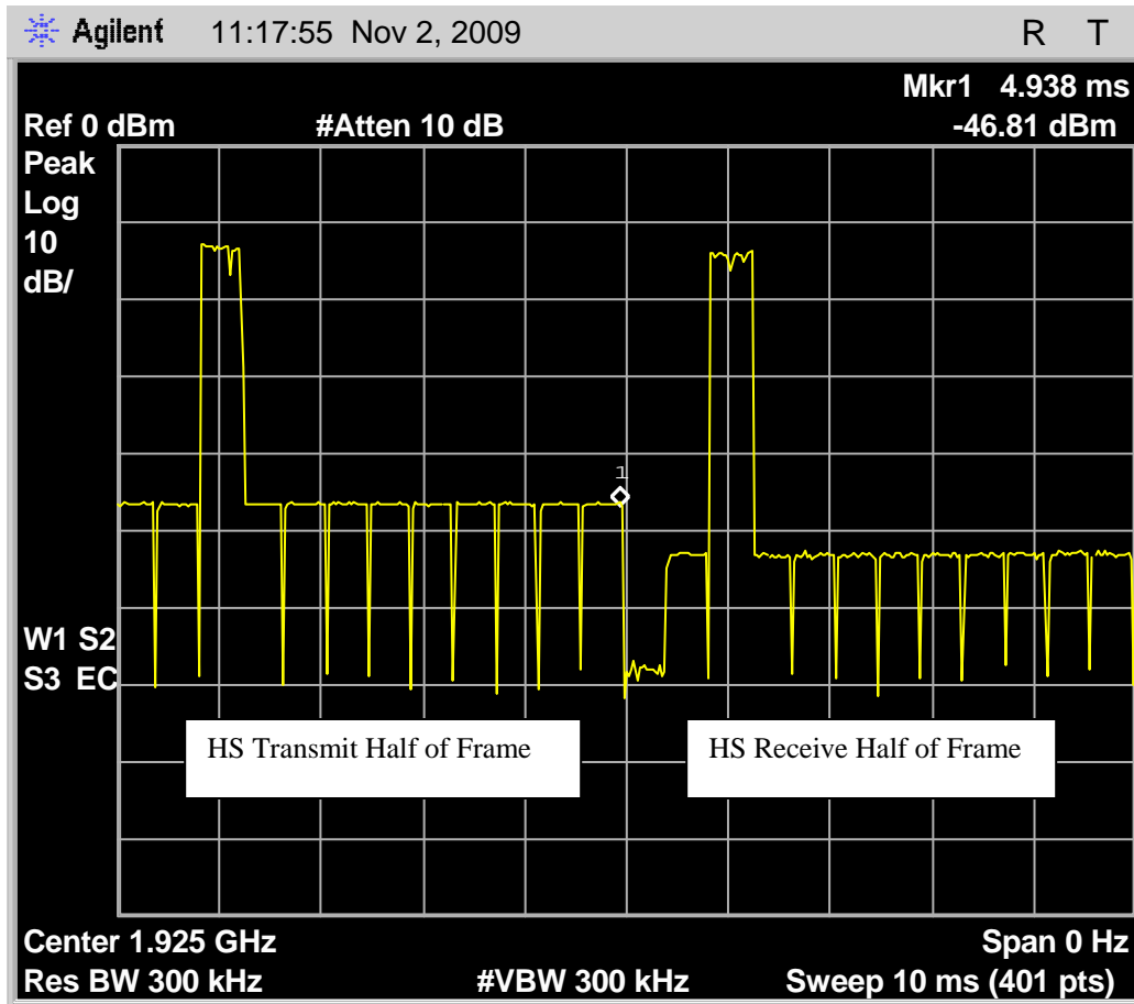
Fig. 72 – Headset EUT selects slot 2 pair which has the lowest maximum level of interference
