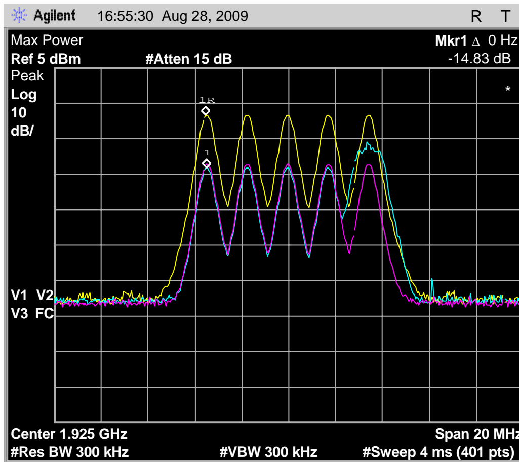
Fig. 94 - Emissions and interference profile spectrum, headset EUT, test 7.3.2.
