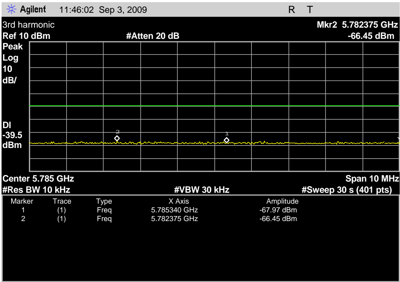
Fig. 37 – headset emissions measured in 10kHz resolution bandwidth in the region where the 1935MHz to 19.3GHz sweep at 300kHz observed a 3 rd harmonic response, for the headset transmitting on the high carrier, 1928.448MHz. A margin of greater than 25dB observed when measured in the specified resolution bandwidth.
