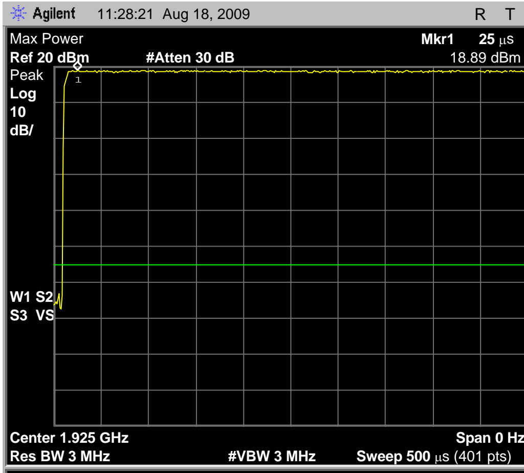
Fig. 75 - Headset EUT transmit power received by spectrum analyzer configured according to the requirements of clause 6.1.2 of C63.17-2006, mid carrier. Maximum observed transmit power is 18.89 dBm in WBM; output power for normal mode on mid channel was 18.89dBm.
