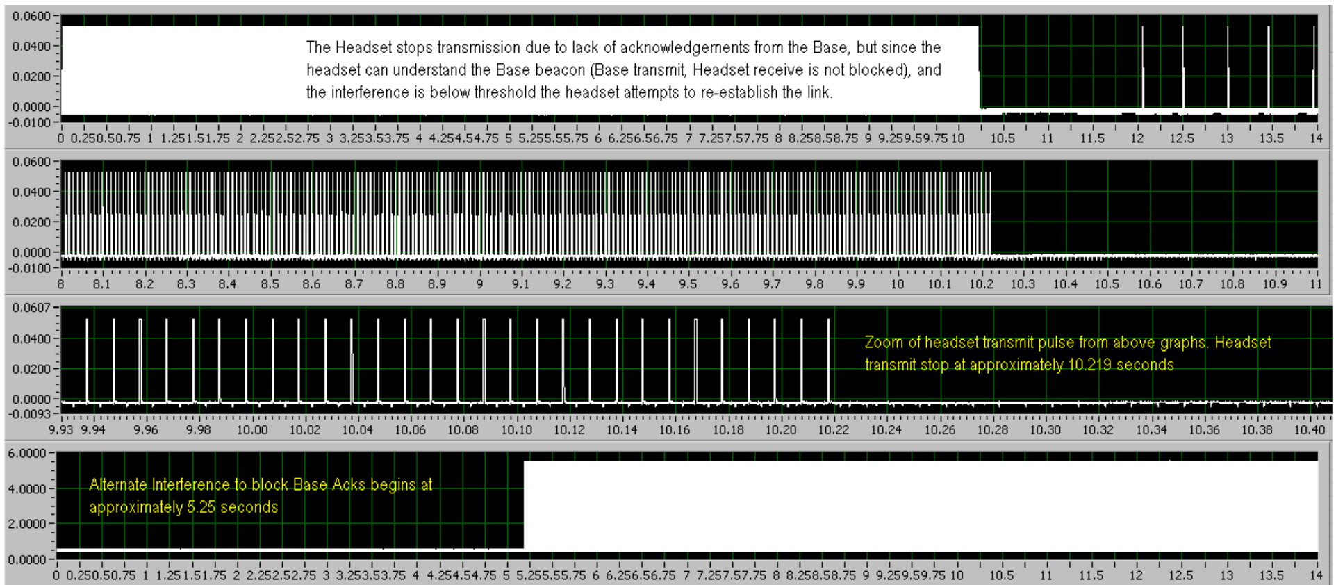
Fig. 70 - RF detector (top three traces) and alternate interference output (bottom trace) as headset EUT transmission goes blocked and transmissions stop.
