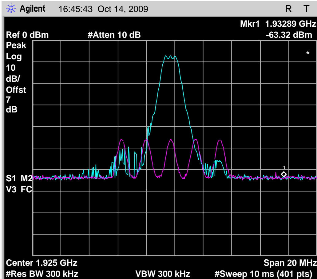
Fig. 84 - Transmit spectrum of 50uS interference pulses, with headset EUT no longer deferring with interference pulses of level T_L - U_M
