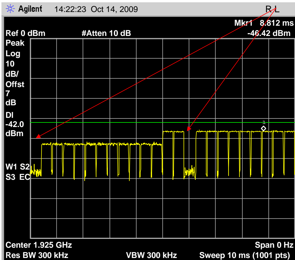
Fig. 73 – Spectrum analyzer screen capture of the interference pattern prior to headset link with companions Base (initial interference profile)
