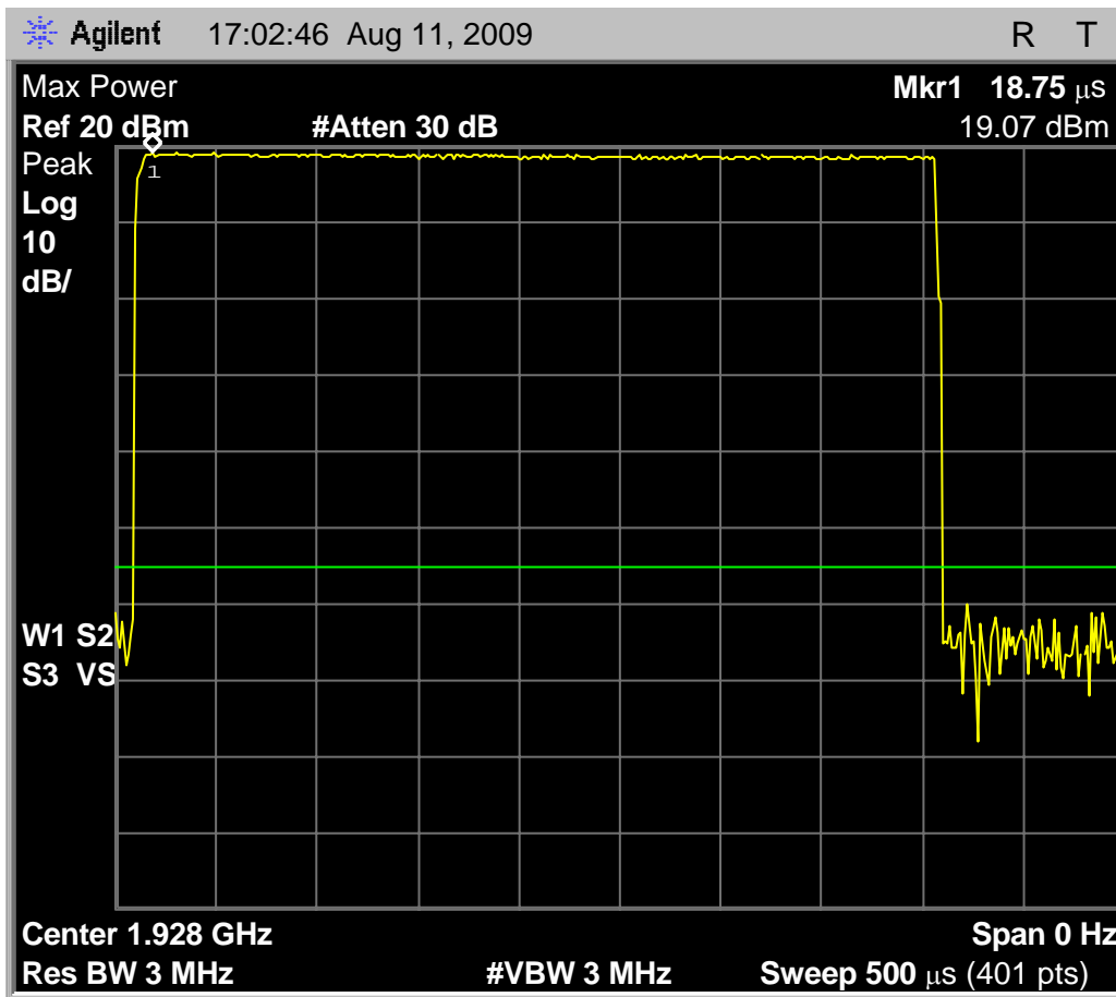
Fig. 10 - Headset EUT transmit power received by spectrum analyzer configured according to the requirements of clause 6.1.2 of C63.17-2006, high carrier. Maximum observed transmit power is 19.07 dBm.
