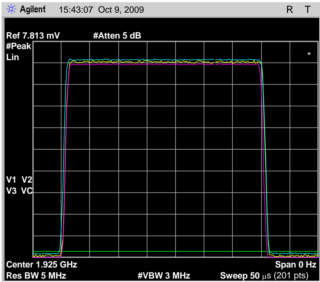
Fig. 62 - 35uS interference pulse for 7.5(d), duration and amplitude variation over the duration of the pulse and over multiple pulses. Spectrum analyzer is set to linear response.
