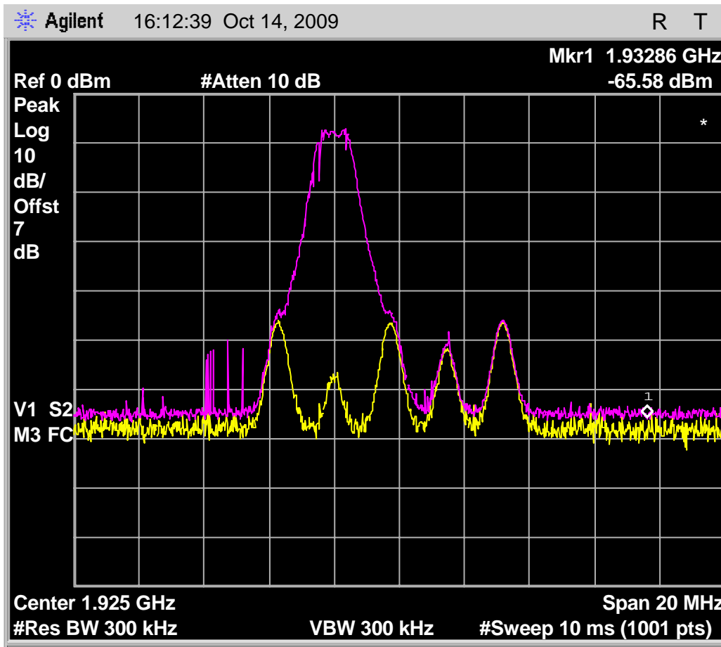
Fig. 82 - Emissions and interference profile spectrum, headset EUT, test 7.3.3(b).
