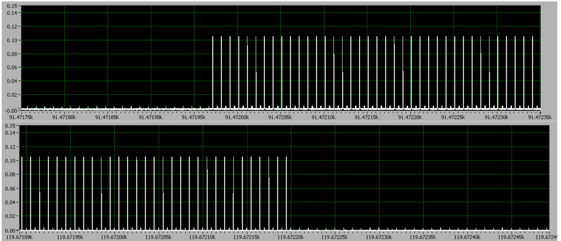
Fig. 71 - RF detector output showing timed initiation of headset EUT transmissions (top trace), then termination (bottom trace) when the headset EUT finds no channels passing the access criteria test. The scale shown is in seconds, with the start of the link at 91.471kS (relative start time), and the termination time being at 119.672k seconds which is equivalent to 28200.3 seconds or 7.83 hours. The headset EUT terminates transmissions after approximately 7 hours and 50 minutes from link initiation, so meeting the requirement of 8.2.2 that the headset execute the access criteria test at least as often as every 28800 seconds (or every 8 hours).
