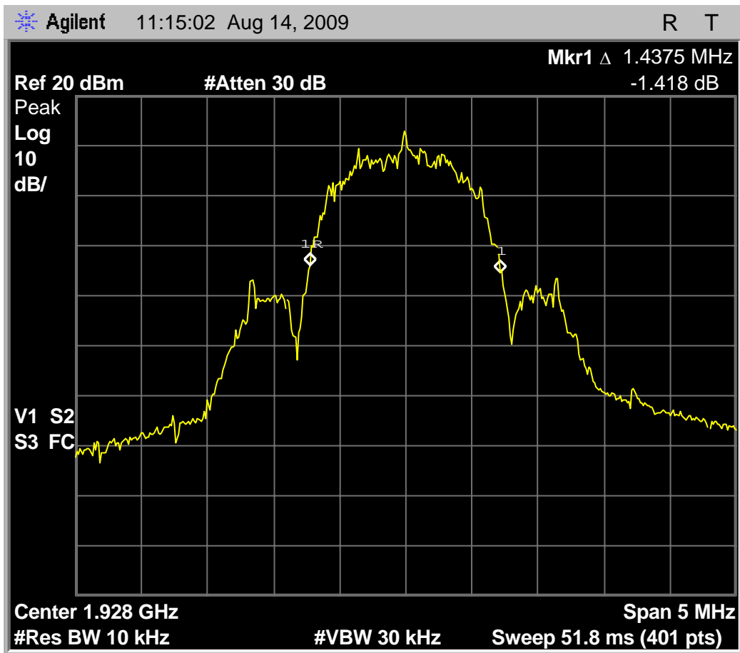
Fig. 13 - Headset EUT, 1.44MHz emissions bandwidth on high carrier.
