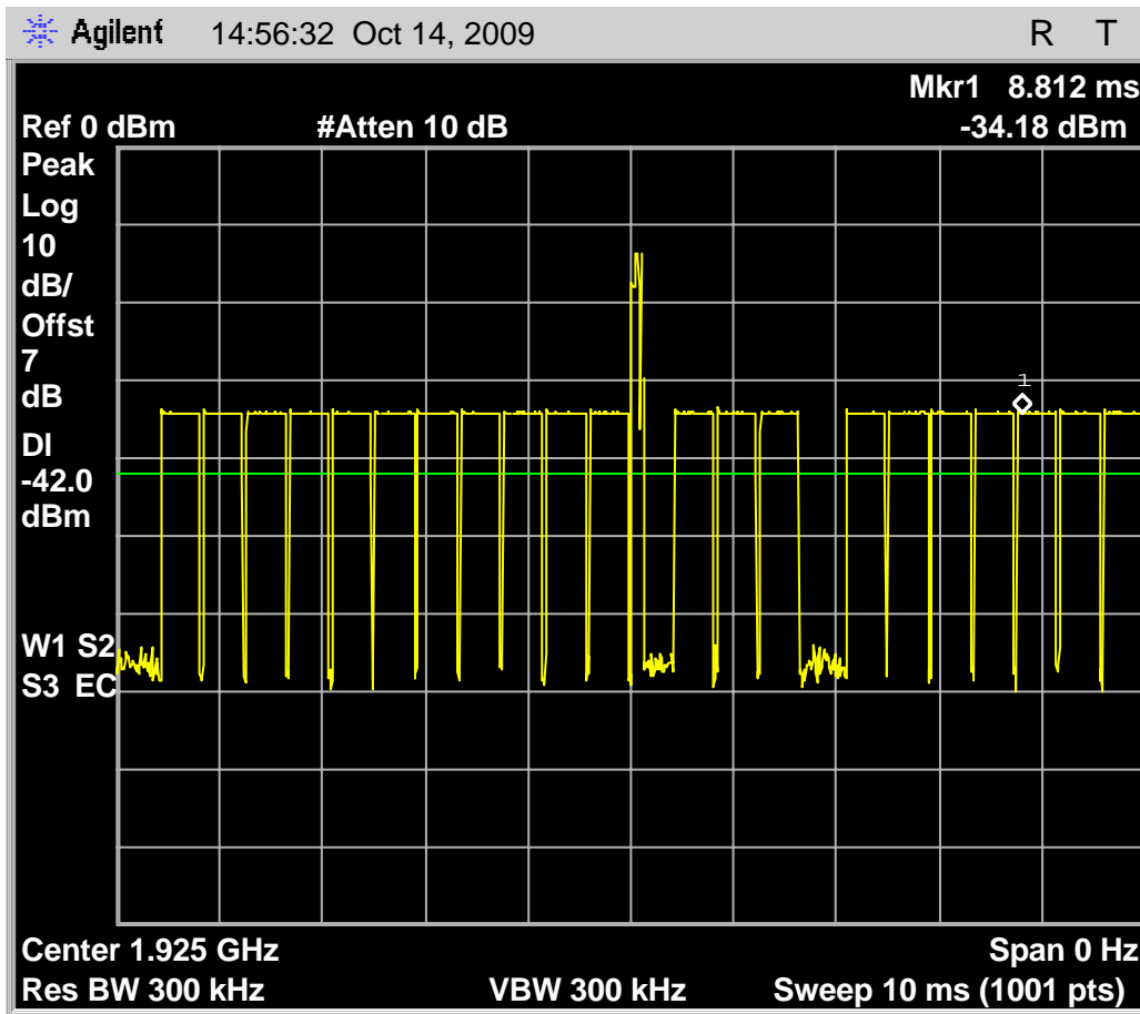
Fig. 78 – Interference profile for the Headset EUT that is above the threshold of -55.6\text{dBm} ( TU + UM ) without an open time slot pair. Slots that are opened are headset transmit slot 0 and headset receive slot 4 (slot 16). Note an additional time slot was opened to provide a place for the Base beacon of the companion device. If the base beacon was to occupy slot 0 or slot 16 a link could not be established and the test would pass but not be valid. Another option would be to force the Base to another carrier, but could not be monitored at the same time as the interference profile of interest.
