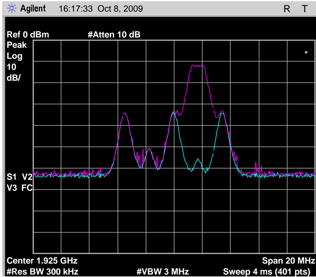
Fig. 52 - Emissions and interference profile spectrum, headset EUT, test 7.3.3(e).
