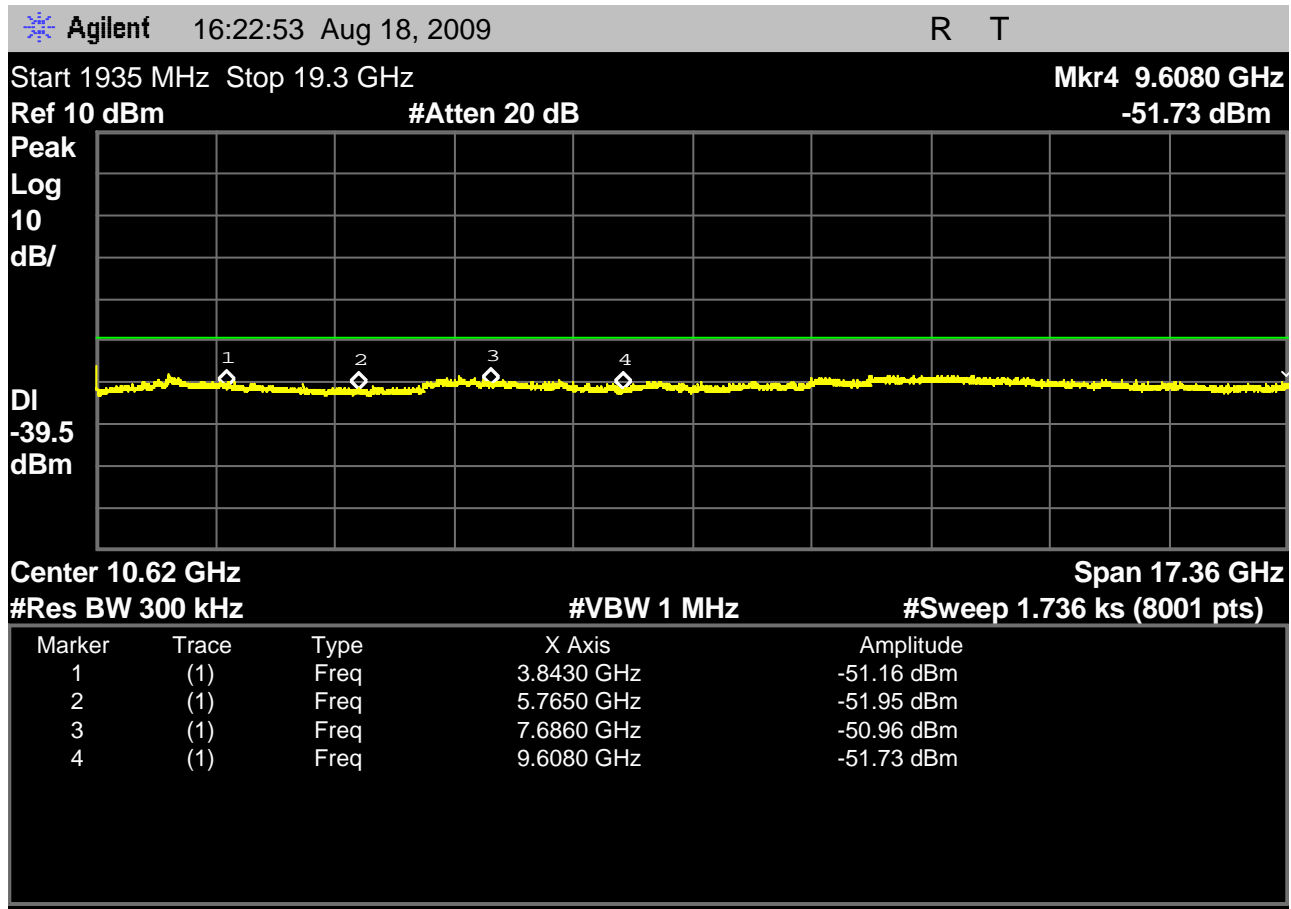
Fig. 95 - headset EUT in minimum power WBM on low carrier, harmonics in this scan are all within specification by 10dB even while measured in the 300kHz and below the harmonics observed in maximum output power mode.
