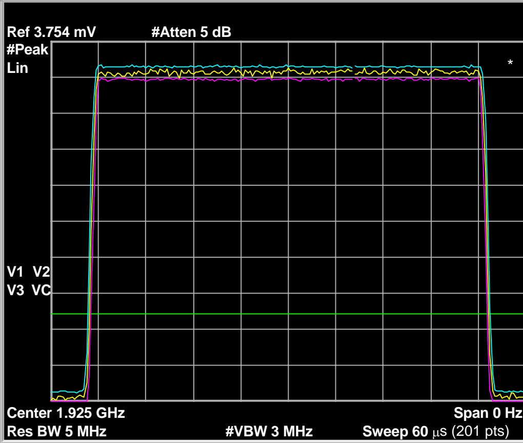
Fig. 58 – 50uS interference pulse for 7.5(c), duration and amplitude variation over the duration of the 50 uS pulse and over multiple pulses. Spectrum analyzer is set to linear response.
