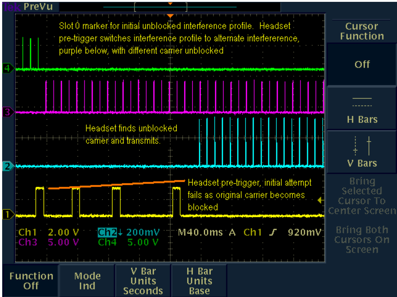
Fig. 54 - Screen shot of oscilloscope showing deferral by the headset EUT in the case where the interference profile changes in the frame previous to intended transmission and the selected time and frequency communications channel becomes blocked; and then later, transmission on unblocked channel.
