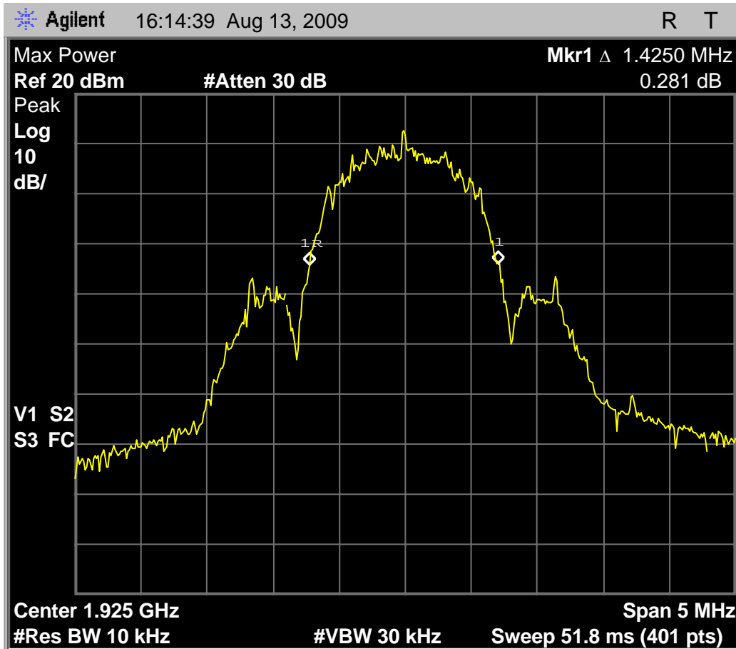
Fig. 80 - Headset EUT in WBM, 1.43MHz emissions bandwidth on mid carrier vs. 1.45MHz in normal mode max power.
