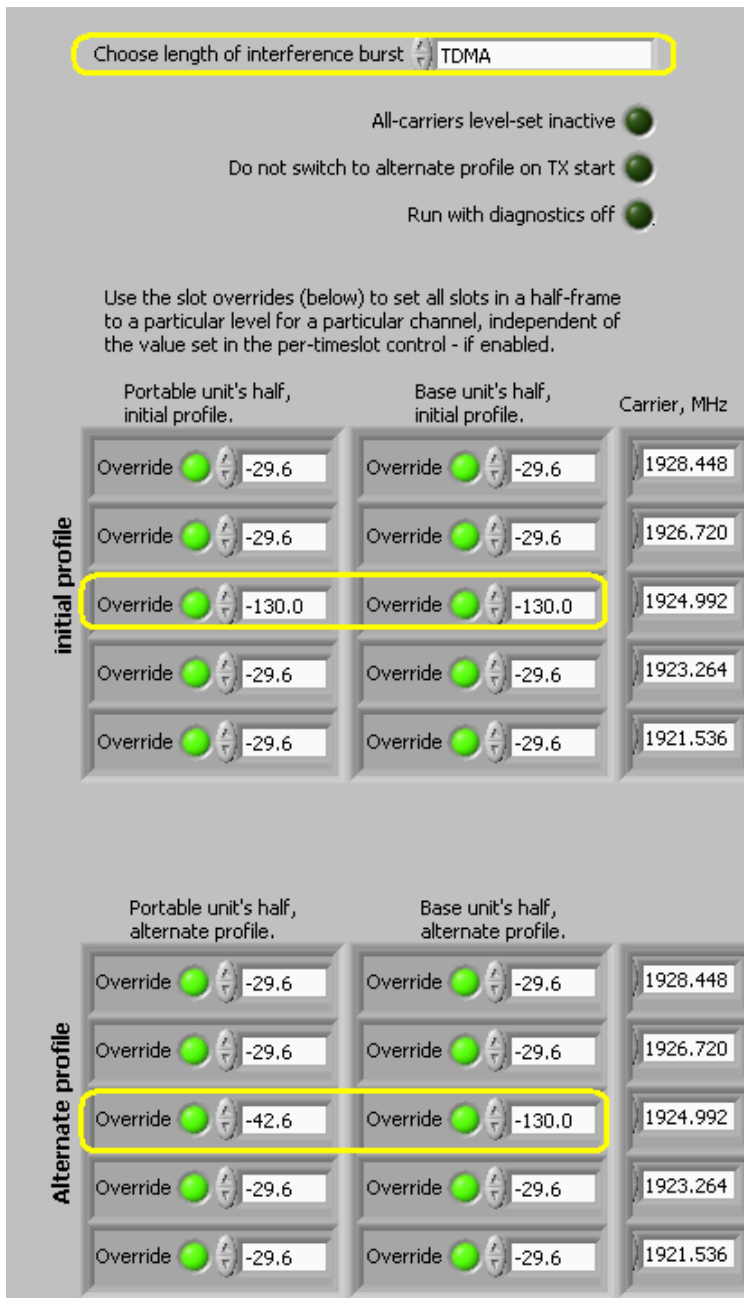
Fig. 69 - PXI-5670 multi-carrier interference generator control panel for the test of 8.2.1(c), for the headset EUT.
