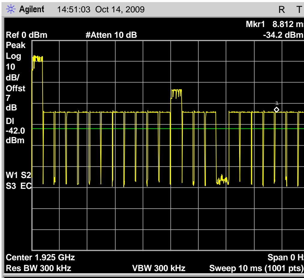
Fig. 77 – Interference profile for the Headset EUT that is above the threshold of -55.6\text{dBm} ( TU + UM ) WITH an open slot pair to demonstrate a link was possible for the test set up when 8.3.2 g) was performed.
