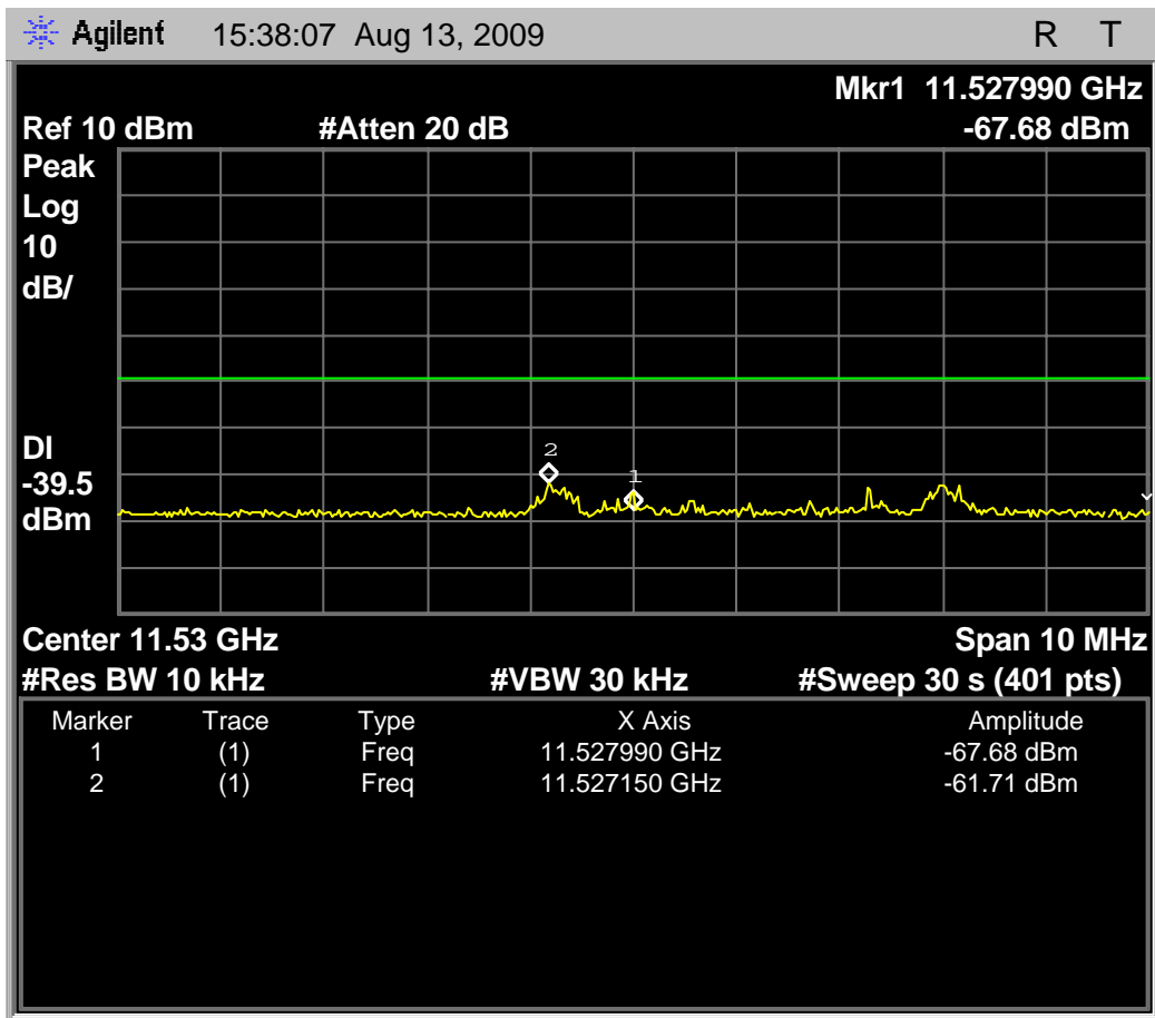
Fig. 32 – headset EUT out-of-band emissions in the region around the 6th harmonic, with the headset EUT transmitting on the lowest carrier, 1921.536MHz.
