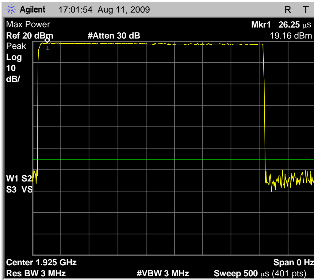
Fig. 9 - Headset EUT transmit power received by spectrum analyzer configured according to the requirements of clause 6.1.2 of C63.17-2006, mid carrier. Maximum observed transmit power is 19.16 dBm
