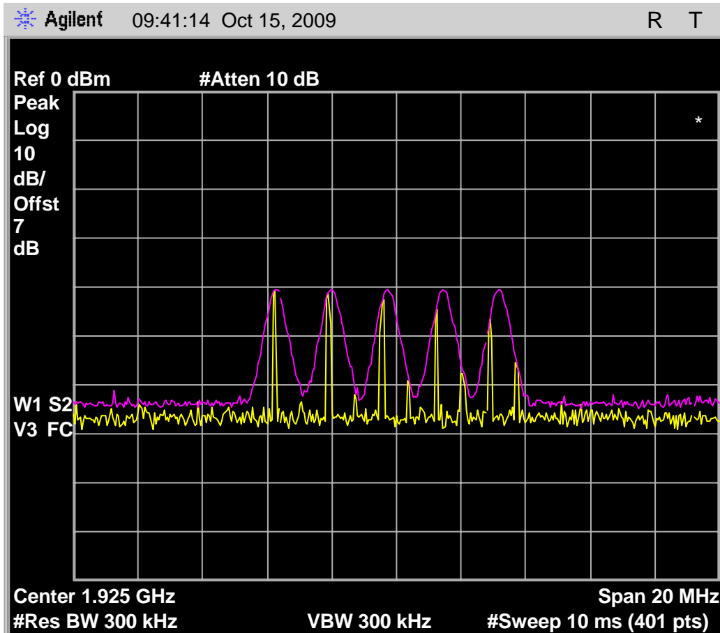
Fig. 86 - Transmit spectrum of 35uS interference pulses in each timeslot for each carrier, with headset EUT deferring due to interference pulses of T_L + U_M + 6\text{dB} ( -69.6\text{dB} ).
