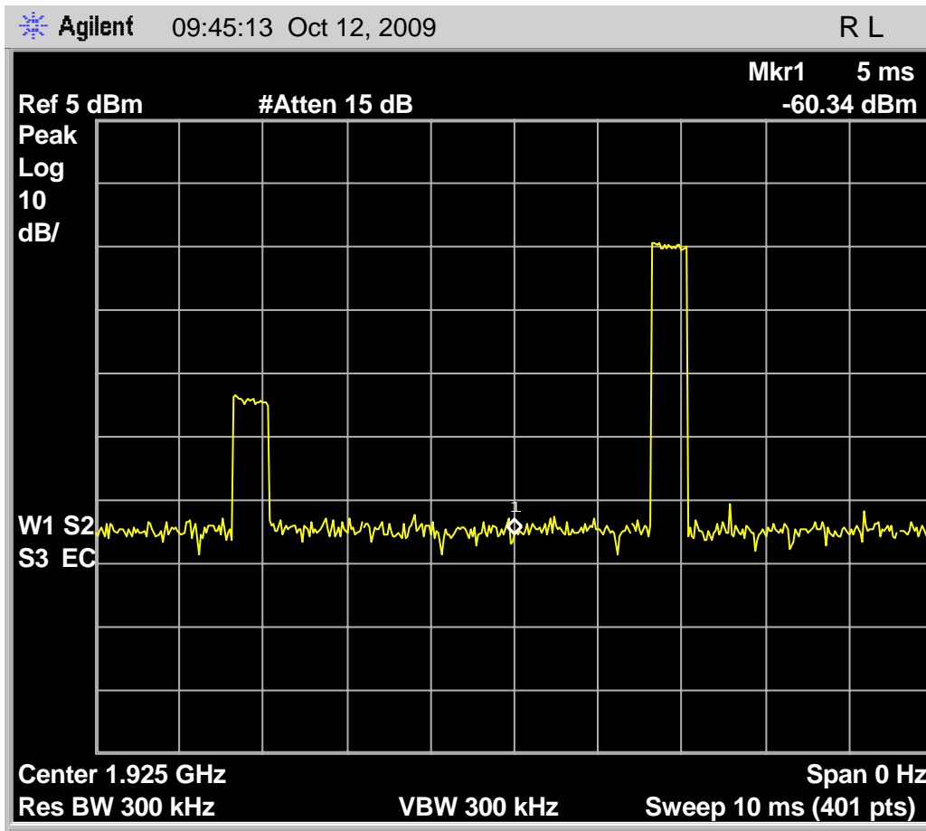
Fig. 68 - Screenshot of spectrum analyzer showing one frame of the channel with the initial interference profile present, which does not block the reception by the base EUT of the headset EUT's transmissions; an acknowledgement is generated when the headset EUT attempts to initiate the communications channel when the TALK button is pressed, and the communications channel is established, so the headset EUT meets the requirements of 8.2.1(b) for proper operation of the test setup when the acknowledgements are unblocked.
