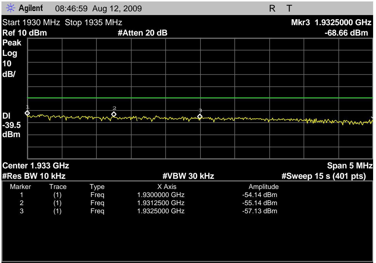
Fig. 36 – headset EUT out-of-band emissions showing the regions from bandedge to +1.25MHz, and from +1.25MHz to +2.5MHz, with the headset EUT transmitting on the highest carrier, 1928.448MHz.
