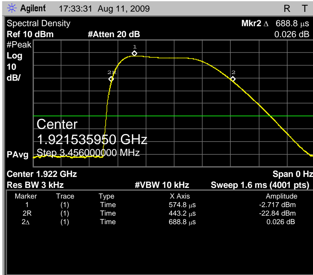
Fig. 14 – Zero-span sweep for headset EUT, low carrier, for 3kHz maximum power spectral density. The peak level is at -2.72 dBm, and the interval between samples at the -20dB points is 688.8us.
