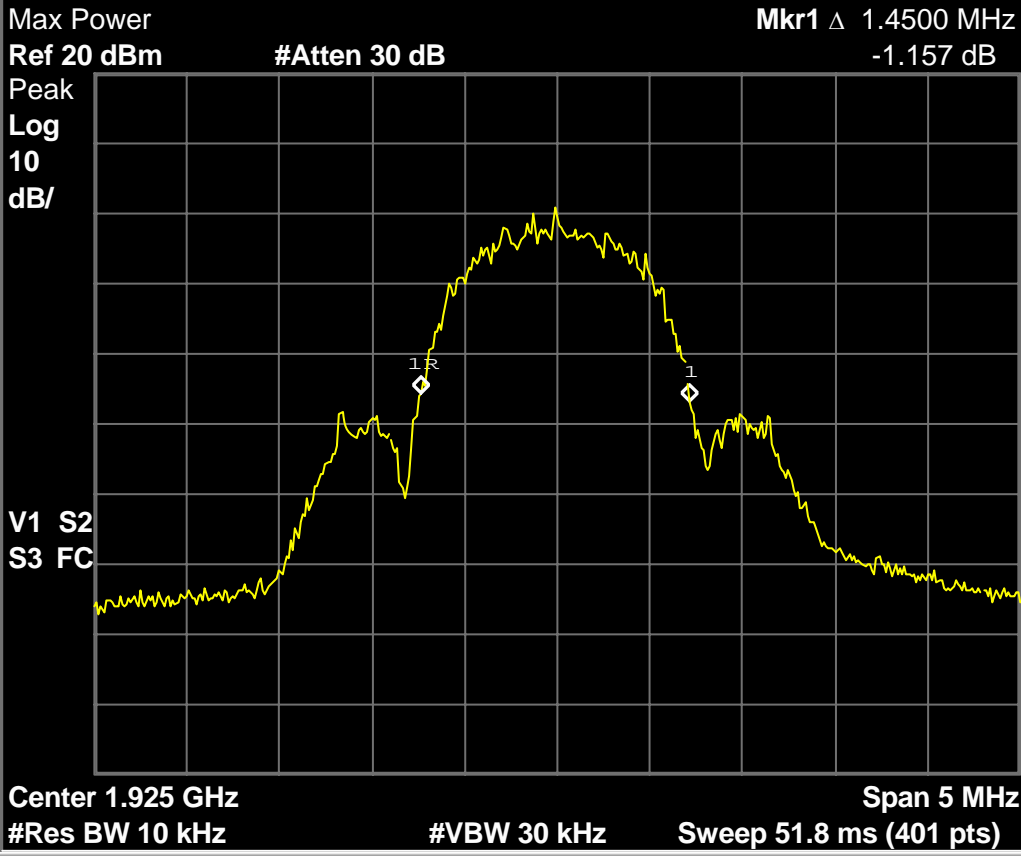
Fig. 93 - Headset EUT in WBM, 1.45MHz emissions bandwidth on mid carrier vs. 1.45MHz in normal mode high power.
