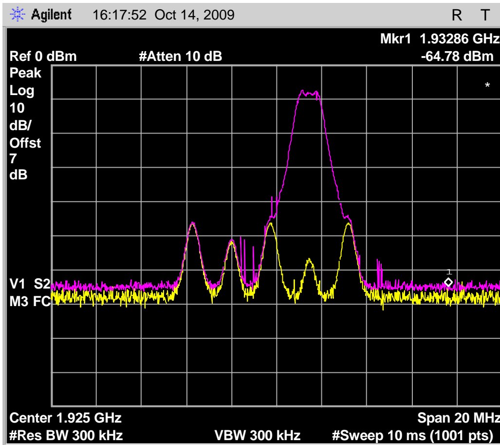
Fig. 83 - Emissions and interference profile spectrum, headset EUT, test 7.3.3(c).
