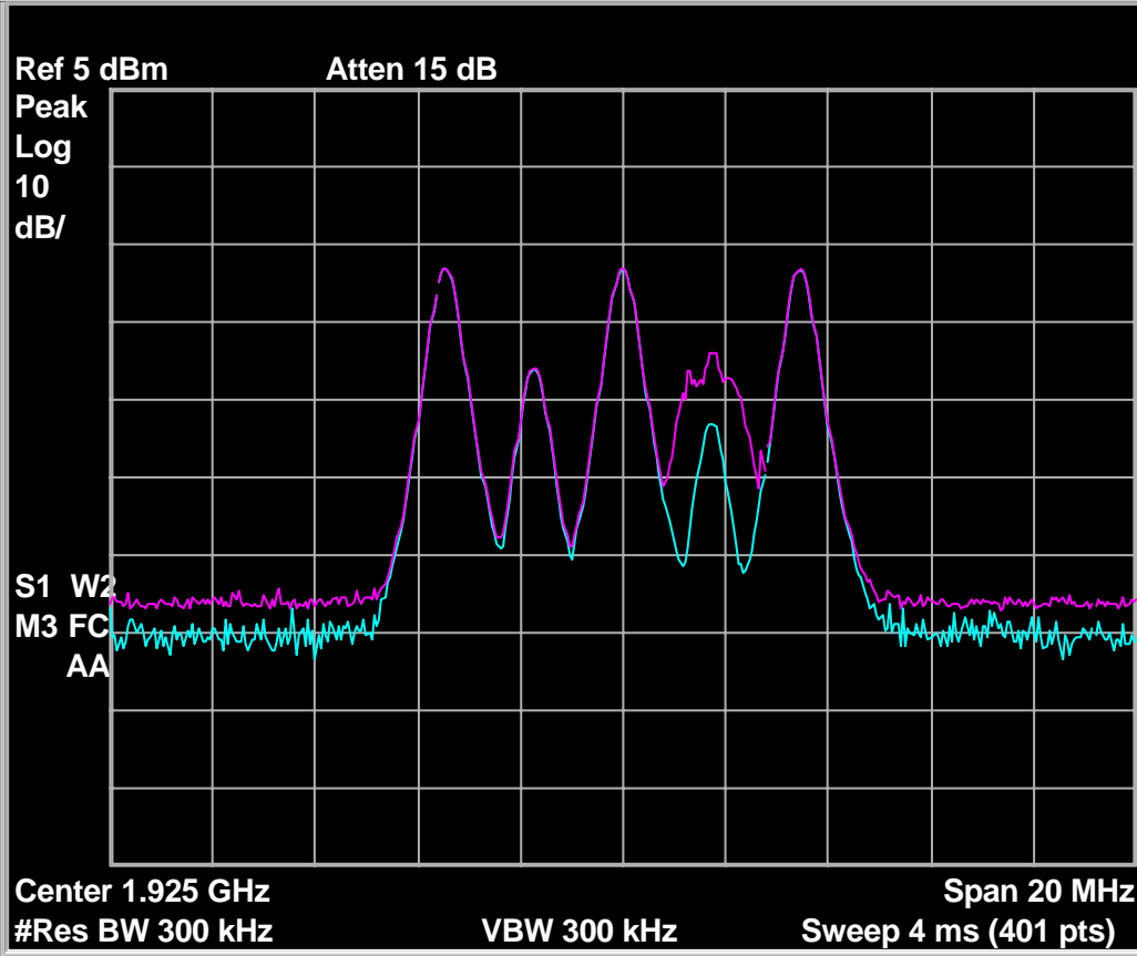
Fig. 100 - Emissions and interference profile spectrum, headset EUT, test 7.3.3(c).
