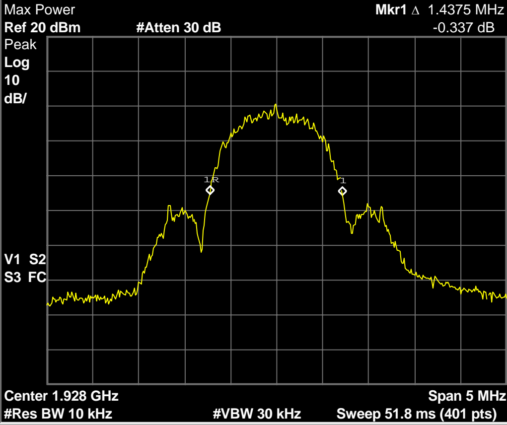
Fig. 94 - Headset EUT in WBM, 1.44MHz emissions bandwidth on high carrier vs. 1.44MHz in normal mode high power.
