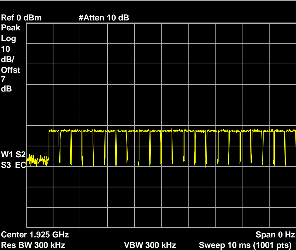
Fig. 90 – Interference profile for the Headset EUT that is above the threshold of -75.6\text{dBm} ( T_L + U_M ) without an open time slot pair. Headset EUT transmit slots that are interference free are 0 and 1 (one WBM slot).
