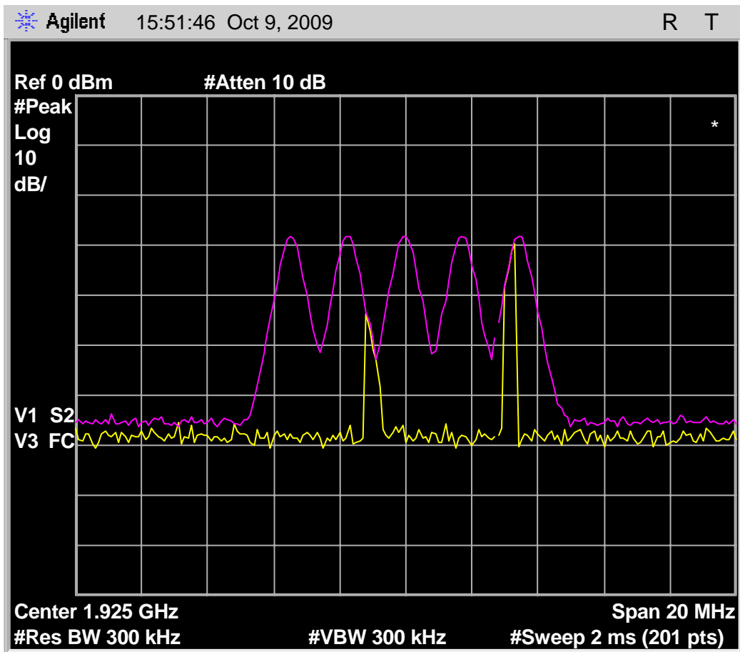
Fig. 63 - Transmit spectrum of 35uS interference pulses in each timeslot for each carrier, with headset EUT deferring due to interference pulses of T_U + U_M + 6\text{dB} .
