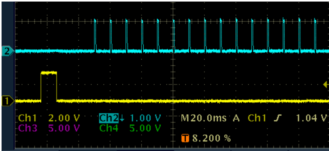
Fig. 85 - Normal initiation of transmissions by the headset EUT in the absence of over-threshold interference; the headset EUT software flags the start of the transmission setup (bottom trace), and transmit emissions are recovered by the RF detector (top trace) in the splitter/combiner network. Proper transmission at T_L - U_M is shown, to validate functionality and to illustrate the getting-ready-to-transmit marker, and the RF detector output.
