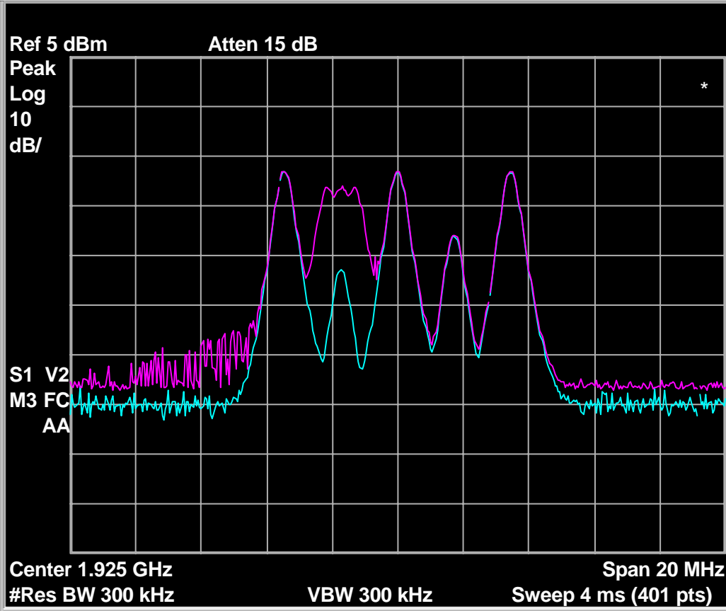
Fig. 99 - Emissions and interference profile spectrum, headset EUT, test 7.3.3(b).
