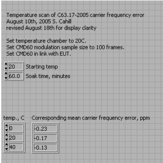
Fig. 45 - Measured mean carrier frequency, headset EUT , at 0C, +20C, +40C.
