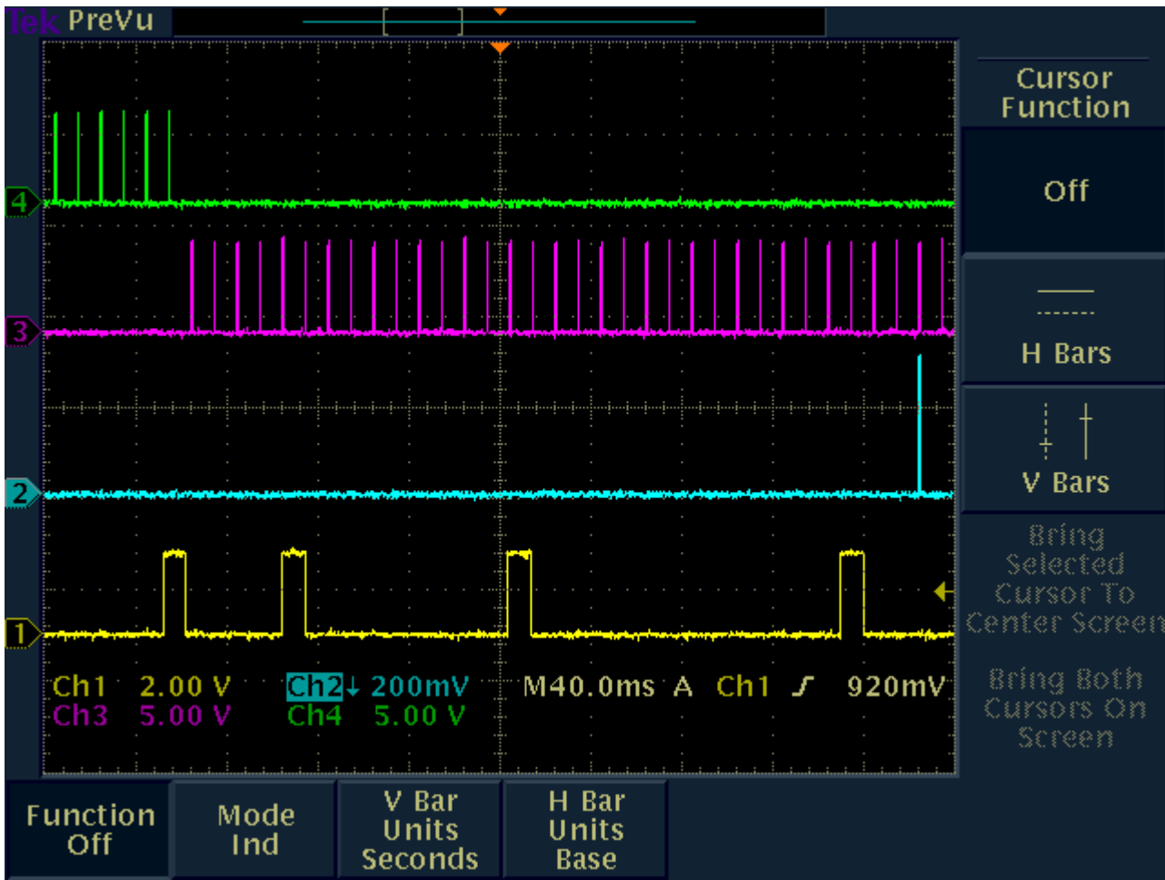
Fig. 67 – Screenshot zoom of the above figure. This screen capture shows that the first actual attempt to transmit a signal from the headset to the Base wasn't until the fourth attempt. The first 4 attempts Ch1 (yellow trace) have no corresponding RF output Ch2 (cyan) trace. The first attempt correctly recognizes that the interference level had changed and thus no RF transmission from Base to headset takes place, and the following two pulses on Ch1 also do not transmit as the RSSI (receive strength indicator) value is too large of a change, by the fourth Ch1 pulse the receiver has re-scanned the frequency time slots and found an acceptable (unblocked, and no large RSSI change) place to transmit.
