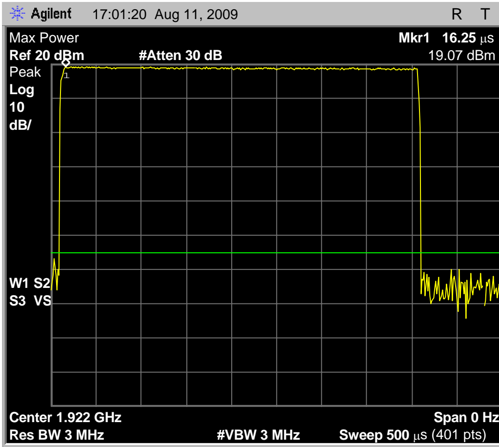
Fig. 8 - Headset EUT transmit power received by spectrum analyzer configured according to the requirements of clause 6.1.2 of C63.17-2006, low carrier. Maximum observed transmit power is 19.07 dBm.
