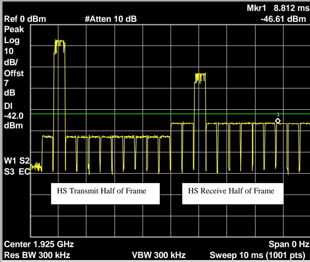
Fig. 74 – Headset EUT selects slot 2 pair which has the lowest maximum level of interference
