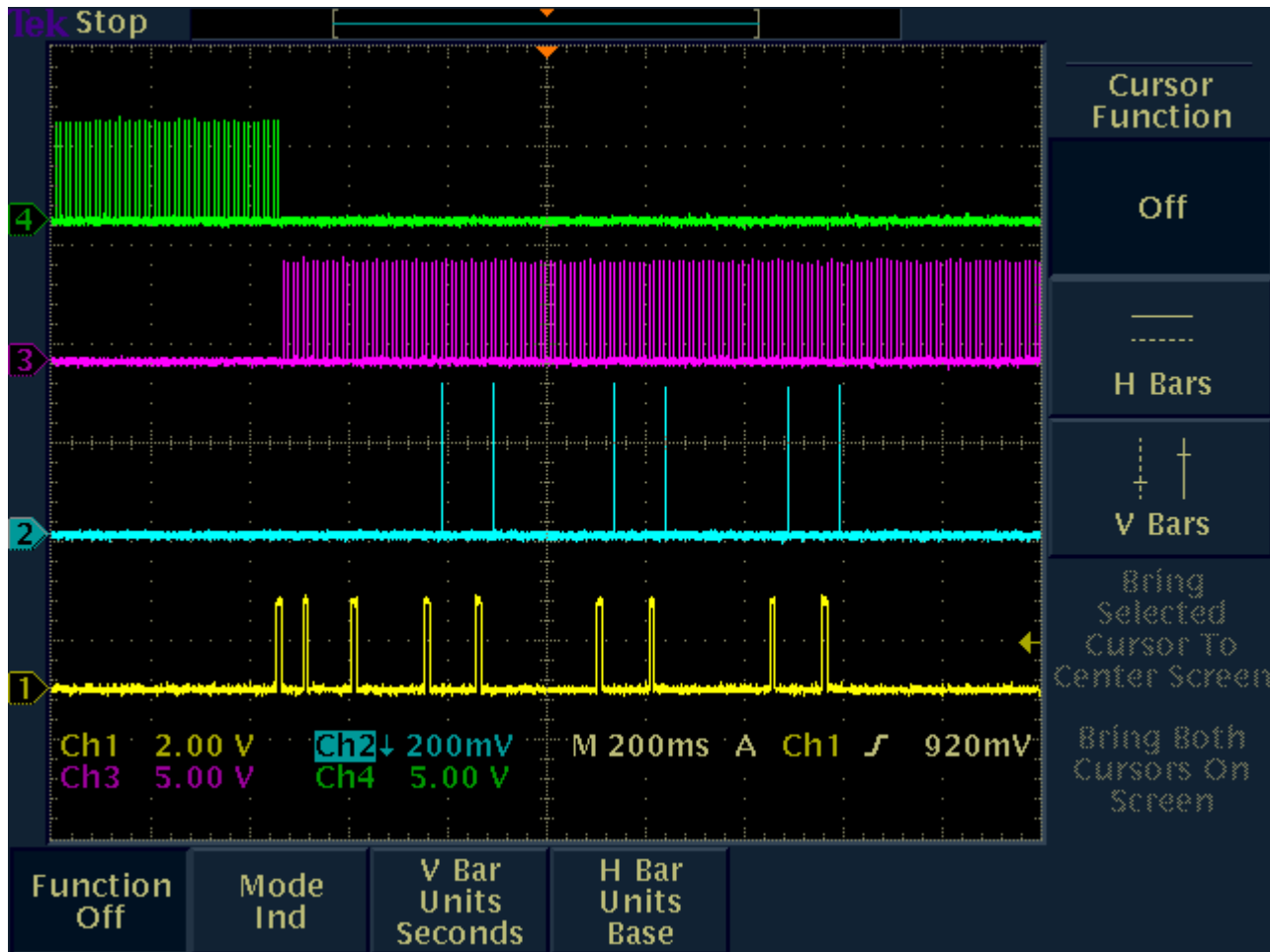
Fig. 66 - Screenshot of headset transmit-attempt flag activity (yellow Ch1 bottom trace) and RF detector output (cyan Ch2 2 nd from bottom) vs. time with the interference profiles (Ch4 is the primary interference which has an opened carrier (-130dBm interference level) and allows the headset and companion Base to idle lock to each other. The magenta trace is the Ch3 alternate interference profile which is automatically switched to when the headset TALK button is pressed. The headset tries multiple times to bring up a link without success as shown by (Ch2) RF detector having no signal after the initial attempts. The test was repeated and the RF detector trace monitored for 20 minutes without any further activity.
