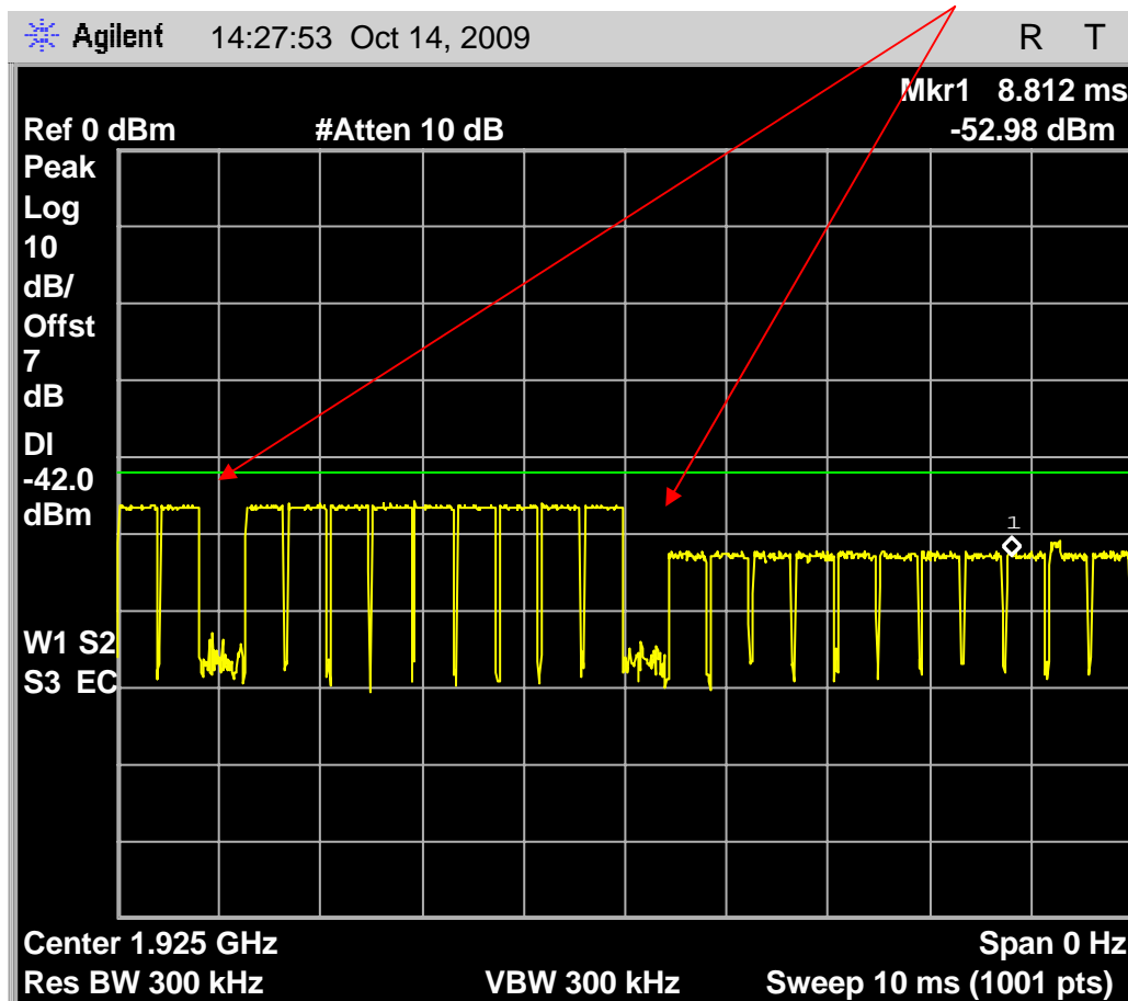
Fig. 75 – Spectrum analyzer screen capture of the interference pattern prior to headset link with companions Base (alternate interference profile from PXI screen capture of Fig 73)
