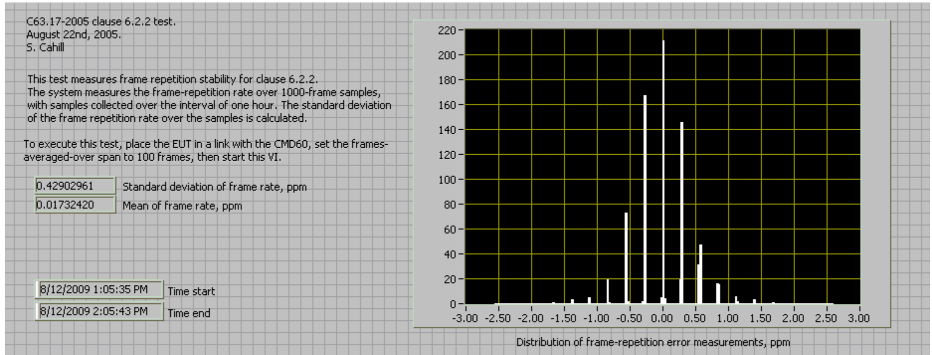
Fig. 46 - Test of headset EUT according to the conditions of clause 6.2.2 for frame repetition rate stability
