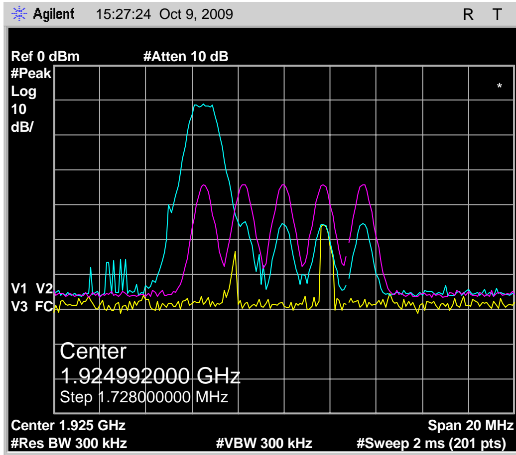
Fig. 59 - Transmit spectrum of 50uS interference pulses, with headset EUT no longer deferring with interference pulses of level T_U - U_M .
