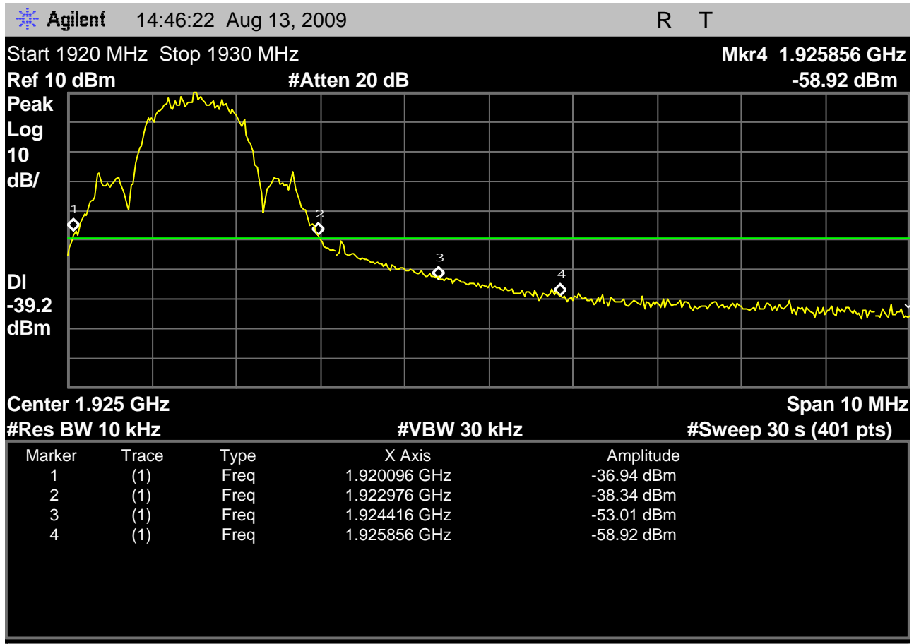
Fig. 20 - Spectrum analyzer screenshot for transmit emissions showing inband unwanted emissions with the headset EUT transmitter at the lowest carrier, 1921.536MHz, according to the requirements of 6.1.6.1.
