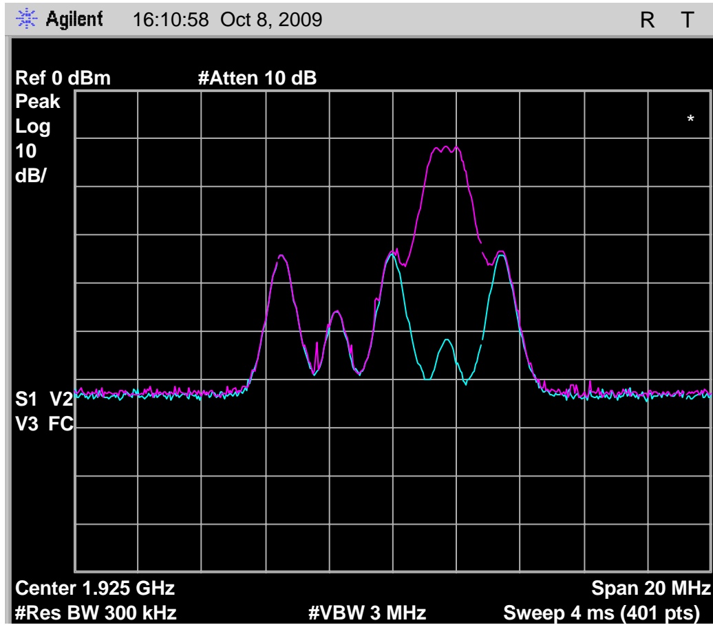
Fig. 50 - Emissions and interference profile spectrum, headset EUT, test 7.3.3(c).
