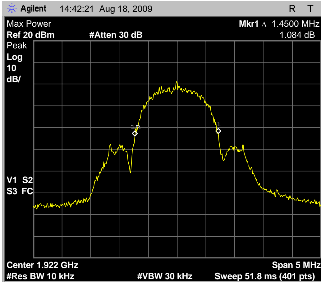
Fig. 92 - Headset EUT in WBM, 1.45MHz emissions bandwidth on low carrier vs. 1.45 MHz in normal mode high power.
