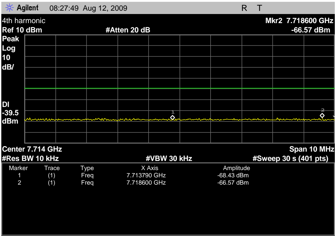
Fig. 40 – headset EUT out-of-band emissions in the region around the 4 th harmonic, with the headset EUT transmitting on the highest carrier, 1928.448MHz. A margin of greater than 25dB observed when measured in the specified resolution bandwidth.
