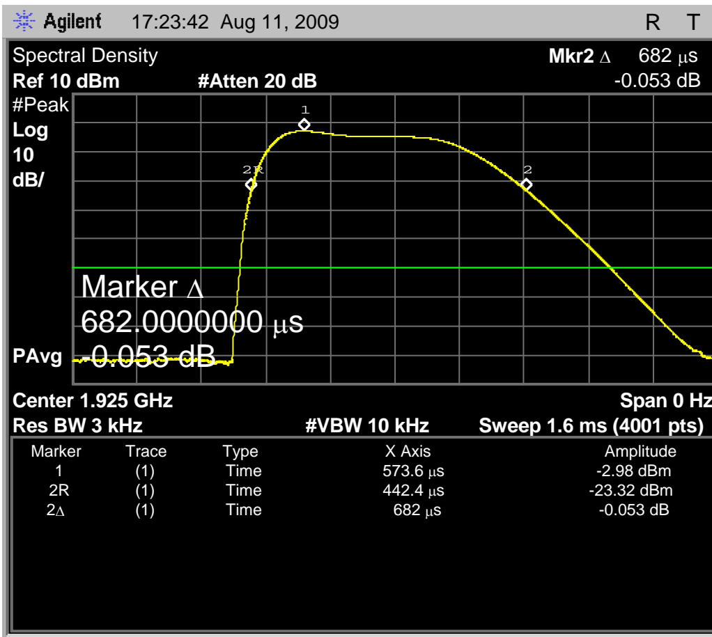
Fig. 16 – Zero-span sweep for headset EUT, middle carrier, for 3kHz maximum power spectral density. The peak level is at -2.98dBm, and the interval between samples at the -20dB points is 682.0us.
