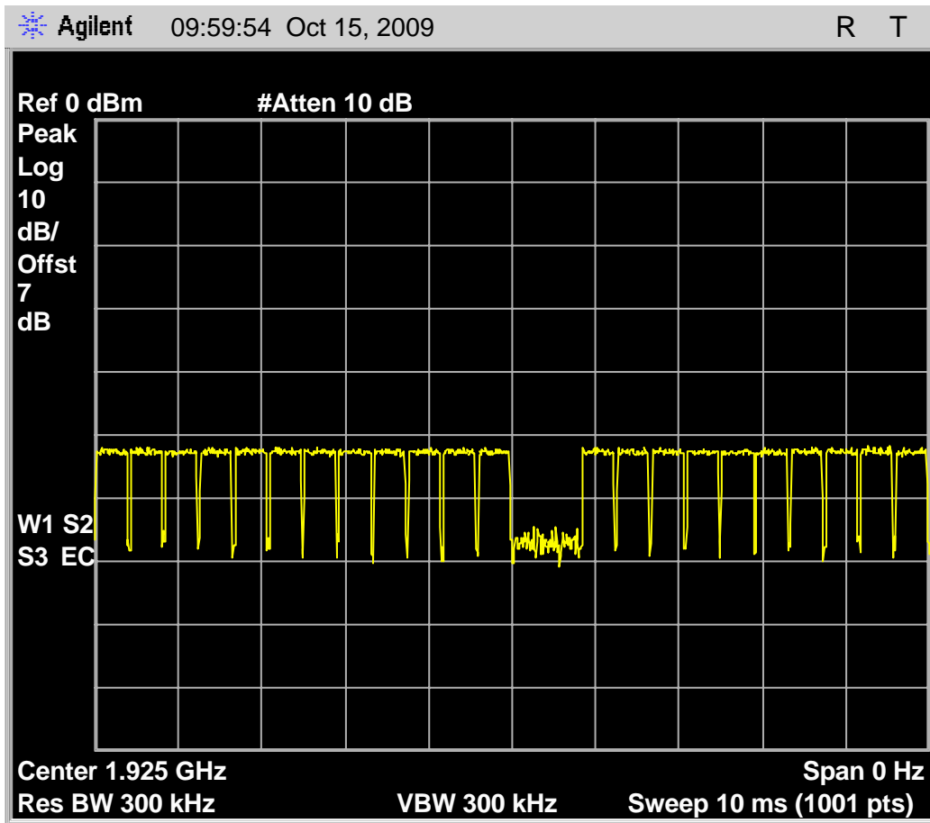
Fig. 88 – Interference profile for the Headset EUT that is above the threshold of -75.6\text{dBm} ( T_L + U_M ) without an open time slot pair. Slots that are interference free are headset receive slots 0 and 1 (slot 12 and 13).
