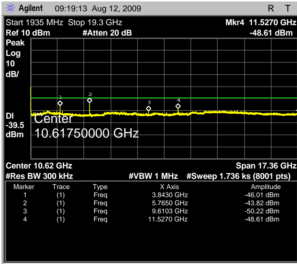
Fig. 27 – headset EUT out-of-band emissions including the regions from 1935MHz to 19.3GHz with the headset EUT transmitting on the lowest carrier, 1921.536MHz.
