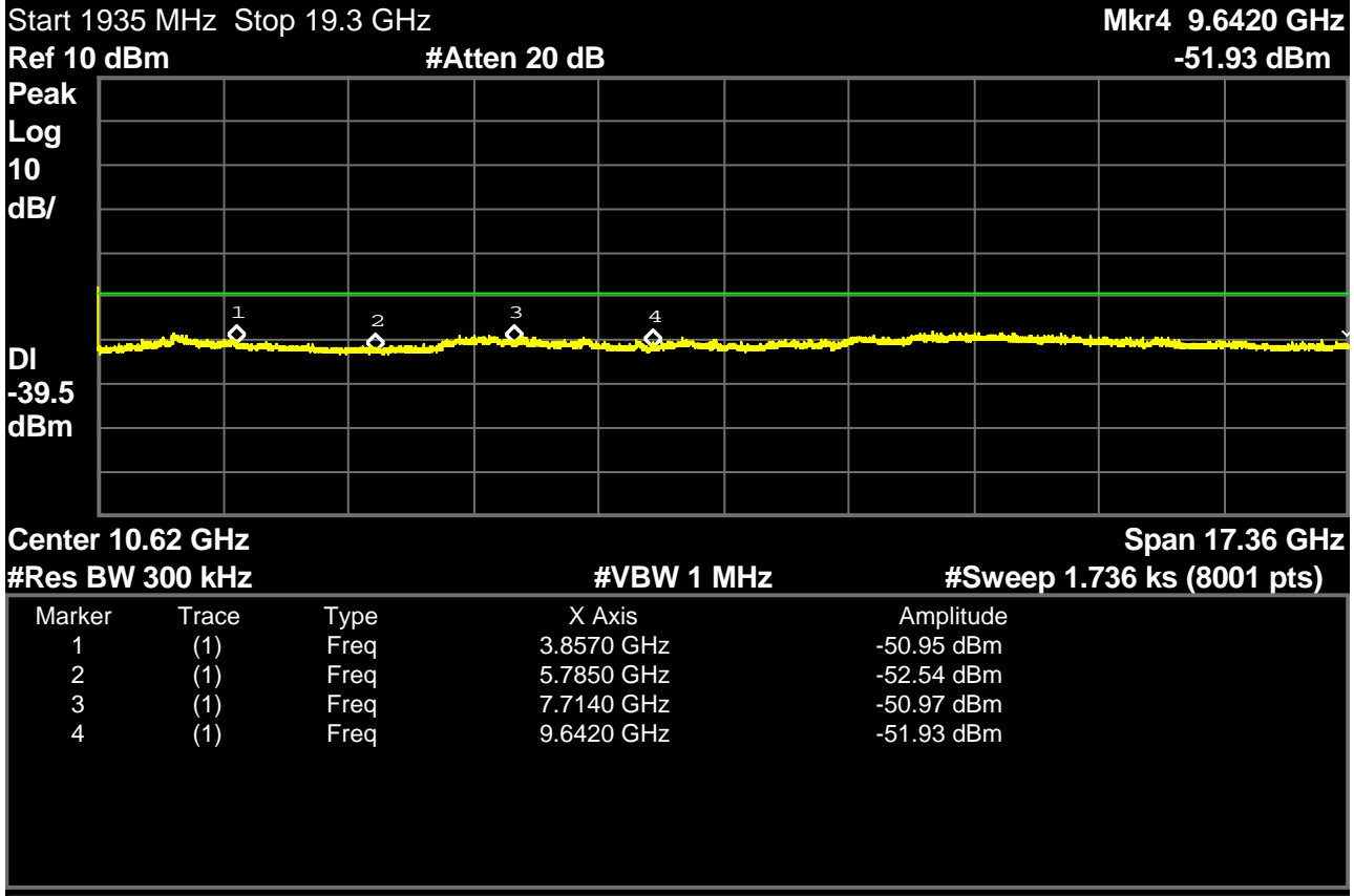
Fig. 96 - headset EUT in minimum power WBM on high carrier, harmonics all below the noise floor even with the increased resolution bandwidth, see section 6.1 of main report.
