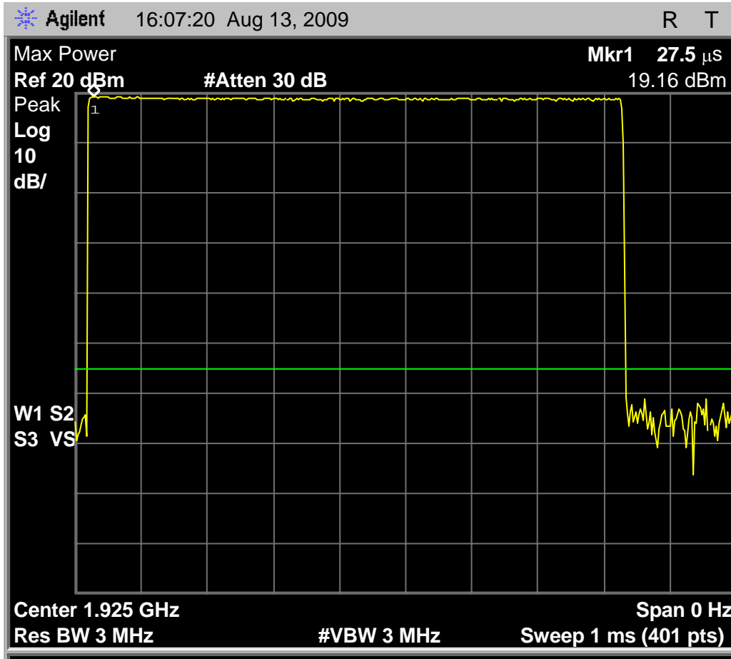
Fig. 79 - Headset EUT transmit power received by spectrum analyzer configured according to the requirements of clause 6.1.2 of C63.17-2006, mid carrier. Maximum observed transmit power is 19.16dBm in WBM; output power for normal mode on mid channel was 19.16dBm.
