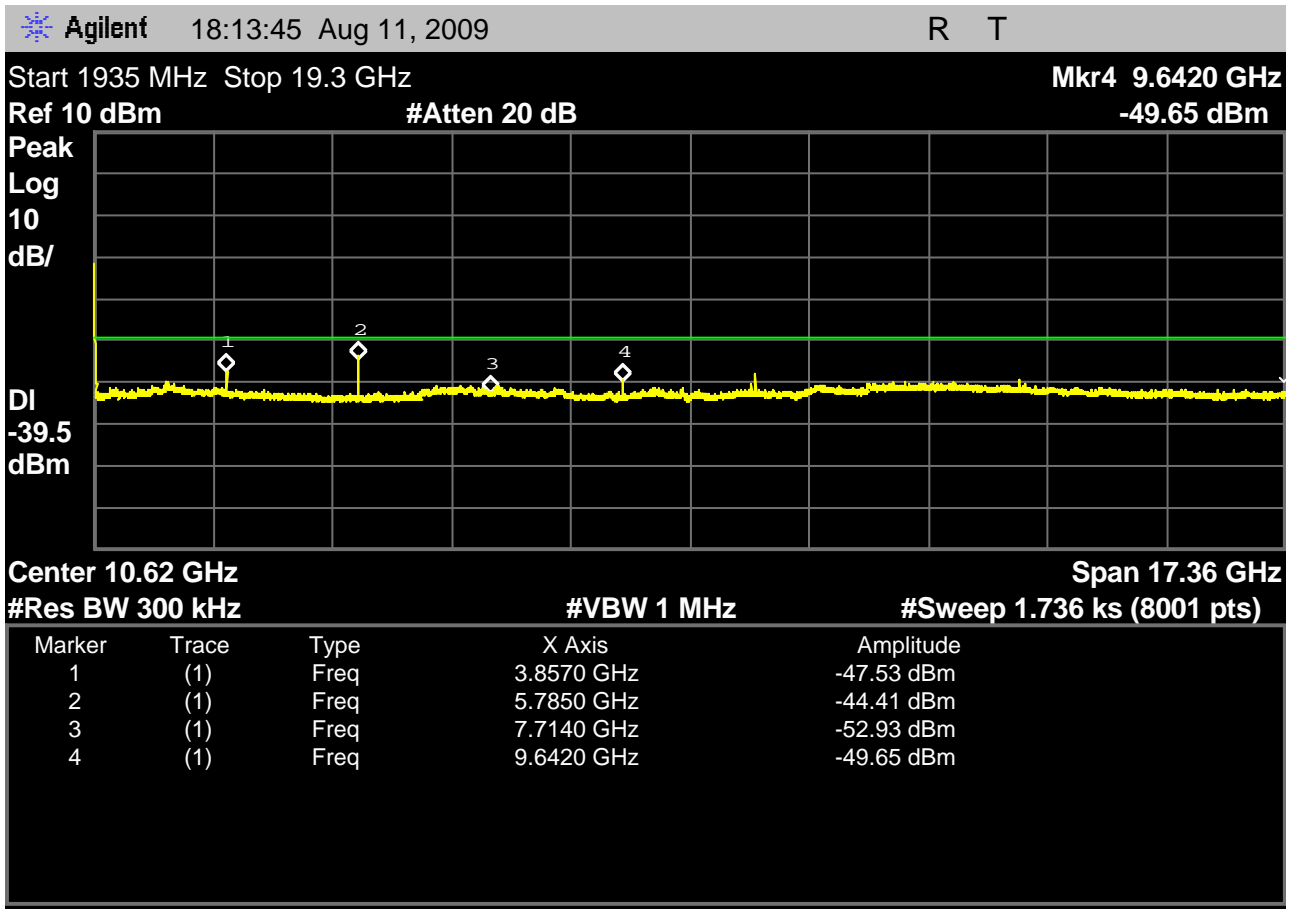
Fig. 37 – headset EUT out-of-band emissions including the regions from 1935MHz to 19.3GHz with the headset EUT transmitting on the highest carrier, 1928.448MHz.
