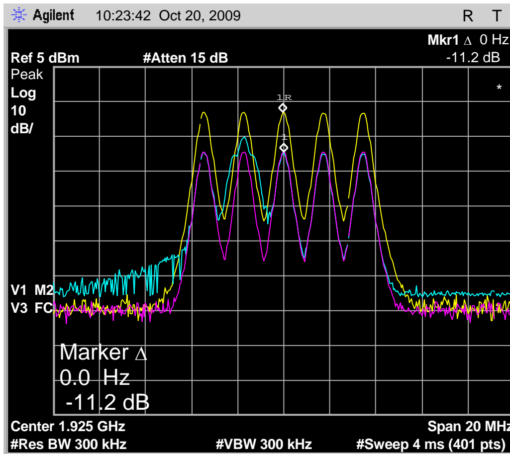
Fig. 98 - Emissions and interference profile spectrum, headset EUT, test 7.3.2.
