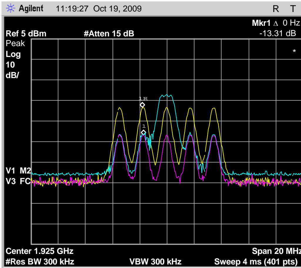
Fig. 97 - Emissions and interference profile spectrum, headset EUT, test 7.3.1 in low power WBM.
