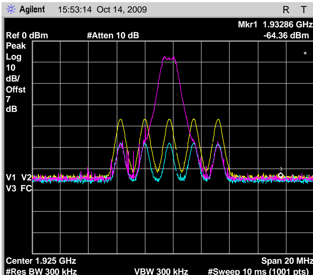
Fig. 81 - Emissions and interference profile spectrum, headset EUT, test 7.3.1 in WBM.
