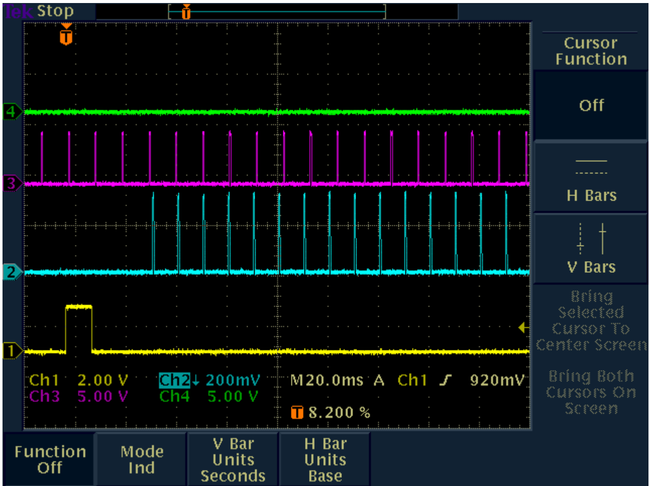
Fig. 60 - Normal initiation of transmissions by the headset EUT in the absence of over-threshold interference; the headset EUT software flags the start of the transmission setup (bottom yellow trace), and transmit emissions are recovered by the RF detector (third trace down-cyan) in the splitter/combiner network. The second trace from the top (magenta) indicates the interference profile was switched to T_U - U_M for which transmission is allowed. The top trace (green) was the T_U + U_M interference level, which prevented headset transmissions.
