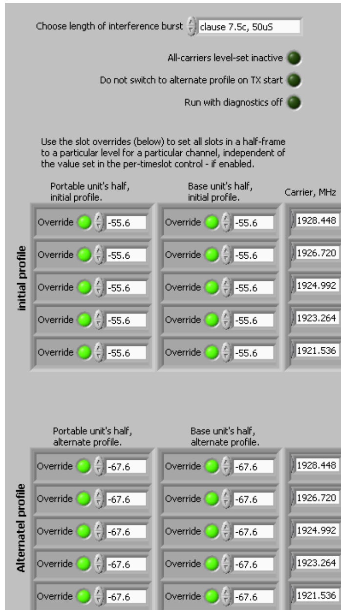
Fig. 55 - Control panel for multi-carrier interference generator, set to 50uS pulses in all timeslots on all carriers, for the test of 7.5(c).
