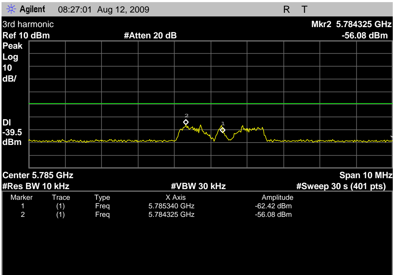
Fig. 39 – headset emissions measured in 10kHz resolution bandwidth in the region where the 1935MHz to 19.3GHz sweep at 300kHz observed a 3 rd harmonic response of -56.08dBm, for the headset transmitting on the high carrier, 1928.448MHz. A margin of greater than 15dB observed when measured in the specified resolution bandwidth.
