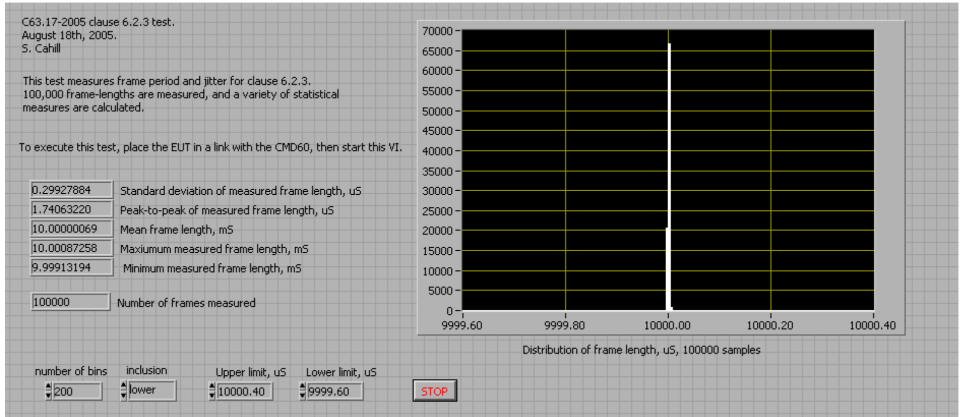
Fig. 47 - Test of headset EUT for frame period and jitter, according to the requirements of clause 6.2.3.
