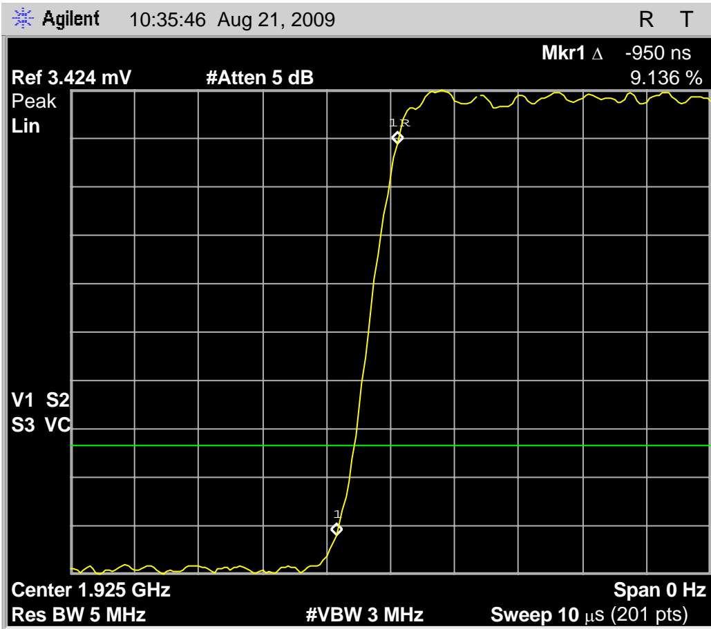
Fig. 53 - Rise time of interference pulse, per the requirements of 7.5 for less than 1uS for 10% to 90% transition.
