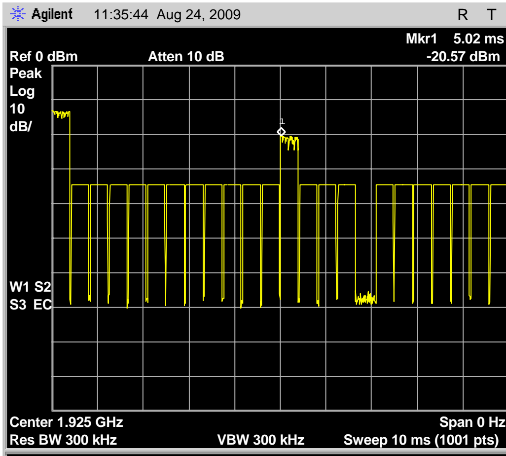
Fig. 74 – Interference profile for the Headset EUT that is above the threshold of -55.6\text{dBm} (T_U + U_M) WITH an open slot pair to demonstrate a link was possible for the test set up when 8.3.2 g) was performed.
