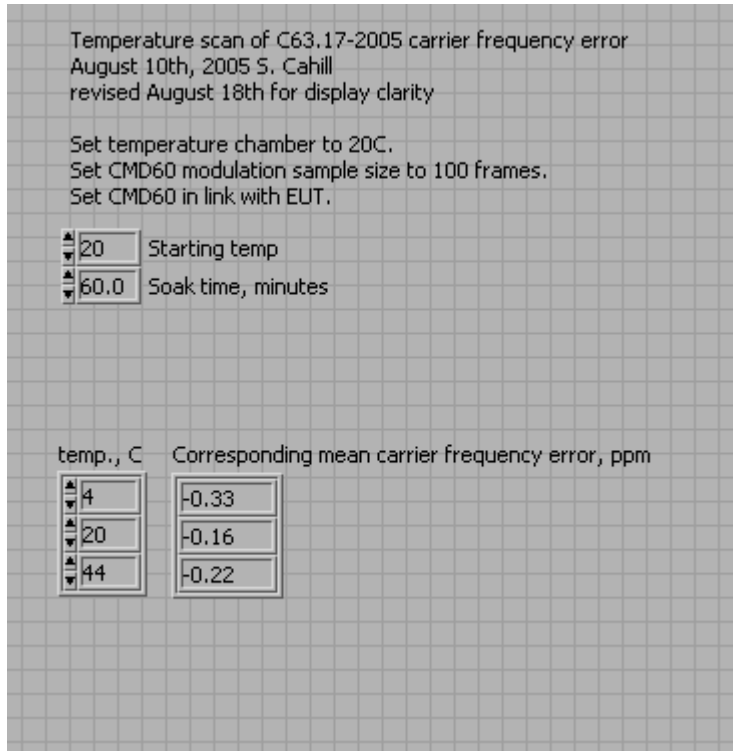
Fig. 41 - Measured mean carrier frequency, headset EUT , at +4C, +20C, +44C.
