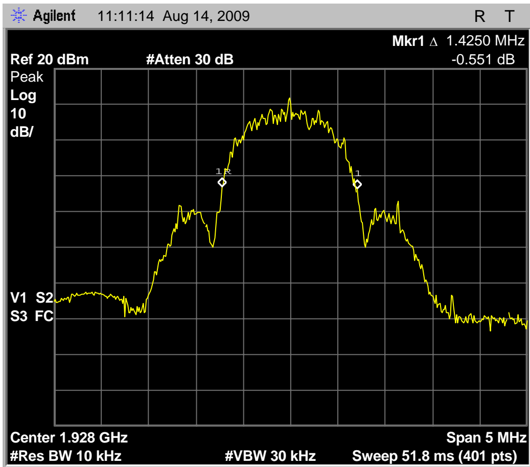
Fig. 13 - Headset EUT, 1.43MHz emissions bandwidth on high carrier.
