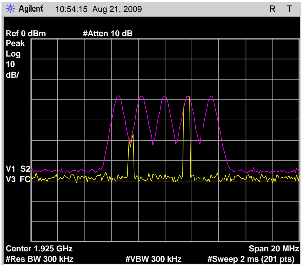
Fig. 59 - Transmit spectrum of 35uS interference pulses in each timeslot for each carrier, with headset EUT deferring due to interference pulses of T_U + U_M + 6\text{dB} .
