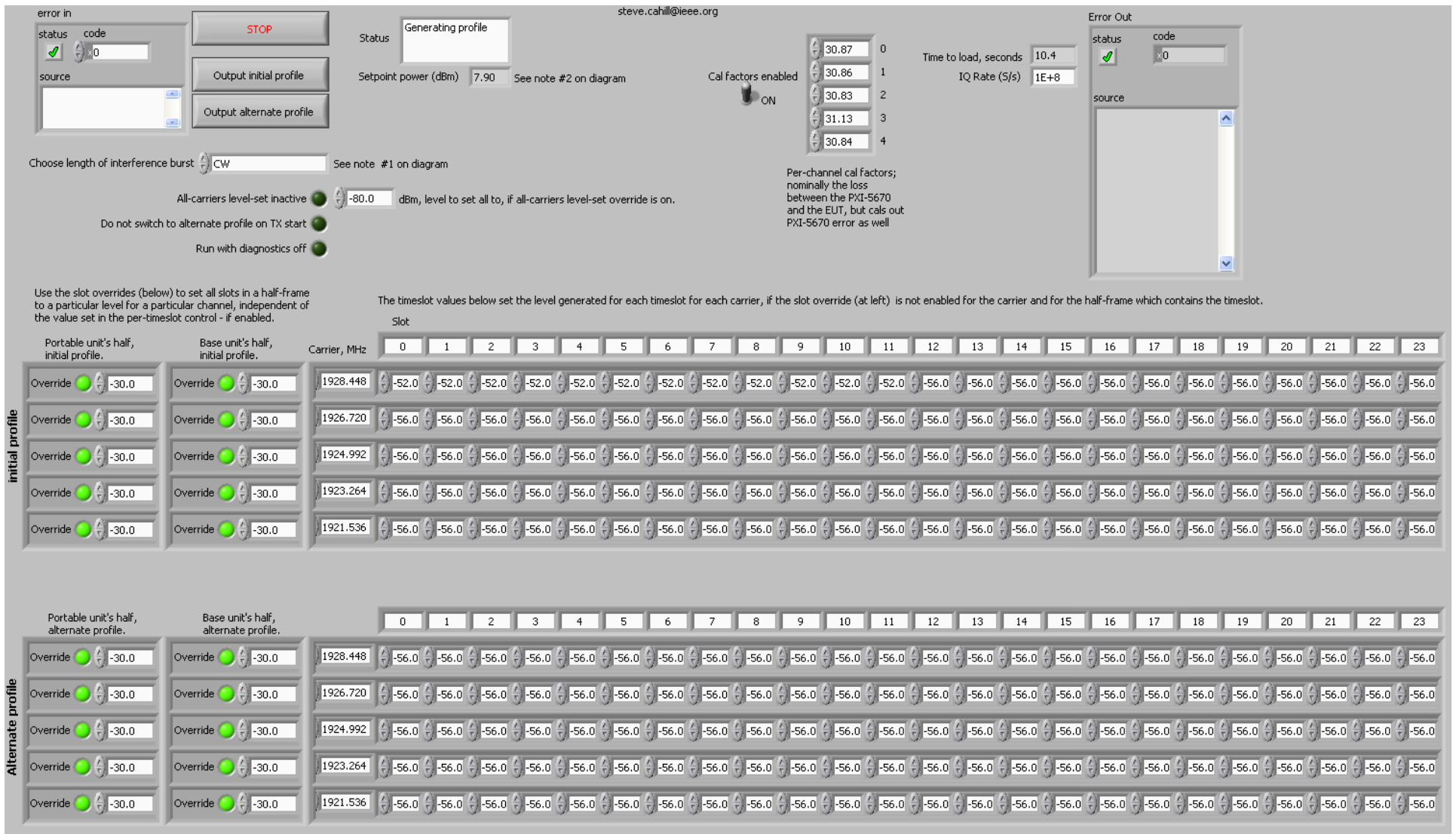
Fig. 5 - Screenshot of control VI for PXI-5670 taken with all carriers enabled, for -30dBm calibration accuracy test.
