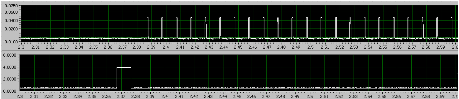
Fig. 87 - Normal initiation of transmissions by the headset EUT in the absence of over-threshold interference; the headset EUT software flags the start of the transmission setup (bottom trace) at t = 2.36 seconds, and transmit emissions are recovered by the RF detector (top trace) in the splitter/combiner network beginning at t = 2.38 seconds. Proper transmission at T_L - U_M is shown, to validate functionality and to illustrate the getting-ready-to-transmit marker, and the RF detector output.
