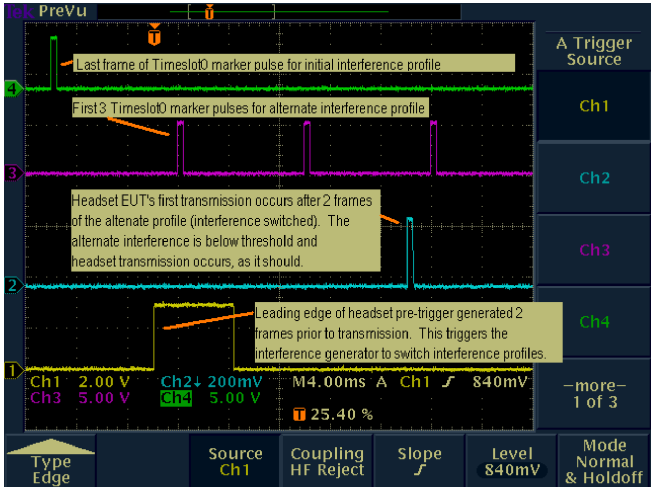
Fig. 52 - Example oscilloscope screenshot showing transition from initial to alternate interference profile in the frame before headset EUT initiation of transmission of the communications channel; for this example the alternate interference profile is configured to meet the access criteria. The text of the notes is best viewed at 150% magnification.
