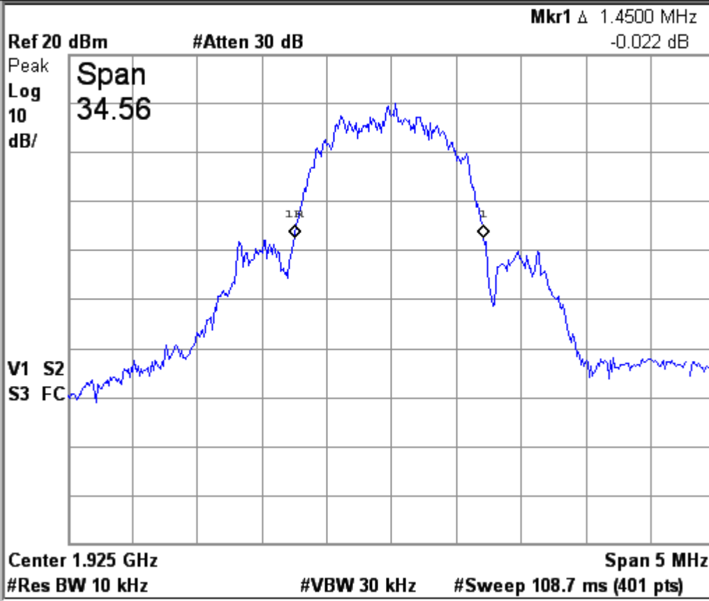
Fig. 12 - Headset EUT, 1.45MHz emissions bandwidth on middle carrier.
