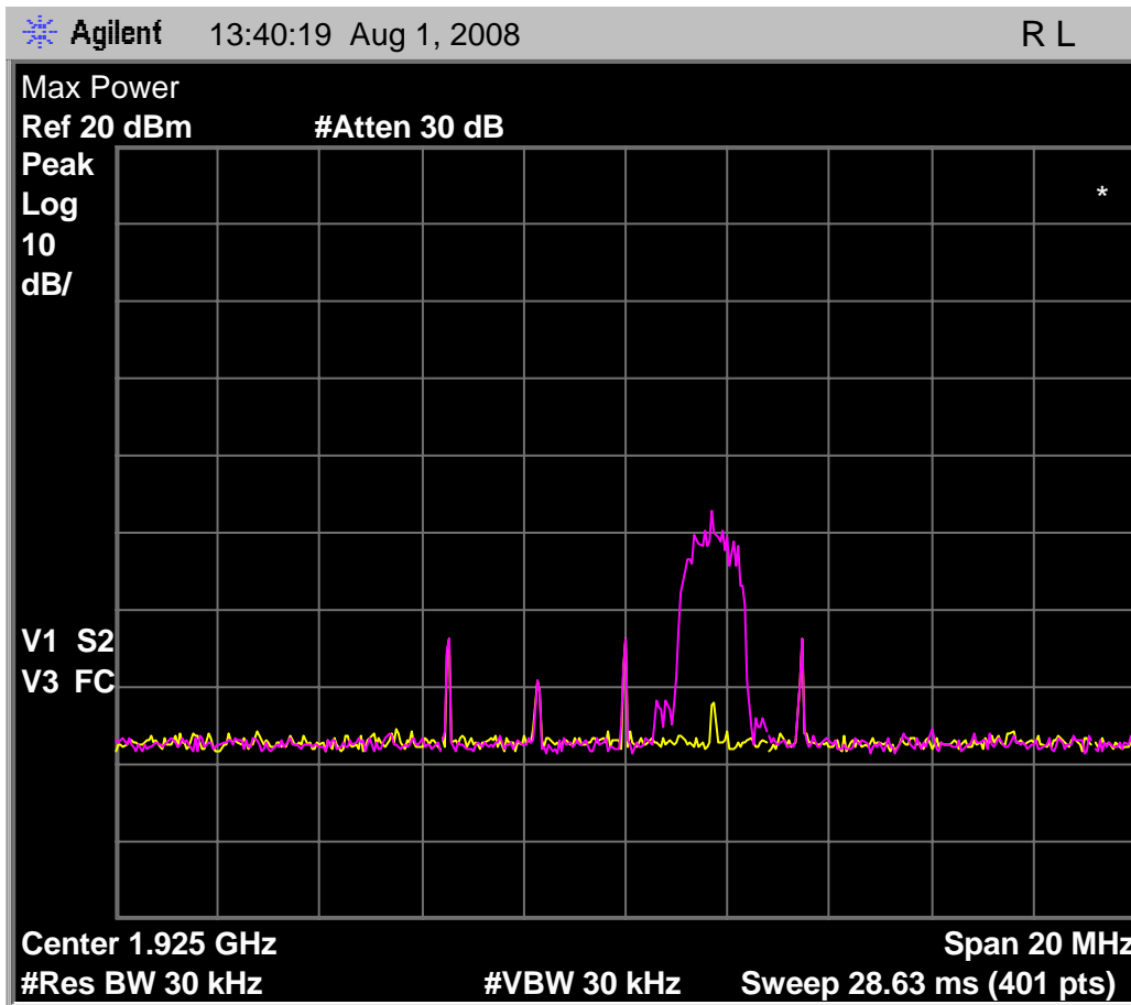
Fig. 85 - Emissions and interference profile spectrum, headset EUT, test 7.3.3(c).
