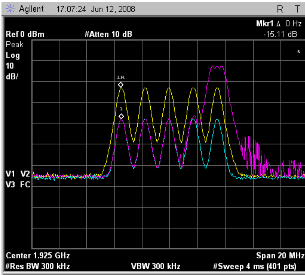
Fig. 47 - Emissions and interference profile spectrum, headset EUT, test 7.3.2.
