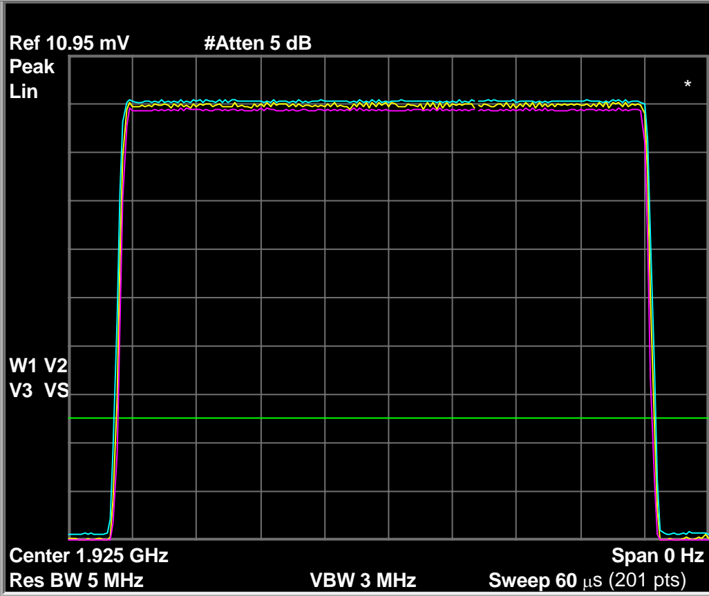
Fig. 57 – 50uS interference pulse for 7.5(c), duration and amplitude variation over the duration of the 50 uS pulse and over multiple pulses. Spectrum analyzer is set to linear response.
