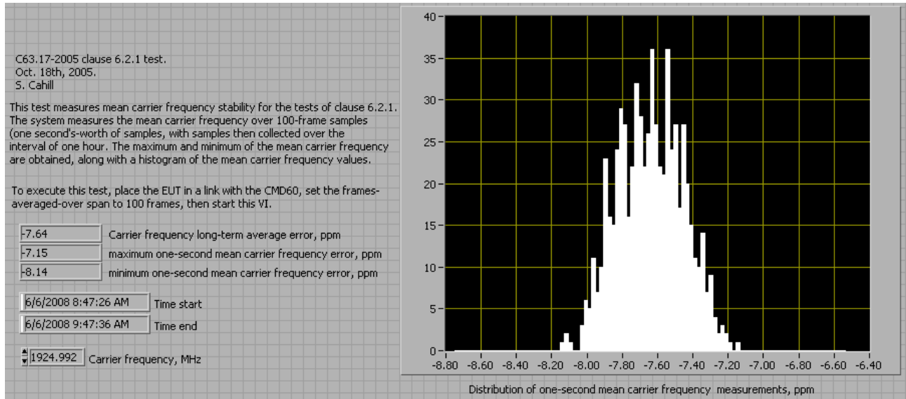
Fig. 43 - Measured one-second mean carrier frequency, headset EUT, and observed maximum, average value and observed minimum of the mean carrier frequency.
