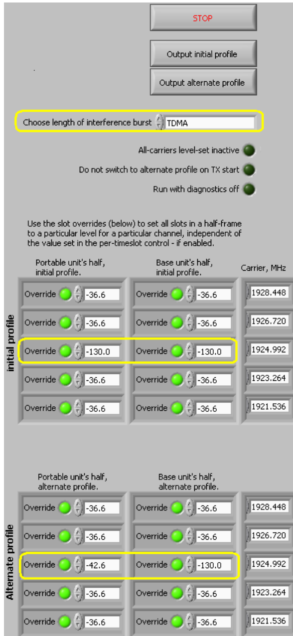
Fig. 70 - PXI-5670 multi-carrier interference generator control panel for the test of 8.2.1(c), for the headset EUT.
