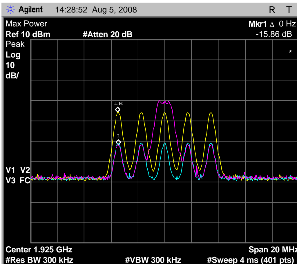
Fig. 99 - Emissions and interference profile spectrum, headset EUT, test 7.3.1 in low power WBM.
