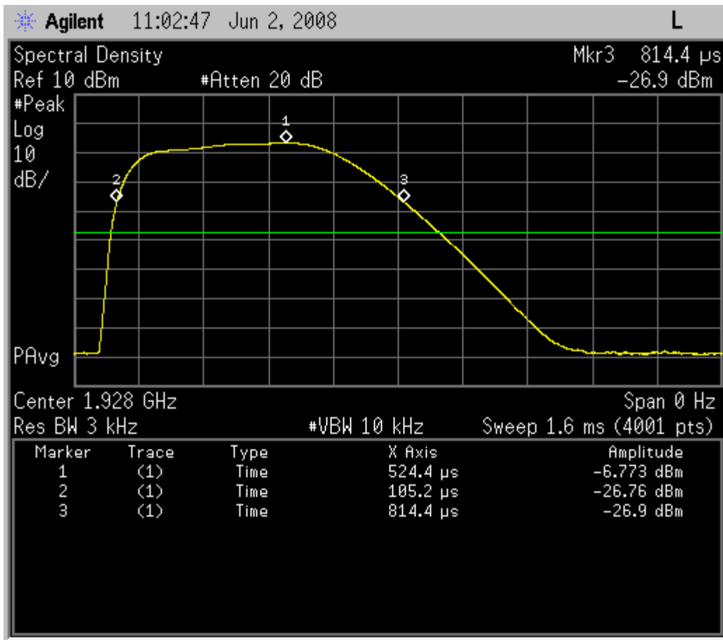
Fig. 18 – Zero-span sweep for headset EUT, high carrier, for 3kHz maximum power spectral density. The peak level is at -6.773dBm, and the interval between samples at the -20dB points is from 105.2us to 814.4us, or 709.2us.
