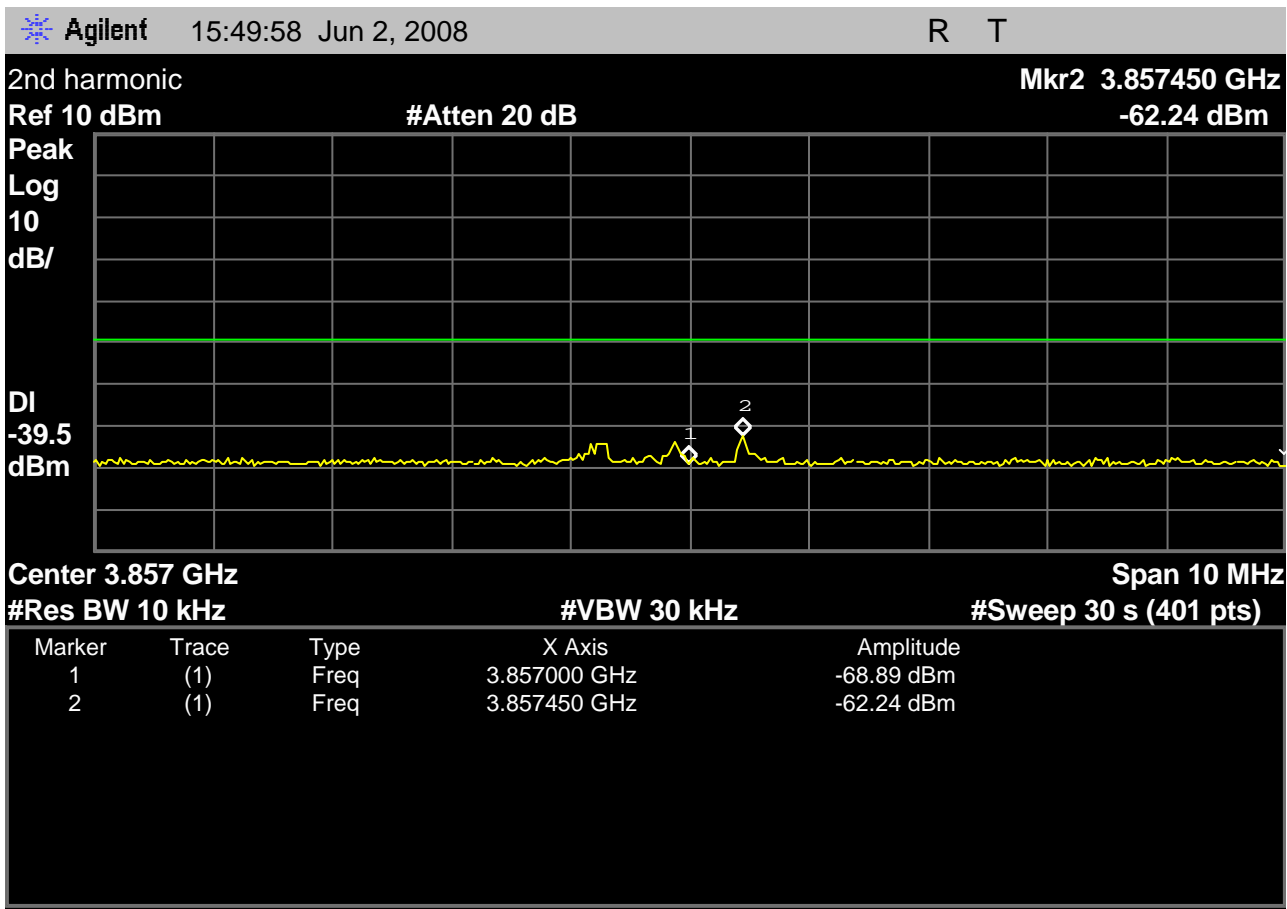
Fig. 37 – headset emissions measured in 10kHz resolution bandwidth in the region where the 1935MHz to 19.3GHz sweep at 300kHz observed a 2 nd harmonic response, for the headset transmitting on the high carrier, 1928.448MHz. A peak of -62.24dBm is measured in the specified resolution bandwidth, a margin of 22.7dB from the -39.5dBm spec limit.
