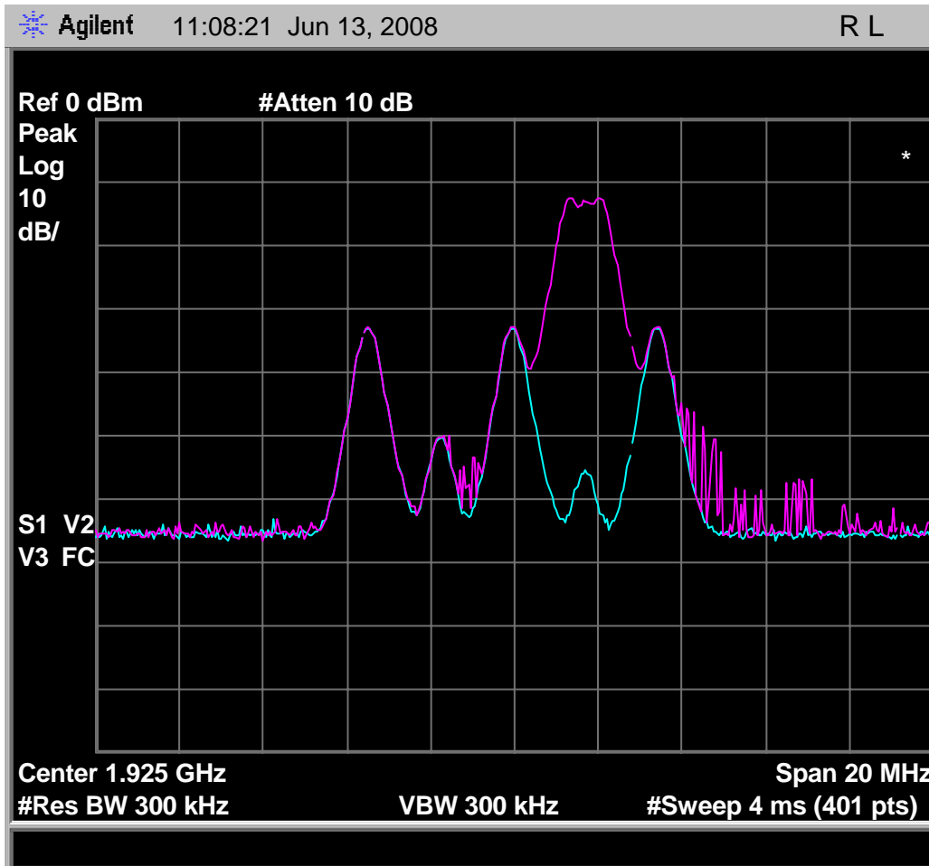
Fig. 51 - Emissions and interference profile spectrum, headset EUT, test 7.3.3(e).
