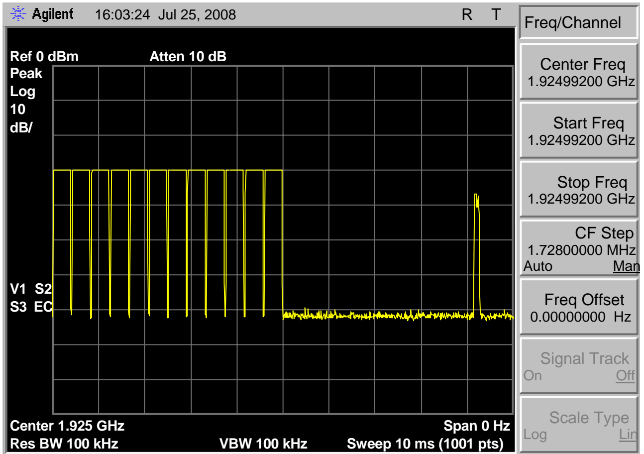
Fig. 65 - One frame of transmissions for a headset EUT and base companion device with a beacon present, interference present and high enough to block headset-to-base communications. Slots 0 – 11 have the interference present and slot 20 has the base companion device transmit beacon signal.
