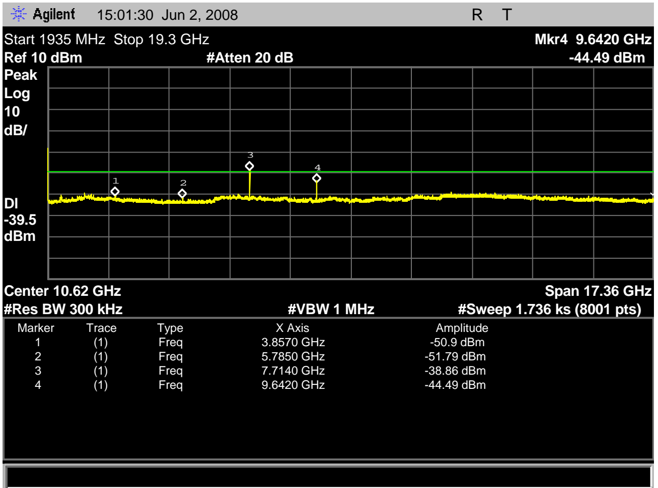
Fig. 36 – headset EUT out-of-band emissions including the regions from 1935MHz to 19.3GHz with the headset EUT transmitting on the highest carrier, 1928.448MHz.
