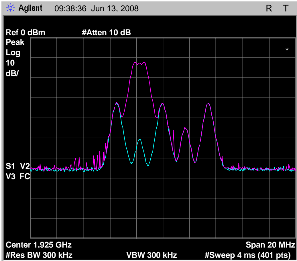
Fig. 48 - Emissions and interference profile spectrum, headset EUT, test 7.3.3(b).
