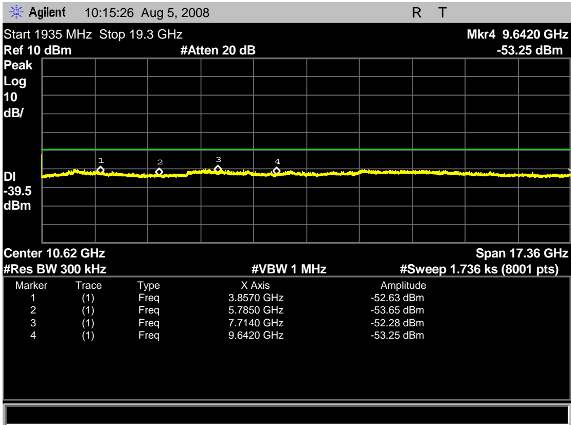
Fig. 98 - Headset EUT in minimum power WBM on high carrier, harmonics all below the noise floor in minimum power mode, unlike harmonic level with headset EUT configured for maximum output power, see section 6.1 of main report.
