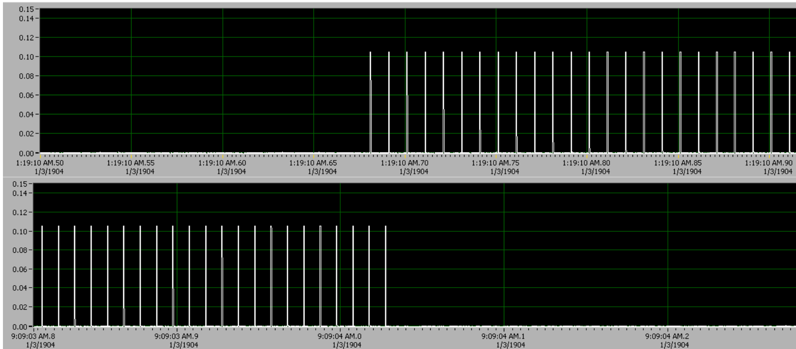
Fig. 73 - RF detector output showing timed initiation of headset EUT transmissions (top trace), then termination (bottom trace) when the headset EUT finds no channels passing the access criteria test. The headset EUT terminates transmissions at 9:09:04 (hour:min:sec), which was 7 hours and 50 minutes from the link initiation time of 1:19:10, so meeting the requirement of 8.2.2 that the headset execute the access criteria test at least as often as every 28800 seconds (or every 8 hours).
