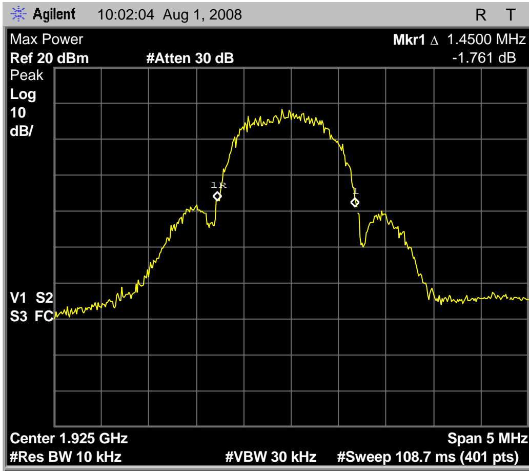
Fig. 82 - headset EUT in WBM, 1.45MHz emissions bandwidth on mid carrier; same results as in normal mode operation.
