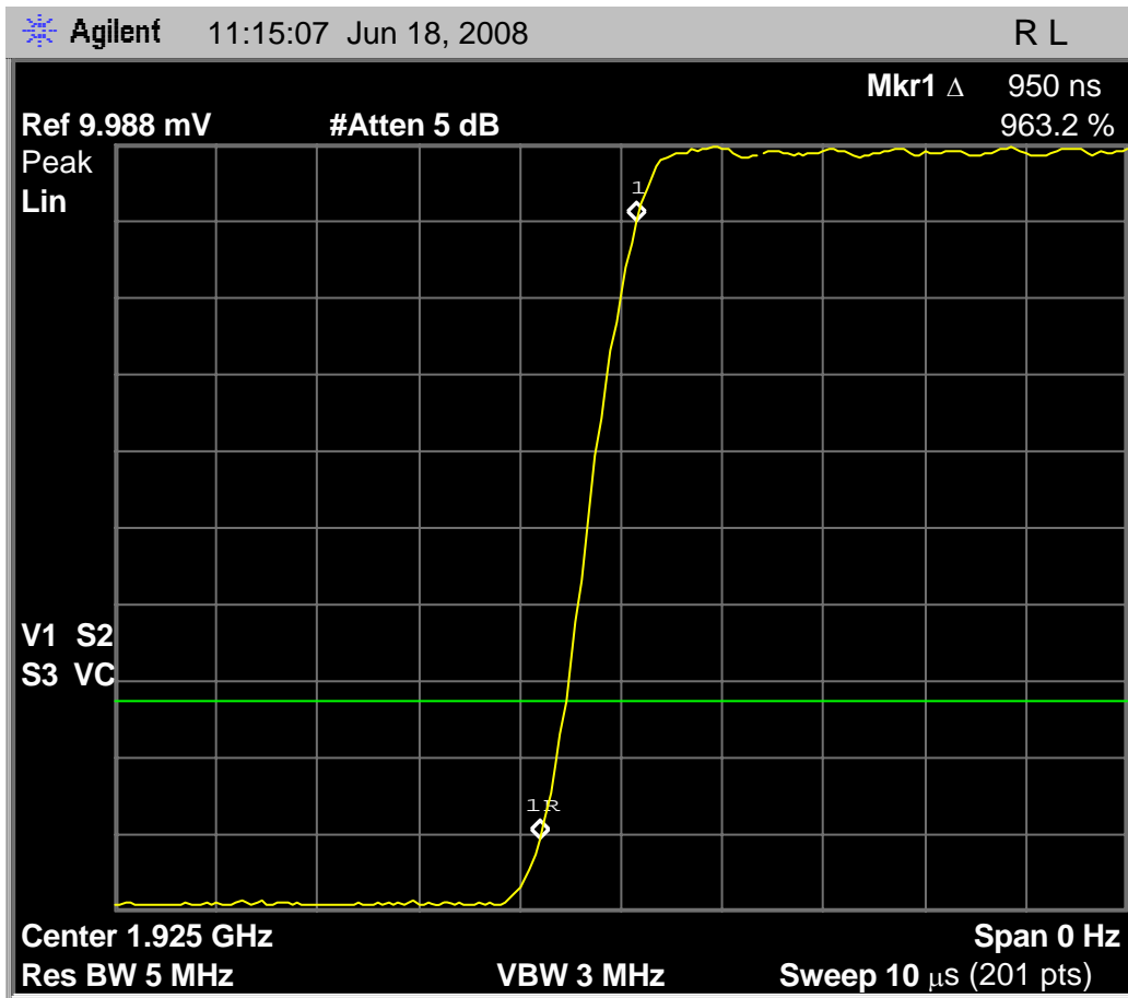
Fig. 56 - Rise time of interference pulse, per the requirements of 7.5 for less than 1uS for 10% to 90% transition.
