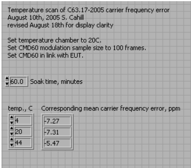
Fig. 44 - Measured mean carrier frequency, headset EUT , at +4C, +20C, +44C.
