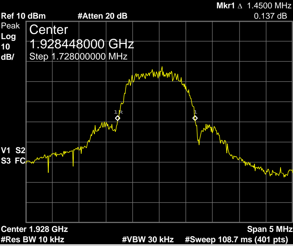
Fig. 96 - Headset EUT in WBM, 1.45MHz emissions bandwidth on high carrier vs. 1.44MHz in normal mode high power.
