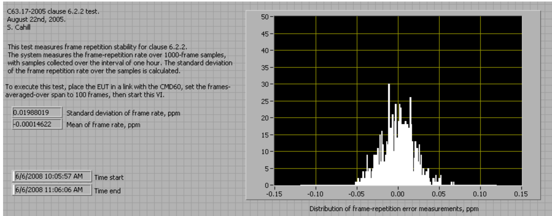
Fig. 45 - Test of headset EUT according to the conditions of clause 6.2.2 for frame repetition rate stability
