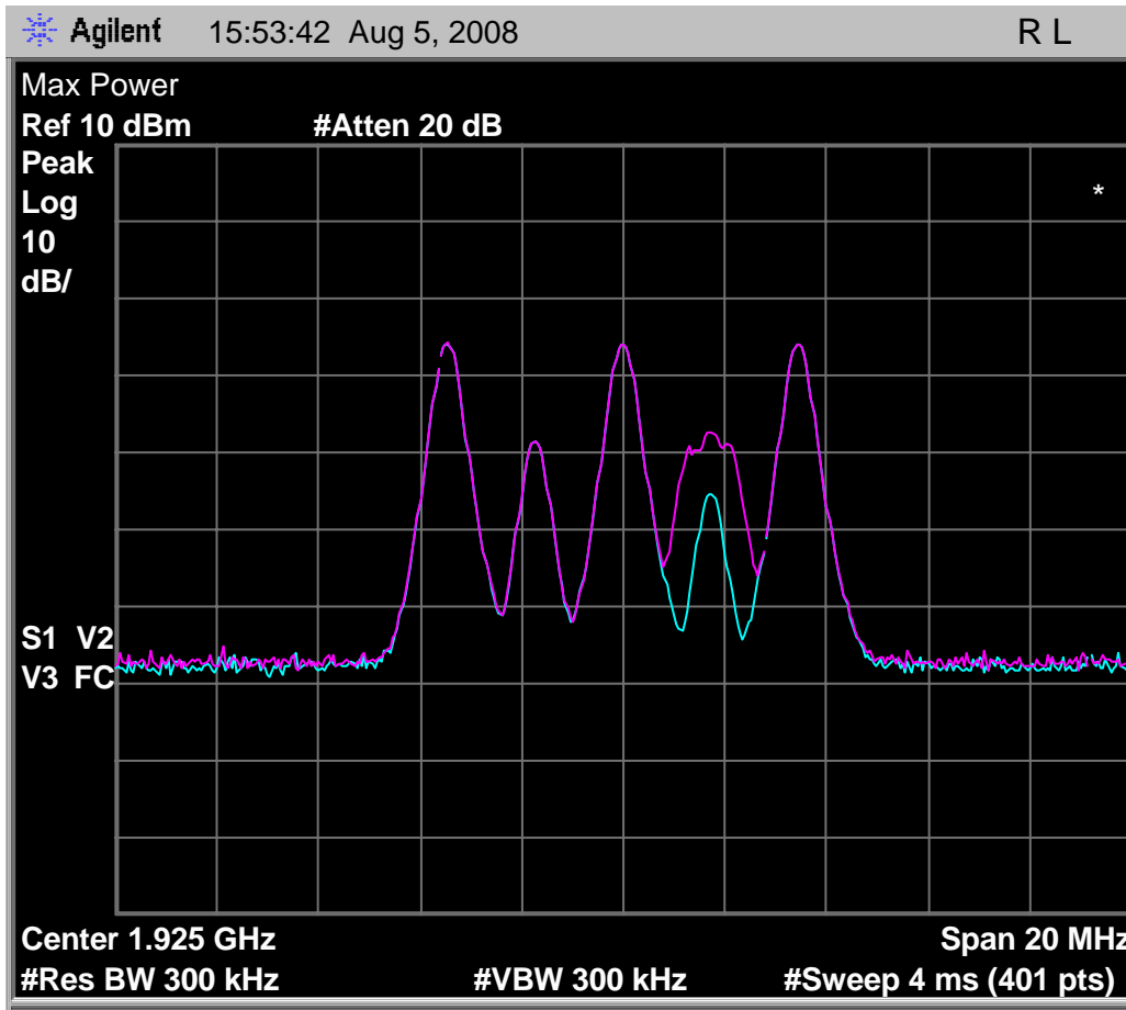
Fig. 102 - Emissions and interference profile spectrum, headset EUT, test 7.3.3(c).
