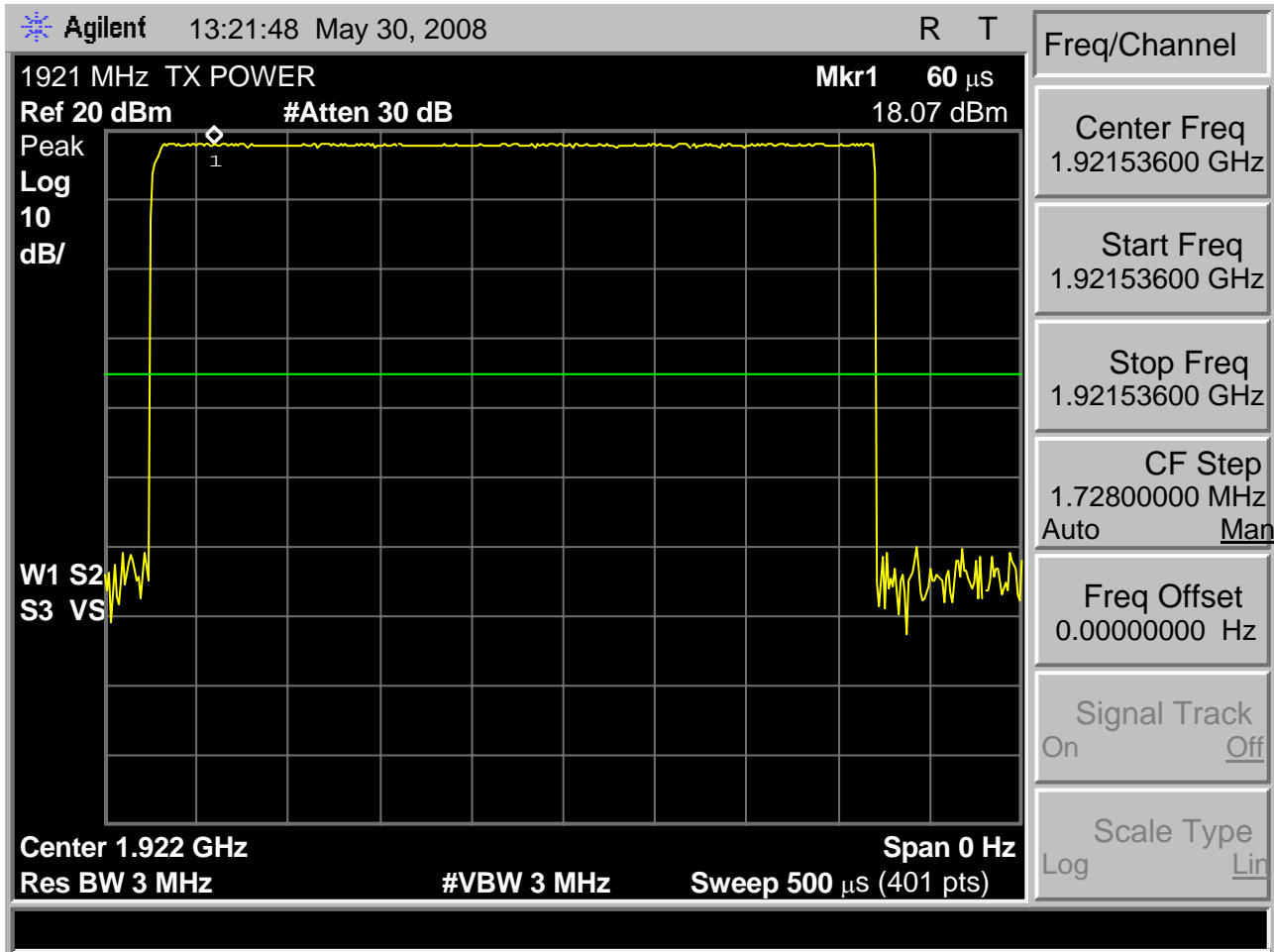
Fig. 8 - Headset EUT transmit power received by spectrum analyzer configured according to the requirements of clause 6.1.2 of C63.17-2006, low carrier. Maximum observed transmit power is 18.07 dBm.
