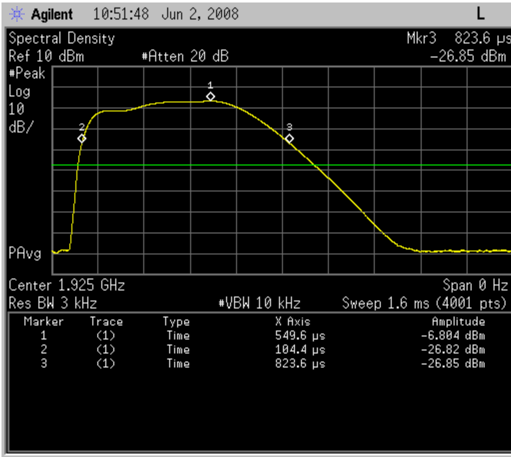
Fig. 16 – Zero-span sweep for headset EUT, middle carrier, for 3kHz maximum power spectral density. The peak level is at -6.804dBm, and the interval between samples at the -20dB points spans 104.4us to 823.6us, or 719.2us.
