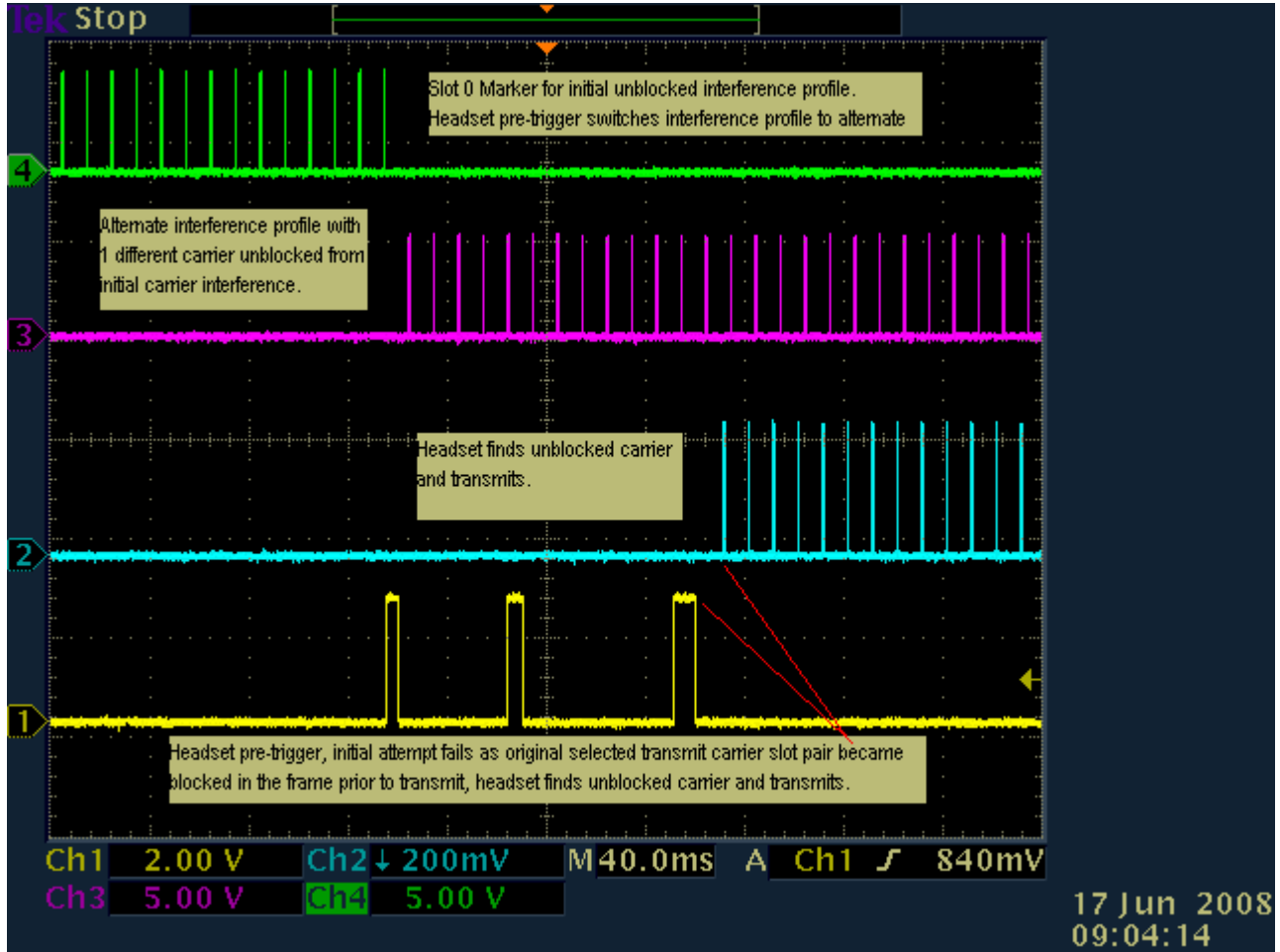
Fig. 53 - Screen shot of oscilloscope showing deferral by the headset EUT in the case where the interference profile changes in the frame previous to intended transmission and the selected time and frequency communications channel becomes blocked; and then later, transmission on unblocked channel.
