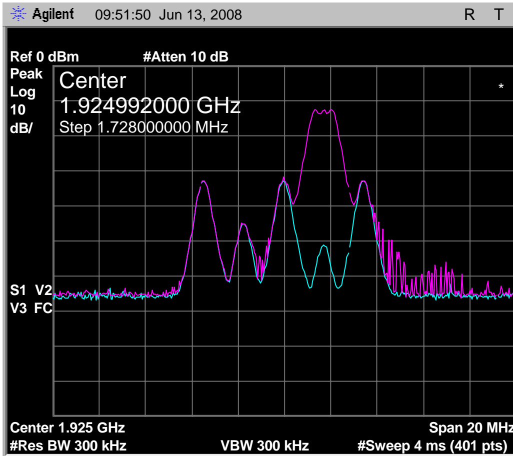
Fig. 49 - Emissions and interference profile spectrum, headset EUT, test 7.3.3(c).
