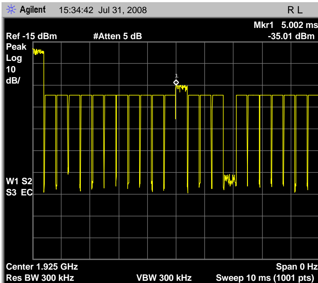
Fig. 79 – Interference profile for the Headset EUT that is above the threshold of -54.6\text{dBm} ( T_U + U_M ) WITH an open slot pair to demonstrate a link was possible for the test set up when 8.3.2 g) was performed.
