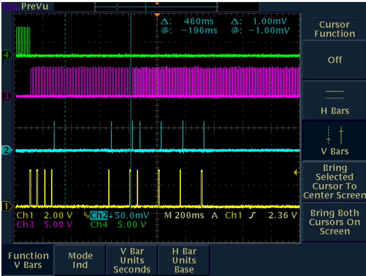
Fig. 67 - Screenshot zoom of the above oscilloscope screen capture. Ten attempts to bring up a link were attempted by the headset, none had a successful acknowledgement from the Base; since the Base never heard the headset's request due to the alternate interference level in the headset transmit half of the frames.
