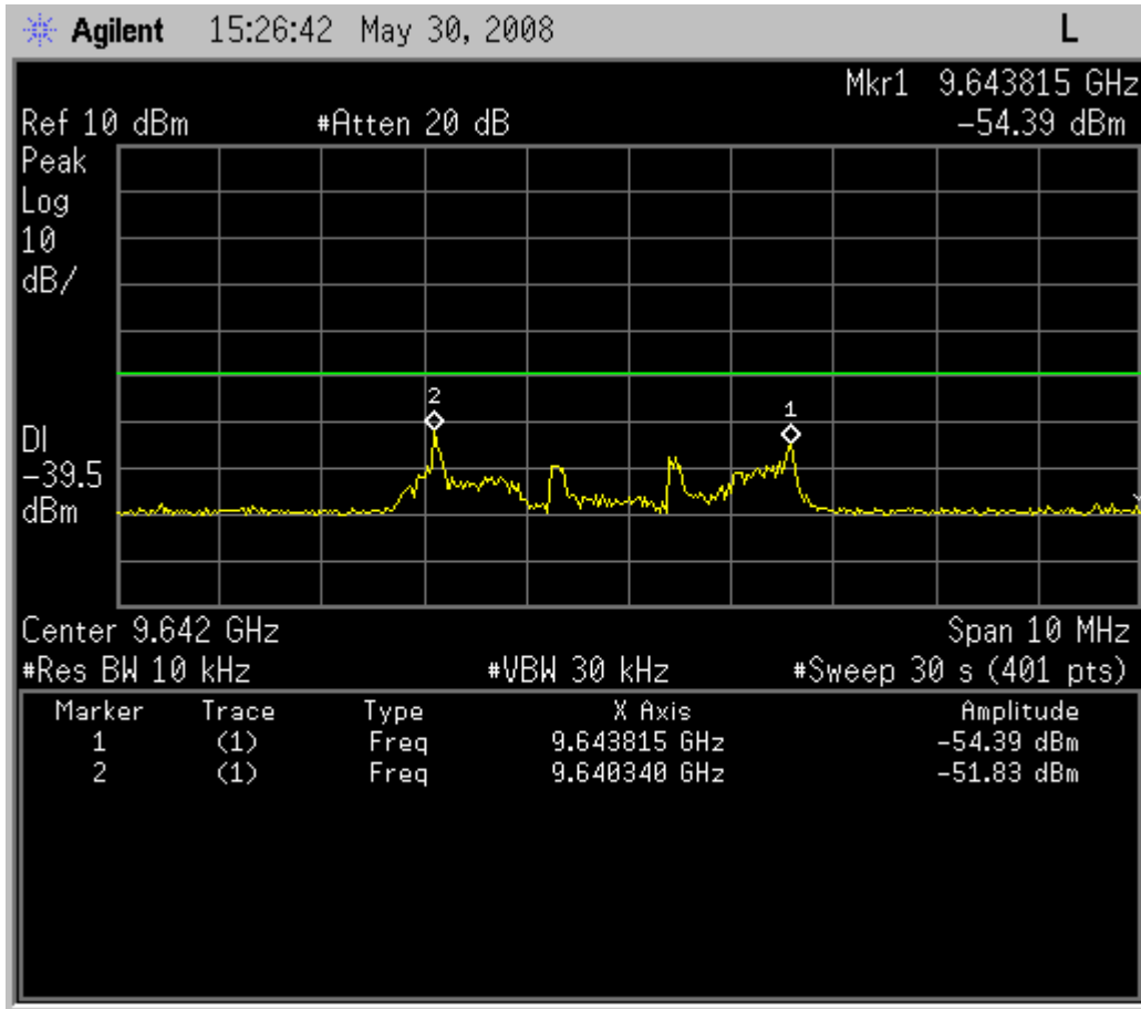
Fig. 40 – headset EUT out-of-band emissions in the region around the 5 th harmonic, with the headset EUT transmitting on the highest carrier, 1928.448MHz.
