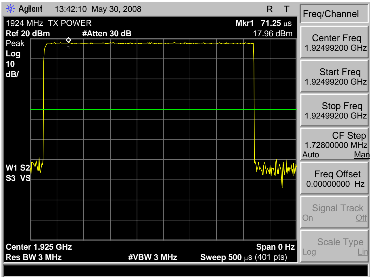
Fig. 9 - Headset EUT transmit power received by spectrum analyzer configured according to the requirements of clause 6.1.2 of C63.17-2006, mid carrier. Maximum observed transmit power is 17.96 dBm
