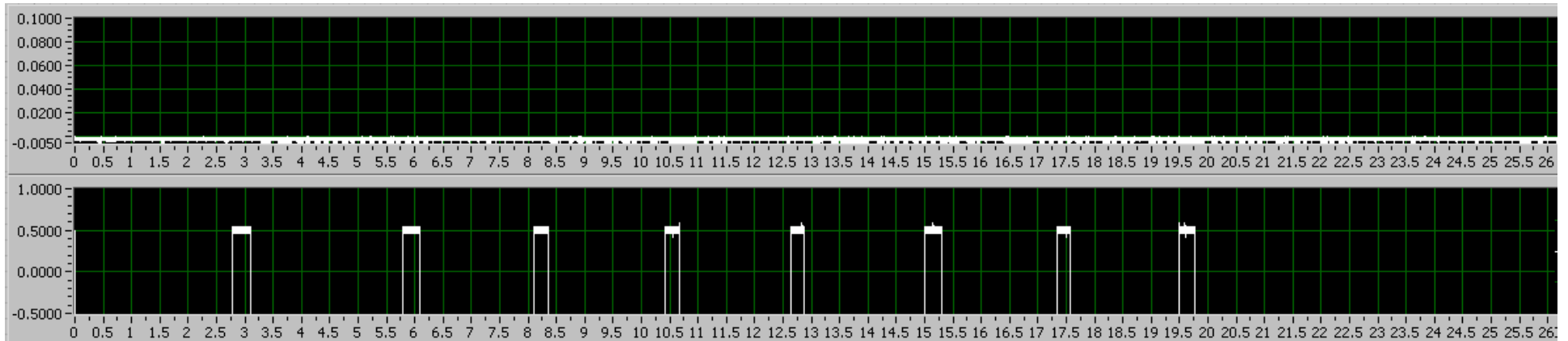
Fig. 58 - Headset EUT shown deferring when all channels are blocked with 50uS pulses at T_U + U_M . Top trace is detected RF transmissions (no transmissions are detected), bottom trace is headset EUT transmission setup attempt series (as indicated by the software flag for getting-ready-to-transmit attempts) in response to the press of the TALK button, with each pulse of the software transmission-attempt flag then not being followed by the transmissions, due to the access criteria check failure.
