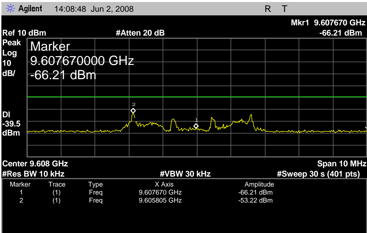
Fig. 31 – headset EUT out-of-band emissions in the region around the 5th harmonic, with the headset EUT transmitting on the lowest carrier, 1921.536MHz.
