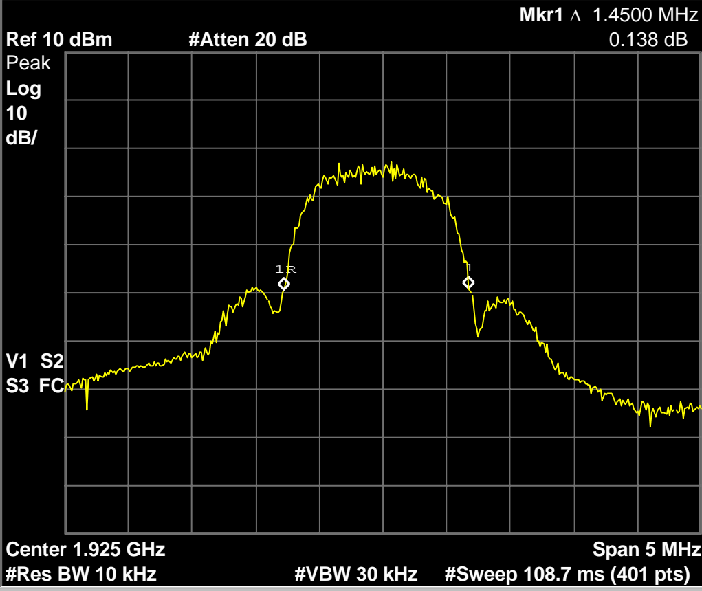
Fig. 95 - Headset EUT in WBM, 1.45MHz emissions bandwidth on mid carrier vs. 1.45MHz in normal mode high power.
