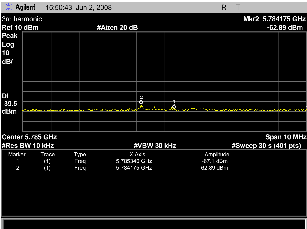
Fig. 38 – headset emissions measured in 10kHz resolution bandwidth in the region where the 1935MHz to 19.3GHz sweep at 300kHz observed a 3 rd harmonic response, for the headset transmitting on the high carrier, 1928.448MHz. A margin of greater than 20dB observed when measured in the specified resolution bandwidth.
