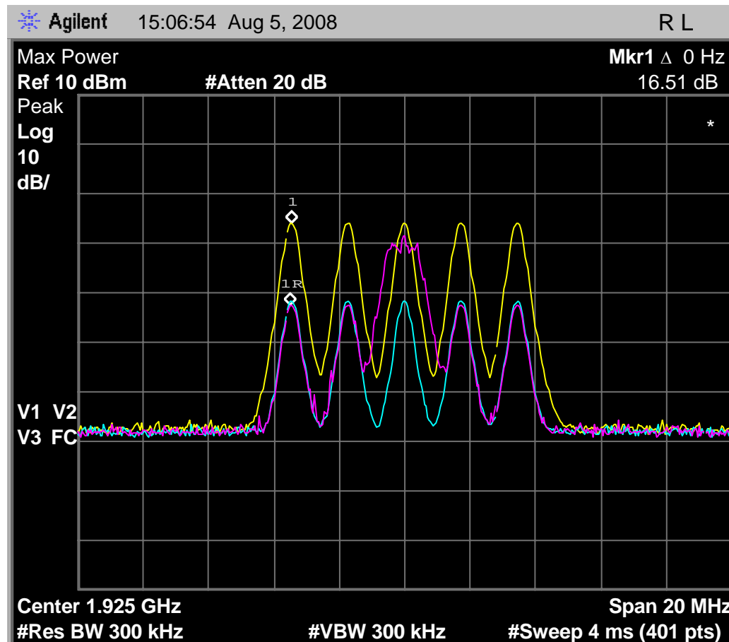
Fig. 100 - Emissions and interference profile spectrum, headset EUT, test 7.3.2.
