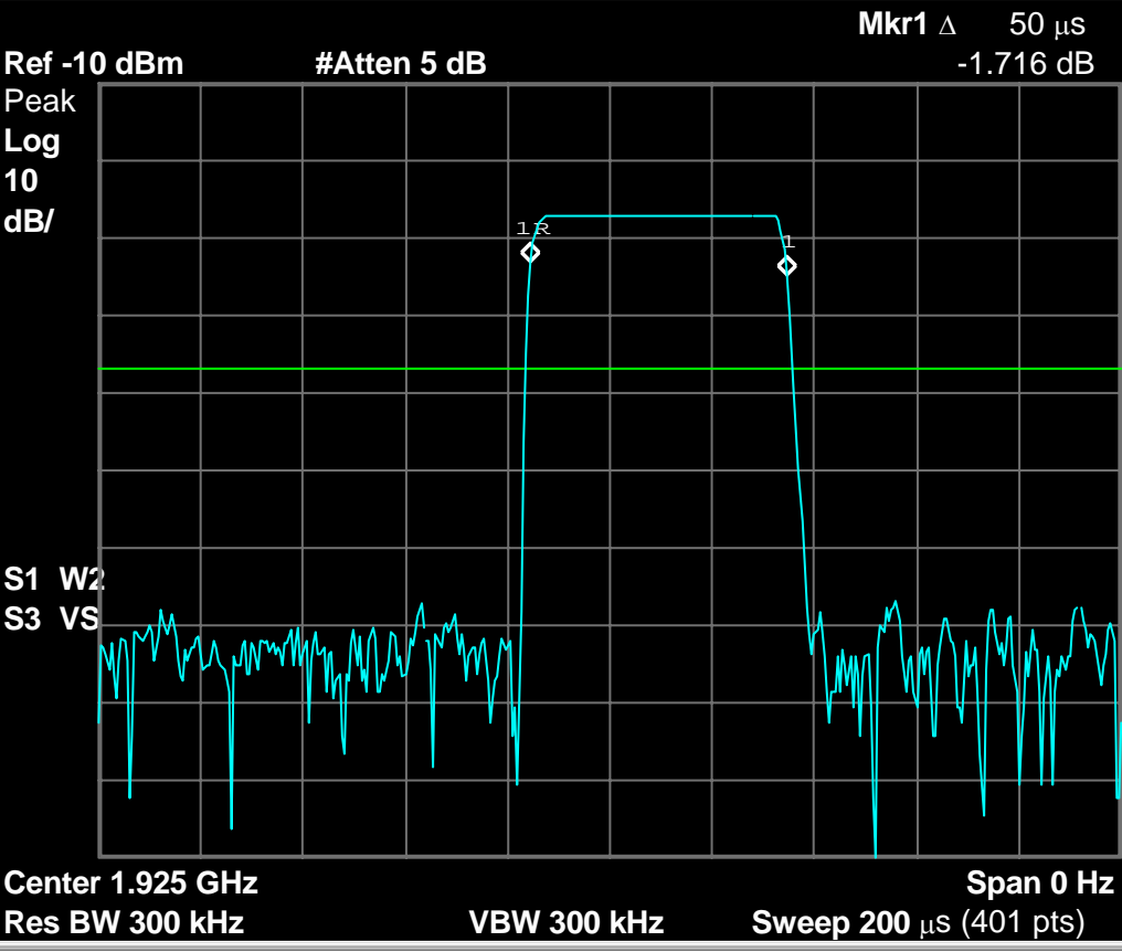
Fig. 55 - Interference pulse, one frame shown, for the test of 7.5(c).
