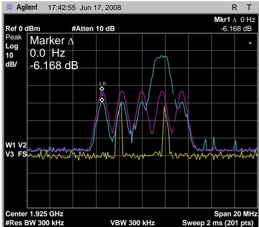
Fig. 59 - Transmit spectrum of 50uS interference pulses, with headset EUT no longer deferring with interference pulses of level T_U - U_M .
