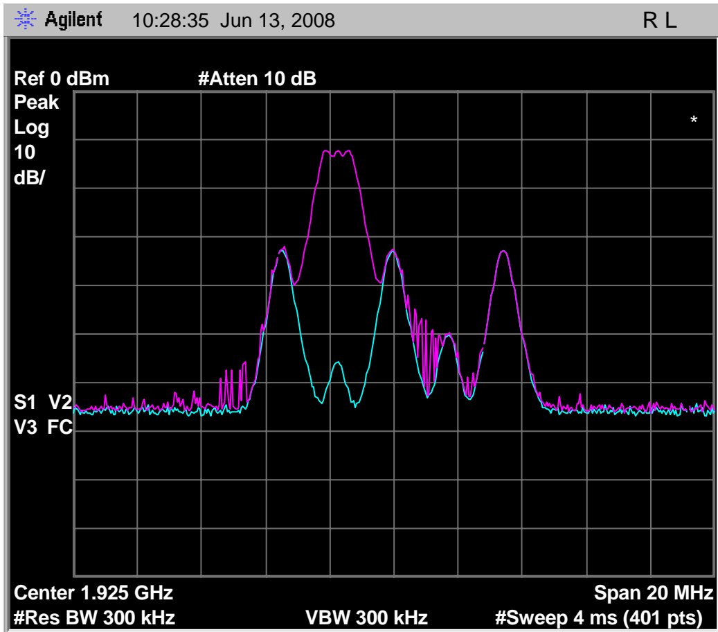
Fig. 50 - Emissions and interference profile spectrum, headset EUT, test 7.3.3(d).
