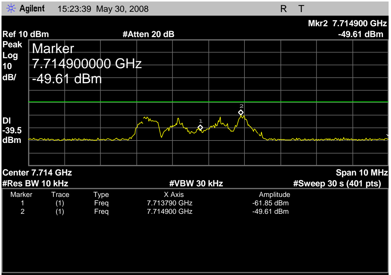
Fig. 39 – headset EUT out-of-band emissions in the region around the 4 th harmonic, with the headset EUT transmitting on the highest carrier, 1928.448MHz.
