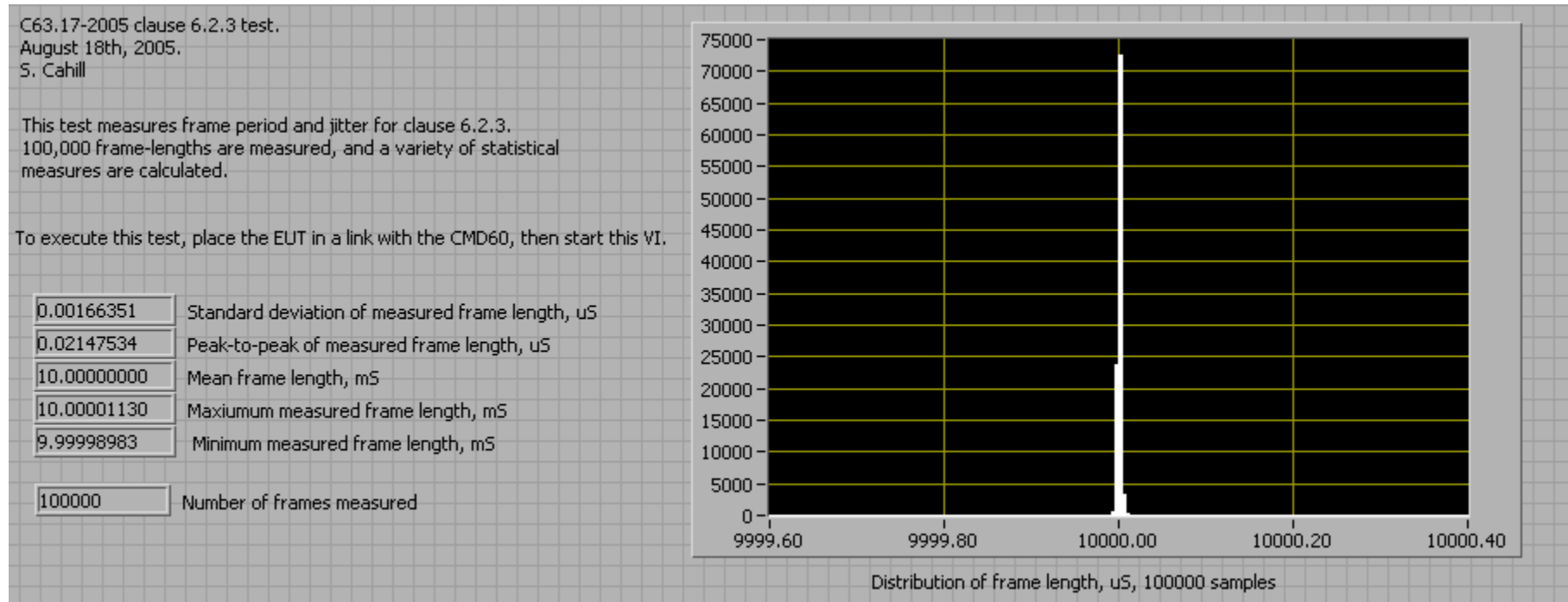
Fig. 46 - Test of headset EUT for frame period and jitter, according to the requirements of clause 6.2.3.
