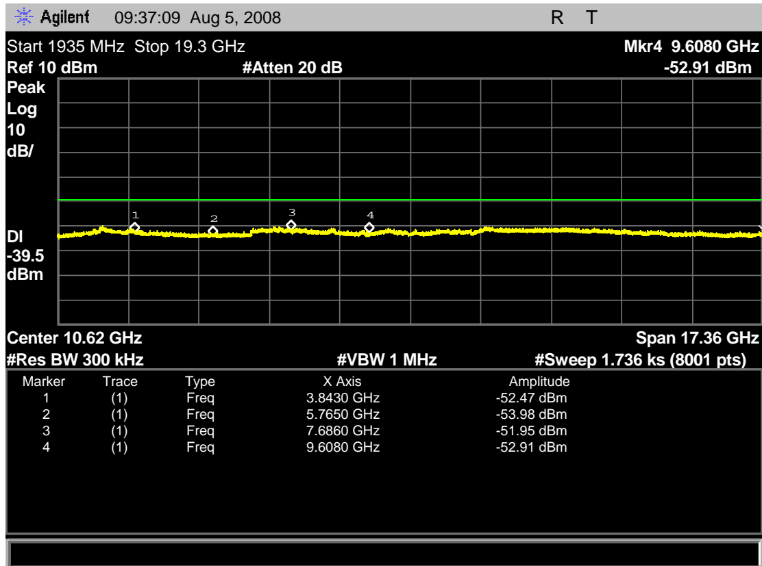
Fig. 97 - Headset EUT in minimum power WBM on low carrier, harmonics all below the noise floor in minimum power mode, unlike harmonic level with headset EUT configured for maximum output power.
