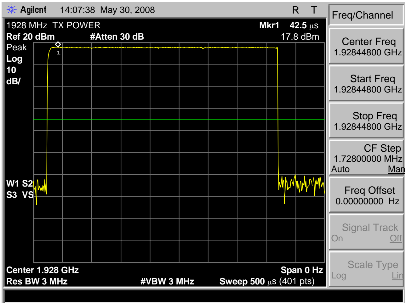
Fig. 10 - Headset EUT transmit power received by spectrum analyzer configured according to the requirements of clause 6.1.2 of C63.17-2006, high carrier. Maximum observed transmit power is 17.80 dBm.
