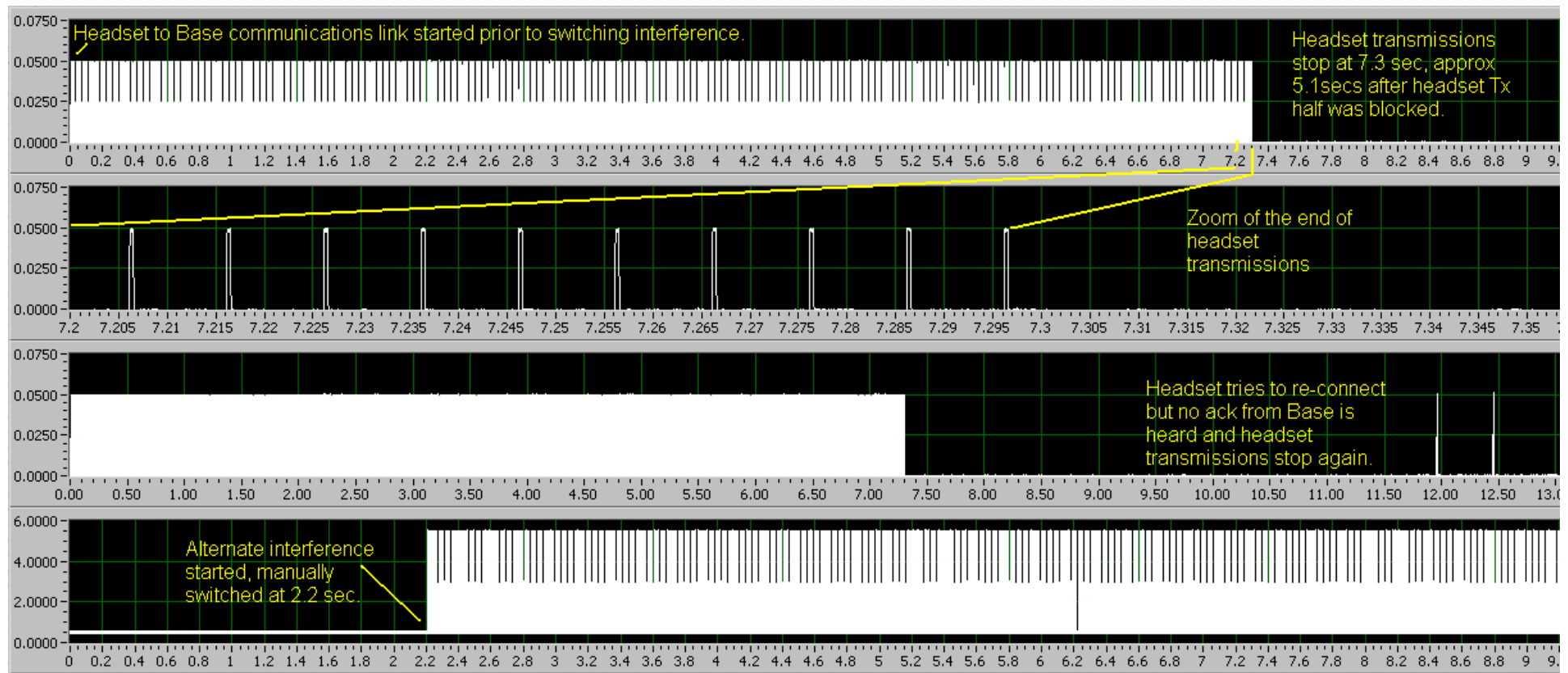
Fig. 71 - RF detector (top three traces) and alternate interference output (bottom trace) as headset EUT transmission goes blocked and transmissions stop.
