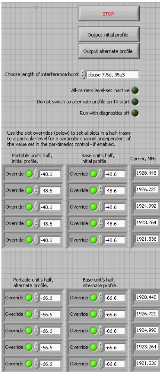
Fig. 61 - The control panel for the multi-carrier interference generator configured to make the interference profile required for 7.5(d).
