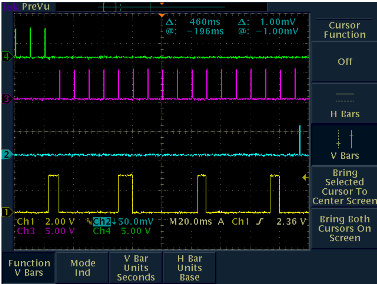
Fig. 68 – Further screenshot zoom of the above 2 figures. This screen capture shows that the first actual attempt to transmit a signal from the headset to the Base wasn't until the fourth attempt. The first 3 attempts Ch1 (yellow) trace have no corresponding RF output Ch2 (cyan) trace. The first attempt correctly recognizes that the interference level had changed and thus no RF transmission from Base to headset takes place, and the following two pulses on Ch1 also do not transmit as the RSSI (receive strength indicator) value is too large of a change, by the fourth Ch1 pulse the receiver has re-scanned the frequency time slots and found an acceptable (unblocked, and no large RSSI change) place to transmit.
