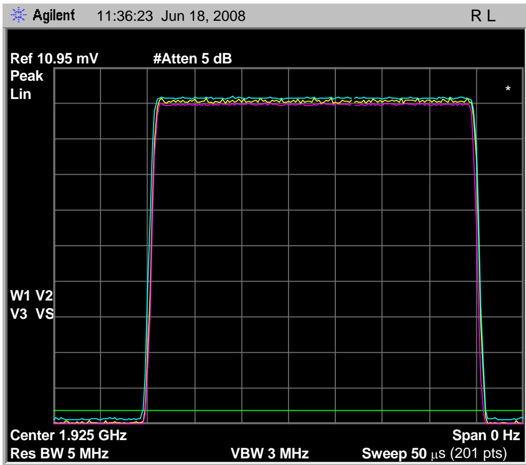
Fig. 62 - 35uS interference pulse for 7.5(d), duration and amplitude variation over the duration of the pulse and over multiple pulses. Spectrum analyzer is set to linear response.
