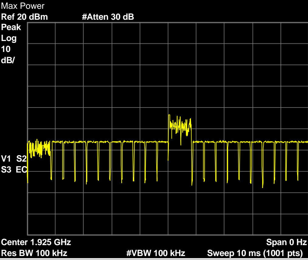
Fig. 93 – Interference profile for the headset EUT that is above the threshold of -74.6\text{dBm} ( T_L + U_M ) WITH an open time slot pair, to ensure the test set up interference synchronization are working correctly, and that the link deferral tests above are valid. Slot pair that is interference free is slots 0 and 1. A traffic link was established validating the test set up.
