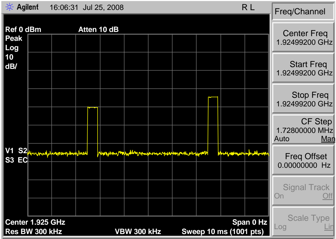
Fig. 69 - Screenshot of spectrum analyzer showing one frame of the channel with the initial interference profile present, which does not block the reception by the base EUT of the headset EUT's transmissions; an acknowledgement is generated when the headset EUT attempts to initiate the communications channel when the TALK button is pressed, and the communications channel is established, so the headset EUT meets the requirements of 8.2.1(b) for proper operation of the test setup when the acknowledgements are unblocked.
