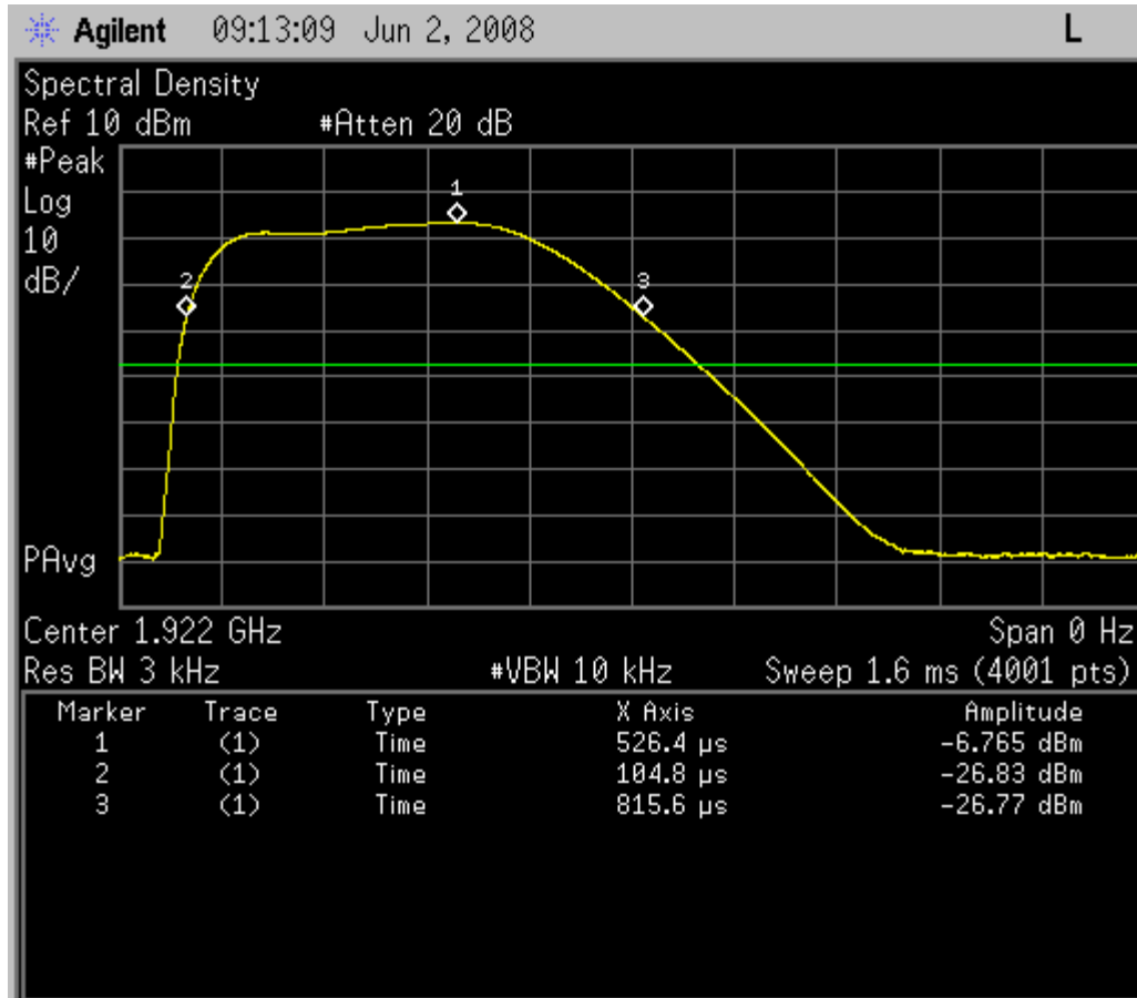
Fig. 14 – Zero-span sweep for headset EUT, low carrier, for 3kHz maximum power spectral density. The peak level is at -6.765 dBm, and the interval between samples at the -20 dB points is from 104.8\mu s to 815.6\mu s, or 710.8\mu s.
