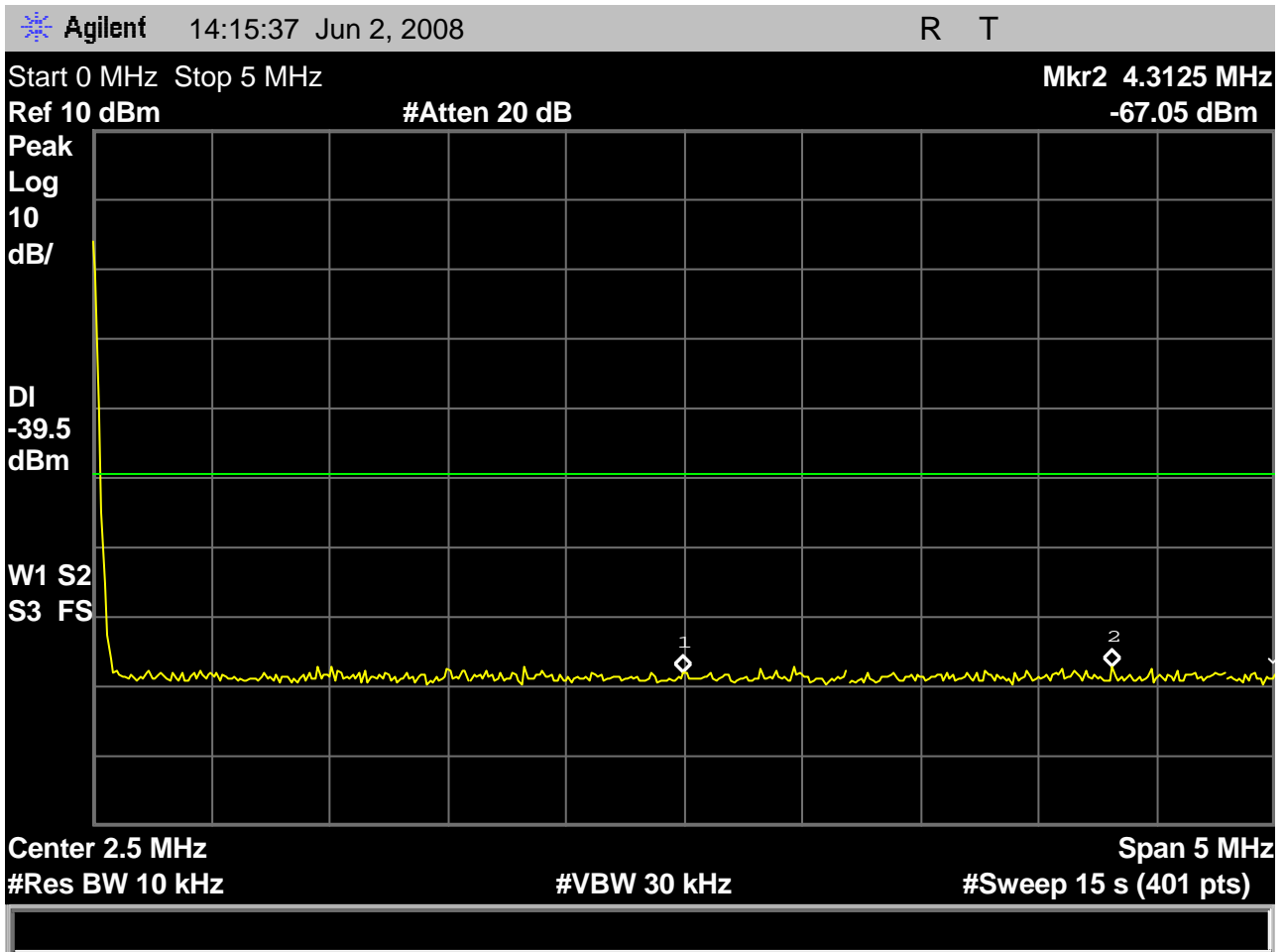
Fig. 32 – headset EUT out-of-band emissions showing the regions from DC to 5MHz, with the transmitter using the highest carrier, 1928.448MHz.
