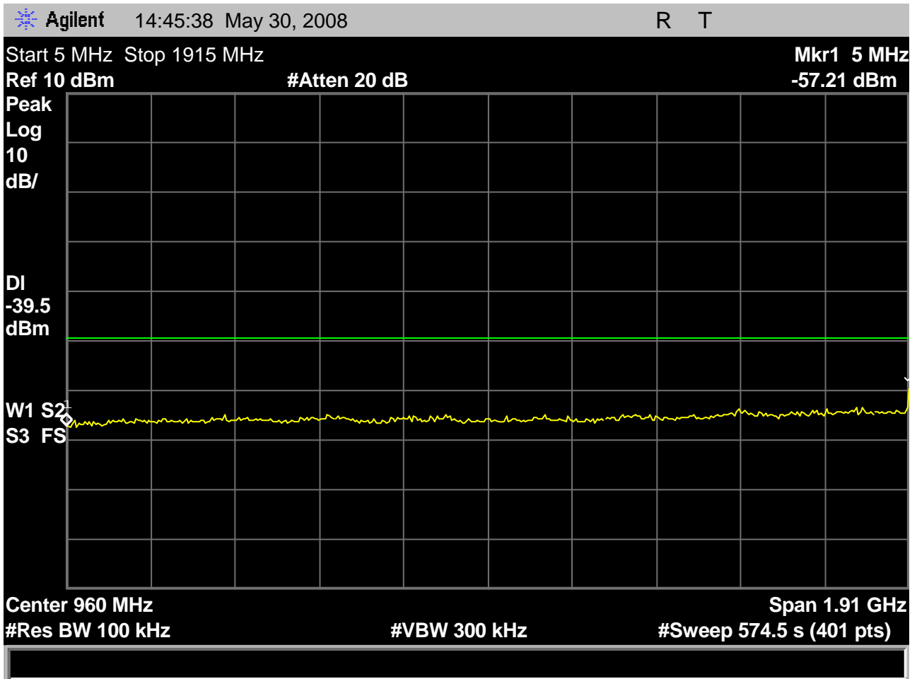
Fig. 33 – headset EUT out-of-band emissions showing the region from 5MHz to 1915MHz, with the transmitter using the highest carrier, 1928.448MHz.
