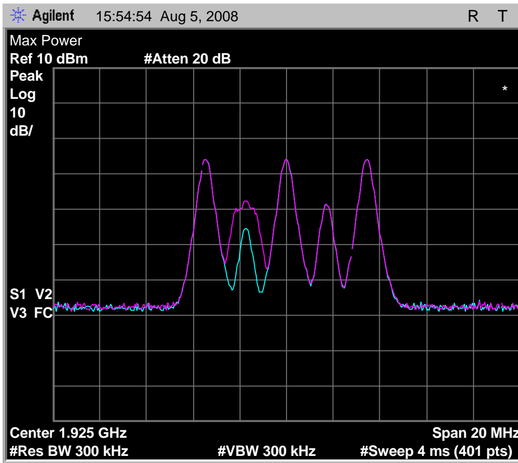
Fig. 101 - Emissions and interference profile spectrum, headset EUT, test 7.3.3(b).
