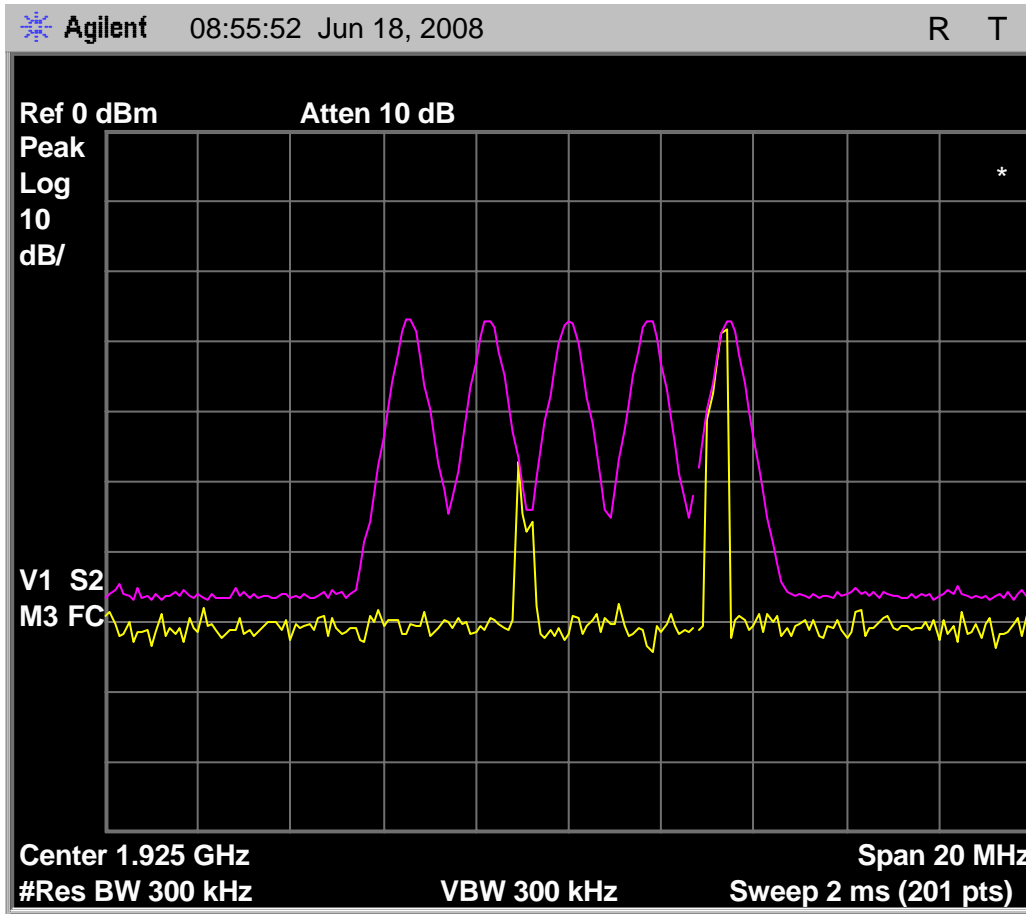
Fig. 88 - Transmit spectrum of 35uS interference pulses in each timeslot for each carrier, with headset EUT deferring due to interference pulses of T_L + U_M + 6dB .
