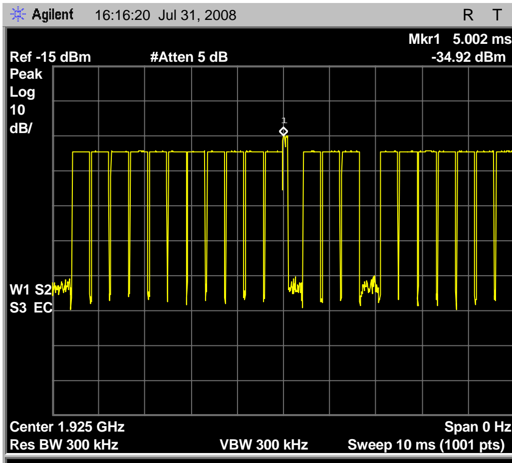
Fig. 80 – Interference profile for the Headset EUT that is above the threshold of -54.6\text{dBm} ( TU + UM ) without an open time slot pair. Slots that are opened are headset transmit slot 0 and headset receive slot 4 (slot 16). Note an additional time slot was opened to provide a place for the Base beacon of the companion device. If the base beacon was to occupy slot 0 or slot 16 a link could not be established and the test would pass but not be valid. Another option would be to force the Base to another carrier, but could not be monitored at the same time as the interference profile of interest.
