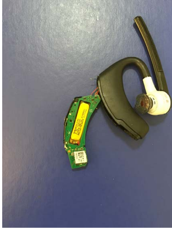
PCBA installed
