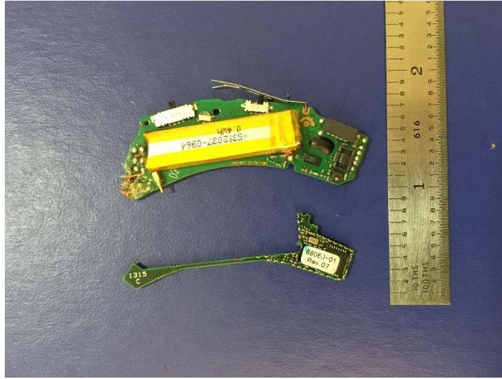
PCBA Top Daughterboard removed
