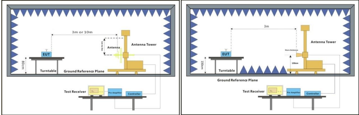
30MHz-1GHz
