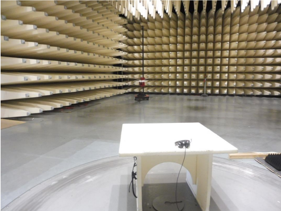
Photo 1: Radiated Emission
