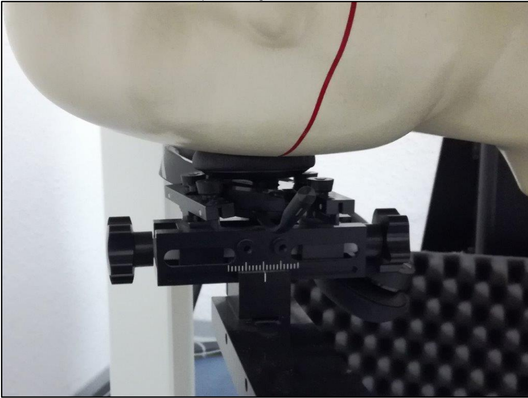
Photo 10: Test position right ear with 0mm distance
