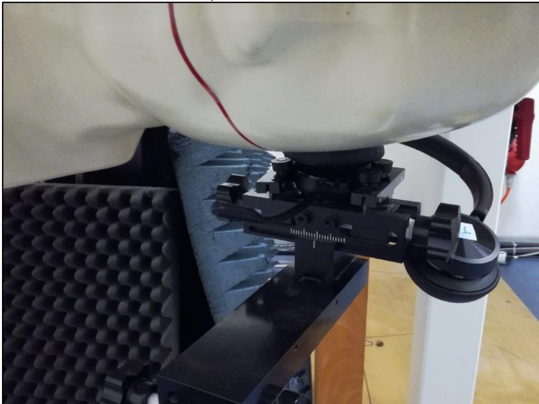
Photo 6: Test position left ear with 0mm distance
