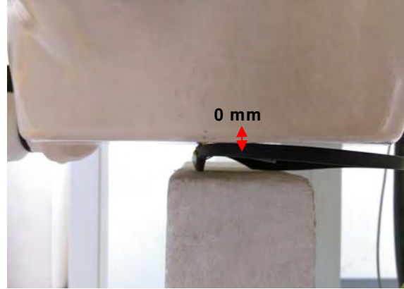
Fig.9 EUT Right side_7 to flat phantom
