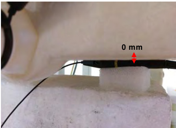
Fig.11 EUT Right side_9 to flat phantom
