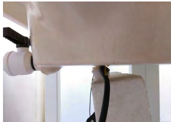
Fig.5 EUT Right side_3 to flat phantom
