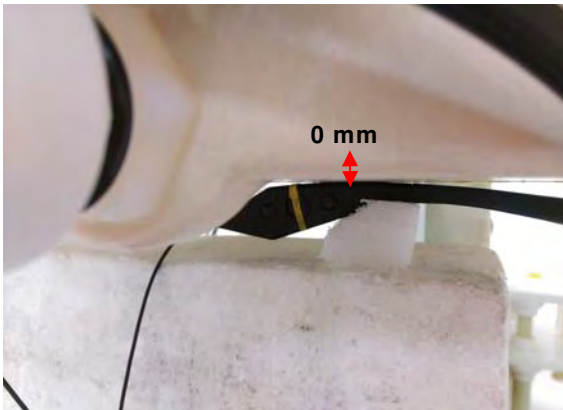
Fig.7 EUT Right side_5 to flat phantom
