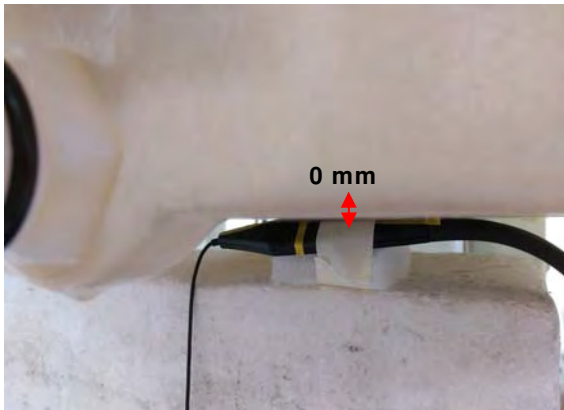
Fig.4 EUT Right side_2 to flat phantom
