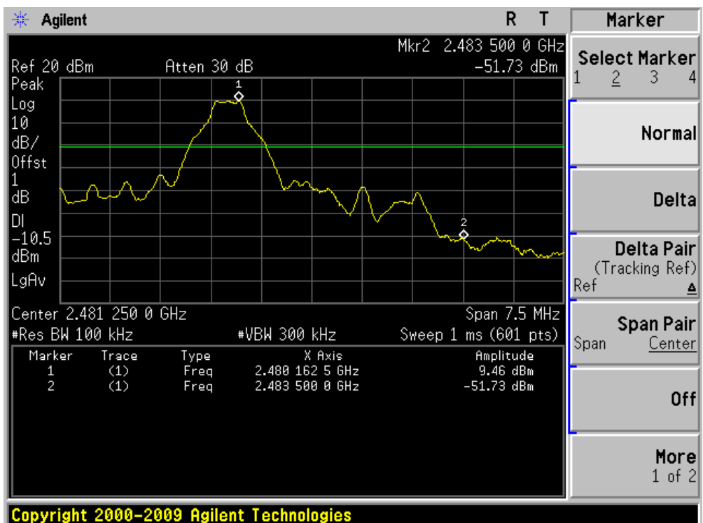
Channel 78 (2480MHz)
