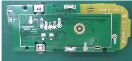
PCB Bottom (Battery Not Installed)
