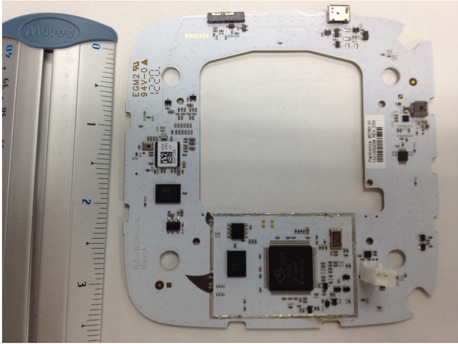
PCB Bottom with Shield Frame Removed
