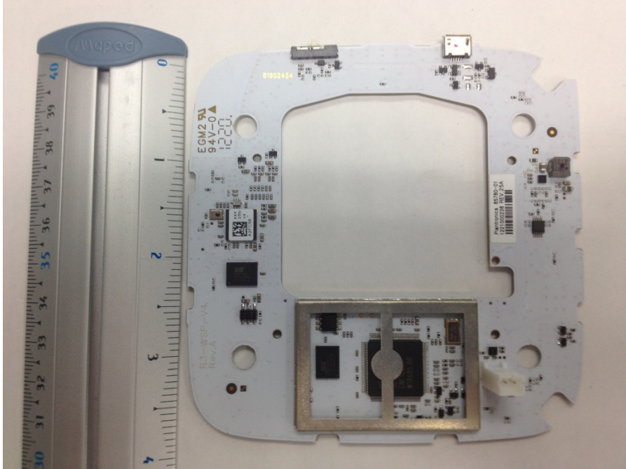
PCB Bottom with Shield Removed
