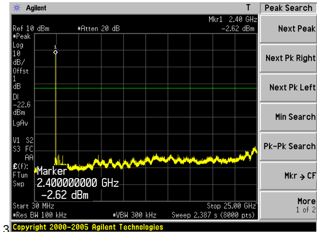
Channel 00 (2402MHz)
