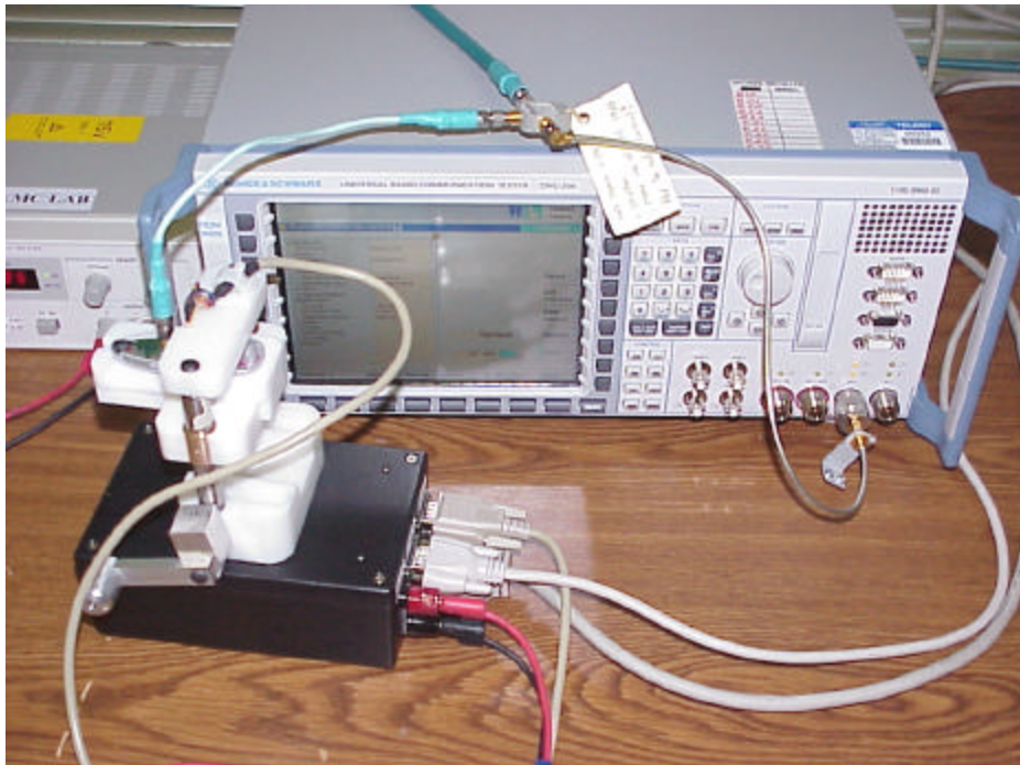
Test setup – conducted measurements-2
