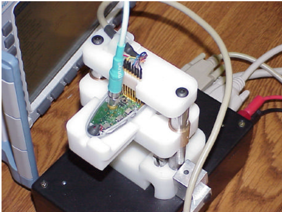
EUT in test fixture
