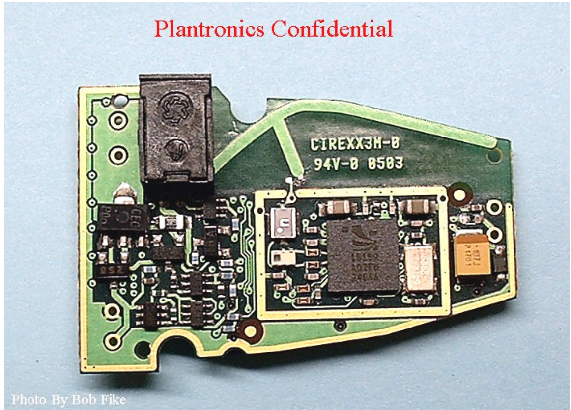
PCB – Bottom view
