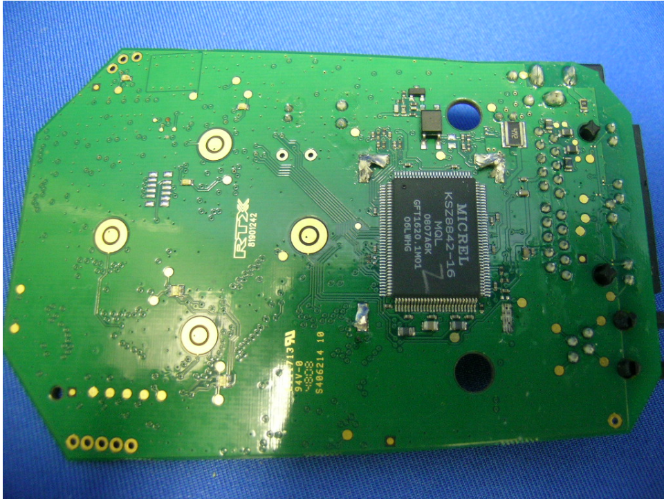
VoIP Headset Adaptor Main PCB solder side
