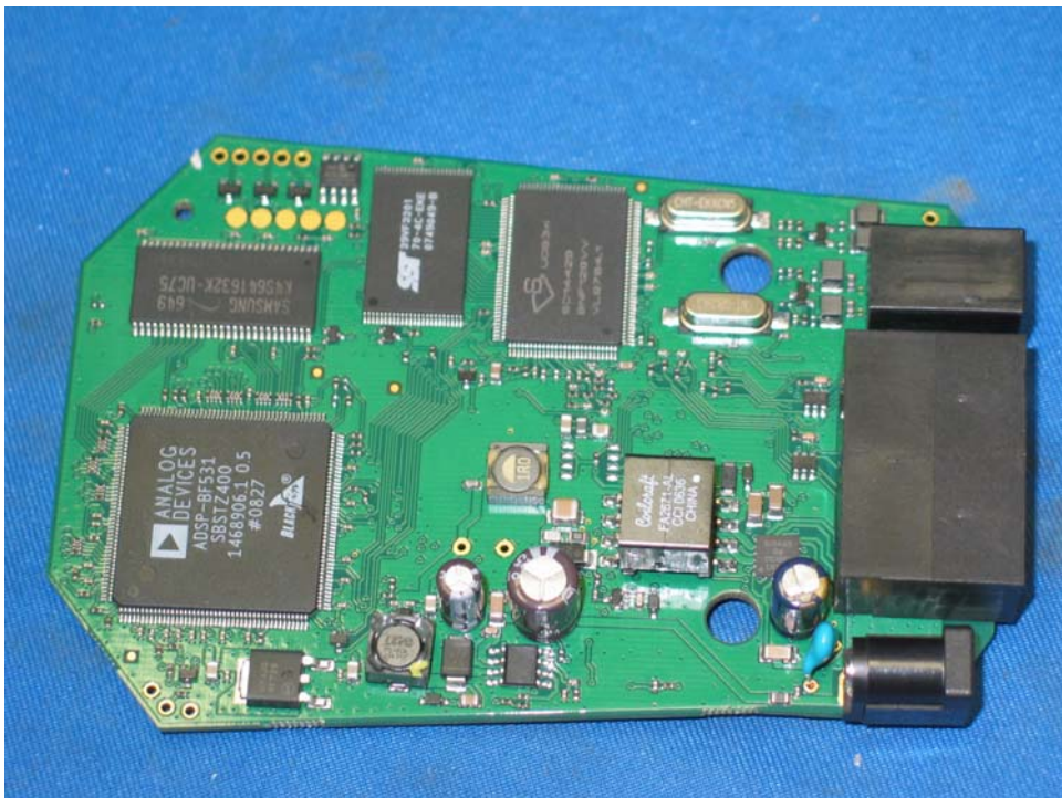
VoIP Headset Adaptor Main PCB comp side
