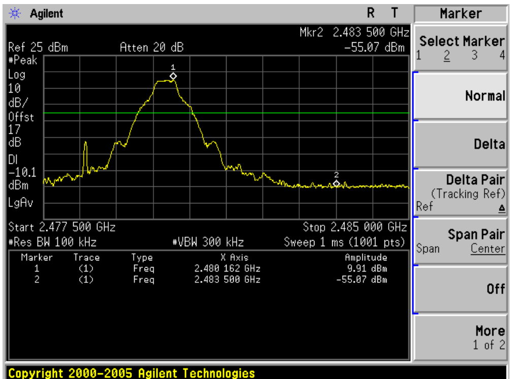
Channel 78 (2480MHz)
