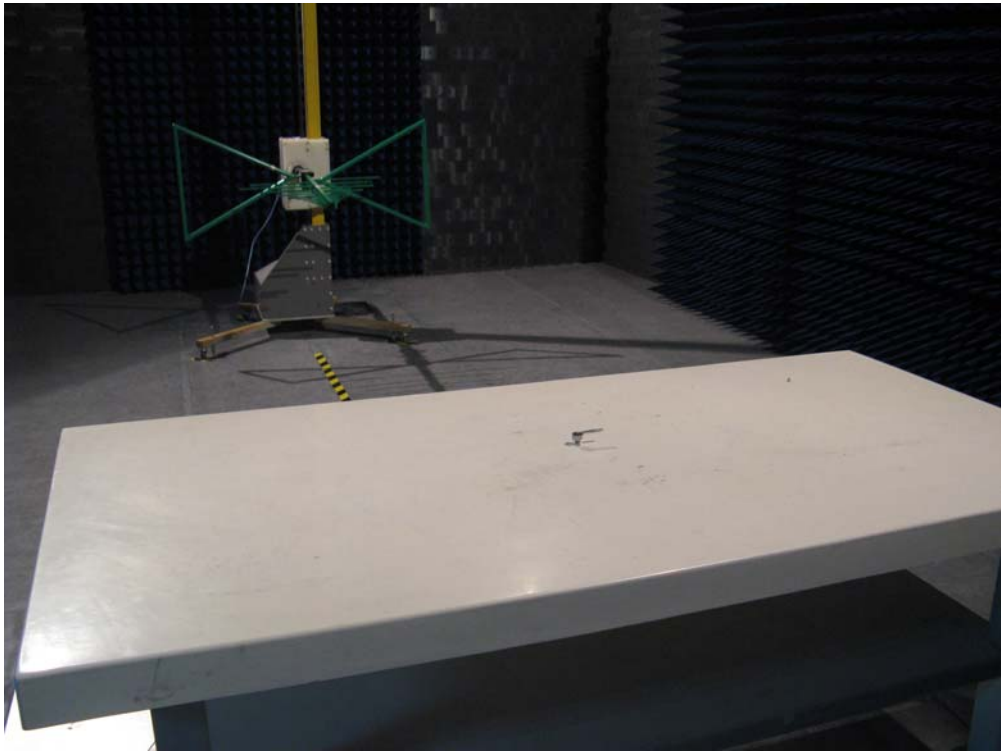
Description : Front View of Radiated Emission Test Setup for Under 1GHz
