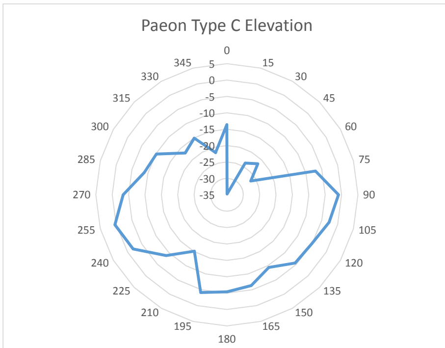
Elevation Peak Gain 0.39dBi
