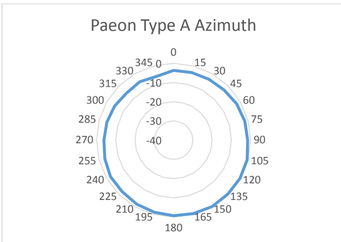
Azimuth Peak Gain -0.053 dBi
