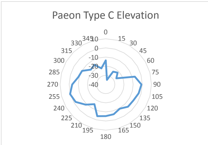
Elevation Peak Gain 0.39dBi
