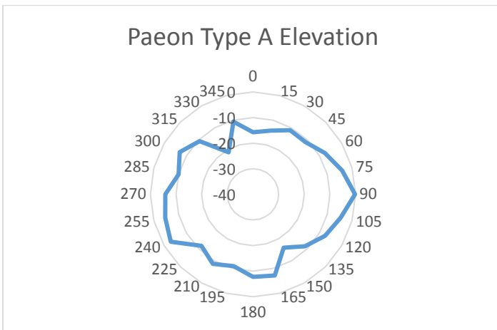
Elevation Peak Gain -0.198i
