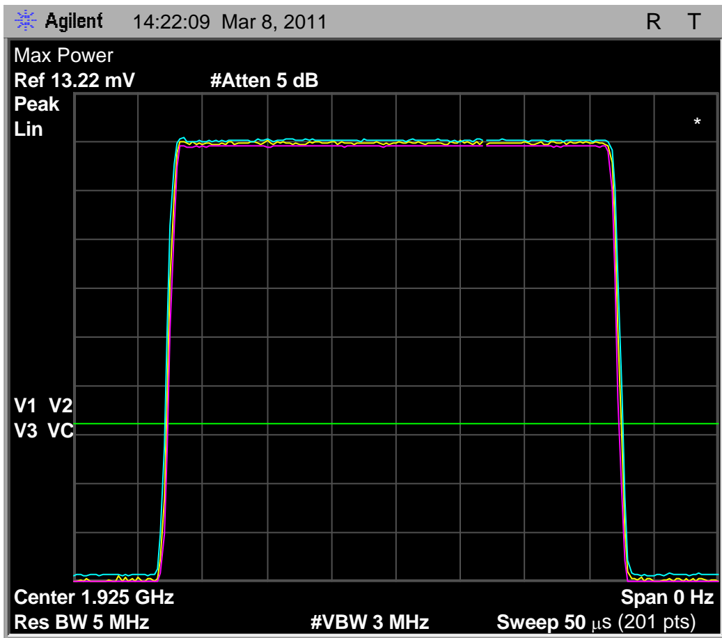
Fig. 55 - 35µs interference pulse for 7.5(d), duration and amplitude variation over the duration of the pulse and over multiple pulses. Spectrum analyzer is set to linear response.
