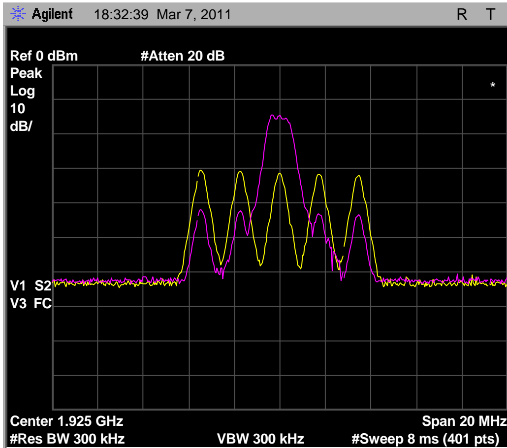
Fig. 53 - Transmit spectrum of 50uS interference pulses, with Base EUT no longer deferring with interference pulses of level T_U - U_M .
