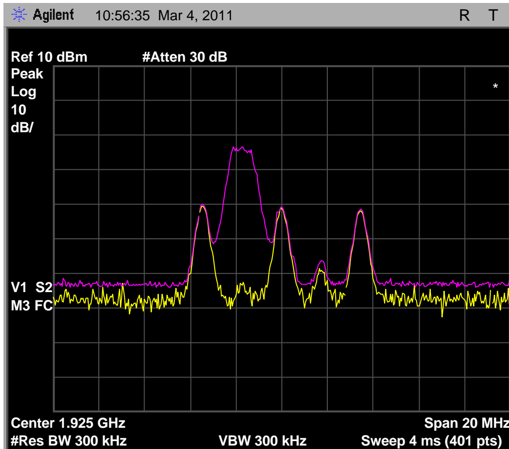
Fig. 46 - Emissions and interference profile spectrum, Base EUT, test 7.3.3(d).
