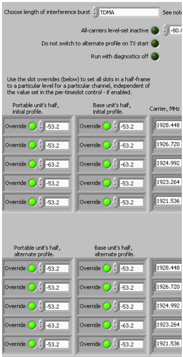
Fig. 61 – Control panel for the multi-carrier interference generator for the test of 8.1.2.
