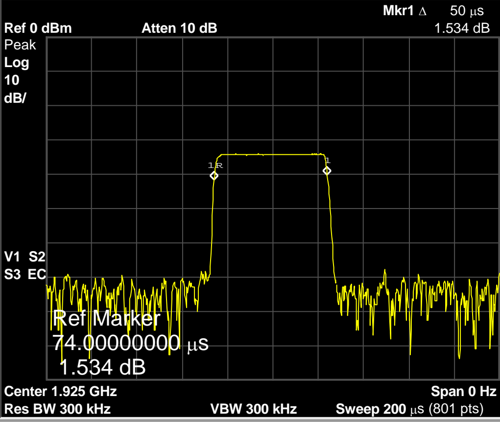
Fig. 49 - Interference pulse, one frame shown, for the test of 7.5(c).
