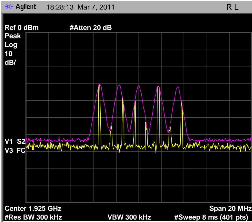
Fig. 52 - Base EUT shown deferring when all channels are blocked with 50uS pulses at T_U + U_M . Top (purple) trace is max hold showing interference only with no Base EUT RF transmissions. Bottom (yellow) trace is an instantaneous capture of individual pulses.
