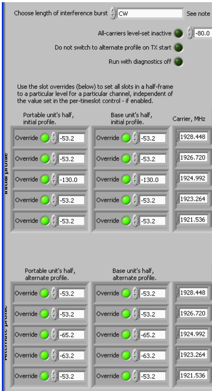
Fig. 63 - PXI-5670 multi-carrier interference generator control panel for the test of 8.2.1(c), for the Base EUT.
