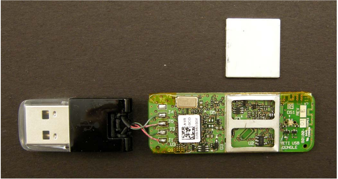
Top PCB Shield cap removed
