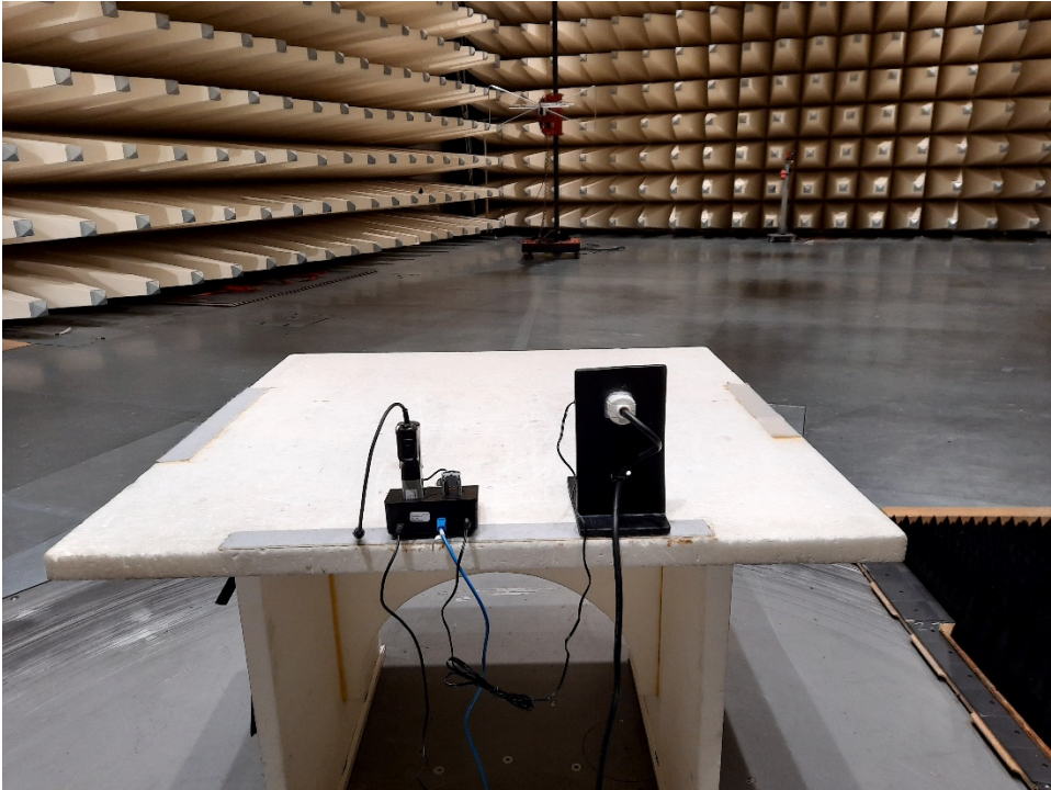
Photo 1: Radiated Emission
