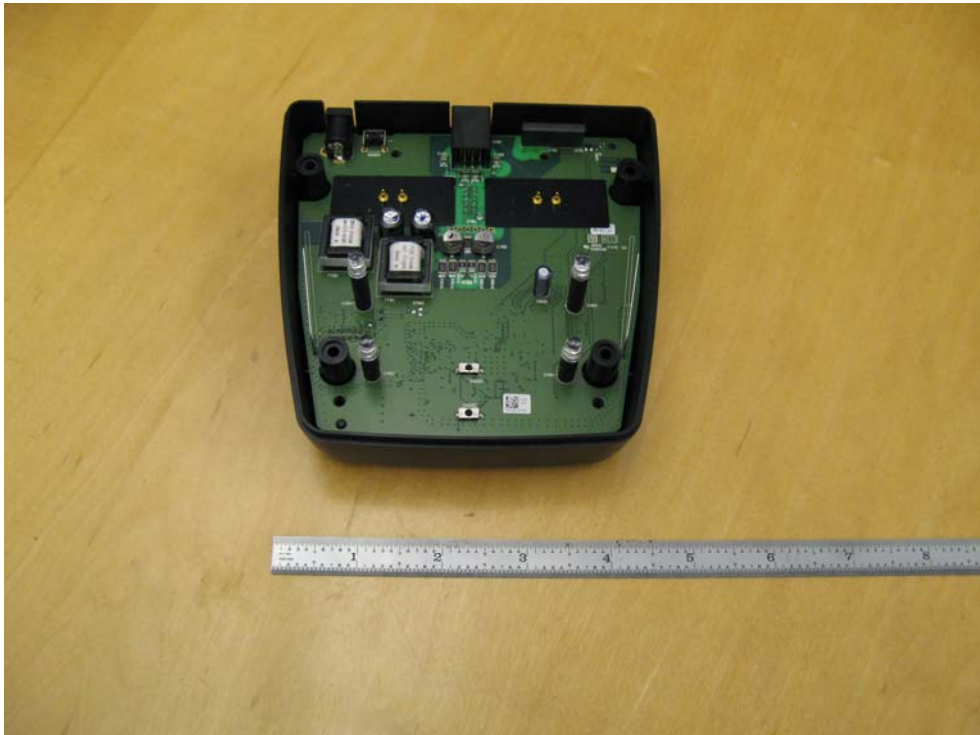
PCB Installed
