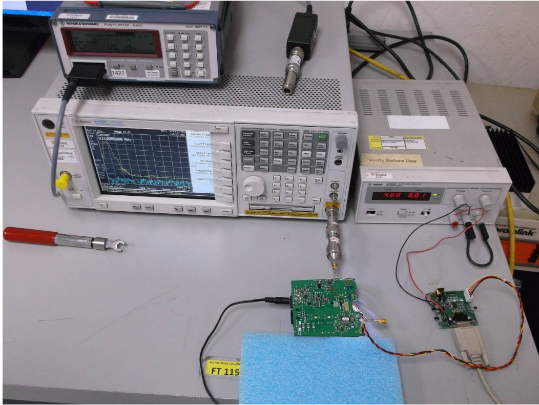
Antenna Port
