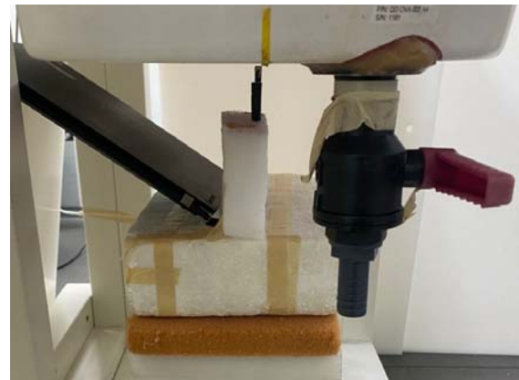
Fig.5 EUT Tip_with cable side to flat phantom
