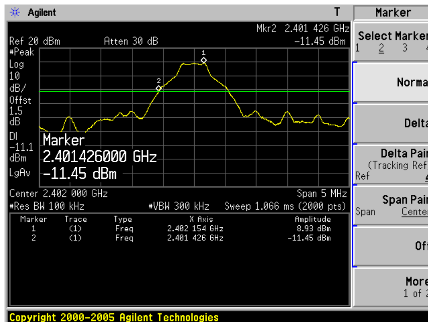
Channel 00 (2402MHz)
