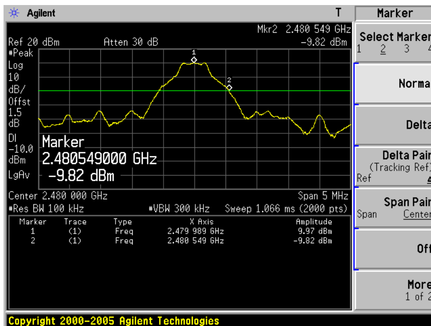
Channel 78 (2480MHz)
