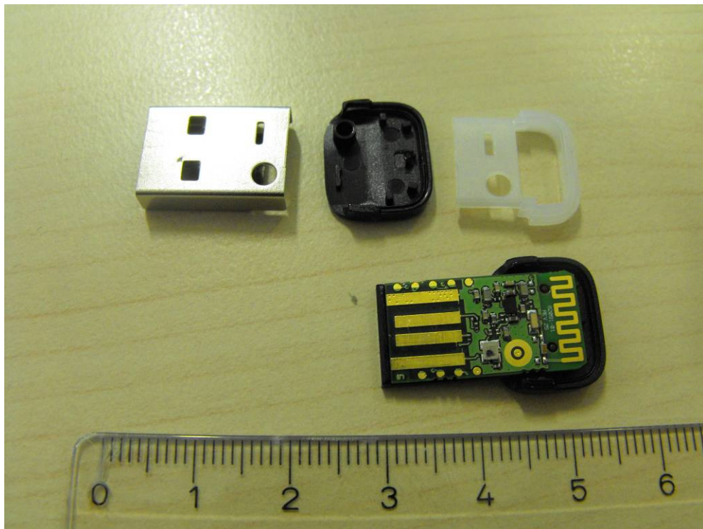
Photo 7: radiated sample
