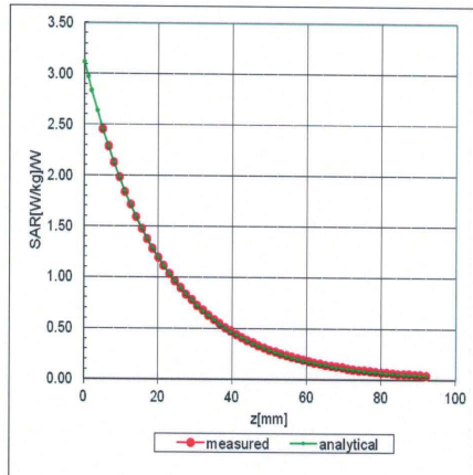
f=750 MHz, WGLS R9(H_convF)
