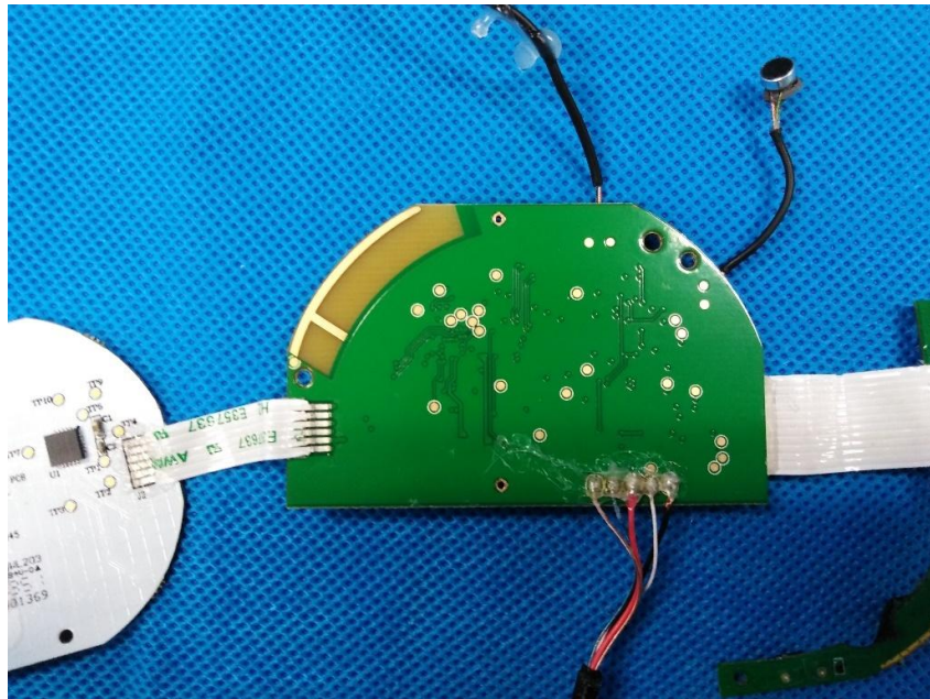
BT Antenna
