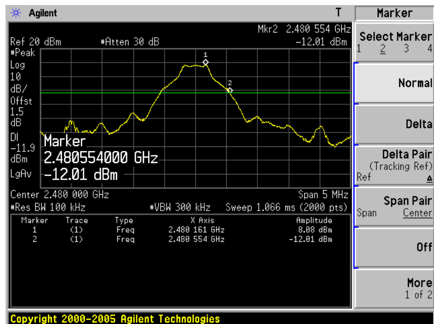
Channel 78 (2480MHz)
