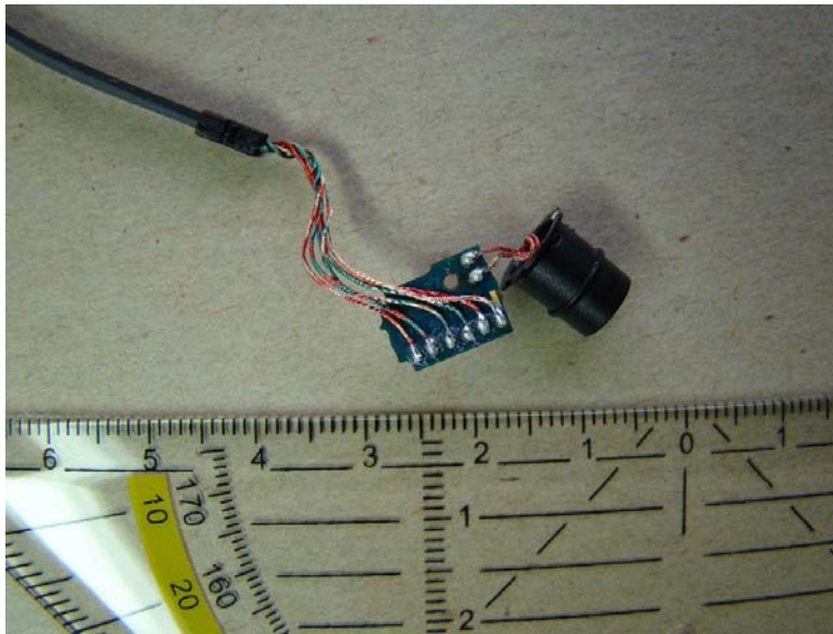
Right PCBA Connector Top
