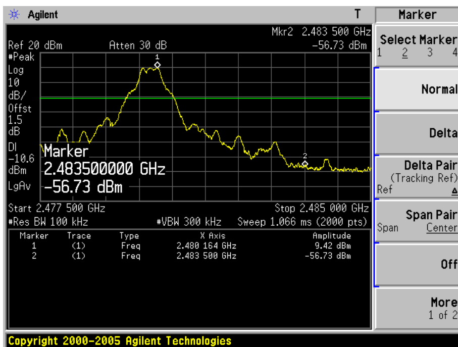
Channel 78 (2480MHz)
