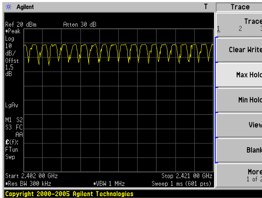
2402 - 2421 MHz
