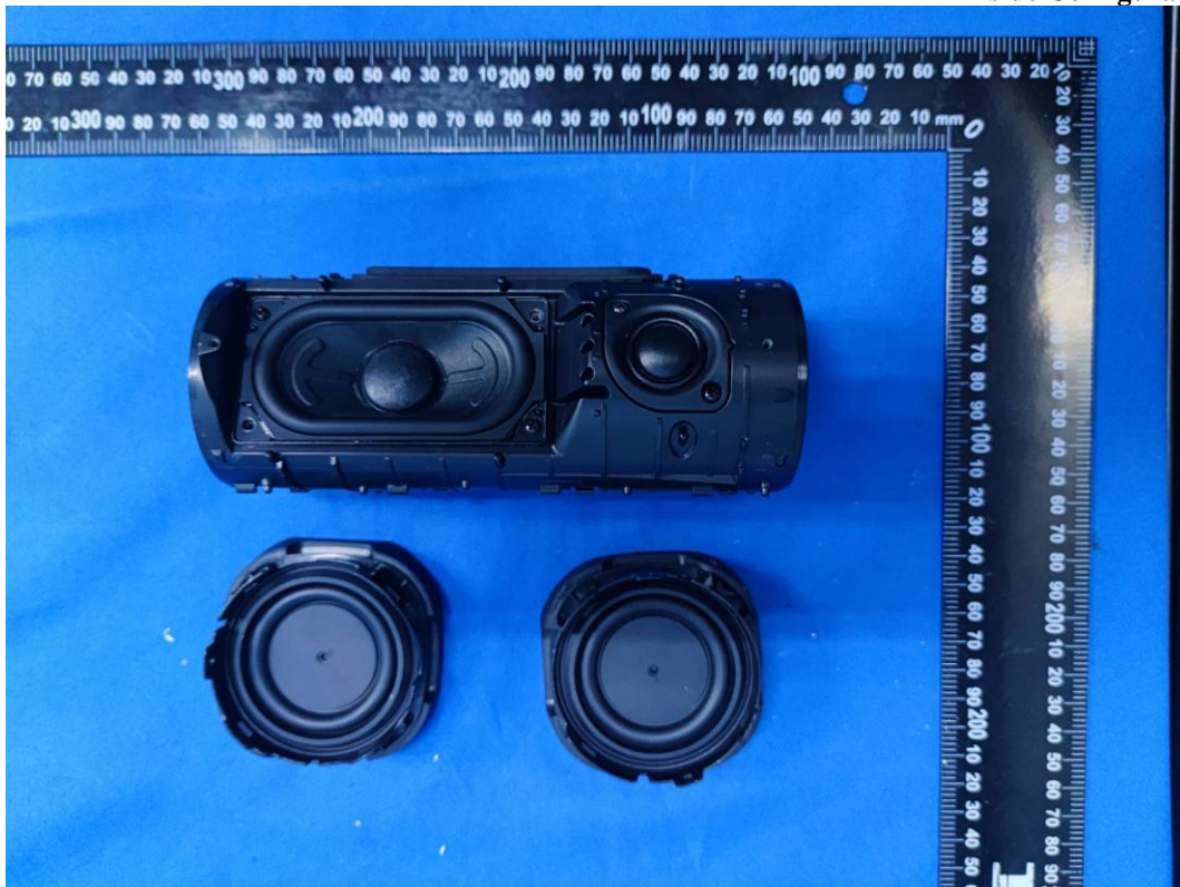
Figure 2 Inside Configuration of the EUT
