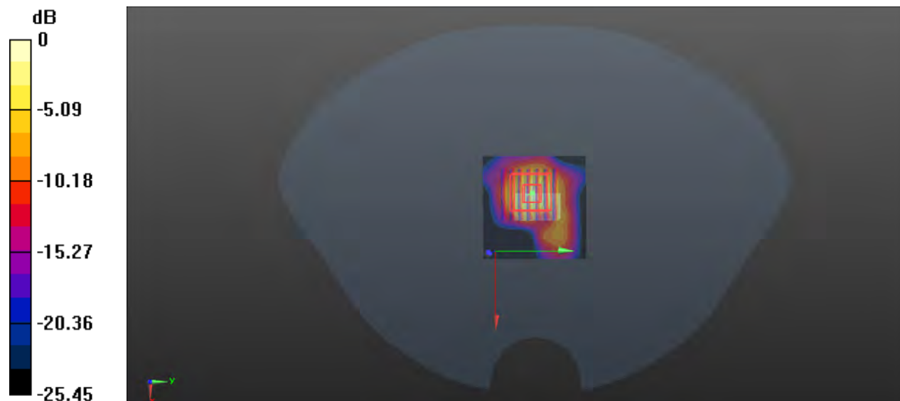
0 dB = 0.141 W/kg
