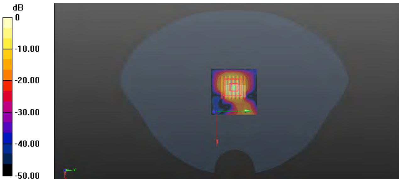
0 dB = 0.399 W/kg
