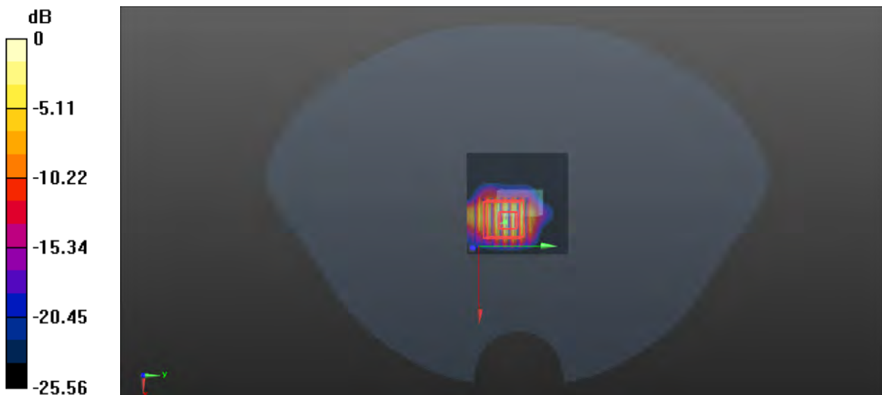
0 dB = 0.133 W/kg
