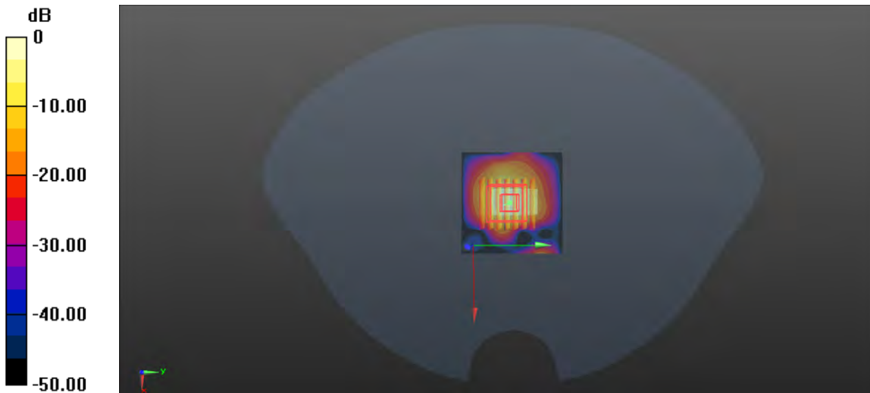
0 dB = 0.295 W/kg
