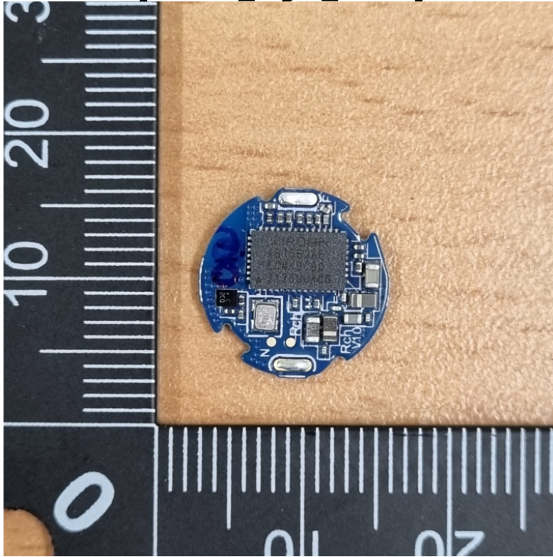
[Earbud_Right_Board]
