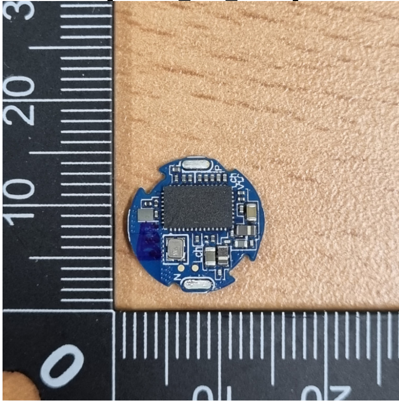
[Earbud_Left_Board]
