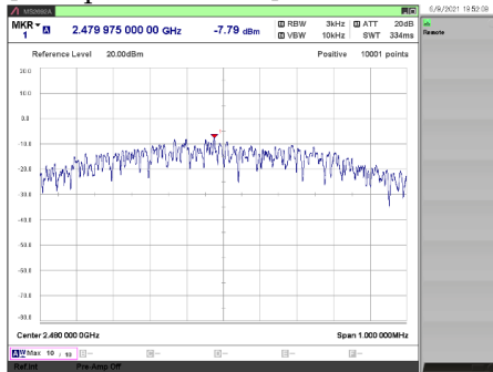
[1 Mbps / 2480 MHz]
