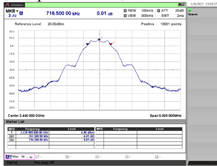
[1 Mbps / 2440 MHz]
