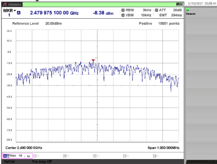
[1 Mbps / 2480 MHz]
