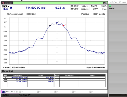
[1 Mbps / 2402 MHz]
