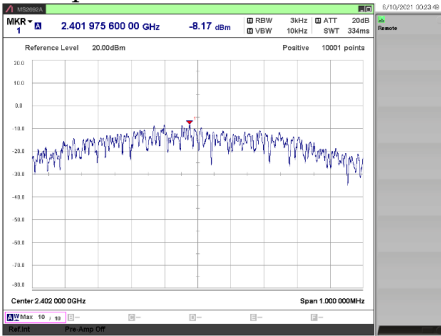
[1 Mbps / 2402 MHz]
