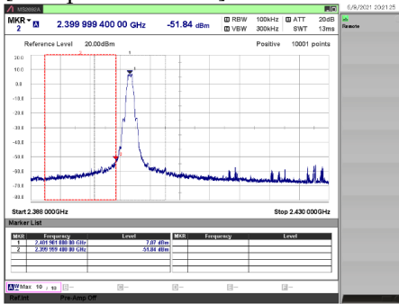
[1 Mbps / 2402 MHz]
