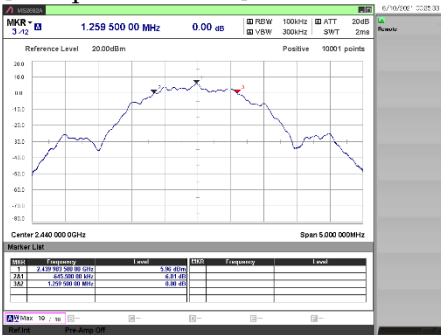
[2 Mbps / 2440 MHz]
