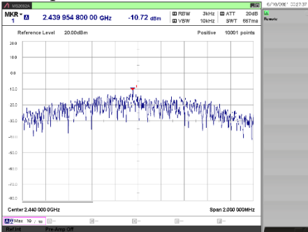
[2 Mbps / 2440 MHz]
