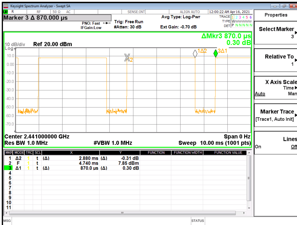
Equation 8-2 Bluetooth Duty Cycle Calculation for Left ear
