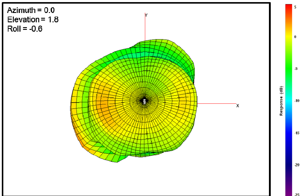
Free-Space Total Gain, Top View, 2476MHz
