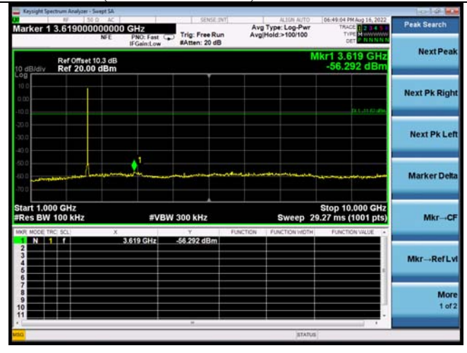
2440MHz(1GHz – 10GHz)
