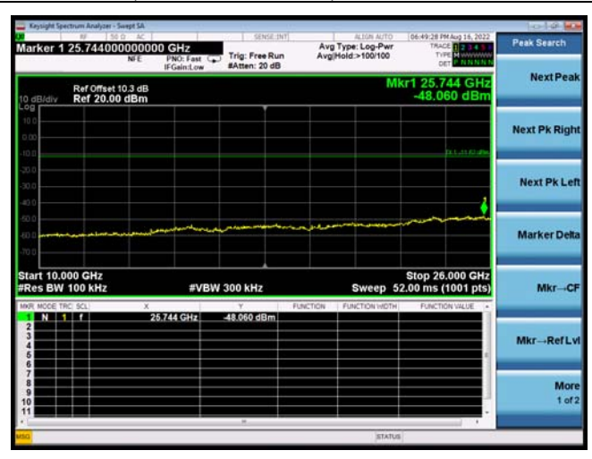
2440MHz(10GHz – 26GHz)
